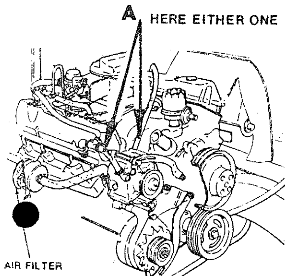
An early-model air injection system.
