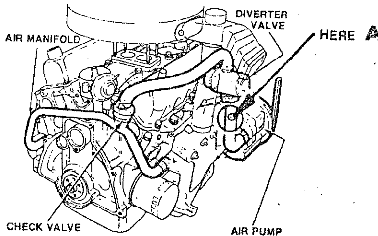
A late-model air injection system. It has fewer parts than the earlier systems. (Ford)
