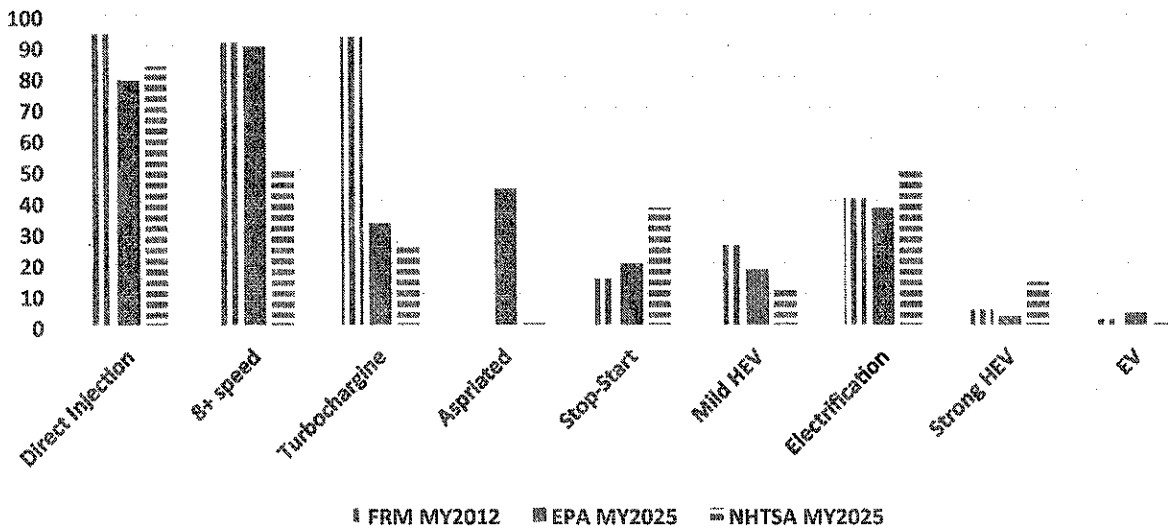
FIGURE 3: PENETRATION OF SPECIFIC TECHNOLOGIES INTO THE FLEET (IN PERCENT)
