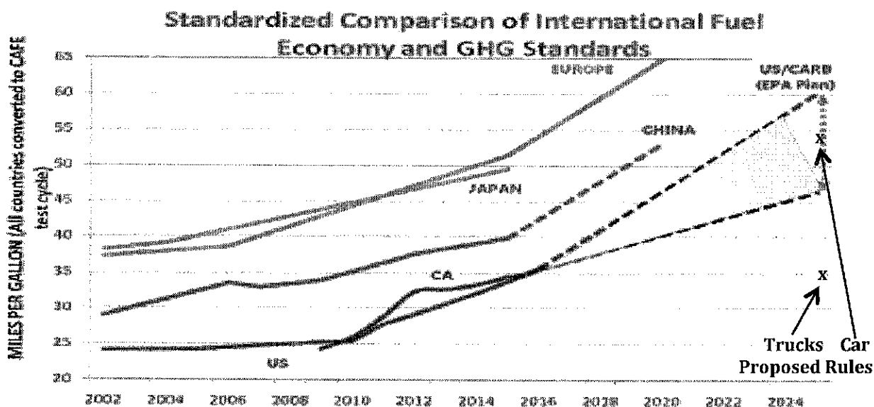
Figure 3: Comparison of Proposed Standard with International Standards
