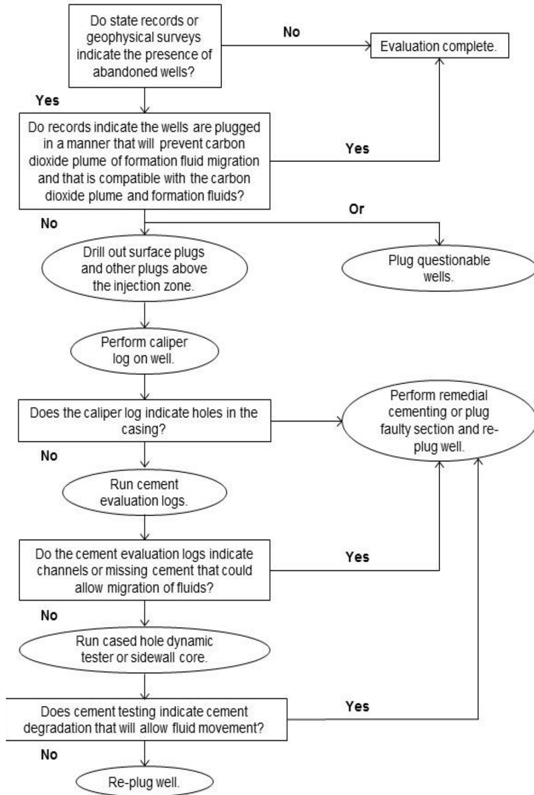
Figure 2. Well evaluation flow chart
