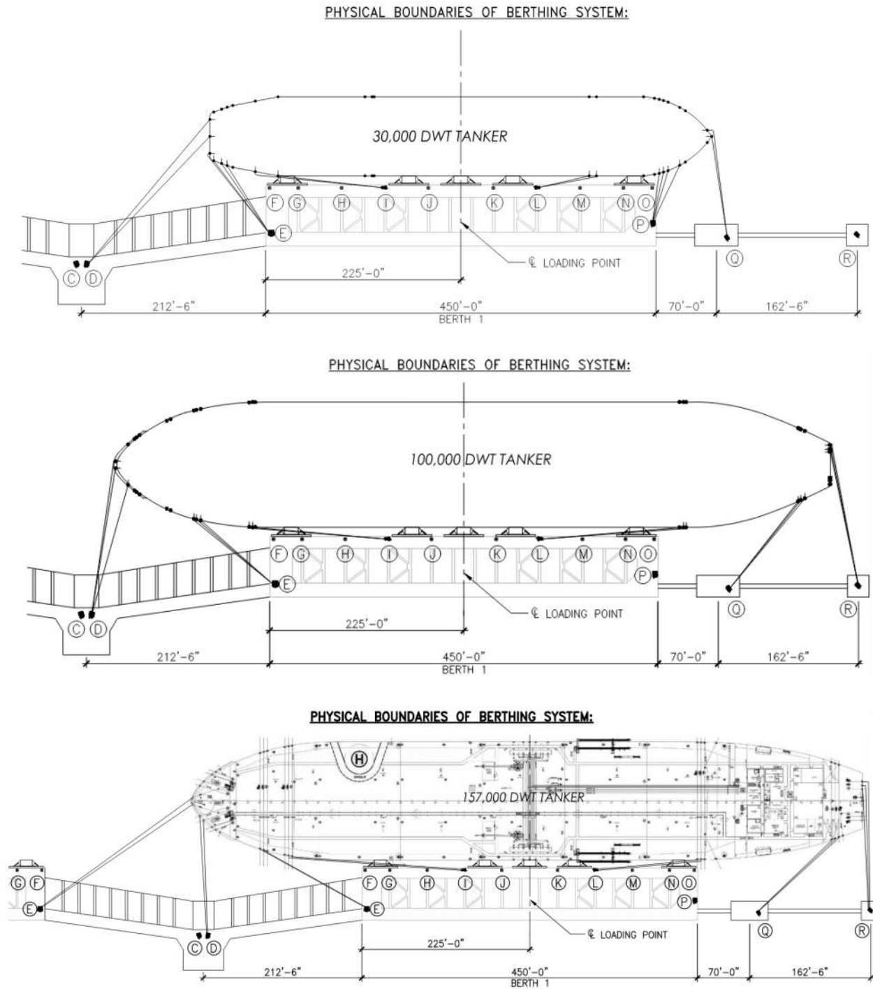
Figure 14 - Example Mooring Configurations with Lines at Stern for Various Size Vessels. (From Attachment 4, Sheets 13, 18, and 20A)
