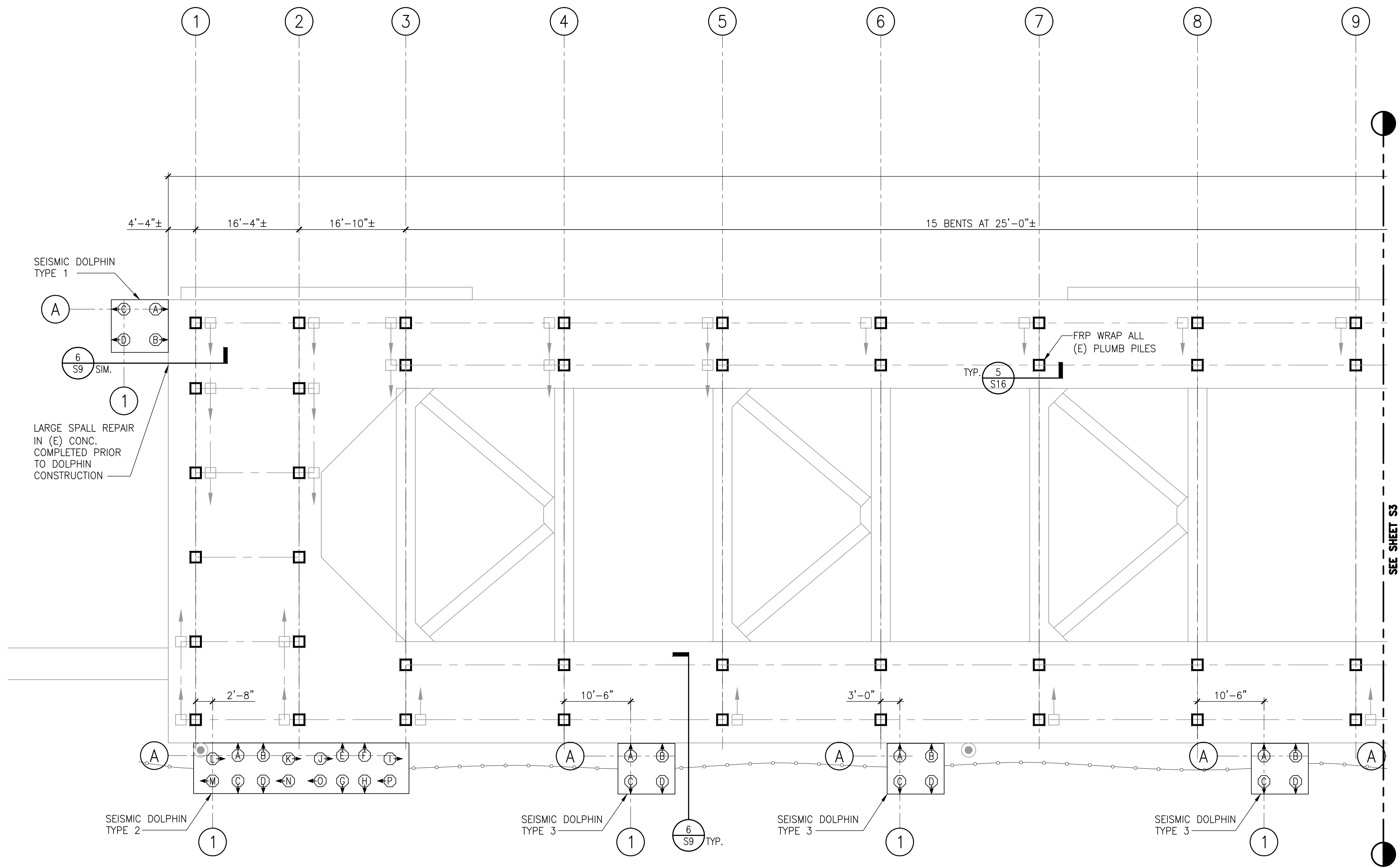
1 PARTIAL DOWNSTREAM LOADING PLATFORM PILE PLAN SCALE: 1"=10'-0"
