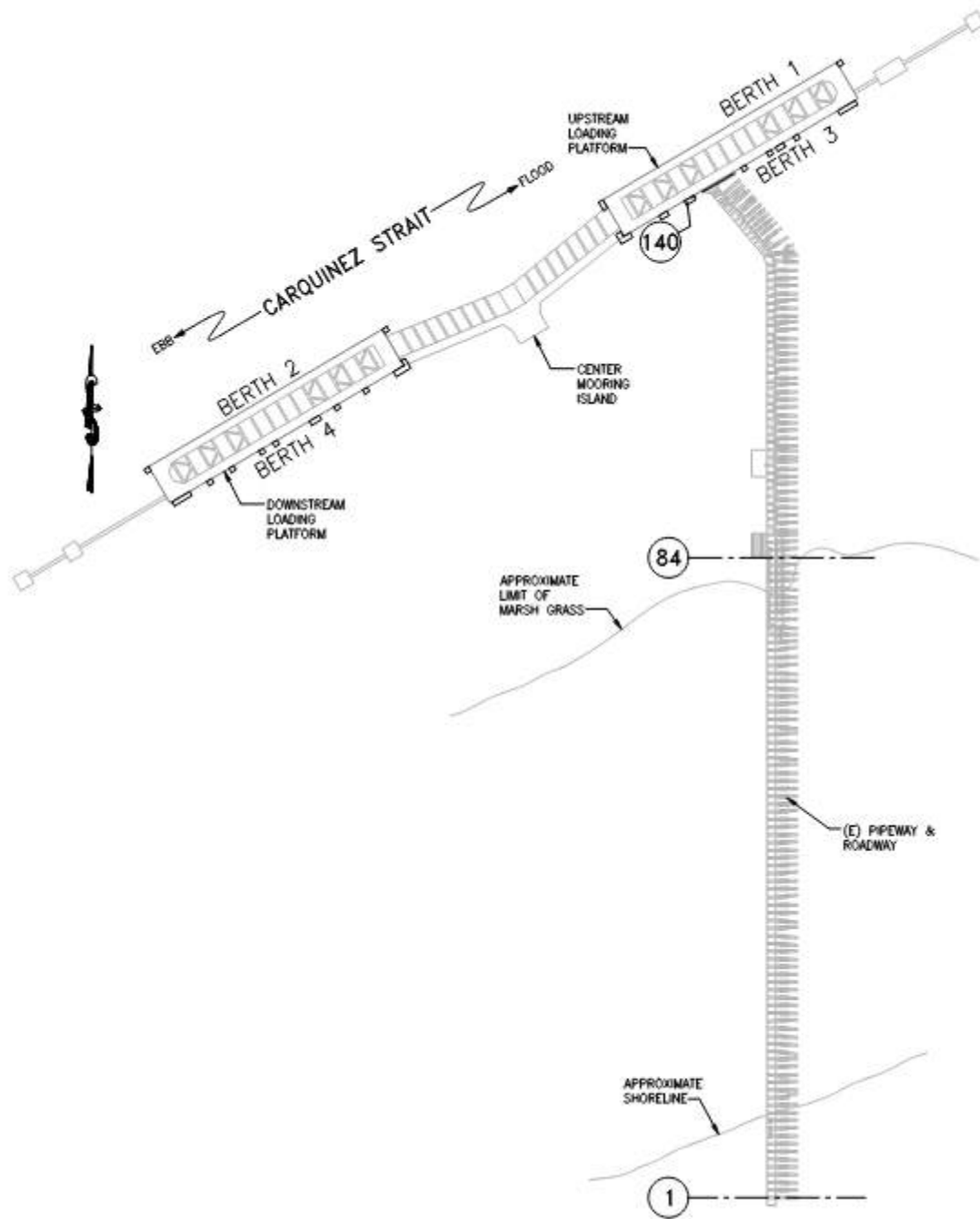
Figure 2 – Terminal Plan
