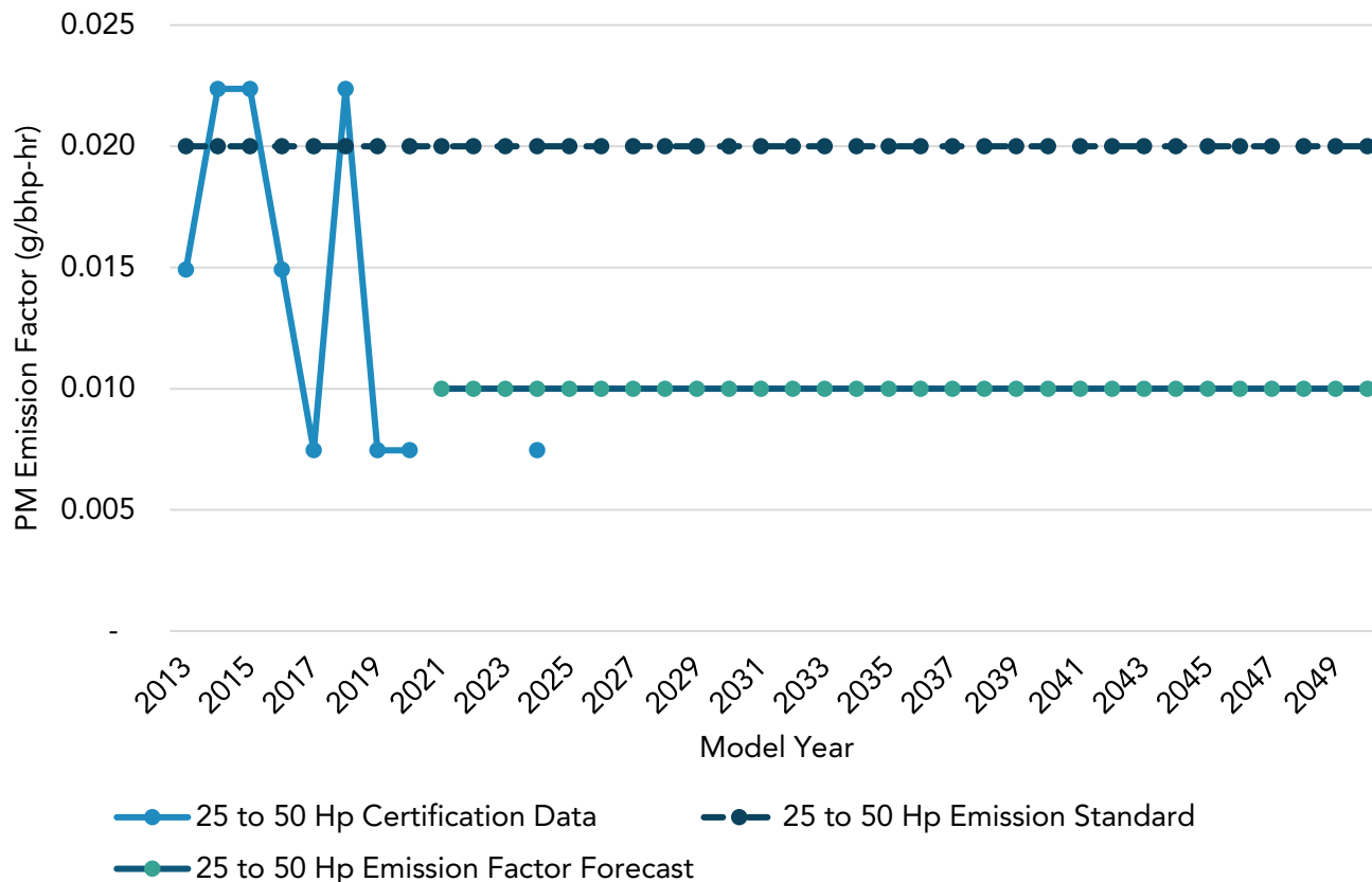
Figure 22. PM Emission Factors for 25 to 50 Horsepower
