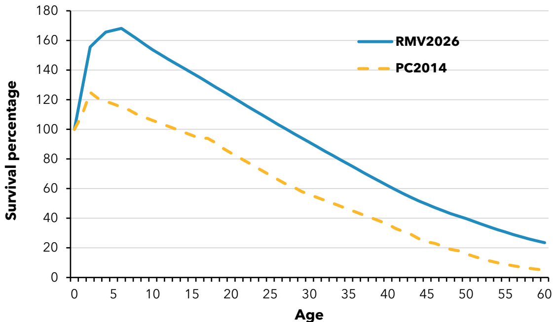
Figure 8: Outboard Survival Curve
