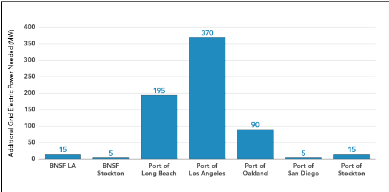
Figure F-2: Additional Load Capacity Needed to Support Fully Zero-Emission CHE by Facility
