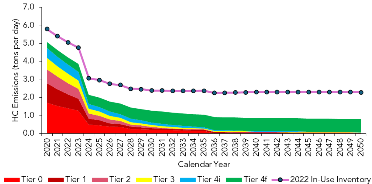
Figure 3. Comparison of Statewide HC Emissions
