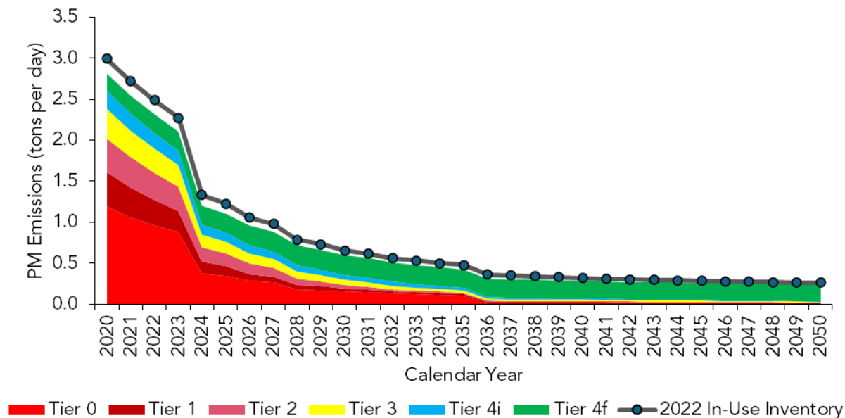
Figure 2. Comparison of Statewide PM Emissions
