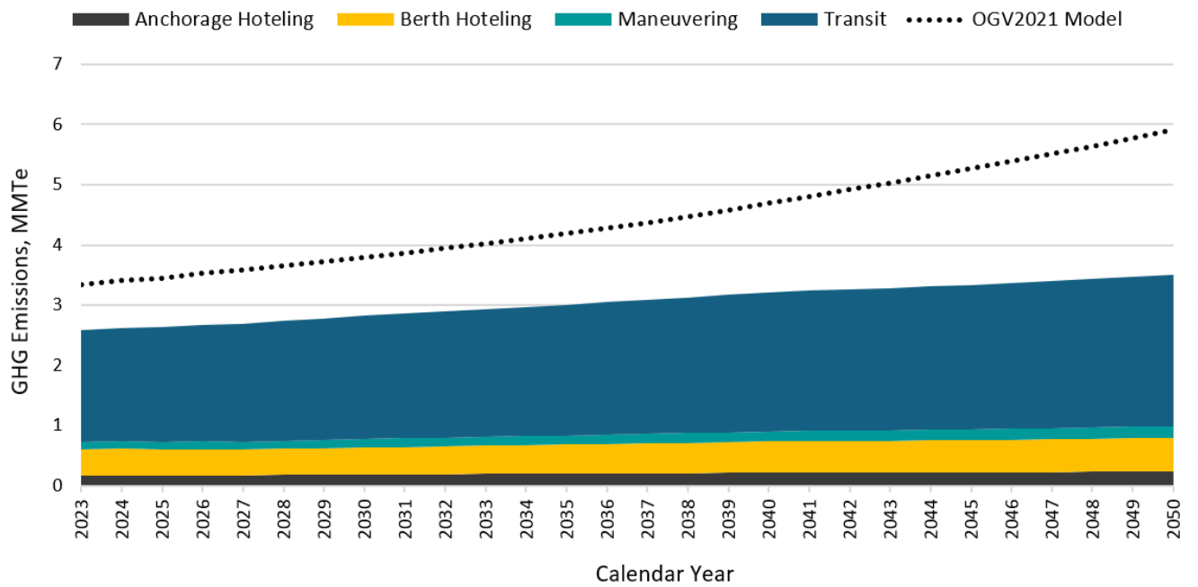
Figure 21. Statewide GHG emissions from OGVs out to 100 nautical miles by mode
