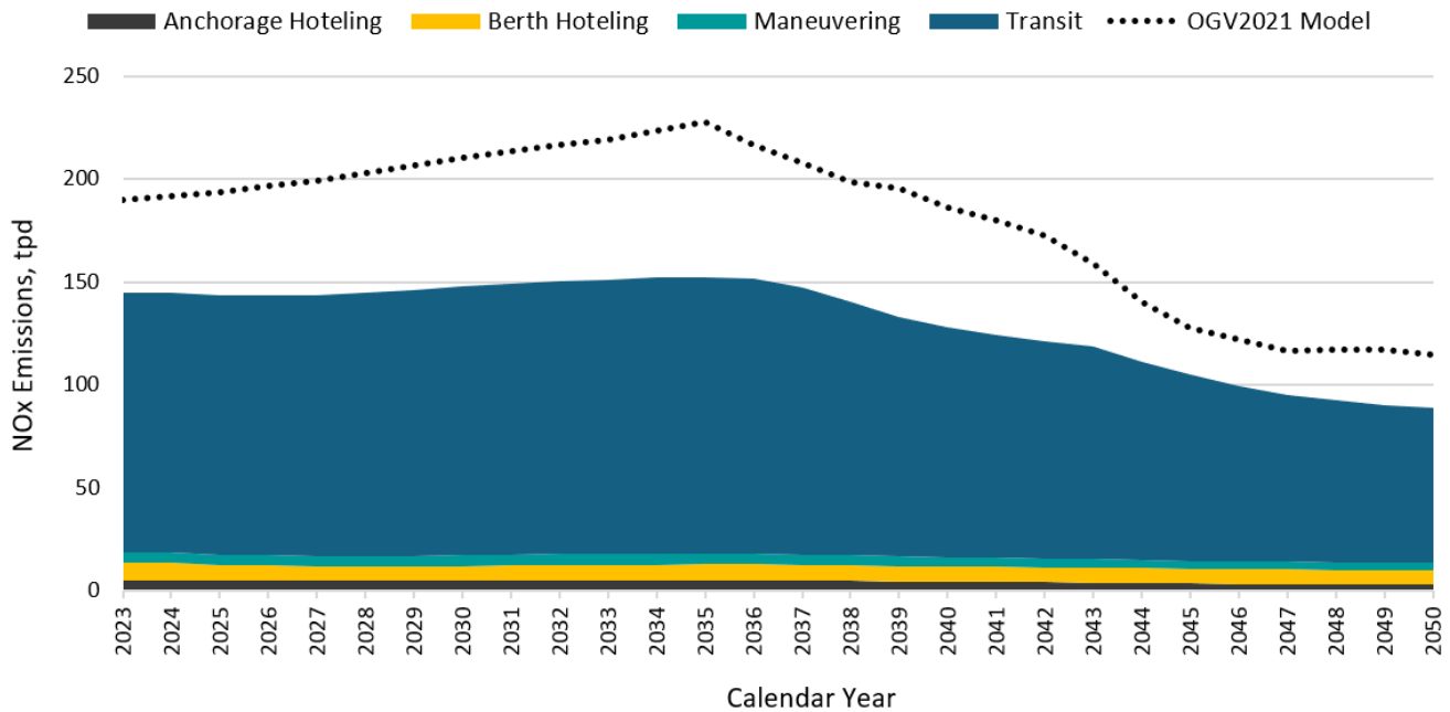
Figure 19. Statewide NOx emissions from OGVs out to 100 nautical miles by mode
