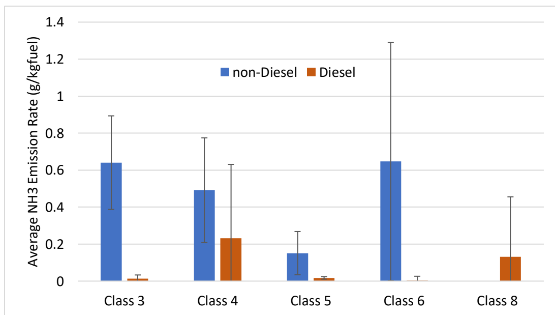
Figure D-7. Average \text{NH}_3 emission rates from HDVs by fuel type and truck class for the Stockton campaign. Error bars indicate 95% CI
