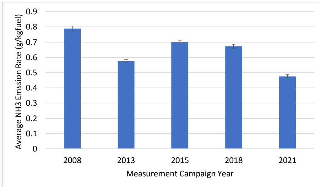
Figure D-4. Overall average \text{NH}_3 emission rate observed at the La Brea RSD site by campaign year. Error bars indicate 95% CI.
