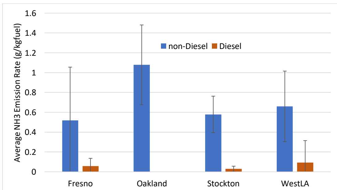
Figure D-5. Average \text{NH}_3 emission rates from HDVs by campaign and fuel type. Error bars indicate 95% CI.
