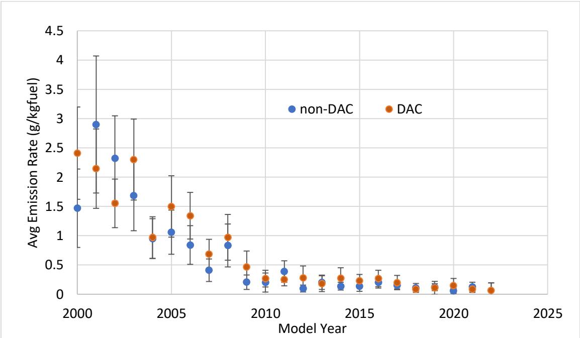
Model Year Average NO Emission Rates – Bakersfield
