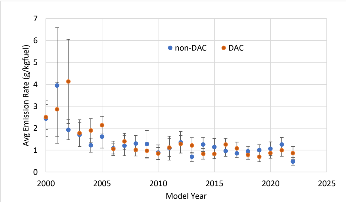
Model Year Average HC Emission Rates – City of Industry
