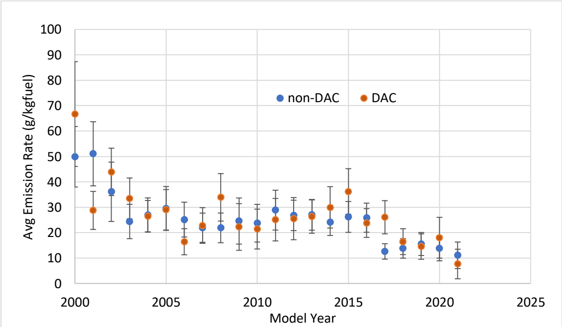
Model Year Average CO Emission Rates – Stockton
