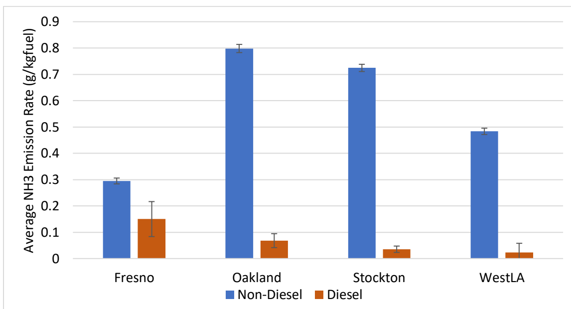
Figure D-1. Average \text{NH}_3 emission rates of LDVs by campaign and fuel type. Error bars represent 95% confidence intervals (CI).
