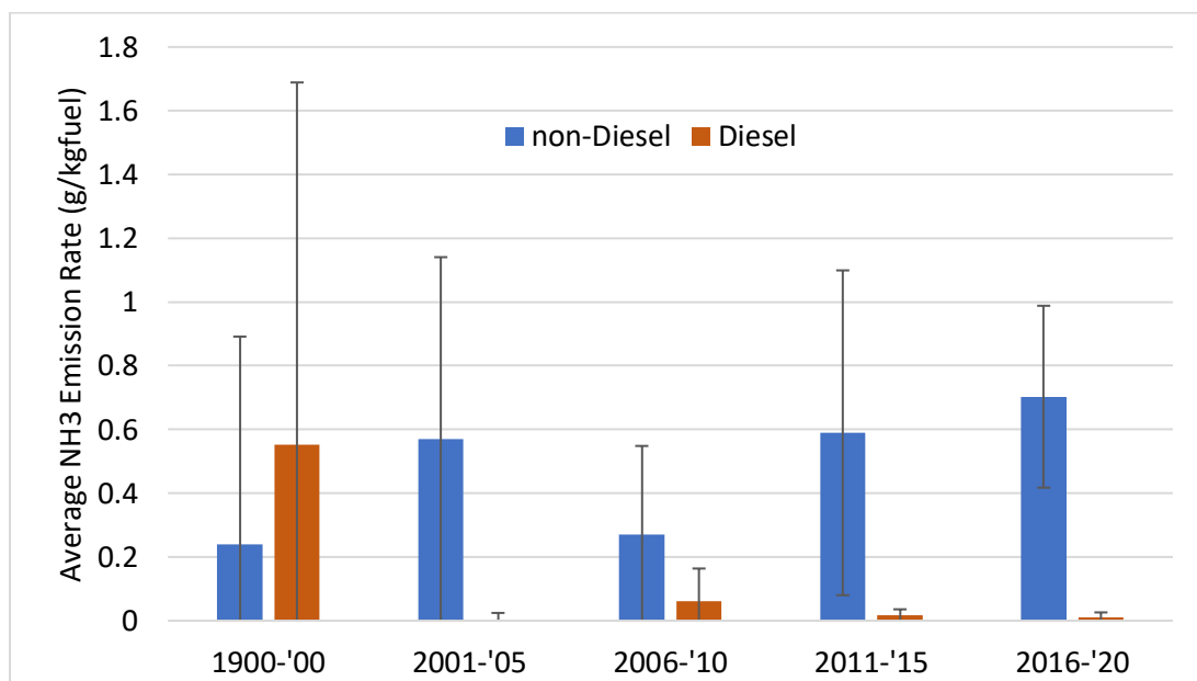
Figure D-6. Average \text{NH}_3 emission rates from HDVs by fuel type and model year bin for the Stockton campaign. Error bars indicate 95% CI.
