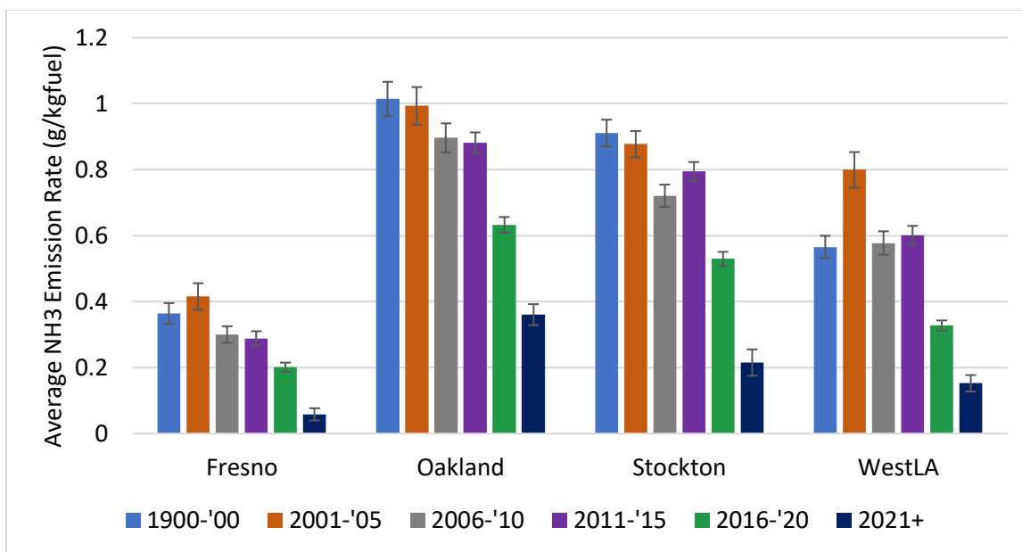
Figure D-2. Average LDV NH 3 emission rates by campaign and model year bin (excluding diesel-powered vehicles). Error bars represent 95% CI.
