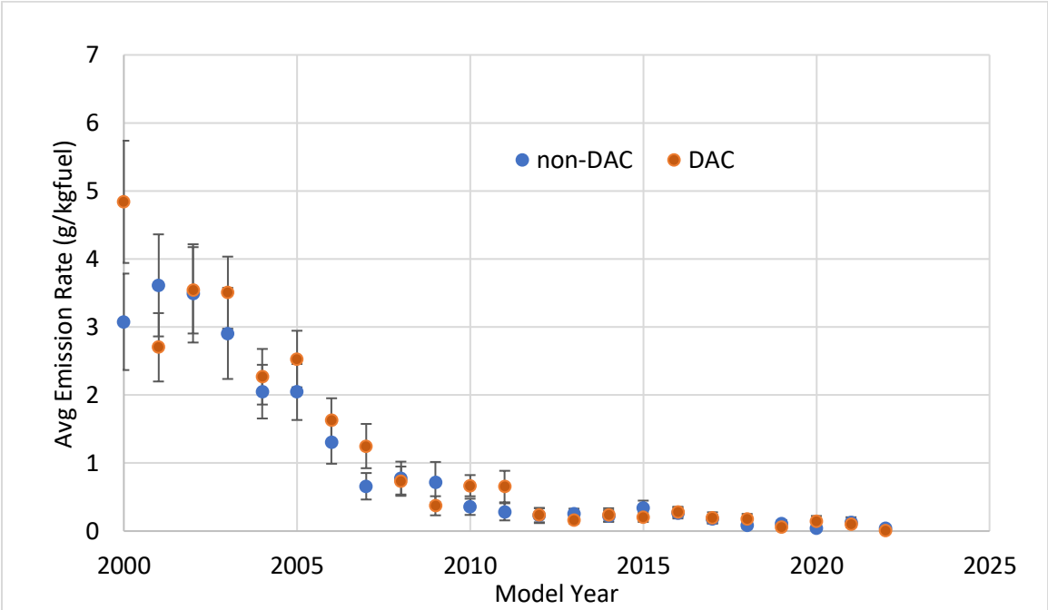
Model Year Average NO Emission Rates – City of Industry
