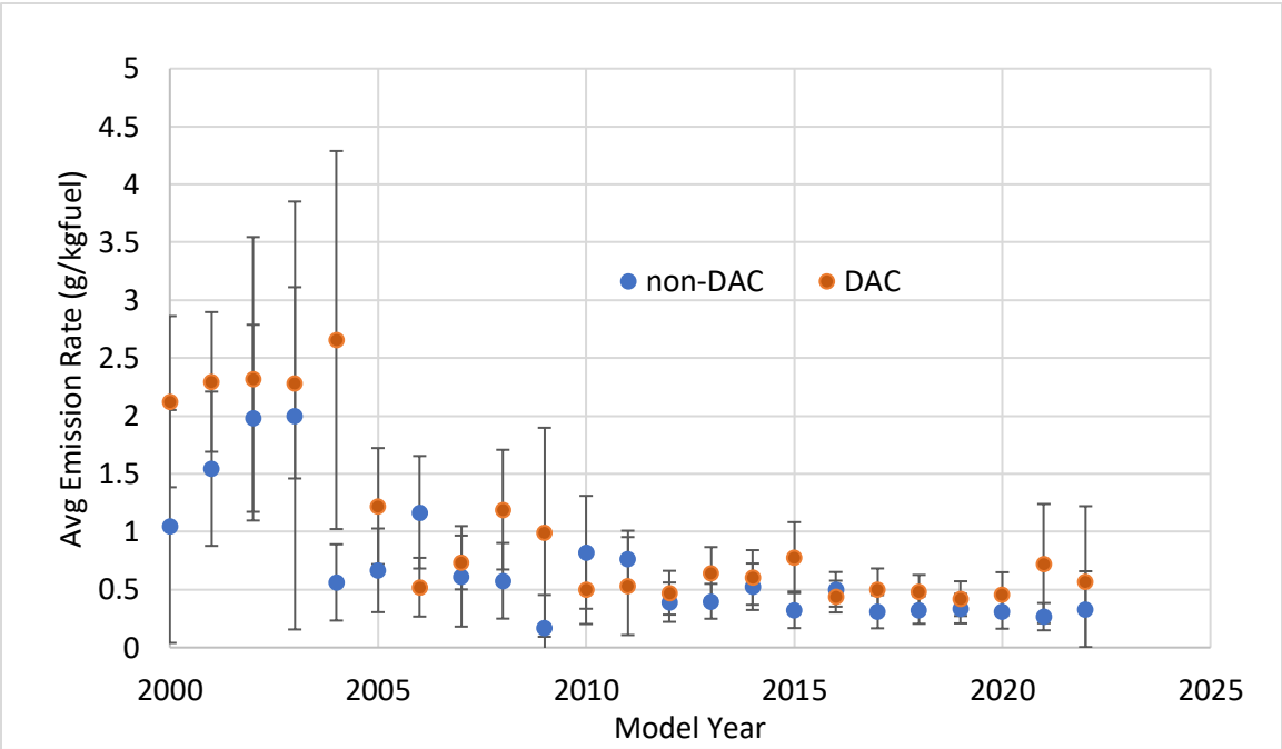
Model Year Average HC Emission Rates - Bakersfield
