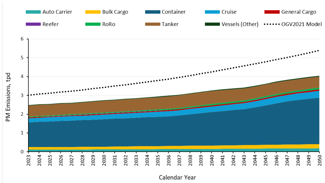
Figure 17. Statewide PM emissions from OGVs out to 100 nautical miles by vessel type.
