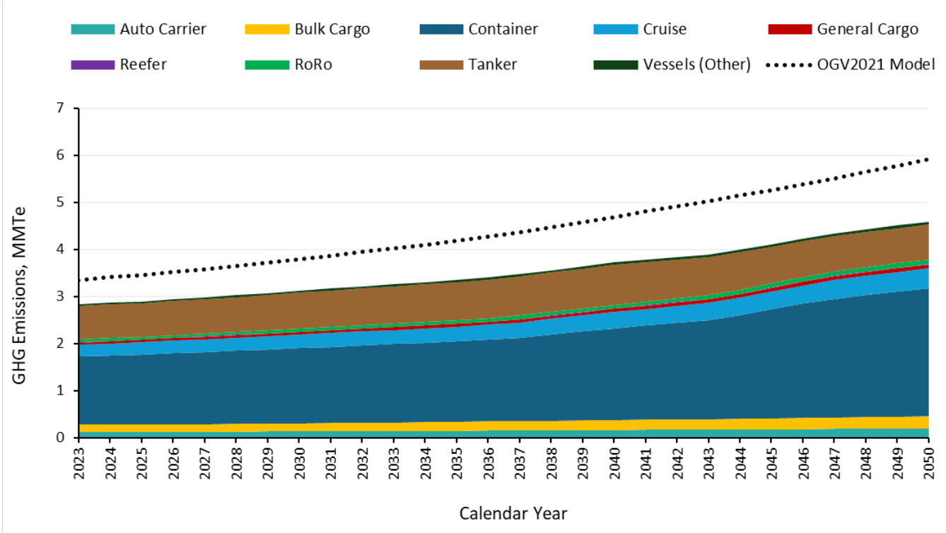
Figure 18. Statewide GHG emissions from OGVs out to 100 nautical miles by vessel type.
