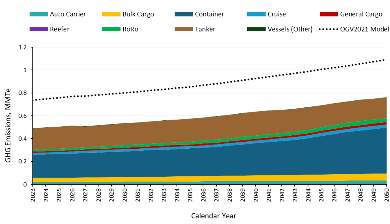
Figure 23. Bay Area GHG emissions from OGVs out to 100 nautical miles by vessel type.
