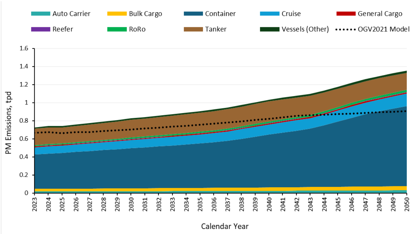
Figure 19. South Coast PM emissions from OGVs out to 100 nautical miles by vessel type.
