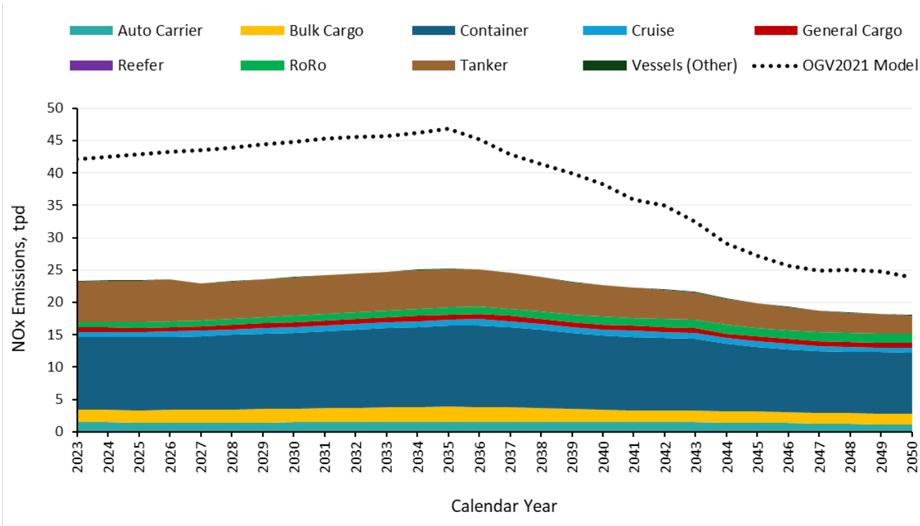
Figure 21. Bay Area NOx emissions from OGVs out to 100 nautical miles by vessel type.
