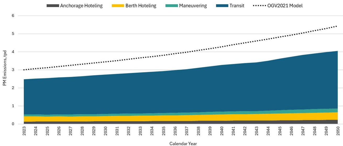
Figure 20. Statewide PM emissions from OGVs out to 100 nautical miles by mode
