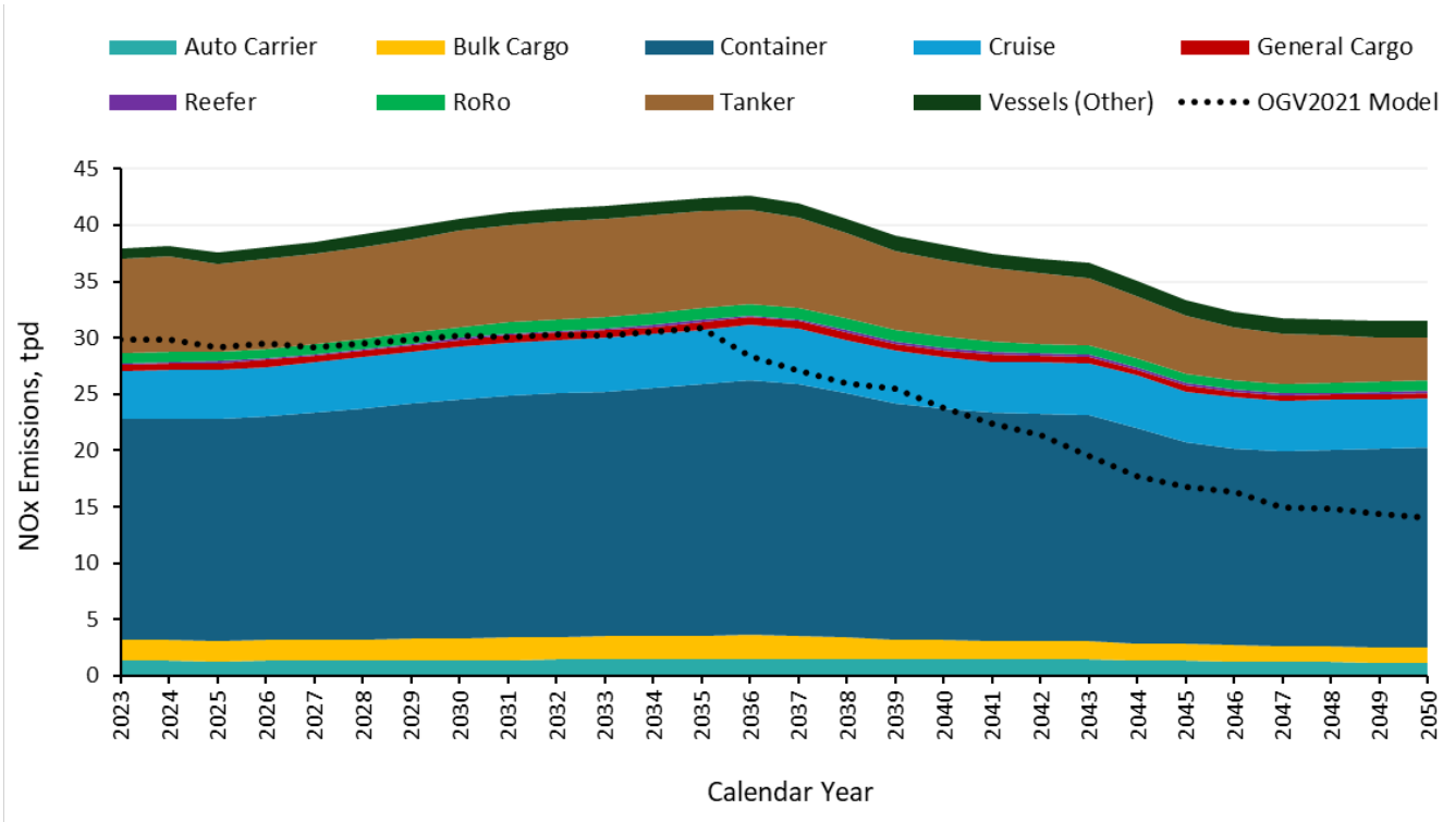
Figure 18. South Coast NOx emissions from OGVs out to 100 nautical miles by vessel type.
