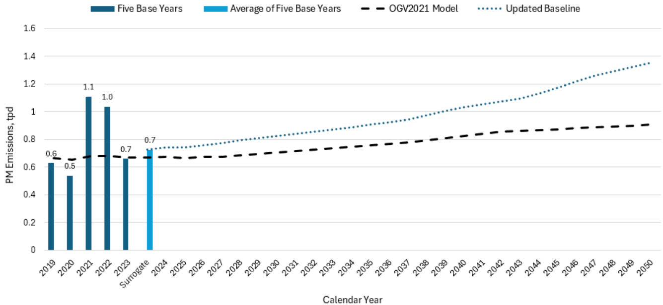
Figure 6. South Coast PM emissions from OGVs out to 100 nm using five-year averaged base year surrogate.
