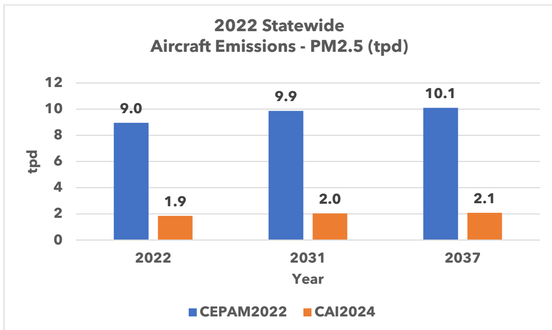
Figure 3: 2022 Annual Statewide PM2.5 Aircraft Emissions (tpd)
