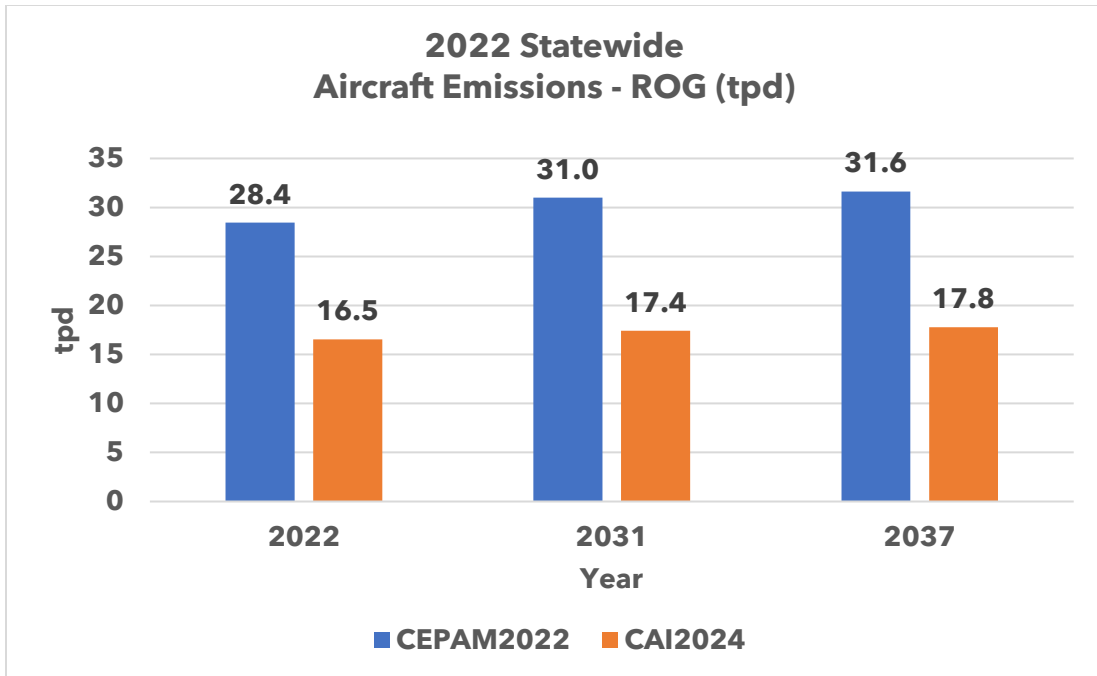
Figure 2: 2022 Annual Statewide ROG Aircraft Emissions (tpd)
