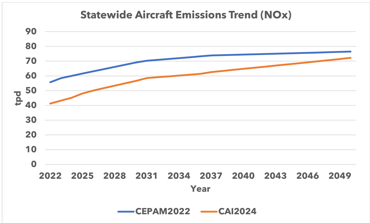
Figure 15: NOx Trend Comparison (CEPAM2022 vs CAI2024)
