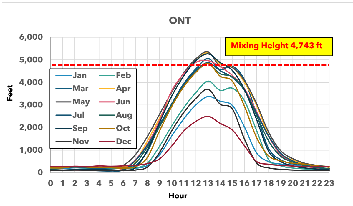
Figure 11: Mixing Height for ONT
