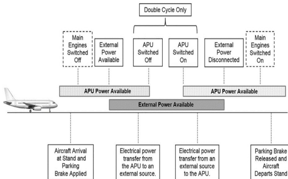
Figure 12: Typical Aircraft Turnaround Procedure (Source: Pahdra 16 )
