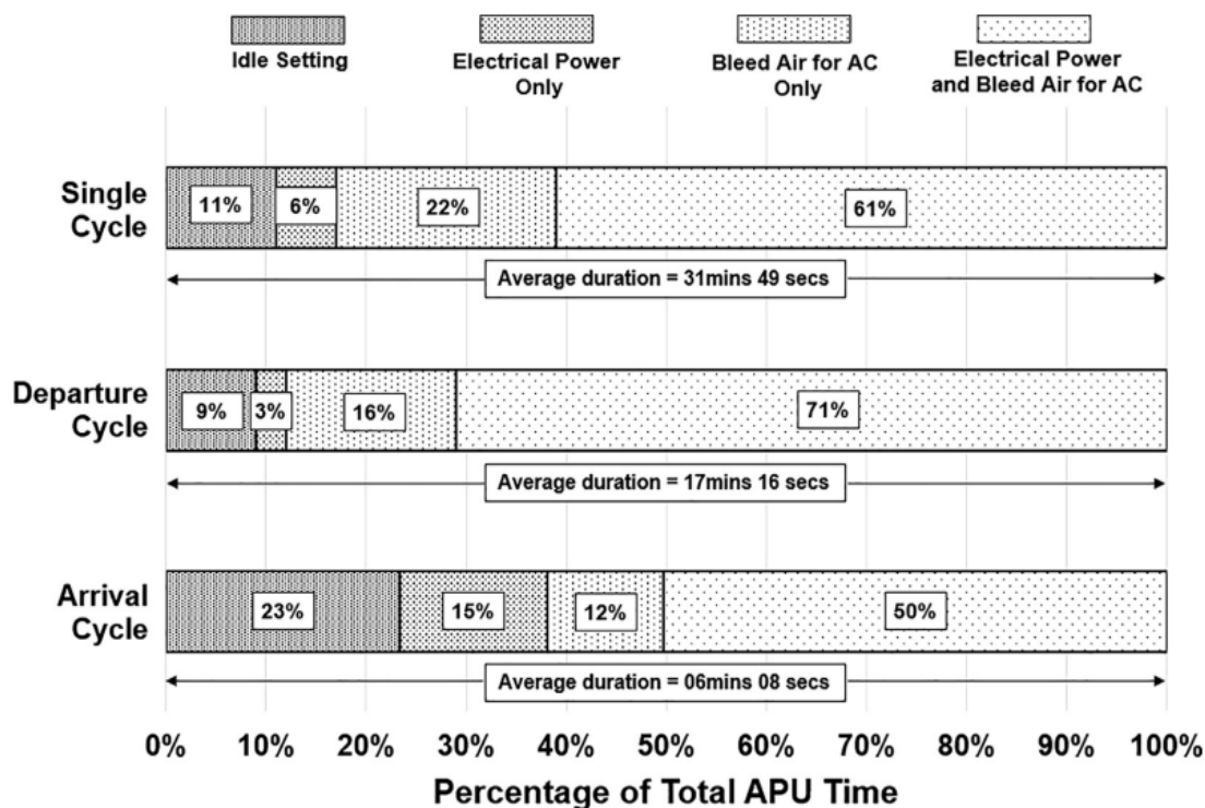
Figure 13: APU Single vs Double Cycle Event (Source: Pahdra 16 )
