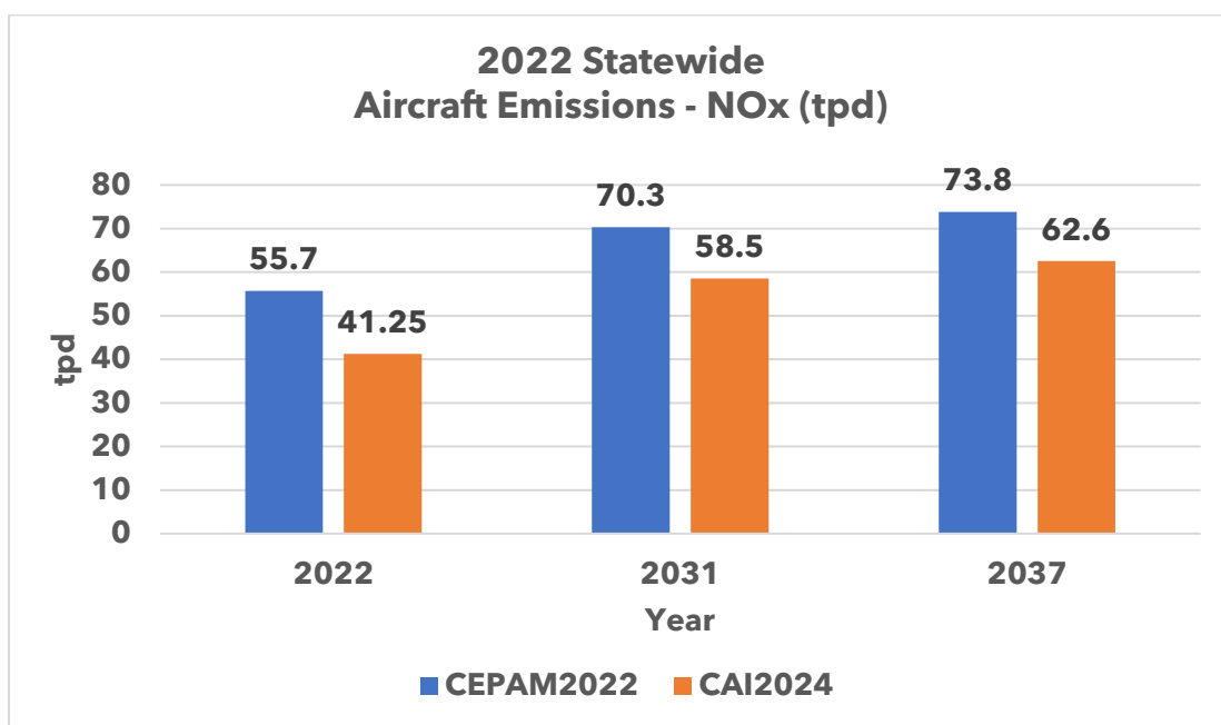
Figure 1: 2022 Annual Statewide NO x Aircraft Emissions (tpd)
