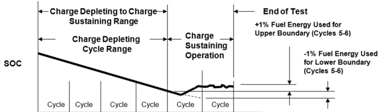
Example of Urban End of Test Conditions for a PHEV with Transitional Range
