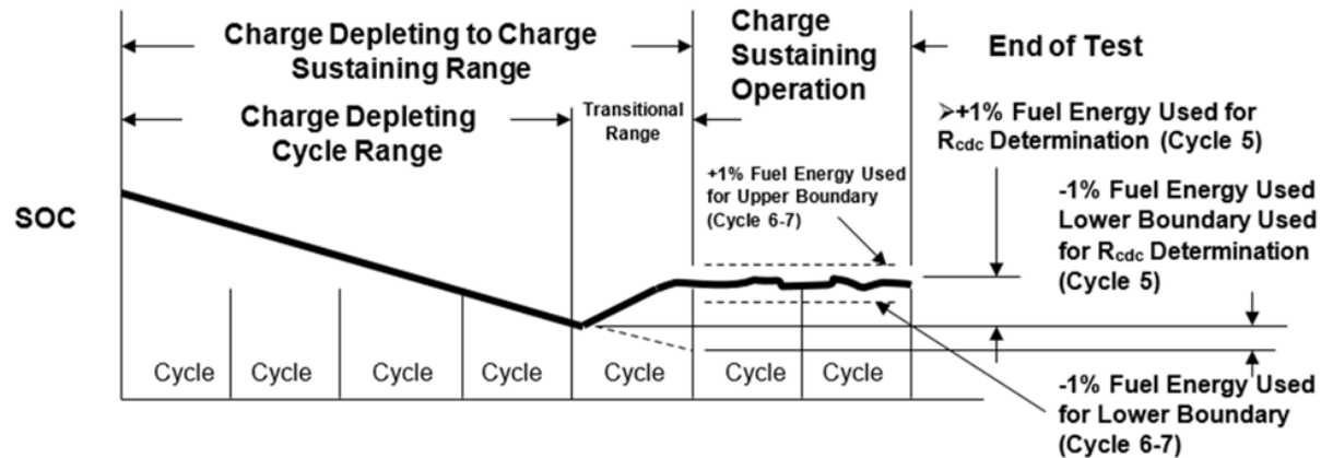
Example of Urban End of Test Conditions for a PHEV with Transitional Range
