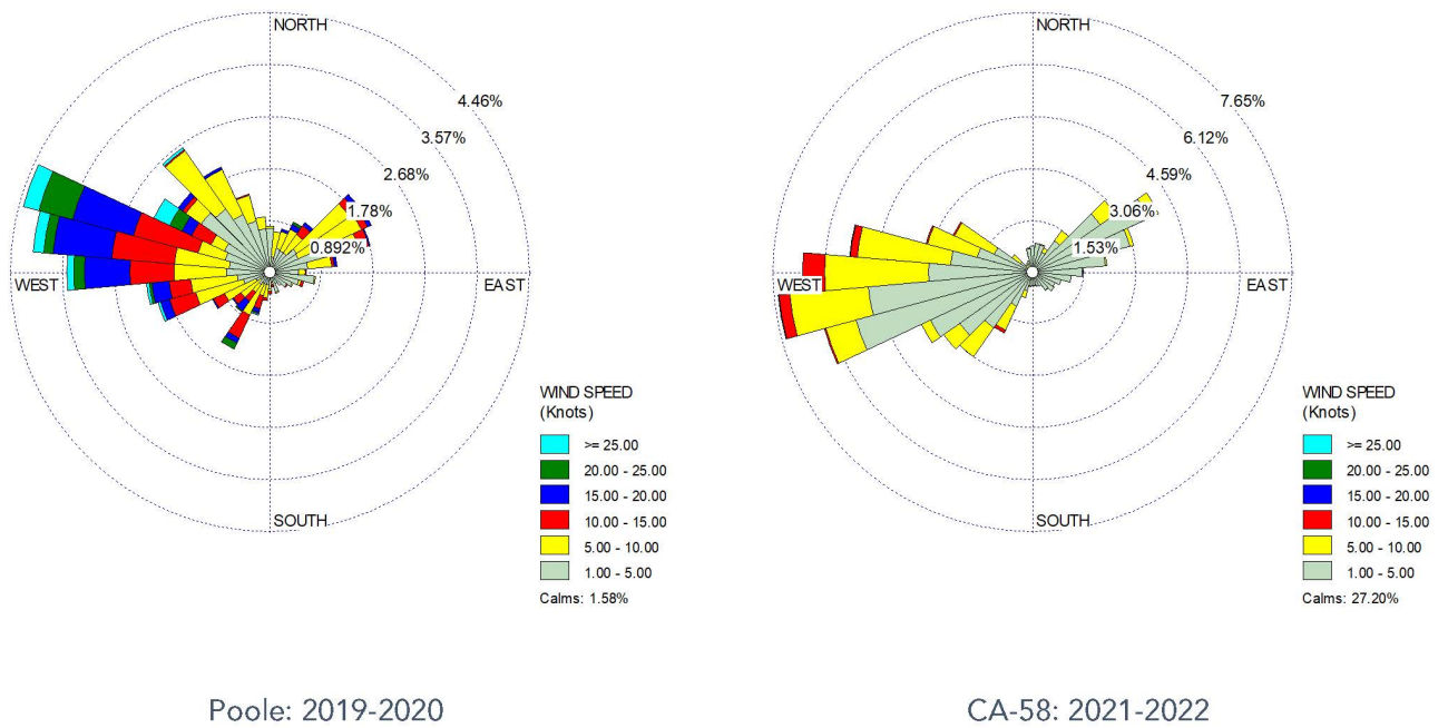
Figure 5: Mojave Seasonal Wind Rose Comparison: September through November
