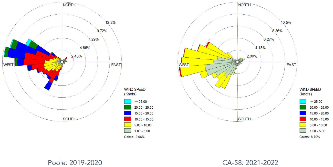
Figure 4: Mojave Seasonal Wind Rose Comparison: June through August
