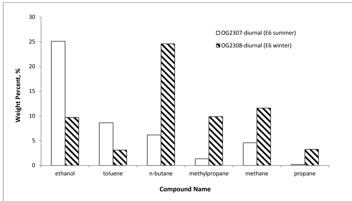
Figure 1. Comparison of selected species between OG2307 and OG2308
