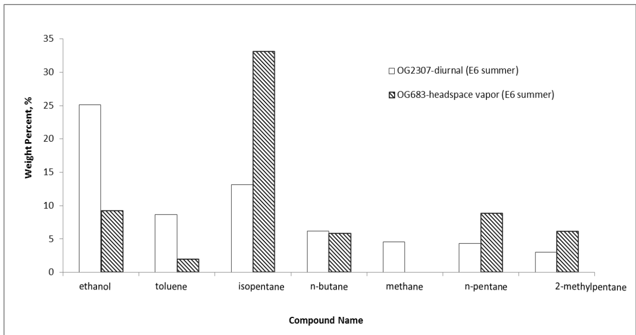
Figure 2. Comparison of selected species between OG2307 and OG683
