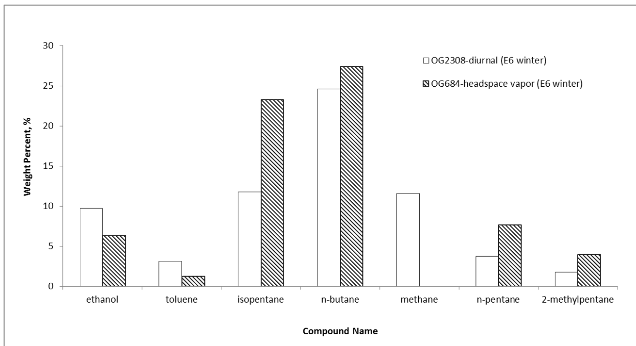
Figure 3. Comparison of selected species between OG2308 and OG684
