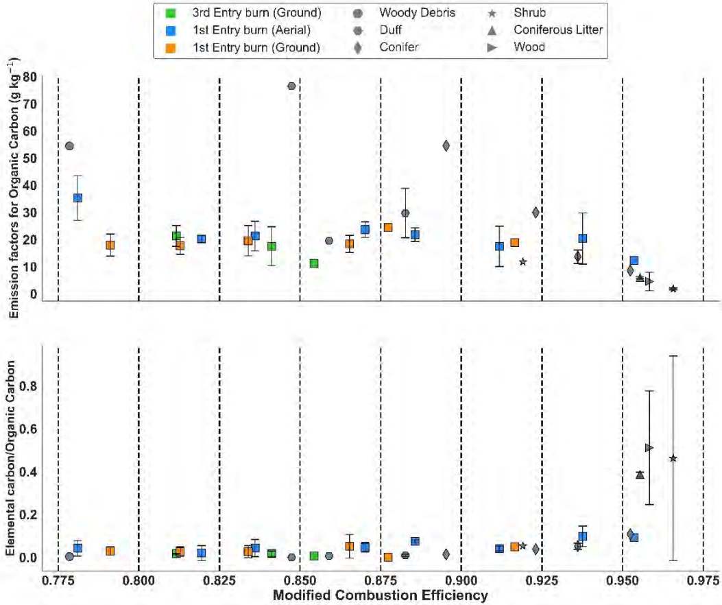
Figure 3.6 Same data as Figure 3.5 collected into 0.025 wide MCE bins to illustrate the lack of a clear MCE dependence for most of the range of measured average MCE conditions.
