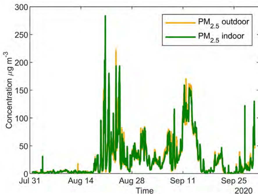
Figure S8.18 Concentration timelines of PM_{2.5} reported by an “indoor” sensor and the nearest outdoor sensor. Because the indoor concentration measured is too close to and too well correlated with the outdoor concentration, this sensor might be placed outdoors. This node was therefore not used in this analysis.
