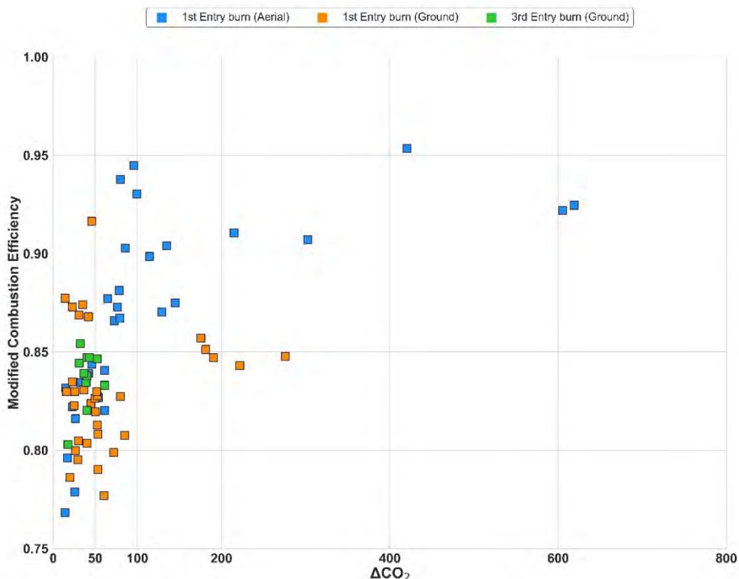
Figure 3.4 Intensity of smoke emissions during the 2017 and 2021 field campaigns as indicated by excess CO 2 (μg/m 3 ) and MCE during ground sampling on the 2017 field campaign (3 rd entry) and ground plus airborne sampling on the 2021 field campaign (1 st entry).
