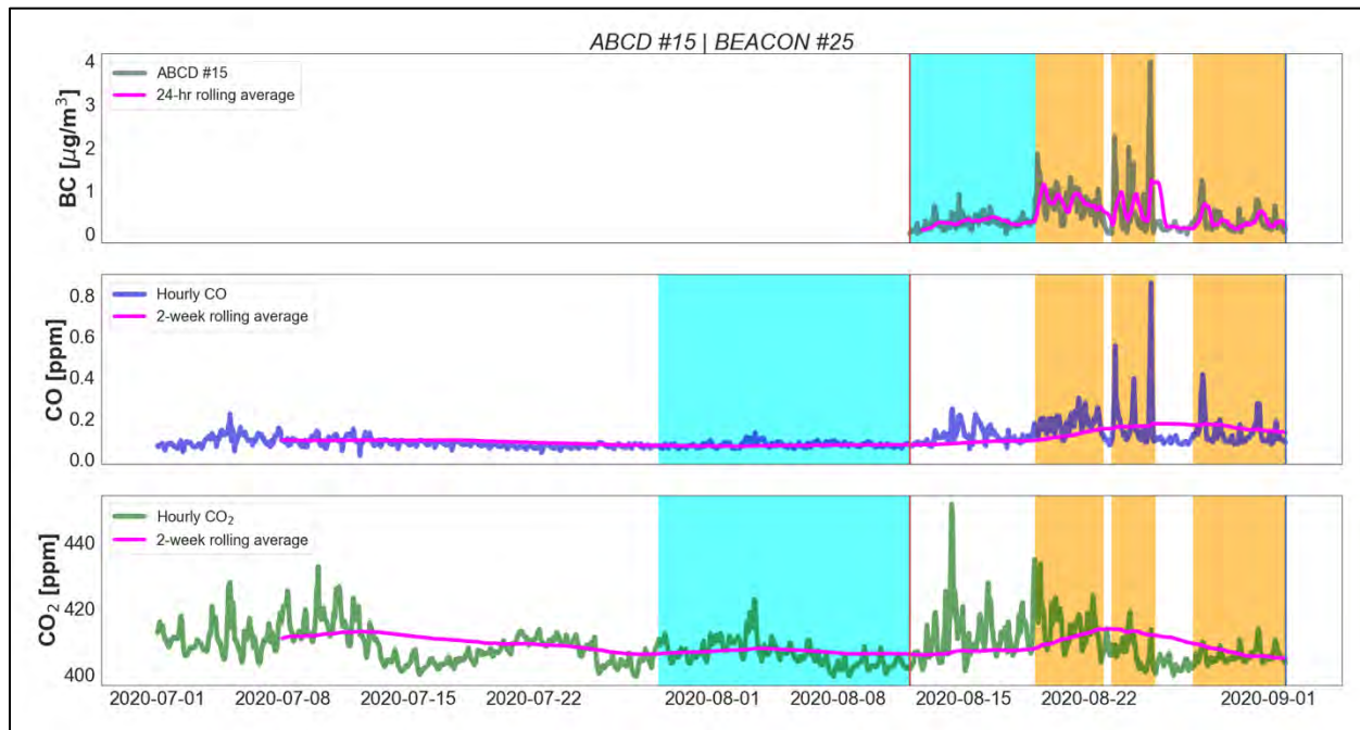
Figure 6.8 Example pairing of ABCD to the nearest BEACO2N node with the hourly concentration of BC, CO and CO 2 plotted from top to bottom, overlaid with the 24-hour rolling average for BC and the 2-week rolling average for CO and CO 2 . Background concentration periods for each pollutant highlighted in blue; wildfire smoke hours highlighted in yellow (see Table 6.1 ).
