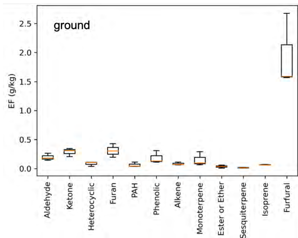
Figure 4.4 Averaged emission factors (EFs) for individual and summed compound classes as measured in ground-based samples.
