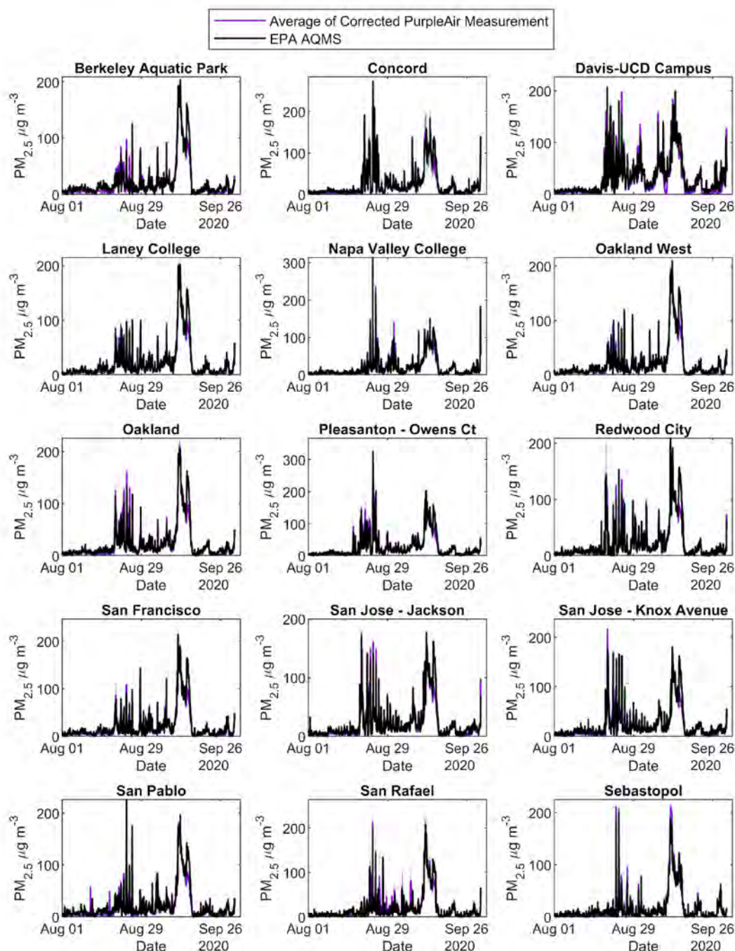
Figure S8.6 Hourly time profile of \text{PM}_{2.5} concentration of the EPA monitors (black) and mean (purple) \pm standard deviation (gray) of \text{PM}_{2.5} (corrected) measured by nearby PurpleAir sensors in the San Francisco Bay Area in August and September 2020. The plots only include EPA monitoring stations having at least three outdoor PurpleAir sensors within 5 km of them. The EPA measurement and nearby PurpleAir sensors measurement agree reasonably well with each other.
