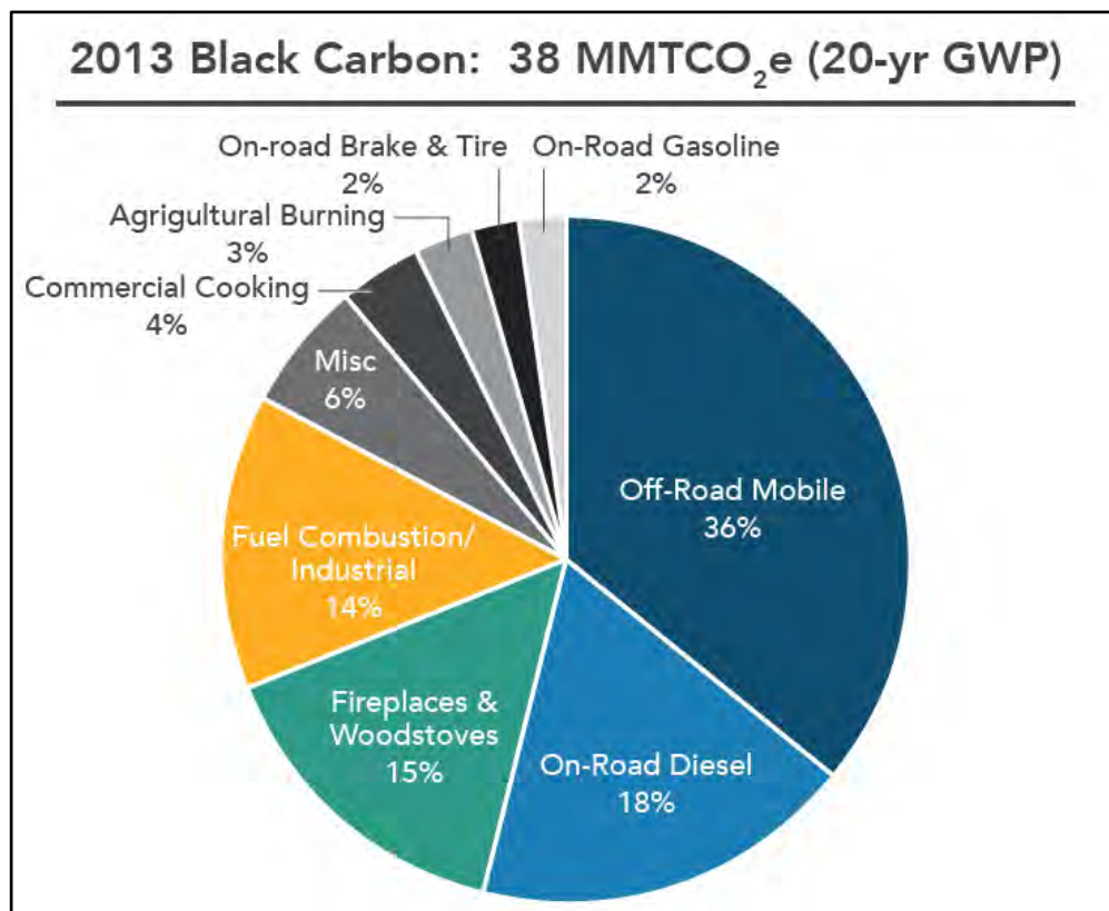
Figure 6.1 Pie chart of CARB 2013 Black Carbon emissions inventory excluding forestry sources. Source: https://ww2.arb.ca.gov/ghg-slcip-inventory
