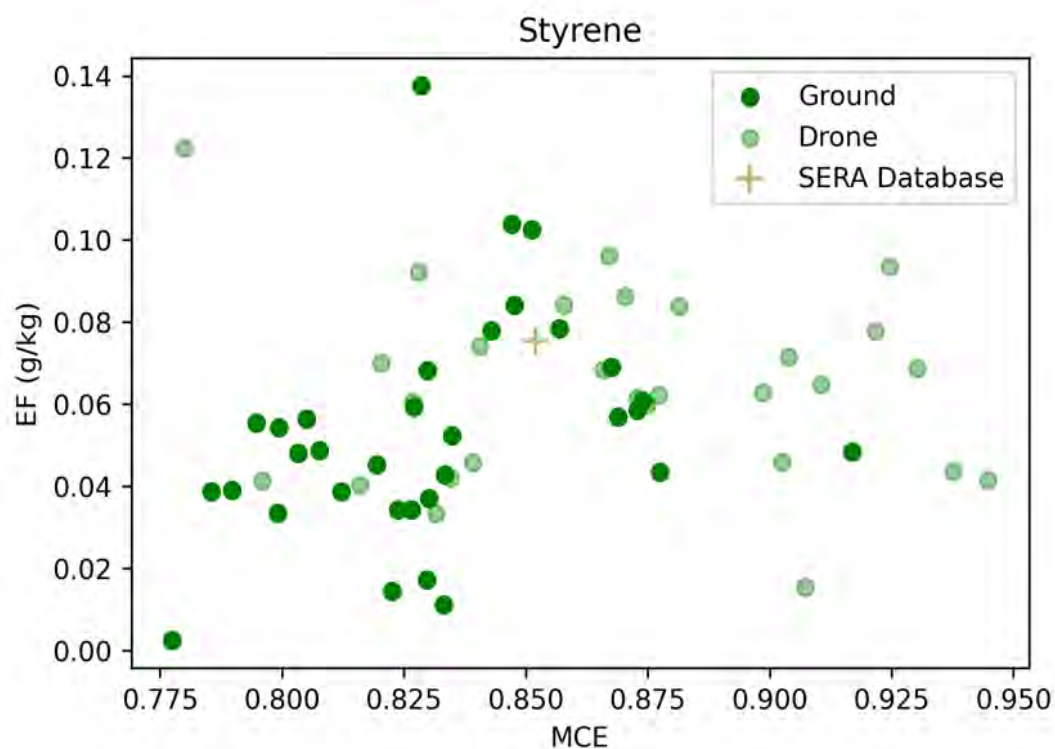
Figure 4.14 Emission factors (EFs) for styrene as measured in ground- and drone-based samples and reported for western coniferous forest in the SERA database.
