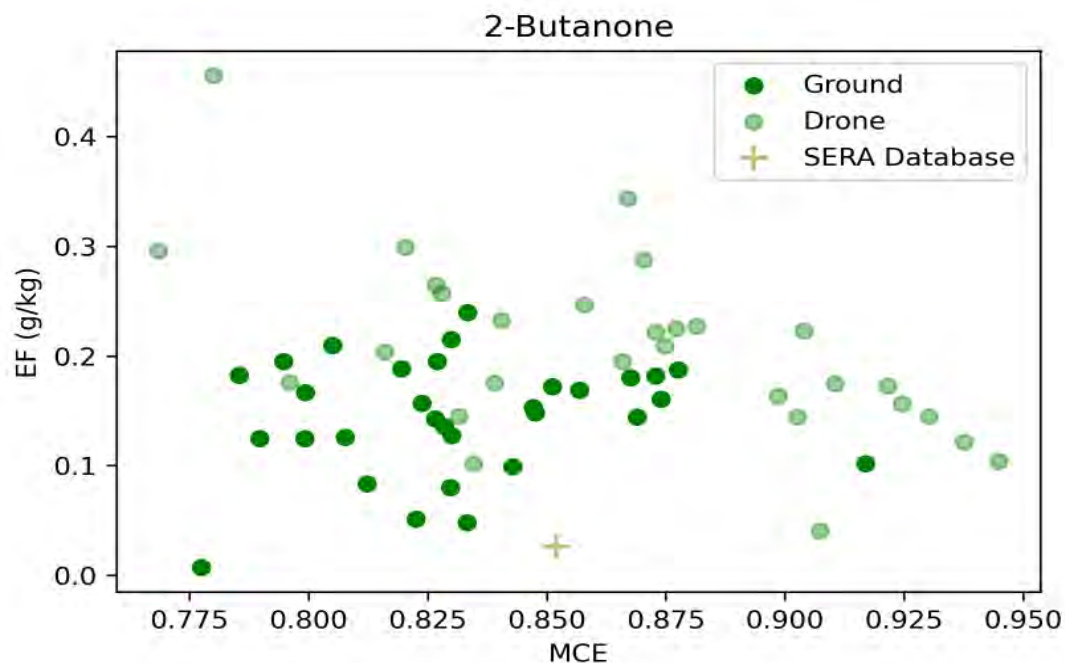
Figure 4.13 Emission factors (EFs) for 2-butanone as measured in ground- and drone-based samples and reported for western coniferous forest in the SERA database.
