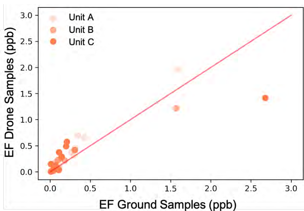
Figure 4.5 Averaged emission factors (EFs) for summed compound classes as measured in drone-based samples.
