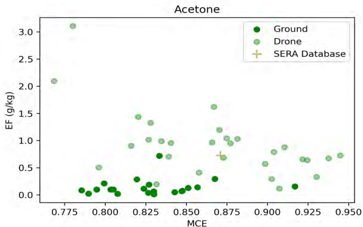
Figure 4.12 Emission factors (EFs) for acetone as measured in ground- and drone-based samples and reported for western coniferous forest in the SERA database.
