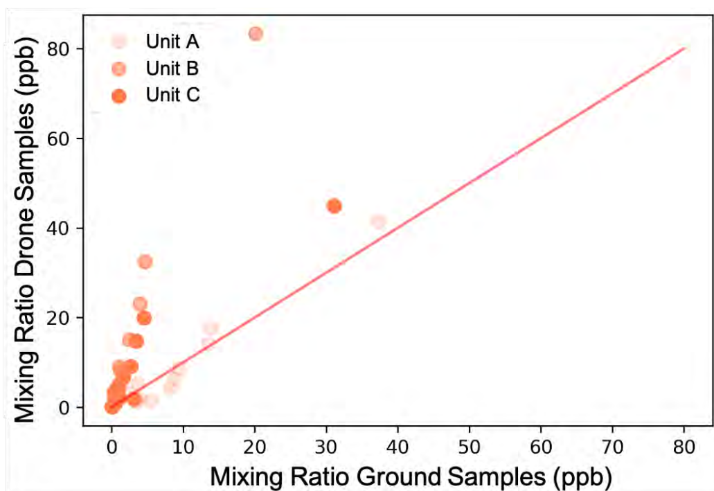
Figure 4.3 Comparison of averaged mixing ratios for summed compound classes as measured in drone-based vs. ground-based samples.
