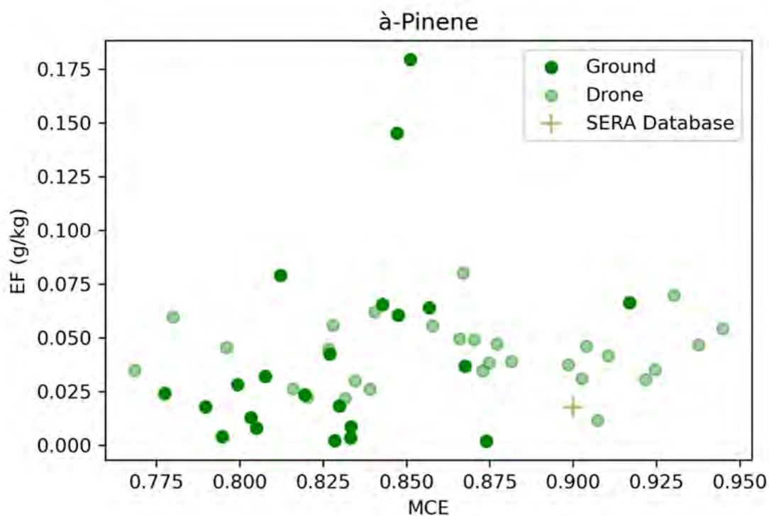
Figure 4.16 Emission factors (EFs) for alpha-pinene as measured in ground- and drone-based samples and reported for western coniferous forest in the SERA database.
