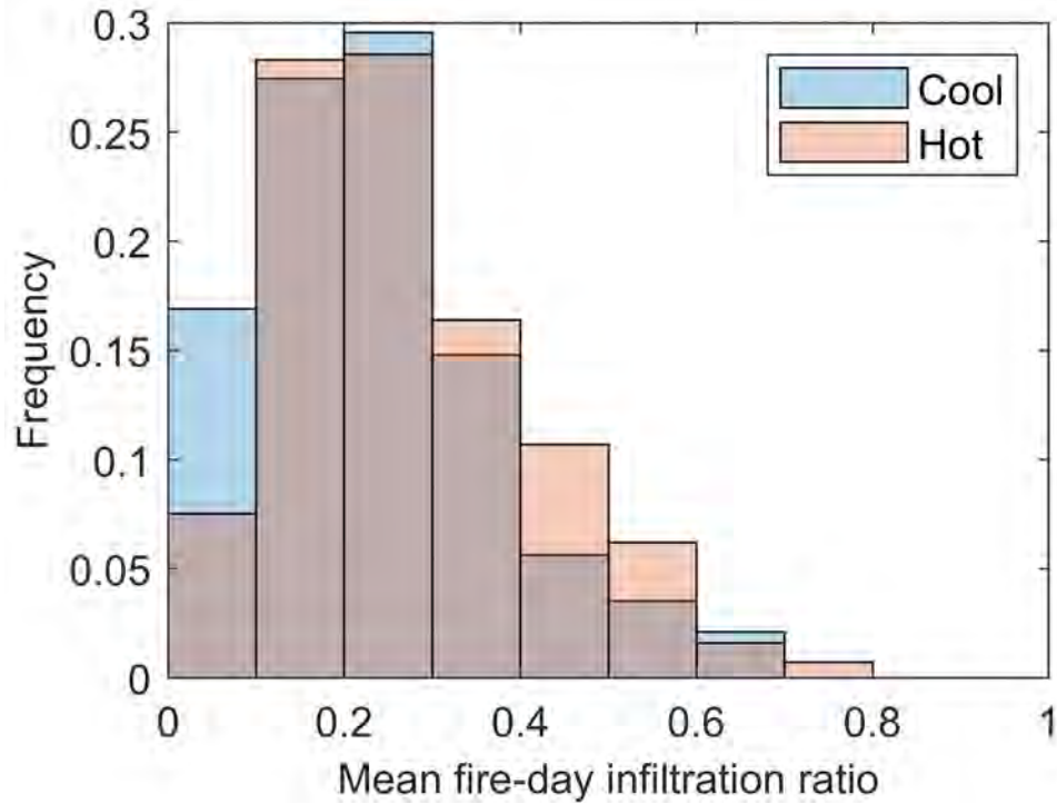
Figure S8.11 Infiltration ratio on fire days for cool buildings (95 th percentile indoor temperature < 30°C, N = 142 ) and hot buildings (95 th percentile indoor temperature \geq 30^\circ\text{C} , N = 1132 ) in the San Francisco Bay Area in August and September 2020. The cool buildings have significantly lower fire-day infiltration ratios than the hot ones ( p < 0.01 ), and 17% of cool buildings had extremely low infiltration ratios ( < 0.1 ).
