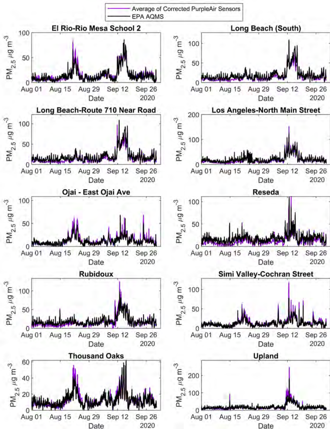
Figure S8.8 Hourly time profile of PM_{2.5} concentration of the EPA monitors and mean (purple) \pm standard deviation (gray) of PM_{2.5} (corrected) measured by nearby PurpleAir sensors in the Greater Los Angeles Area in August and September 2020. The plots only include EPA monitoring stations having at least three outdoor PurpleAir sensors within 5 km of them.
