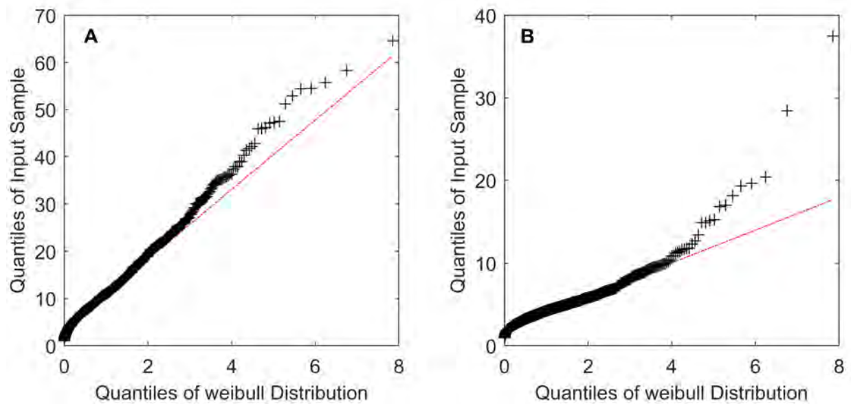
Figure S8.4 Quantile-quantile plots of mean indoor \text{PM}_{2.5} , on the fire days (A) and non-fire days (B) against Weibull distribution. The reference line represents the theoretical Weibull distribution.
