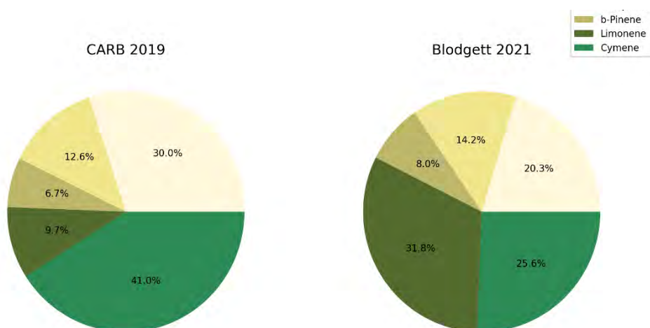
Figure 4.10 Normalized peak areas of representative compounds in 2019 wildfire samples (left) and 2021 prescribed burn samples (right).
