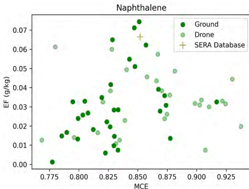
Figure 4.15 Emission factors (EFs) for naphthalene as measured in ground- and drone-based samples and reported for western coniferous forest in the SERA database.
