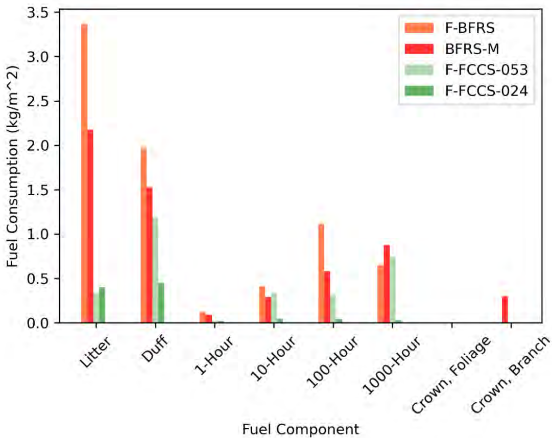
Figure 7.3 Fuel consumption ( \text{kg/m}^2 ) measured at Blodgett Forest Research Station (BFRS-M) and predicted using measured fuel loadings (F-BFRS), FCCS fuelbed ID 053 (default) and FCCS fuelbed ID 024 (LANDFIRE).
