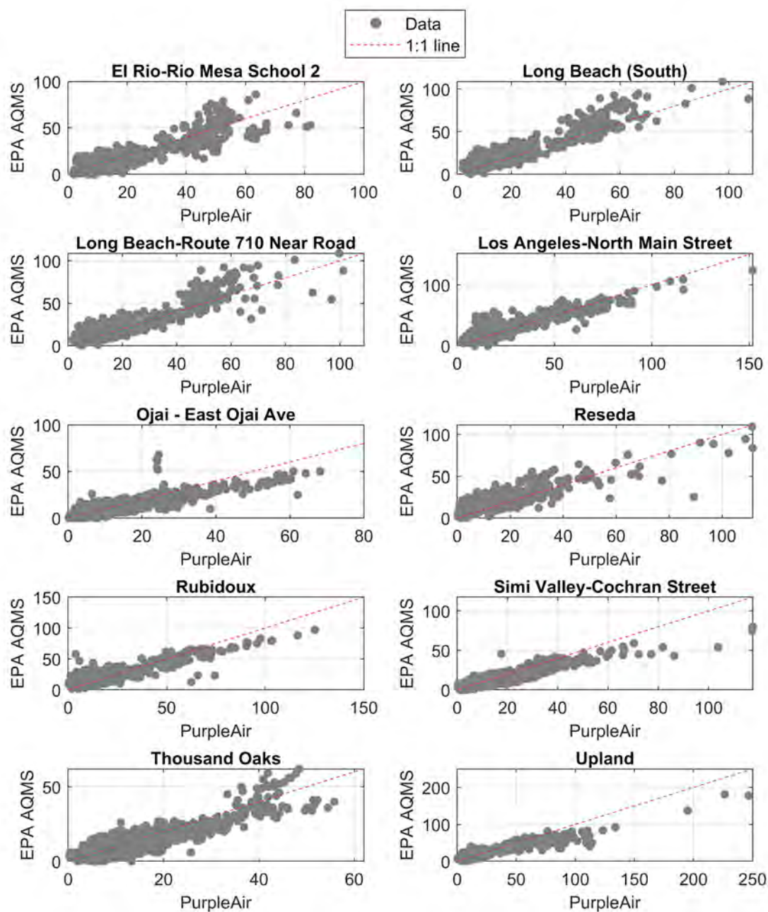
Figure S8.9 Scatter plot of PM 2.5 ( \mu\text{g m}^{-3} ) of the EPA monitors and PM 2.5 (corrected) measured by nearby PurpleAir sensors in the Greater Los Angeles Area in August and September 2020
