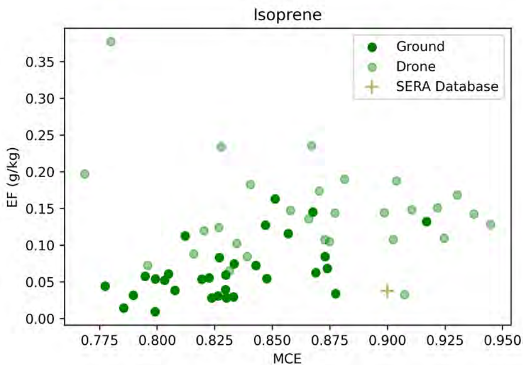
Figure 4.18 Emission factors (EFs) for isoprene as measured in ground- and drone-based samples and reported for western coniferous forest in the SERA database.
