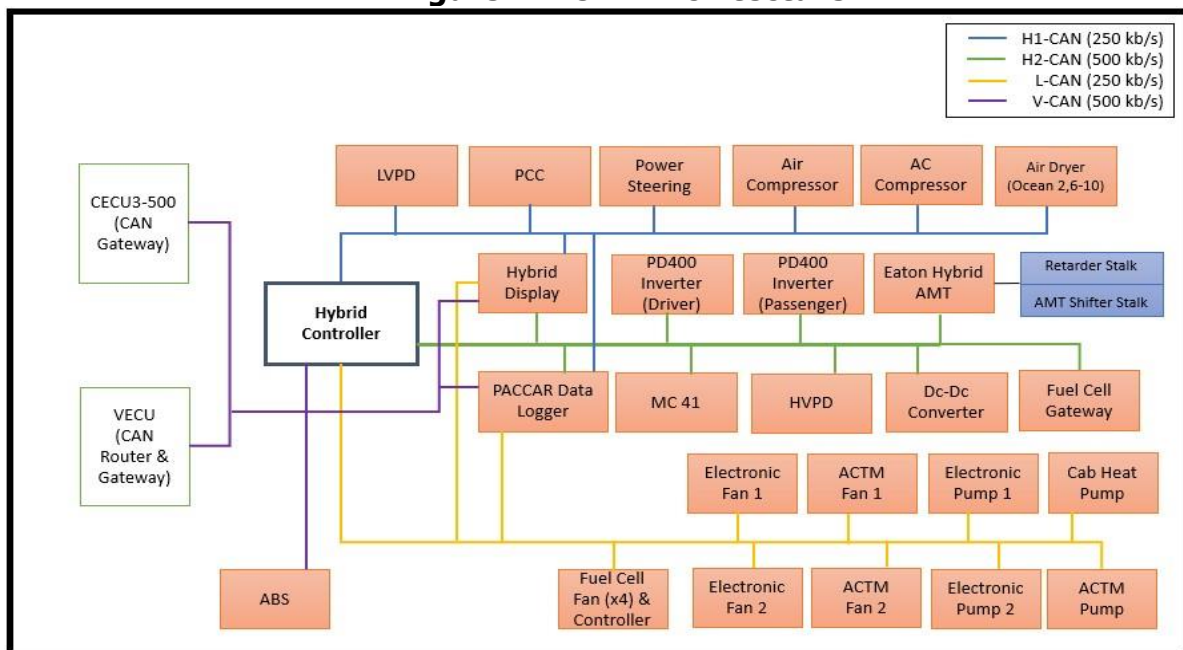
Figure 14. CAN Architecture
