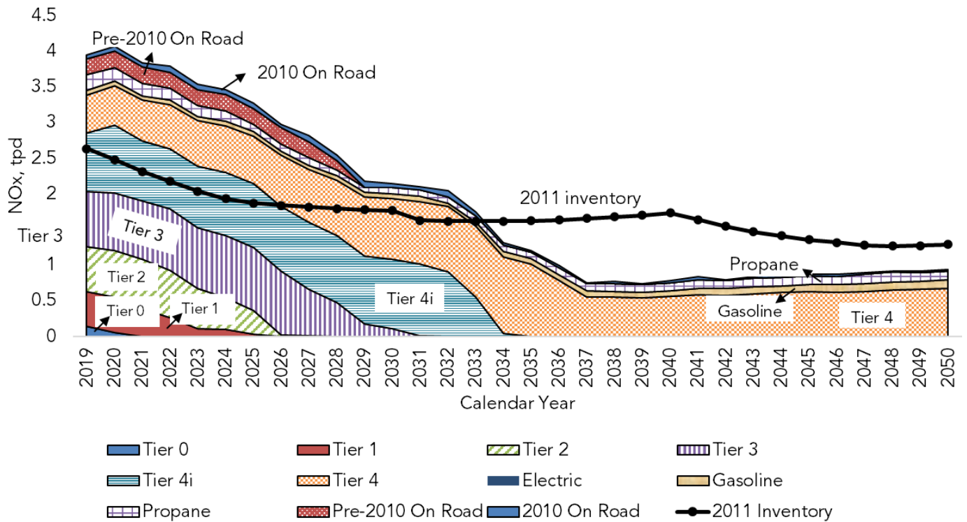
Figure 13: Statewide CHE NOx Emission Projection by Diesel Tier Group and Fuel Type
