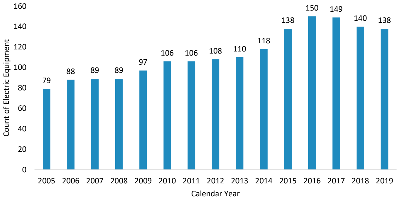
Figure 20: Count of Electric CHE at the Port of Los Angeles
