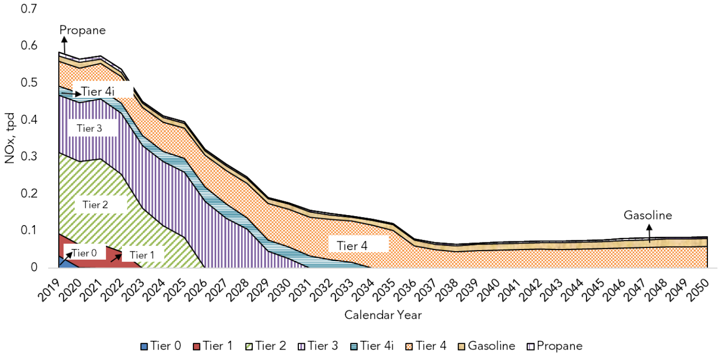
Figure 17: Port of Oakland CHE NOx Emission Projection by Diesel Tier Group and Fuel Type
