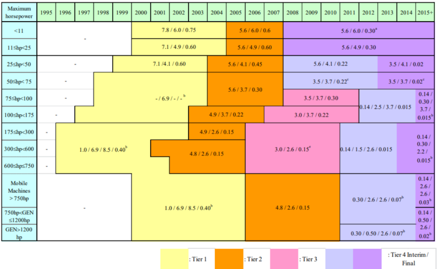
Figure 5: Diesel Engine Standards
