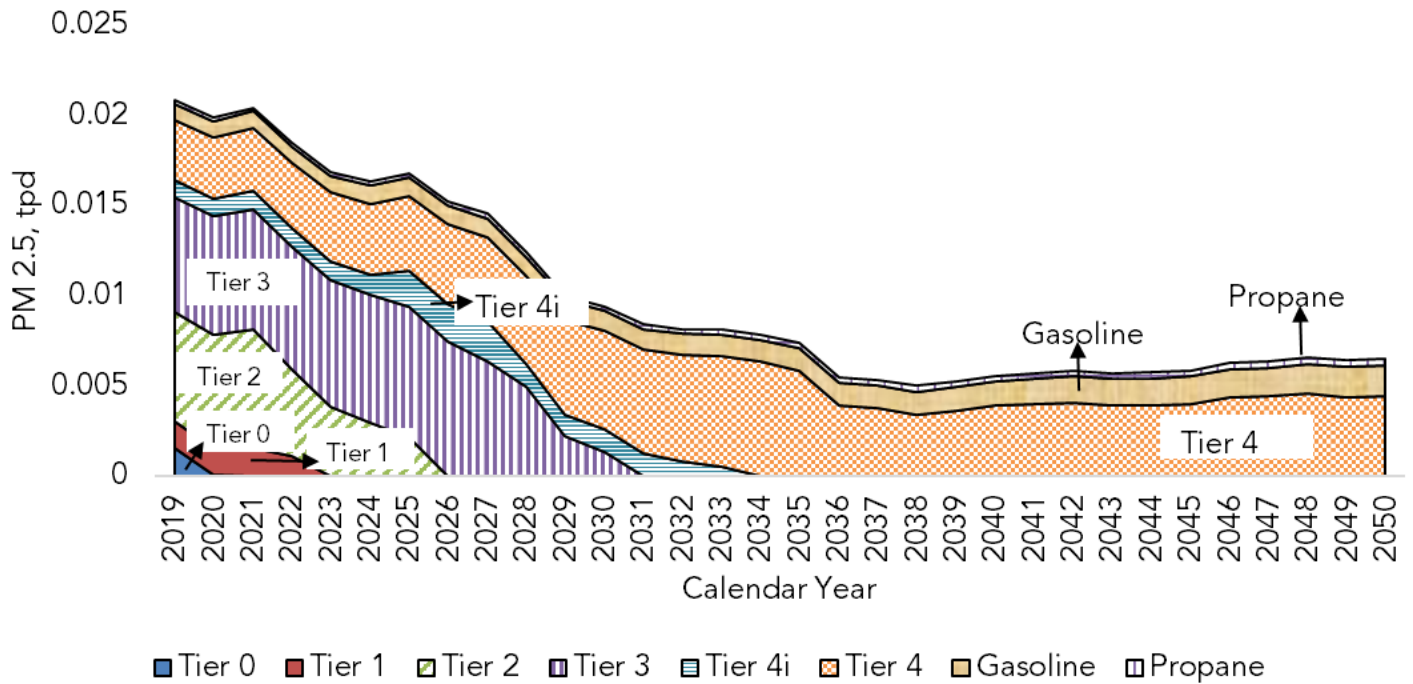
Figure 18: Port of Oakland CHE PM2.5 Emission Projection by Diesel Tier Group and Fuel Type
