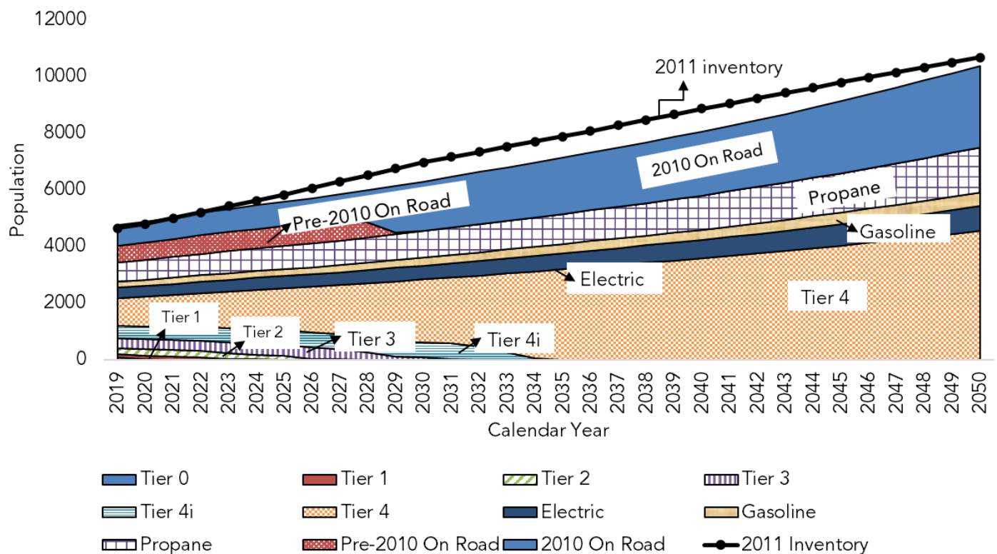
Figure 12: Statewide CHE Population Projection by Diesel Tier Group and Fuel Type
