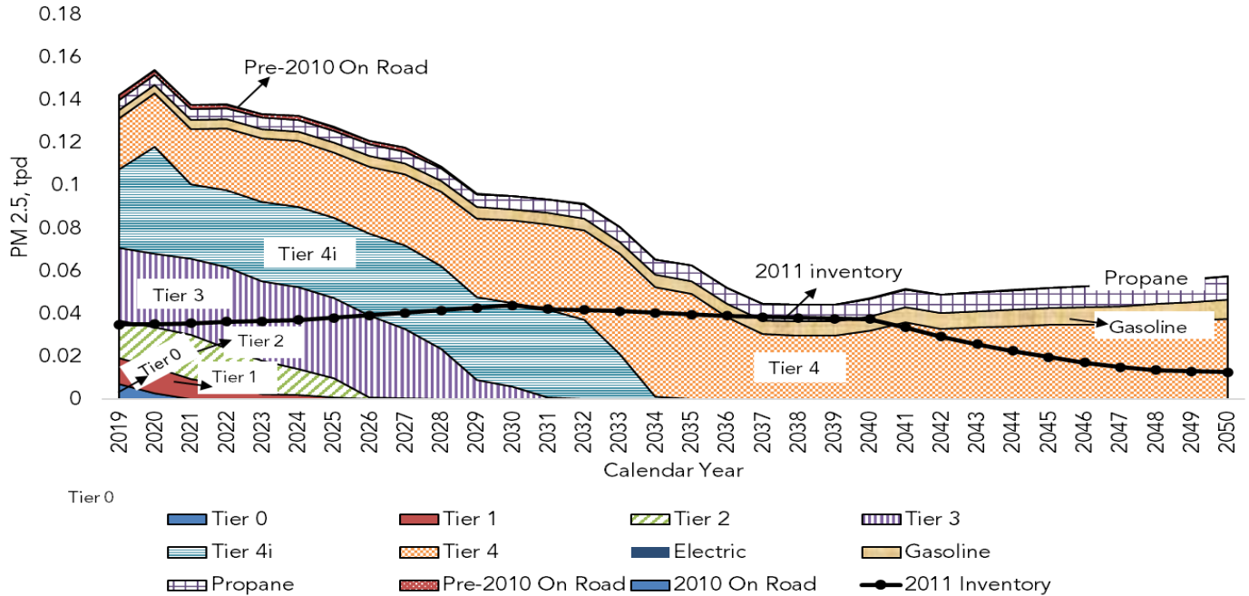
Figure 14: Statewide CHE PM 2.5 Emission Projection by Diesel Tier Group and Fuel Type
