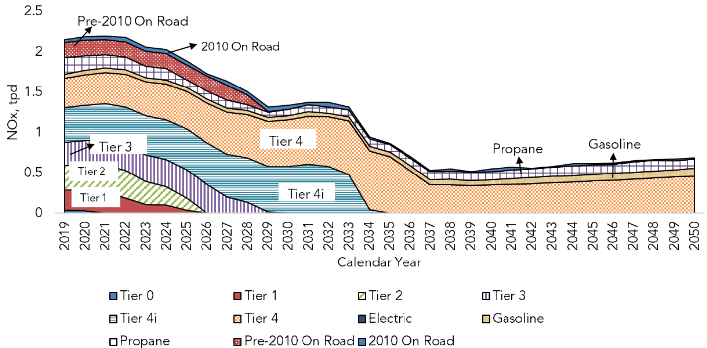
Figure 15: Port of LA/LB CHE NO x Emission Projection by Diesel Tier Group and Fuel Type
