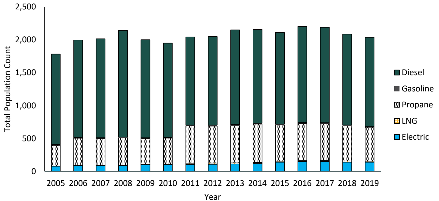
Figure 19: Comparison of CHE fuel types from the Port of Los Angeles
