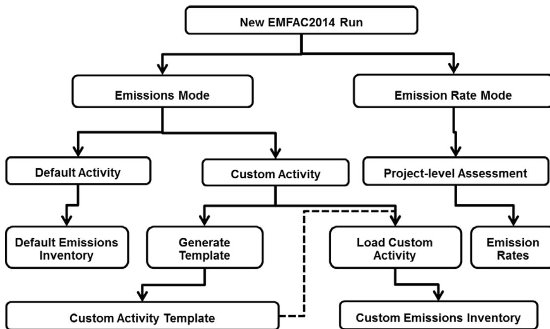
Figure 1-1. EMFAC2014 Overall Flow
