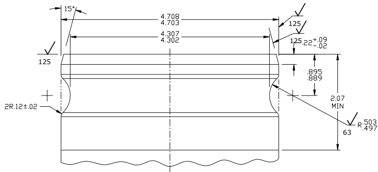
Figure 3B Phase I Vapor Adaptor Cam and Groove Specification
