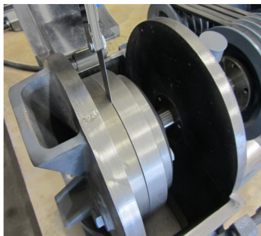
Figure F-5. Reset the plate distance.
