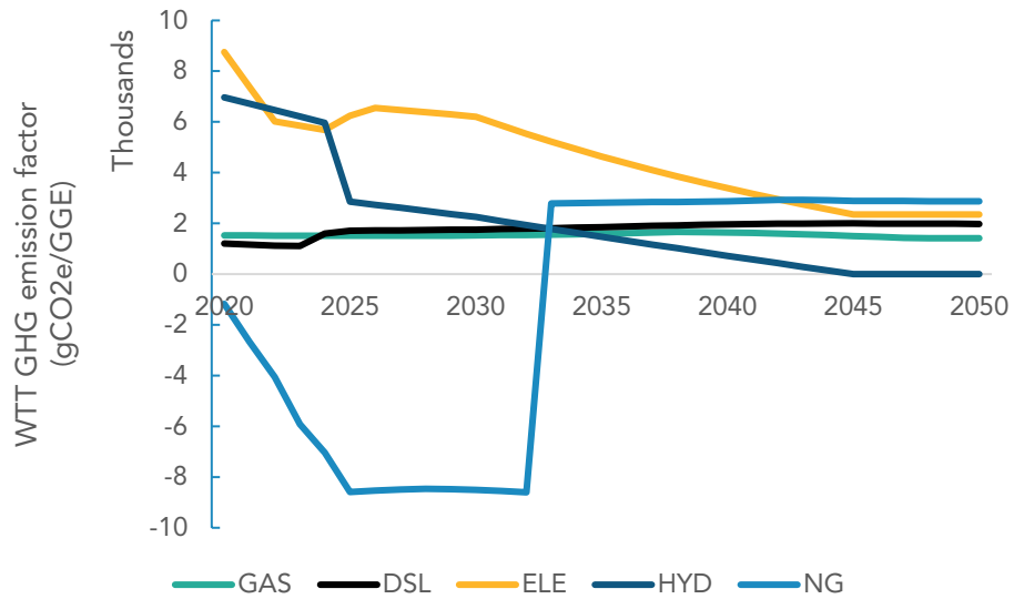
Figure 56 - WTT GHG EFs by Fuel Type 253
