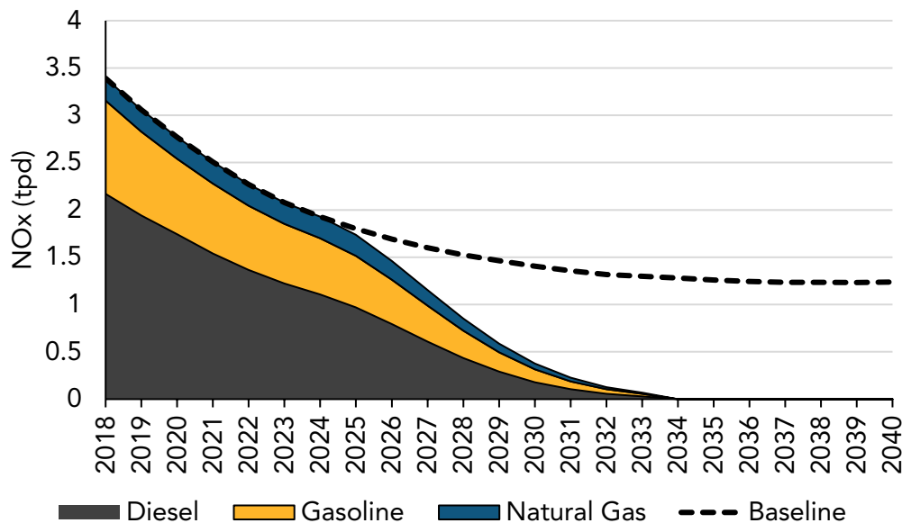
Figure 41 - Statewide NOx Emissions from GSE: MSS Scenario
