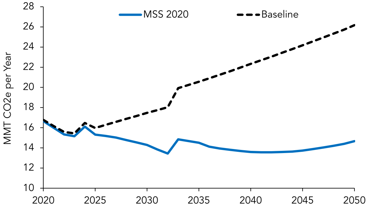
Figure 54 - Statewide Well-to-Wheel GHG Emissions from Off-road Sector
