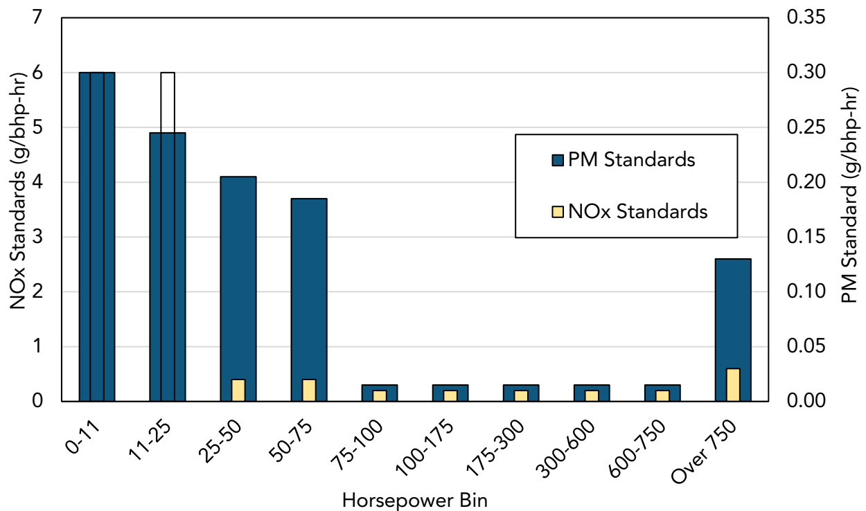
Figure 50 - Tier 4 Final Off-Road Diesel Standards for NOx and PM 218
