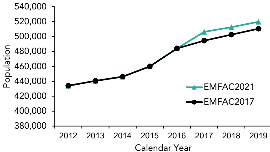
Figure 4.2.1-6. Comparison between EMFAC2021 and EMFAC2017 LHDT diesel population
