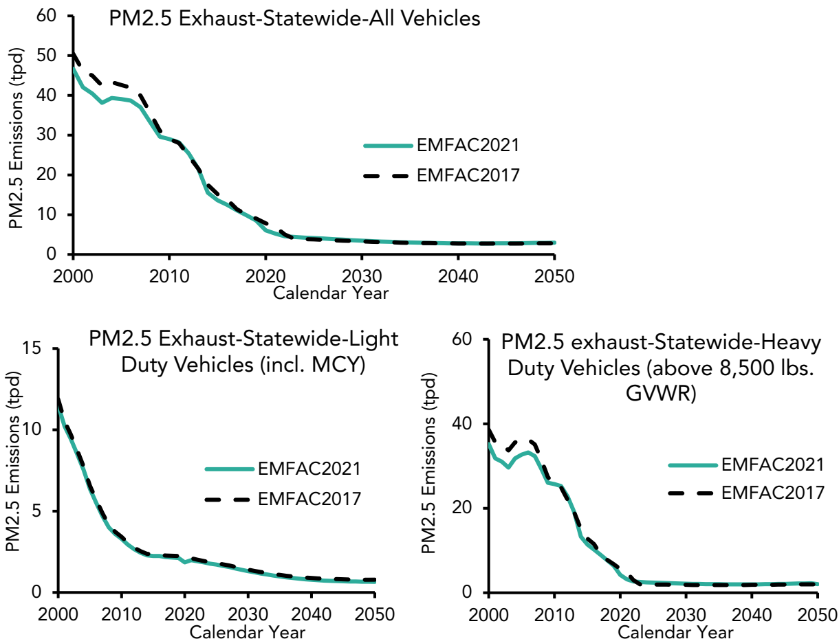
Figure 5.3-3. Comparison of tailpipe PM2.5 emissions between EMFAC2021 and EMFAC2017
