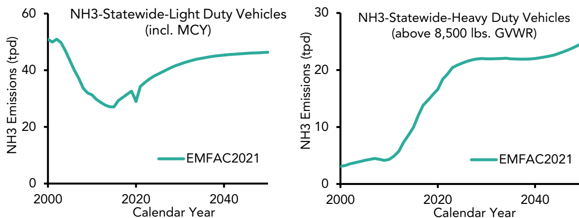
Figure 5.3-6. NH 3 emissions in EMFAC2021
