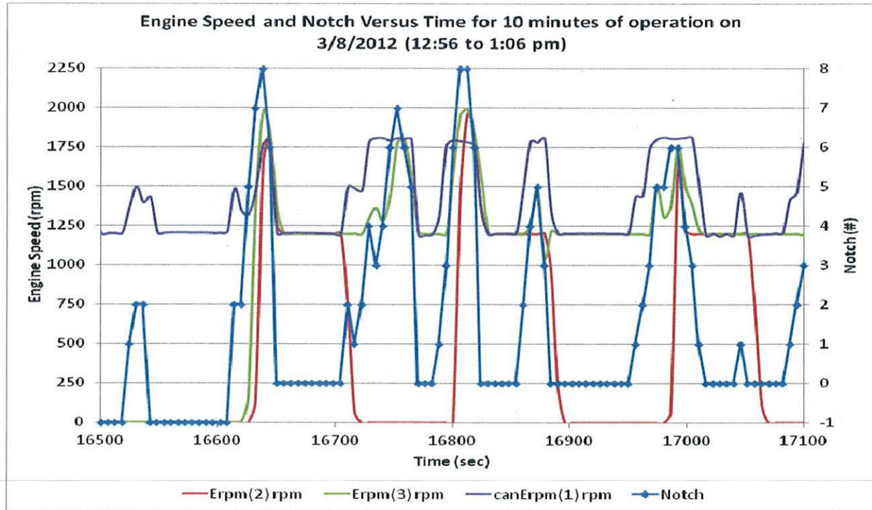
Figure 2.1: Operating Characteristics of the locomotive under original RCL Logic
