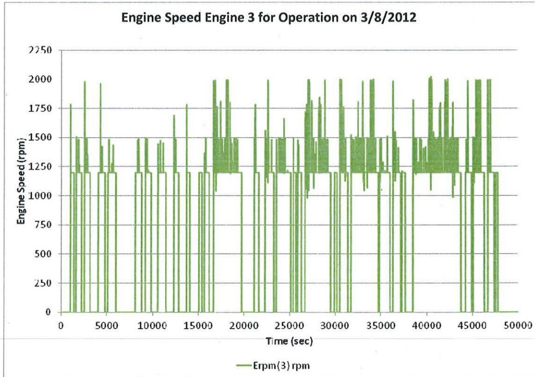
Figure 2.3: Operating conditions of the second non-lead engine under original RCL logic
