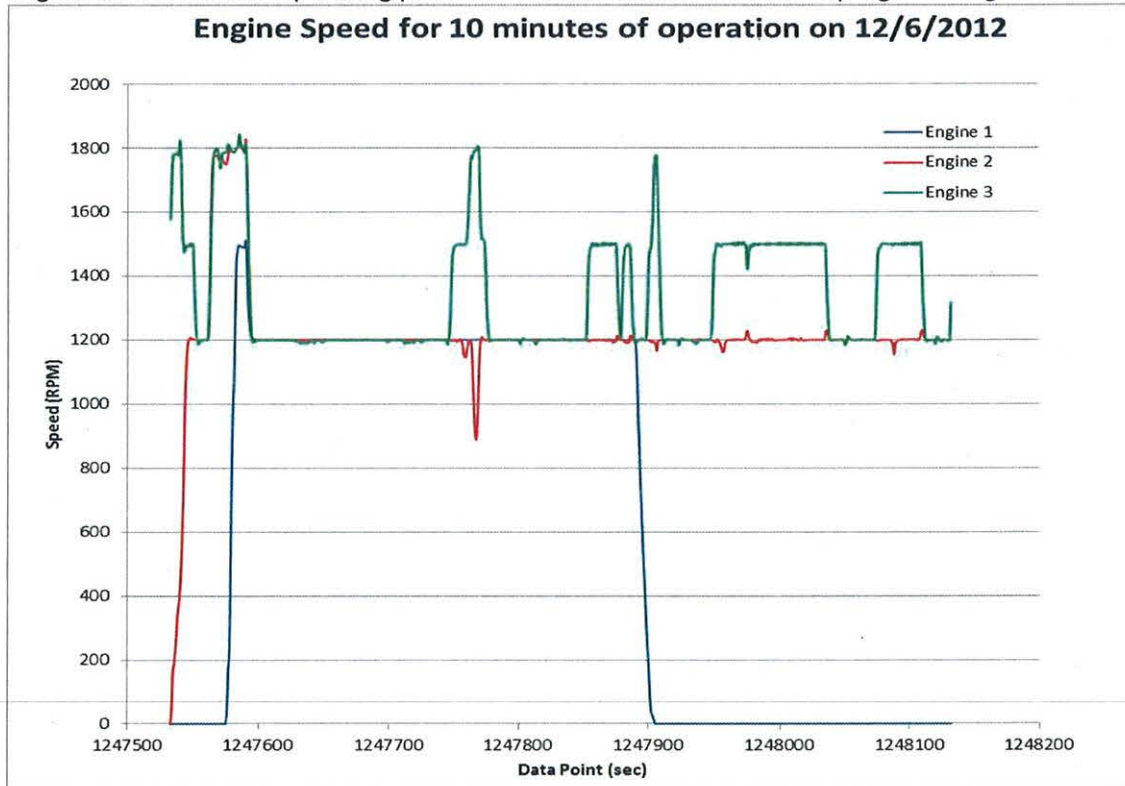
Figure 2.5: 10 minute operating period of the locomotive after the reprogramming of the RCL
