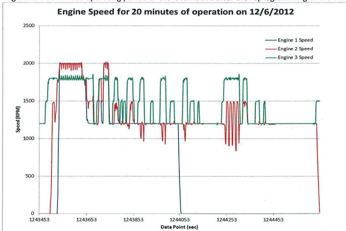
Figure 2.4: 20 minute operating period of the locomotive after the reprogramming of the RCL
