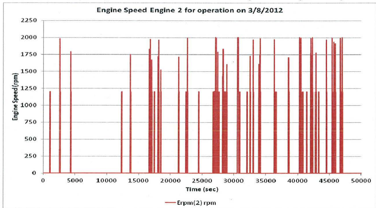
Figure 2.2: Operating characteristics of the first non-lead engine under original RCL logic
