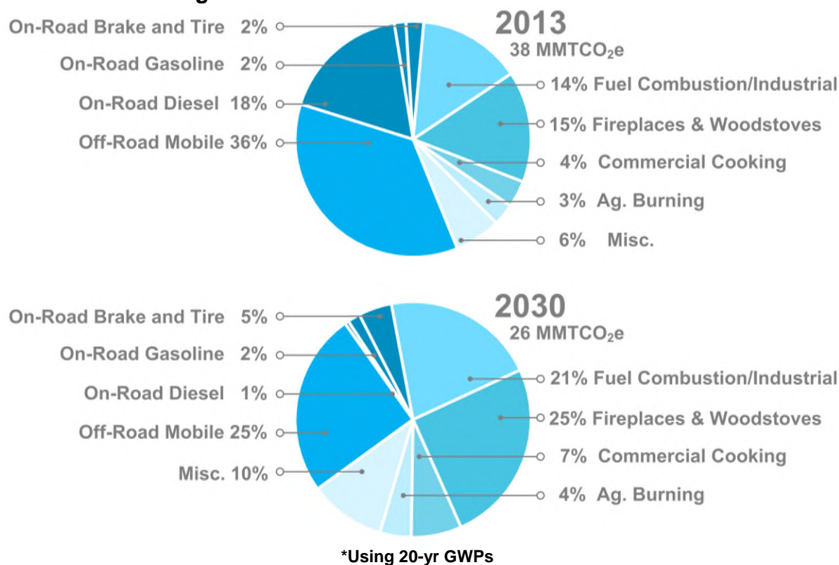
Figure 1. 2013 Black Carbon Emissions and Projected 2030 Emissions* with Existing Measures 4
