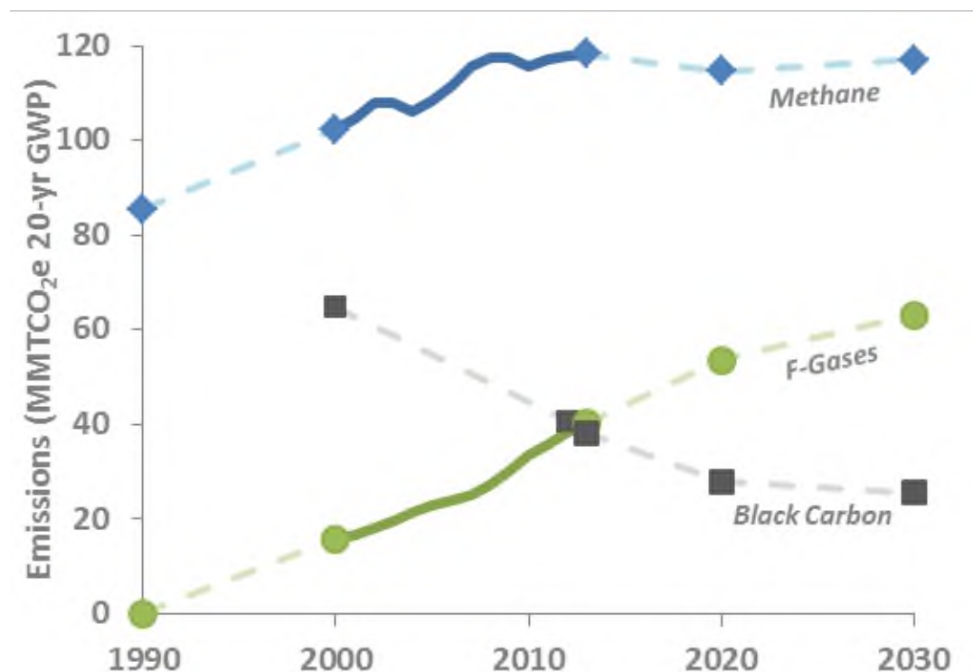
Figure 7. Trends in Methane, F-gases (HFCs), and Black Carbon Emissions with Existing Measures Using 20-year GWPs. 17
