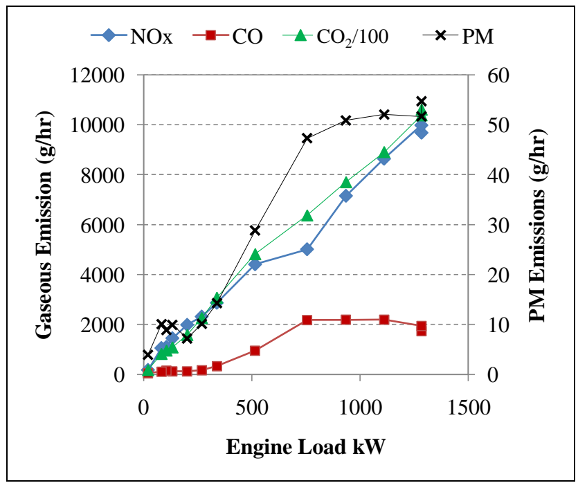
Figure 3-20 Emissions Profile of Main Engine on Hybrid Tug QSK50-M
