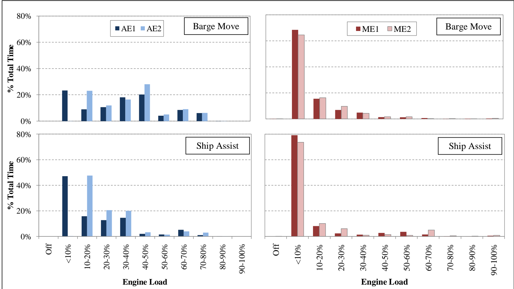
Figure 3-10 Engine Histograms for the Hybrid Tug without Batteries -3
