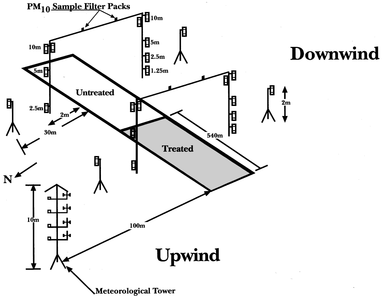
Figure B-1 DRI Testing Equipment and Site Layout
