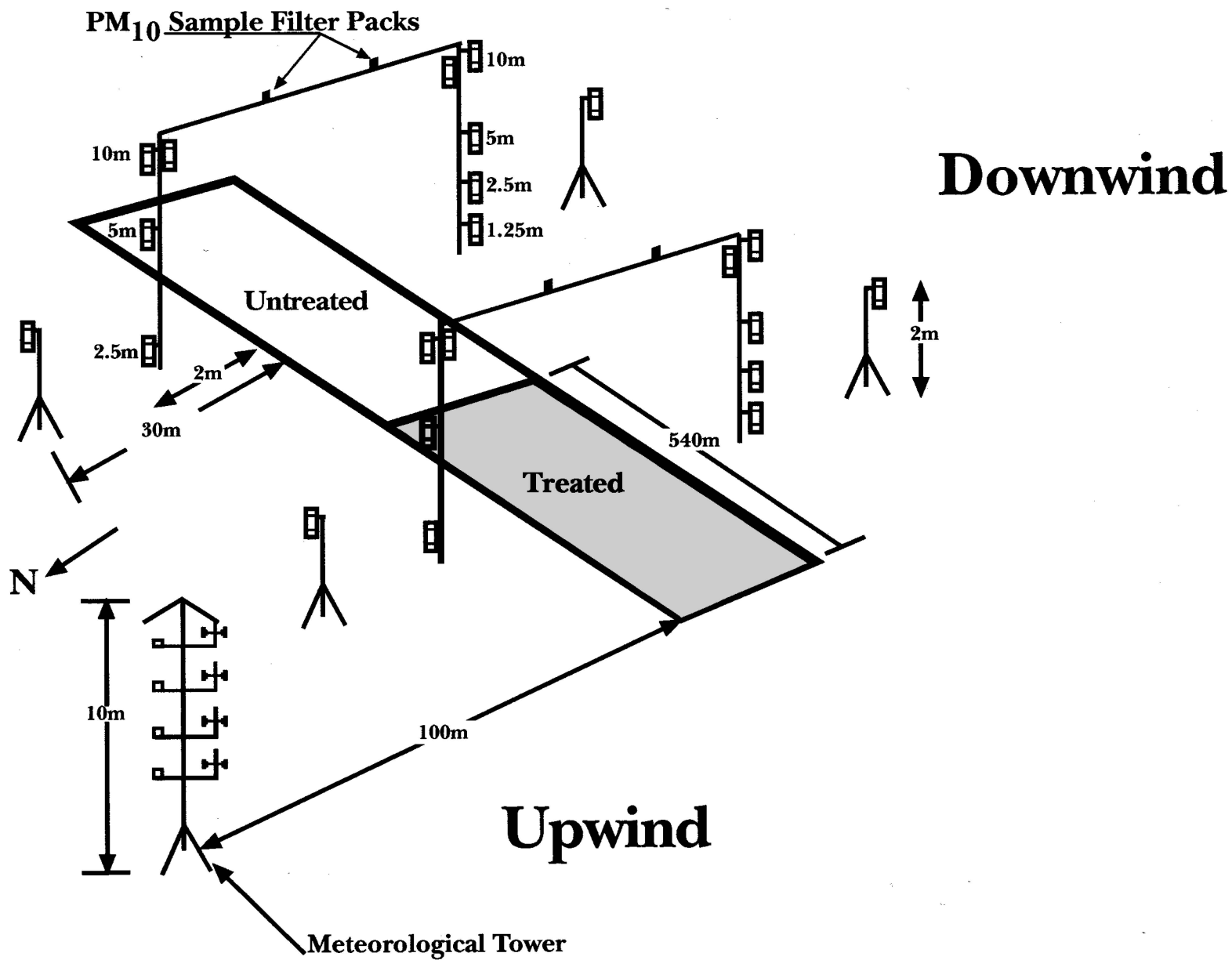
Figure B-2 DRI Testing Equipment and Site Layout
