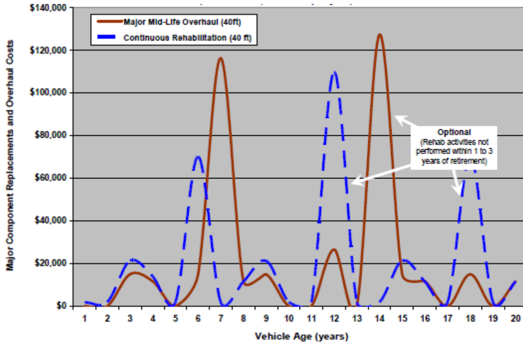
Figure 2: Life Cycle Cost Profile: Major Component Replacements and Overhauls
