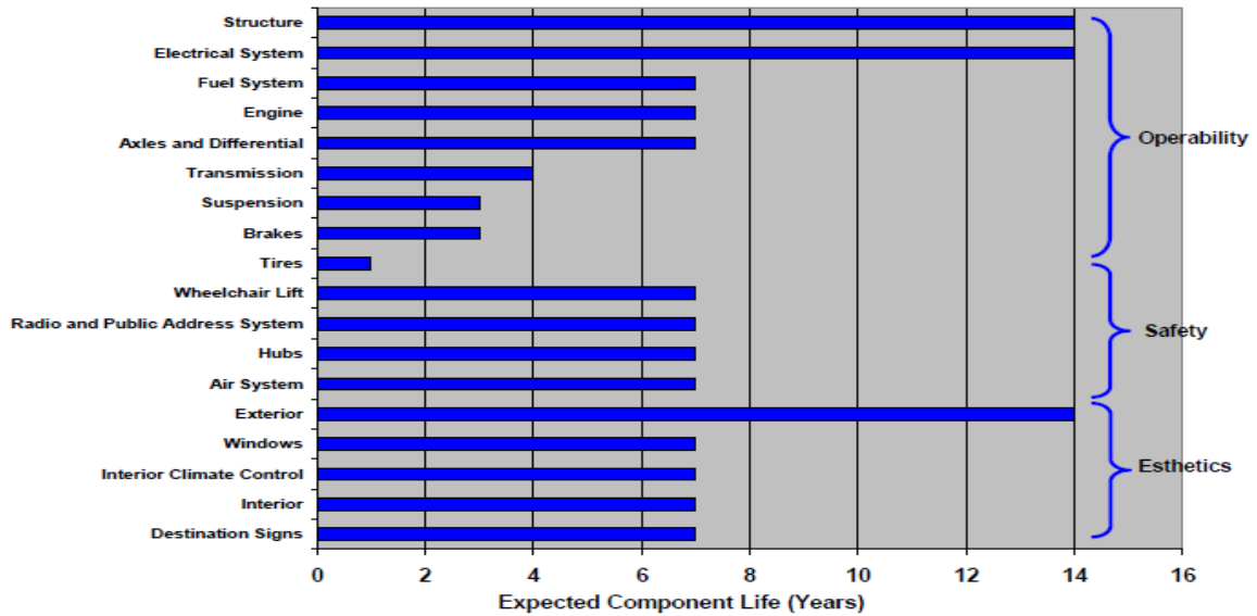
Figure 3: Useful Life of Transit Buses and Vans
