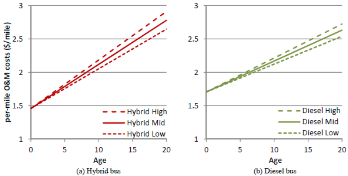
Figure 1: Operating and Maintenance Cost with Age (Diesel and Diesel Hybrid)
