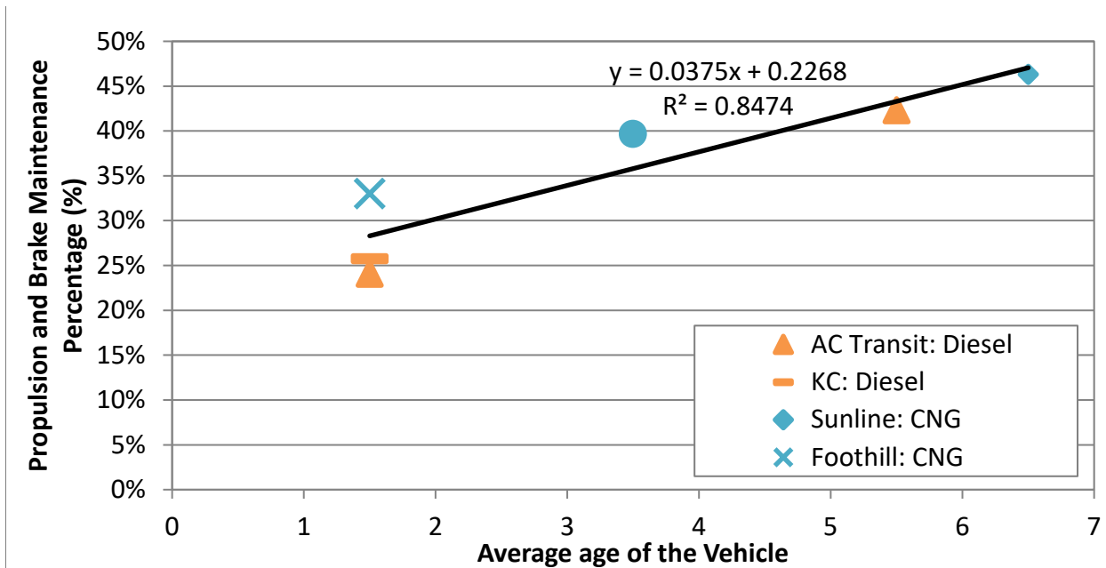
Figure 4 Conventional Bus Propulsion Plus Brake Maintenance Costs
