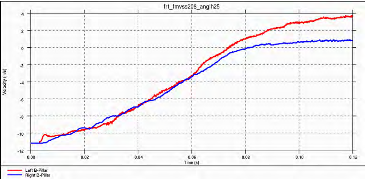
Figure 4.3.3.d: Vehicle velocity during 30°, left-side frontal impact - time to 0 velocity (TTZ) = 76 ms
