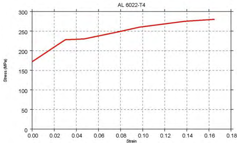
Figure 4.2.2.2.b: 6022 aluminum stress-strain curve
