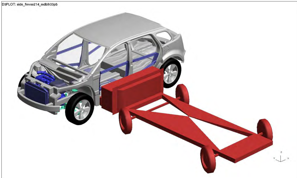
Figure 4.2.5.7.a: Crabbed barrier test model setup
