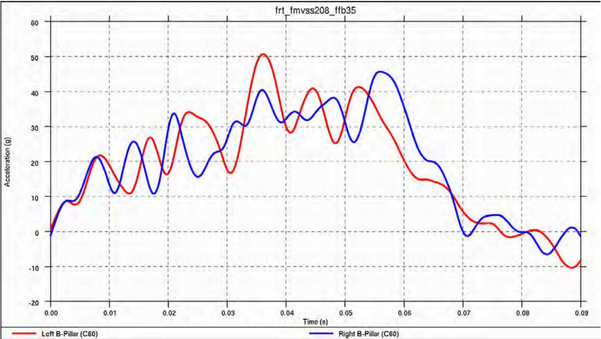
Figure 4.3.1.b: Vehicle acceleration pulse during frontal impact
