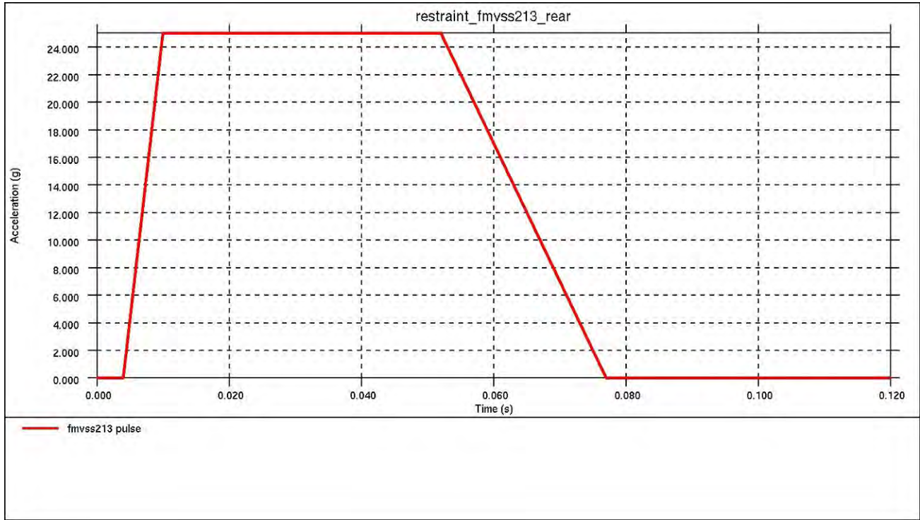
Figure 4.2.5.6.a: Acceleration pulse applied to child-restraint model
