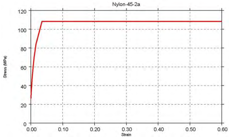
Figure 4.2.2.4.a: 45-2a nylon stress-strain curve
