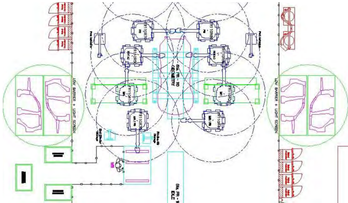
Figure 2.7.aj: Station FR110 assembly layout
