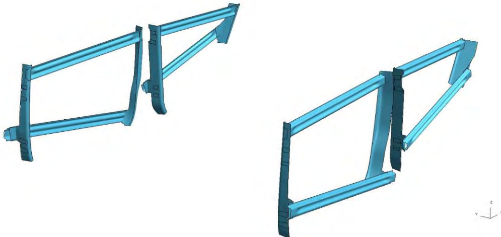
Figure 4.2.1.2.a: Simulated door beams
