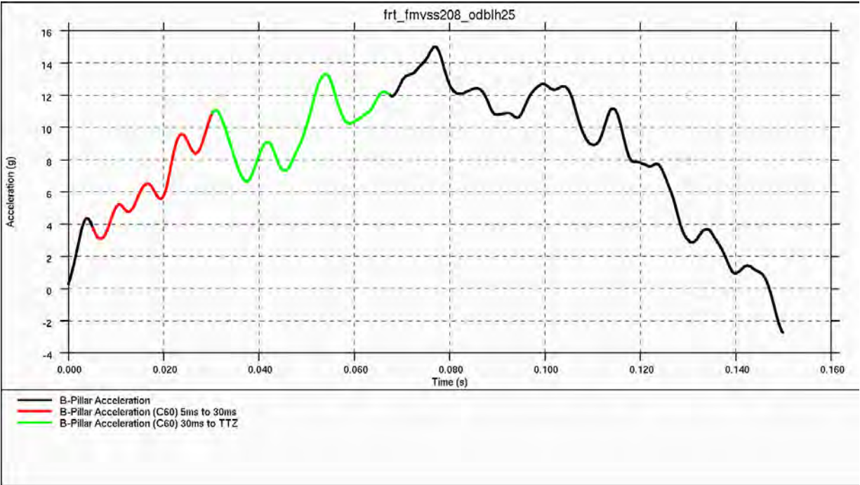
Figure 4.3.2.d: Average vehicle pulse during 40-percent overlap frontal impact
