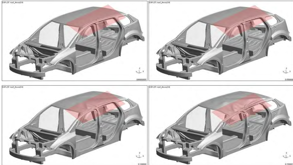
Figure 4.5.4.4.b: Deformation at 0/40/80/150mm of Platen Displacement
