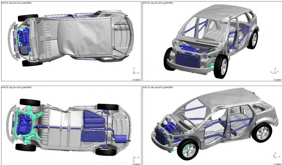
Figure 4.3.8.b: Vehicle deformation after 75°, side, pole impact (pole blanked) – 5 th percentile female
