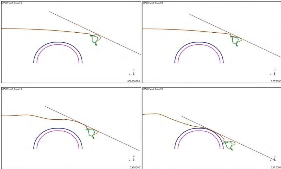
Figure 4.3.10.b: Deformation in relation to occupant head clearance zones (95 th /99 th ) at 0/40/80/150 mm of roof crush platen displacement
