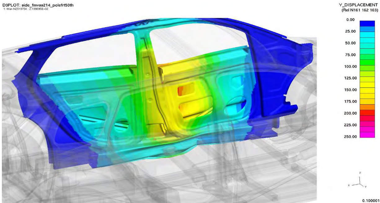
Figure 4.5.4.3.f: Intrusion levels on struckside after 20-mph, 75-degree side-pole impact - front (50 th percentile male)
