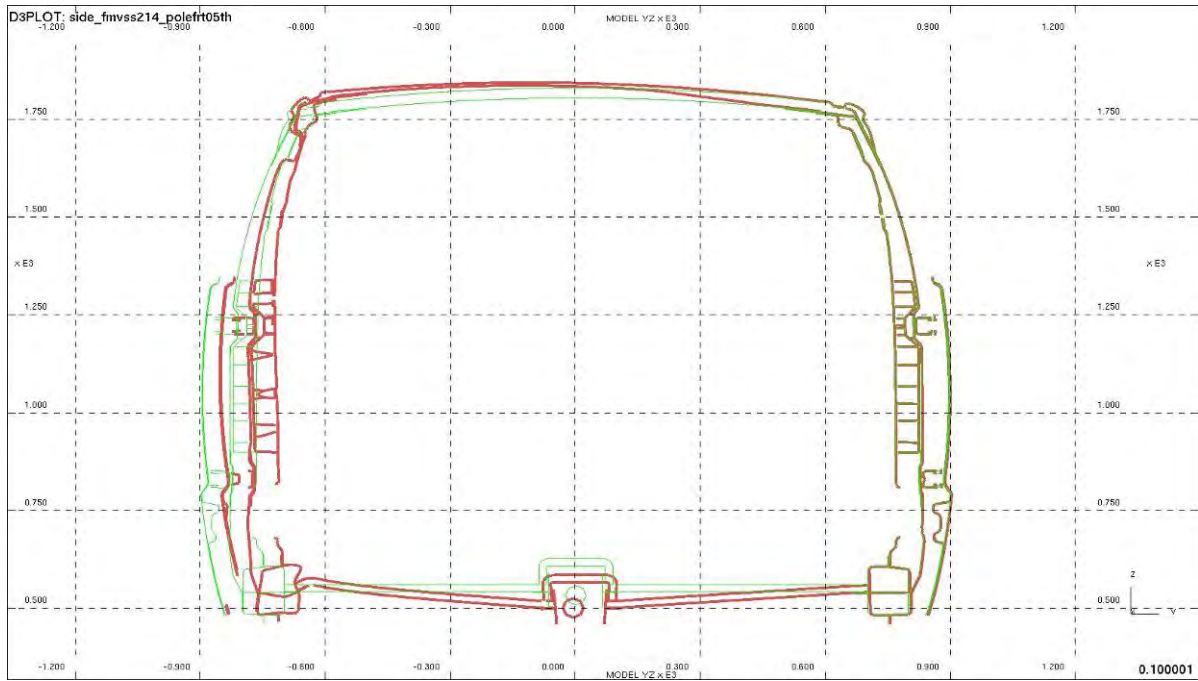
Figure 4.5.4.2.f: Section through B-Pillar, x= 2842
