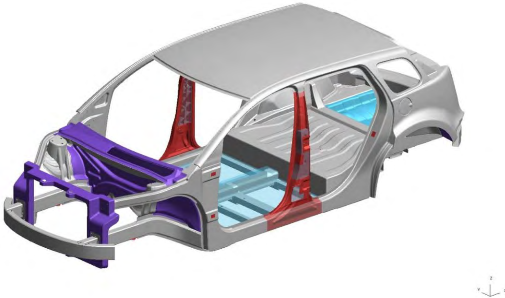
Figure 4.2.3.a: Body-in-white material usage front three-quarter view
