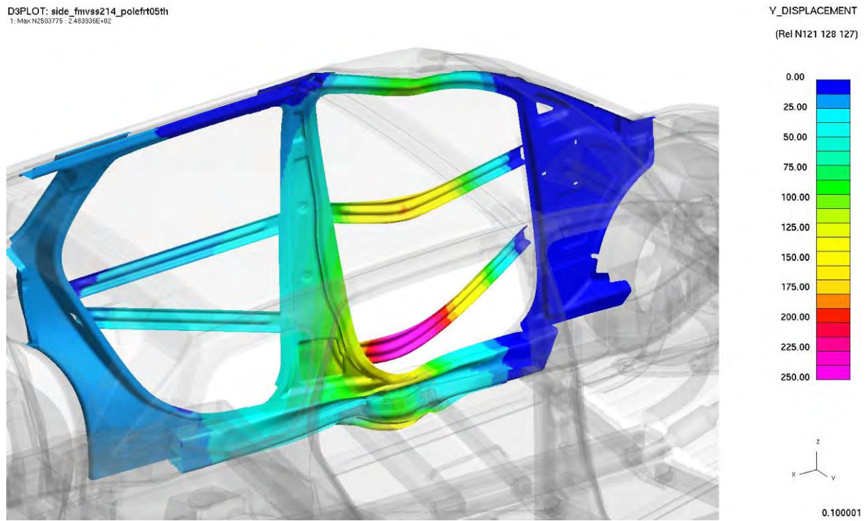
Figure 4.3.8.f: Intrusion levels after 75°, side, pole impact on struck side – 5 th percentile female
