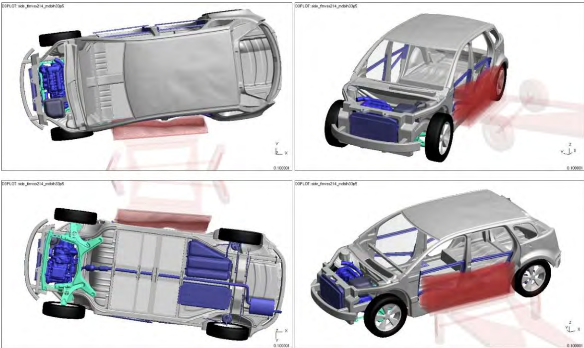
Figure 4.3.7.a: Vehicle deformation (0.1 s) after crabbed barrier impact
