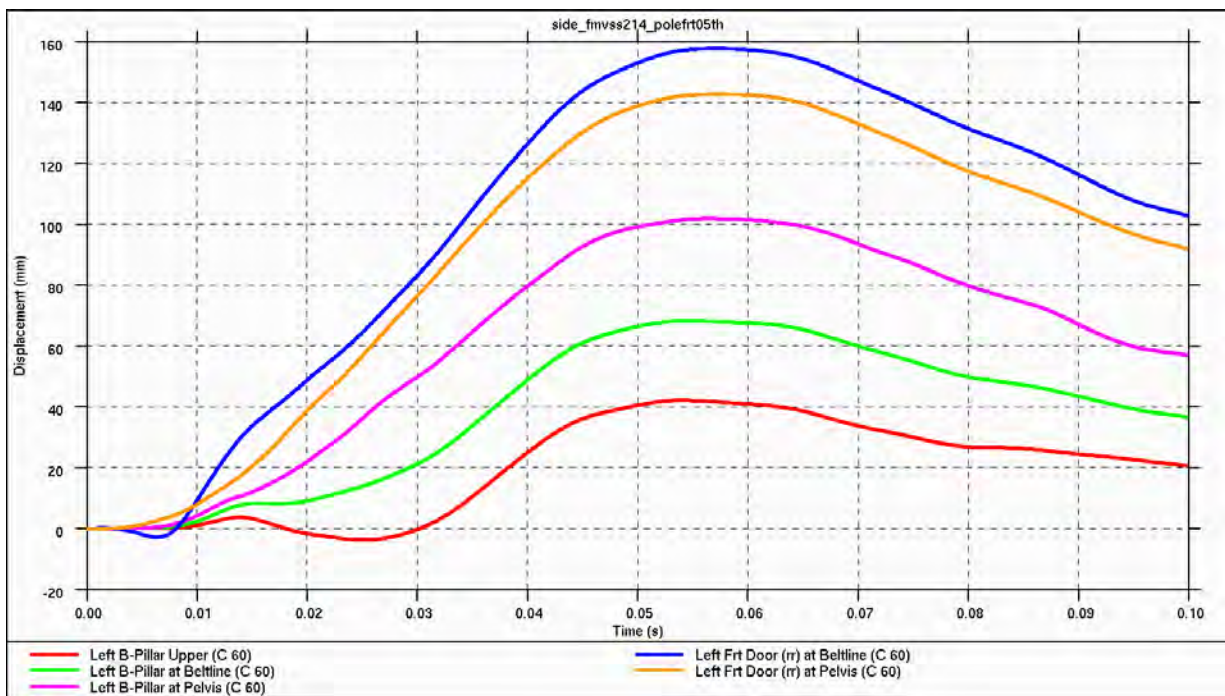
Figure 4.5.4.2.e: Intrusion Displacements (B-Pillar& Front Door)
