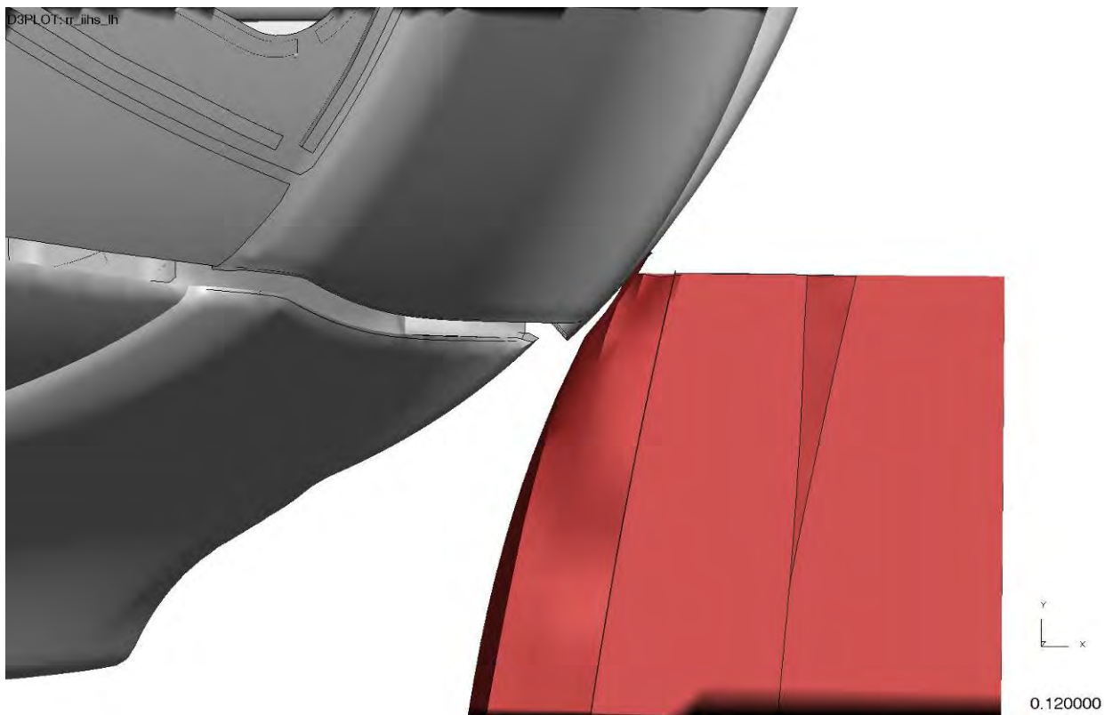
Figure 4.5.4.6.1.b: 'Deformation' @ maximum deflection
