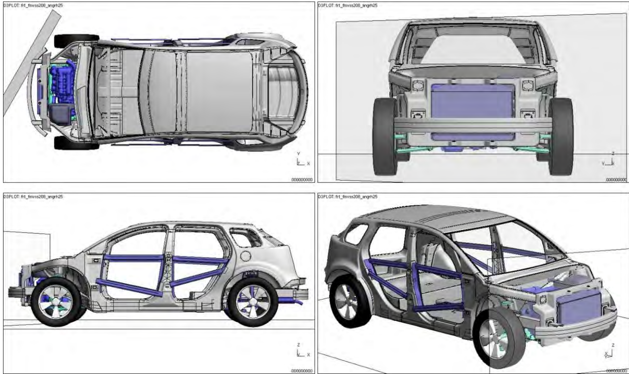
Figure 4.2.5.4.a: 30°, right-side barrier crash-test model setup
