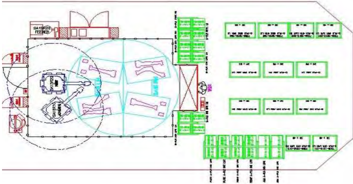
Figure 2.7.c: Station SA15 layout
