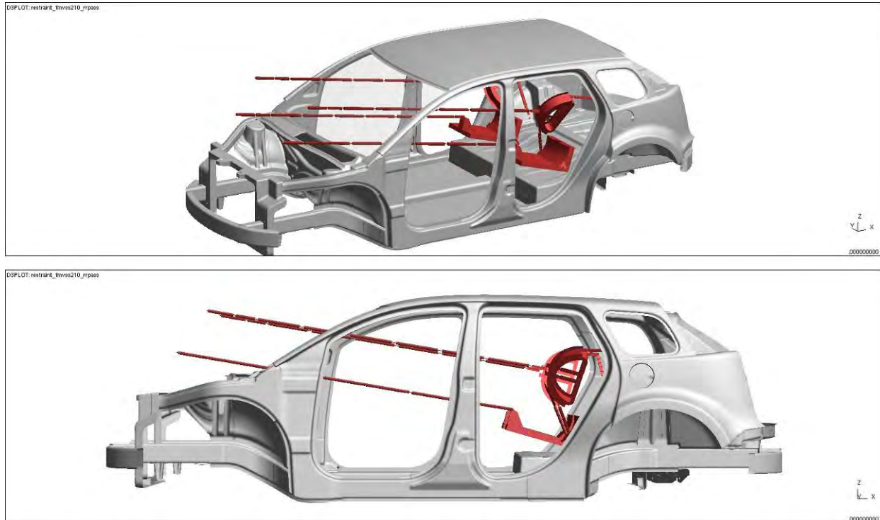
Figure 4.2.5.5.b: Rear seatbelt anchorage test model setup
