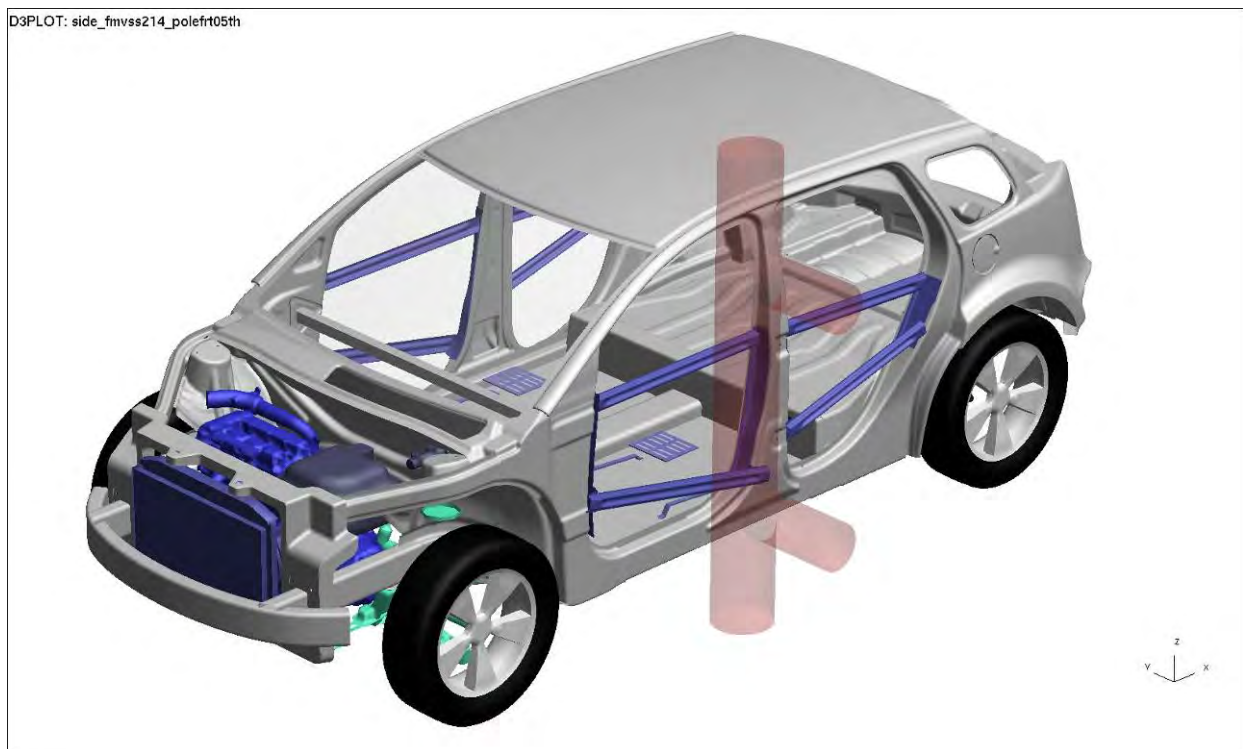
Figure 4.2.5.8.a: Side-pole impact test model setup
