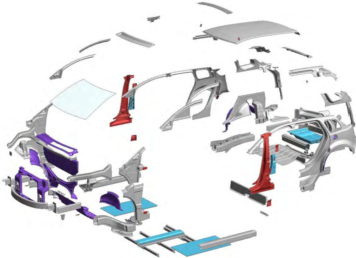
Figure 4.2.3.d: Body-in-white Material Usage Exploded View
