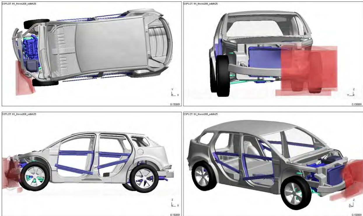
Figure 4.3.2.a: Vehicle deformation (t=0.15 s) after 40-percent overlap frontal impact
