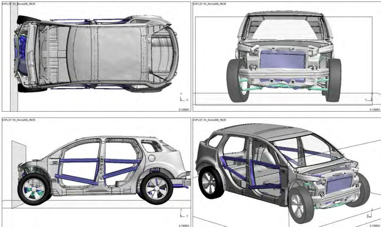
Figure 4.3.1.a: Vehicle deformation (t=0.1 s) after frontal impact
