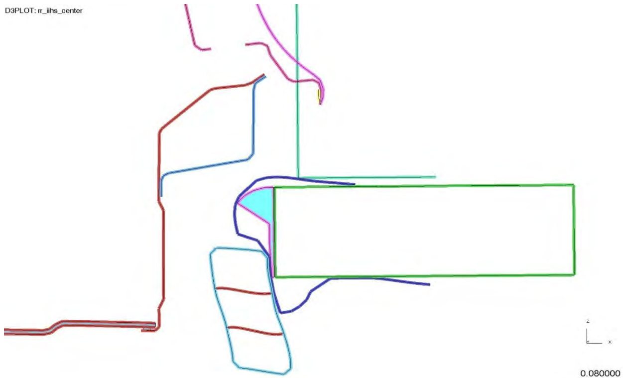
Figure 4.5.4.6.1.a: Maximum deflection showing barrier intrusion into tailgate
