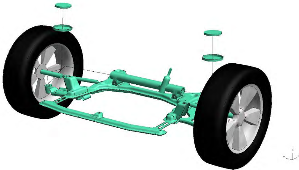
Figure 4.2.1.3.a: Front sub-frame and suspension
