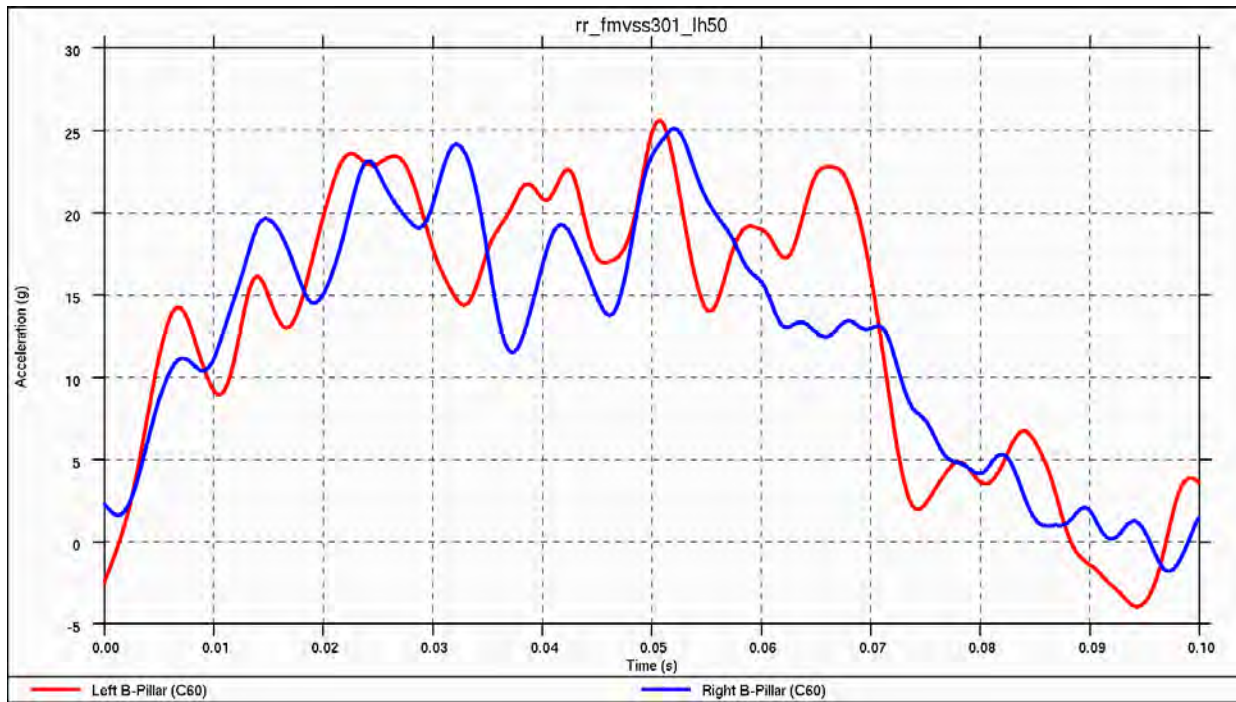
Figure 4.3.11.d: Vehicle acceleration pulse during rear deformable barrier impact
