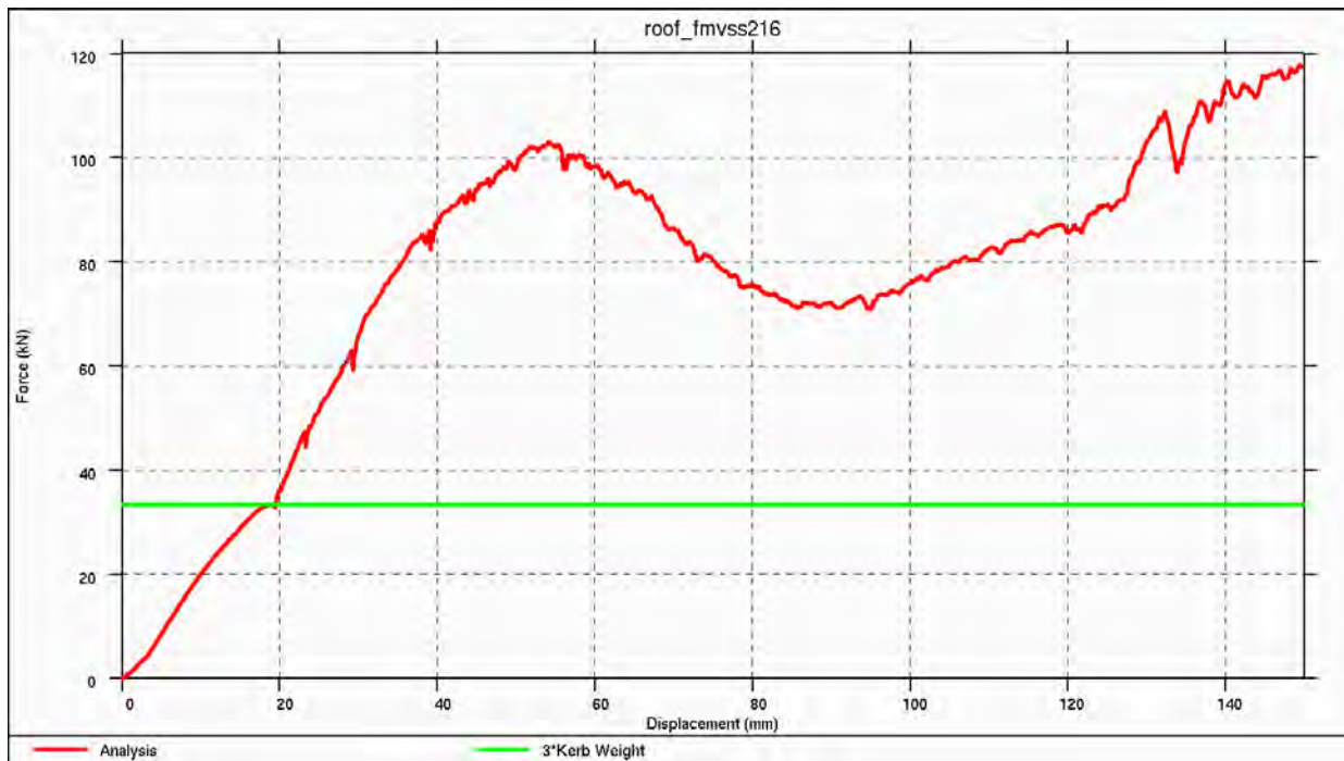
Figure 4.3.10.c: Roof displacement vs. applied force – 3 times curb weight
