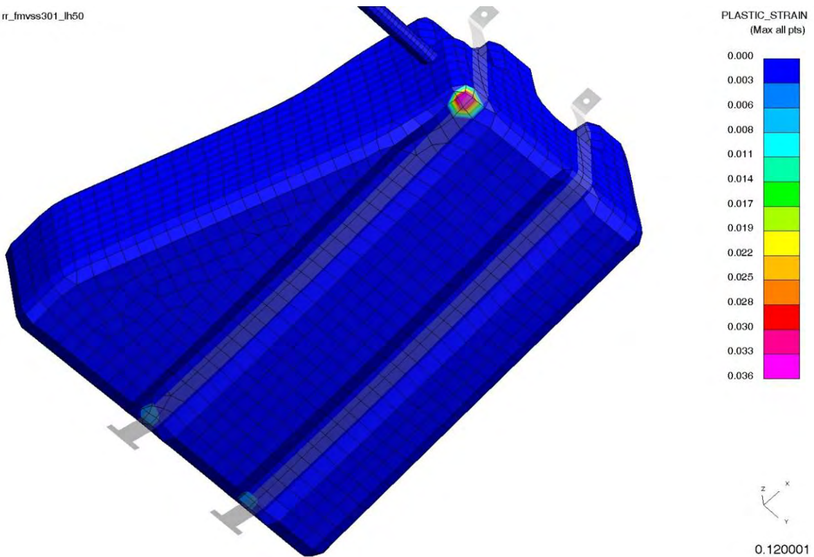
Figure 4.5.4.5.1.a: Fuel Tank Plastic Strain location after rear impact
