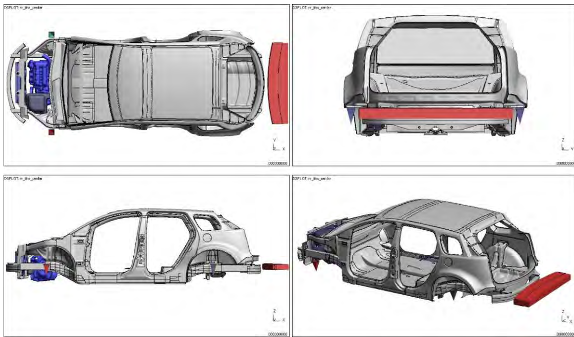
Figure 4.2.5.13.a: IIHS, low-speed rear test model setup ('full impact')
