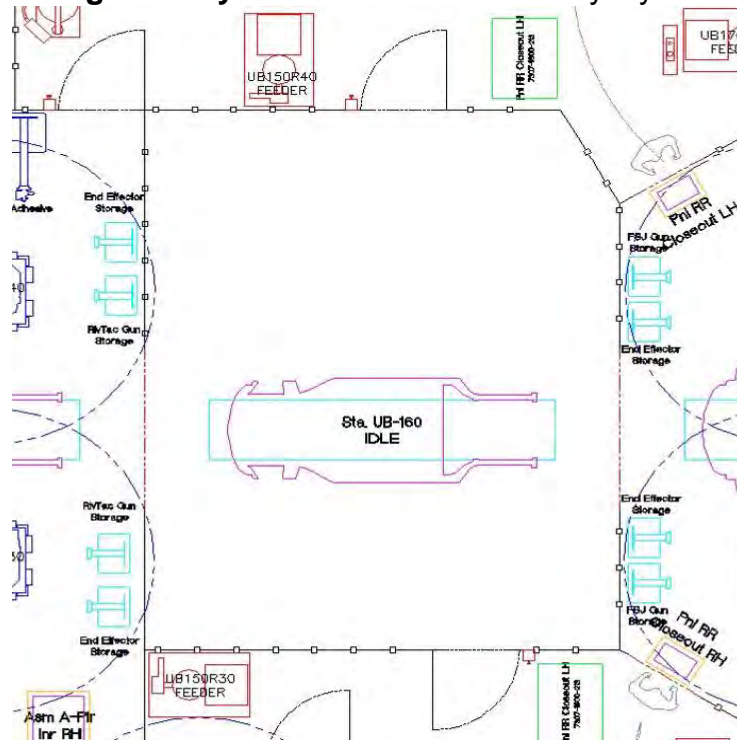
Figure 2.7.z: Station UB160 assembly layout
