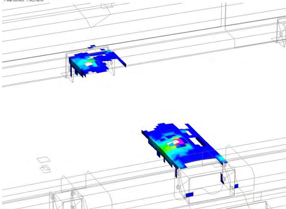
Figure 4.3.5.1.c: Lower seatbelt anchorage plastic strain (@ 0.2 s)
