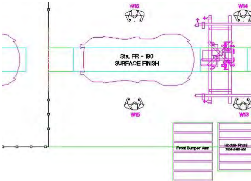
Figure 2.7.ar: Station FR190 assembly layout
