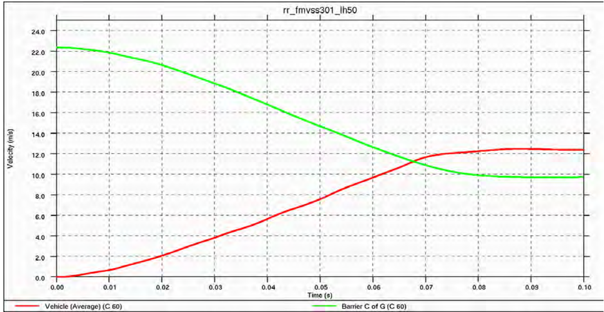
Figure 4.5.4.5.f: Vehicle & Barrier Velocities during rear impact simulation
