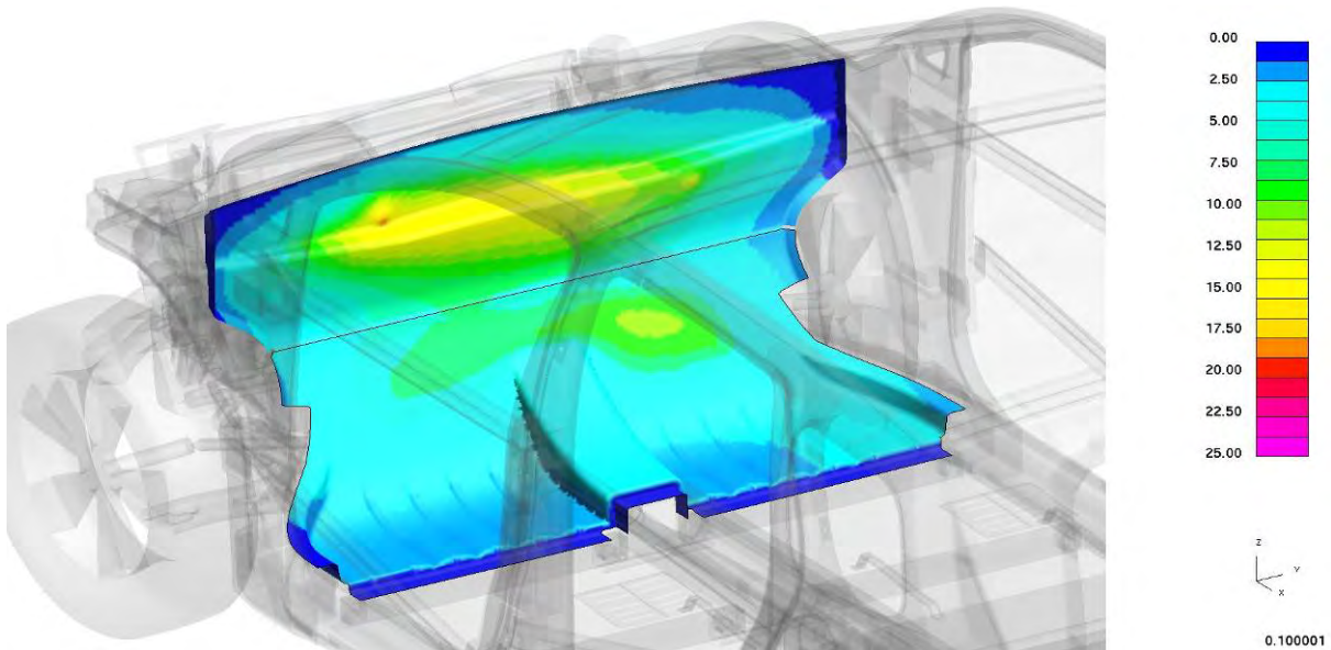
Figure 4.3.1.g: CAE dash intrusion analysis after frontal impact
