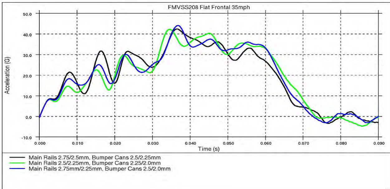
Figure 4.3.1.e: Vehicle acceleration during frontal impact
