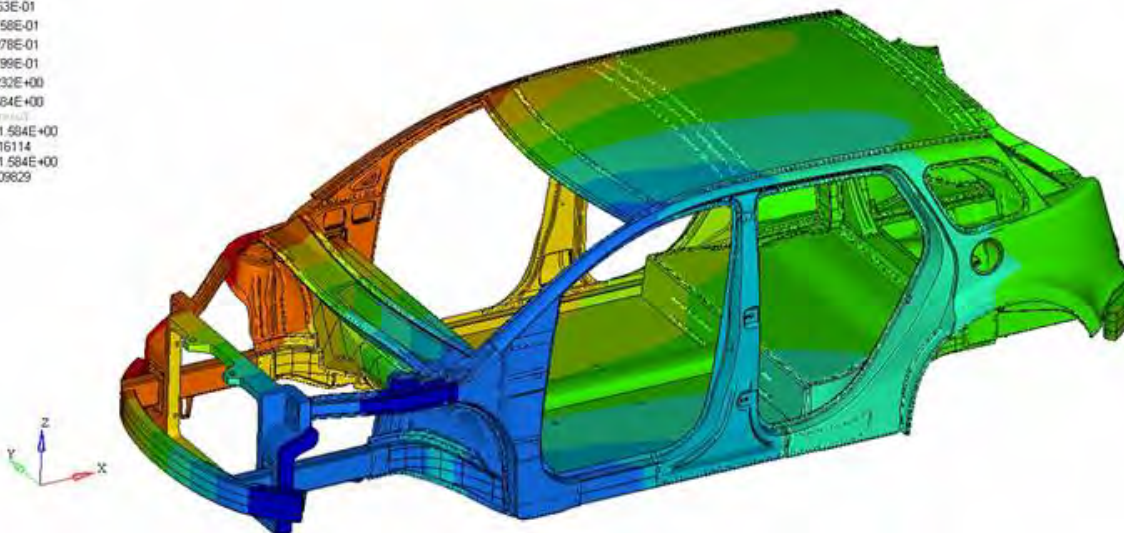
Figure 4.3.14.a: CAE body stiffness analysis
