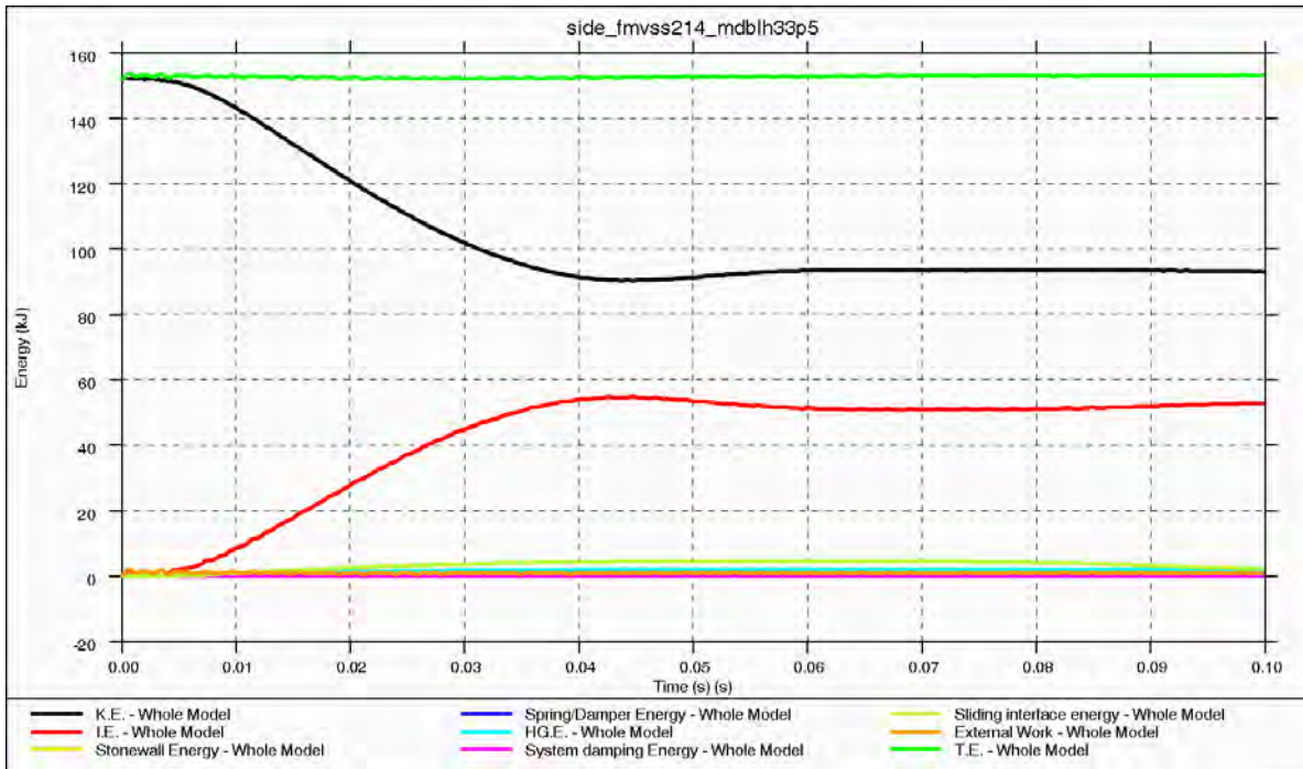
Figure 4.5.4.1.k: Energy Balance
