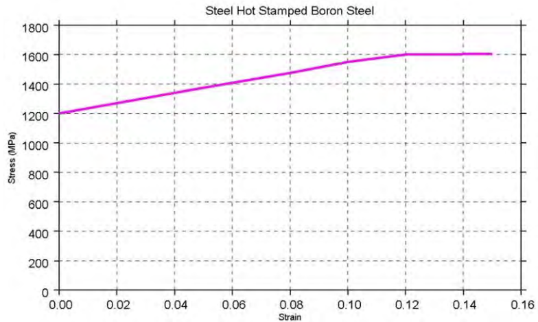
4.2.2.1.c: Hot-stamped, boron steel stress-strain curve
