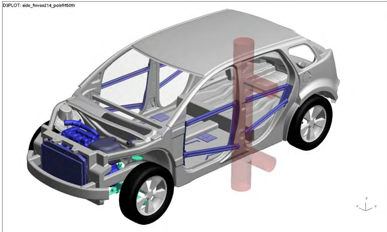
Figure 4.2.5.9.a: Side-pole impact test model setup
