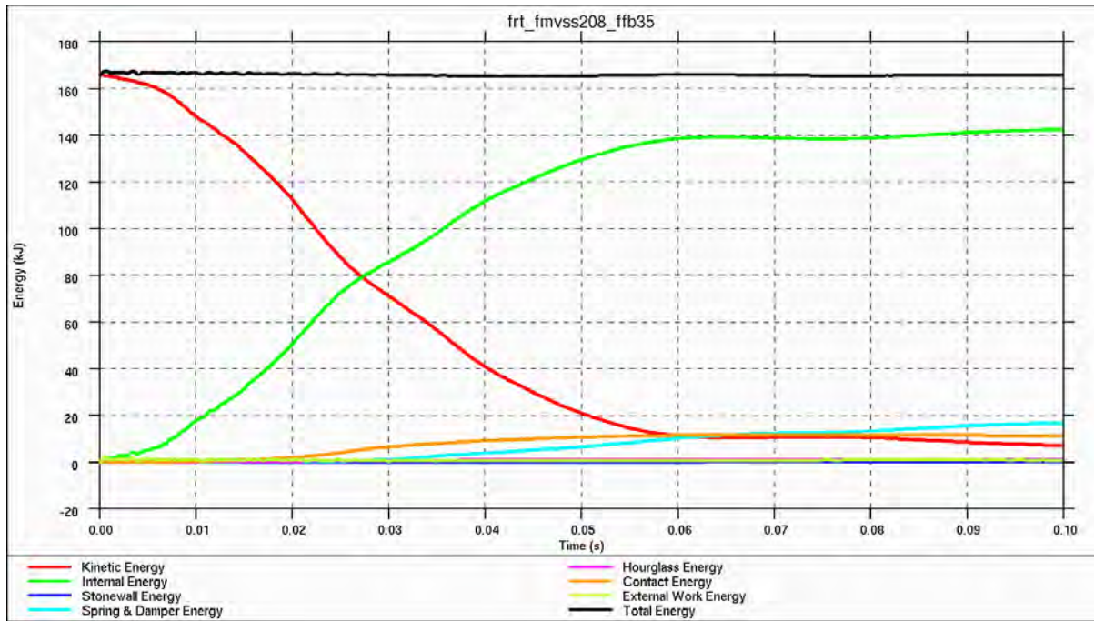
Figure4.3.1.j: Energy balance for frontal impact
