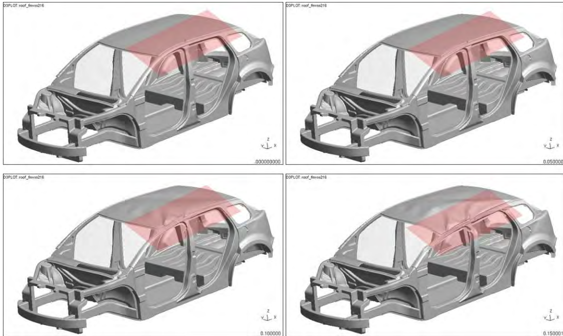
Figure 4.3.10.a: Deformation at 0/40/80/150 mm of roof crush platen displacement
