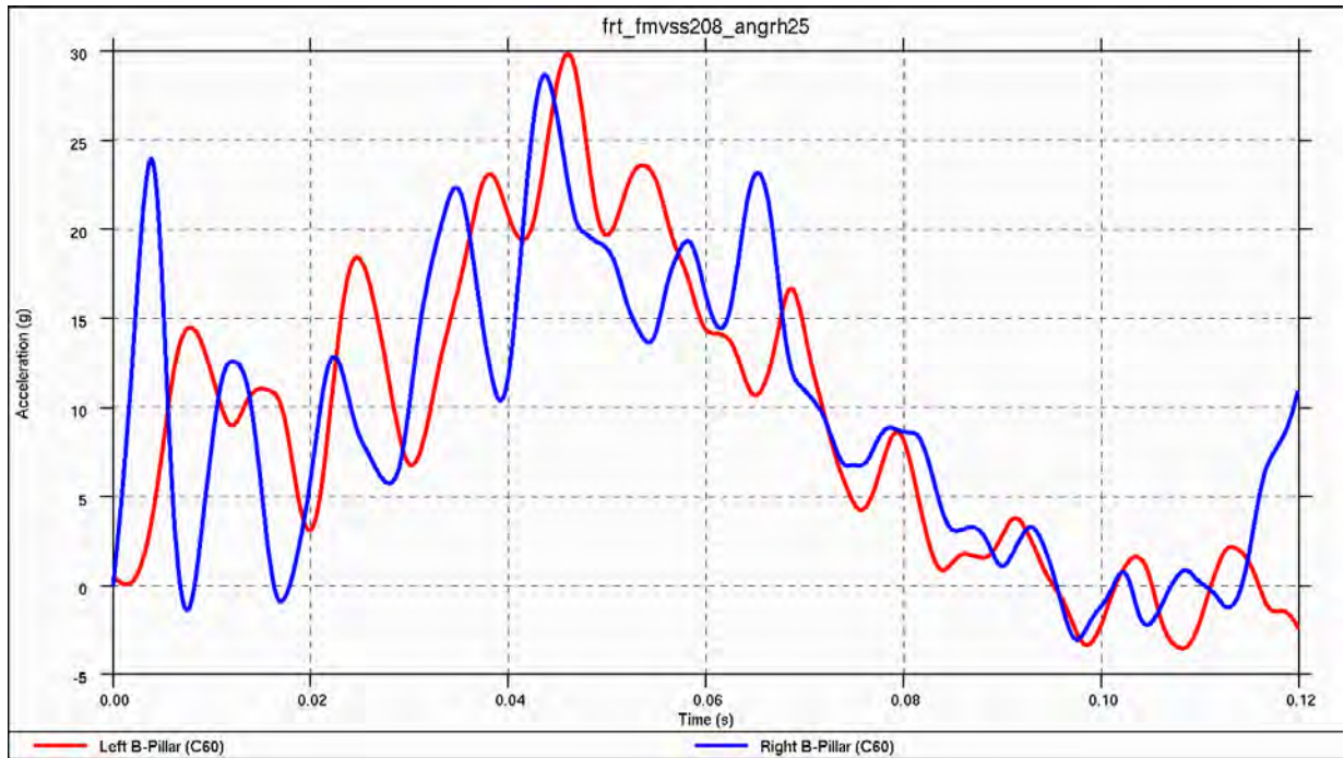
Figure 4.3.4.b: Vehicle acceleration pulse during 30°, right-side frontal impact
