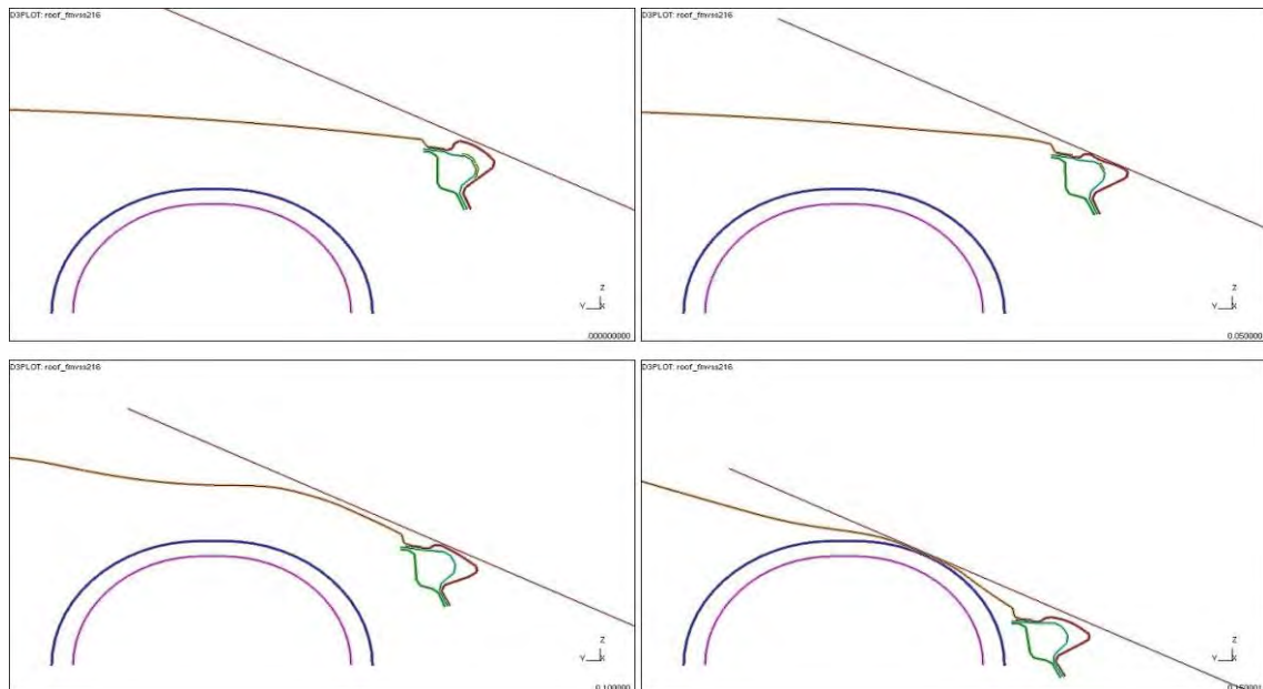
Figure 4.5.4.4.c: Deformation in Relation to occupant head clearance zones (95 th /99 th ) @ 0/40/80/150mm of Platen Displacement
