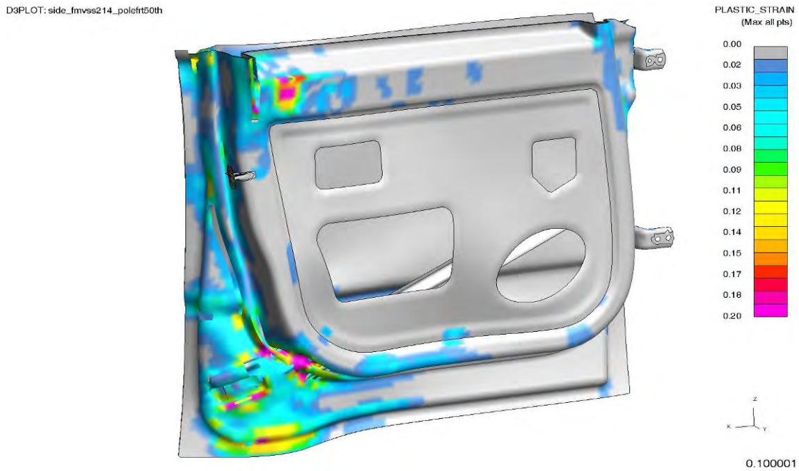
Figure 4.5.4.3.h: Plastic Strain in Front Door after 20-mph, 75-degree side-pole impact -- front (50 th percentile male)
