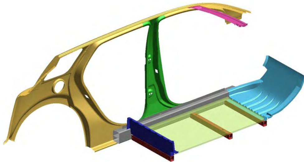
Figure 4.3.8.g: Main energy absorbing body structure for 75°, side, pole impact – 5 th percentile female
