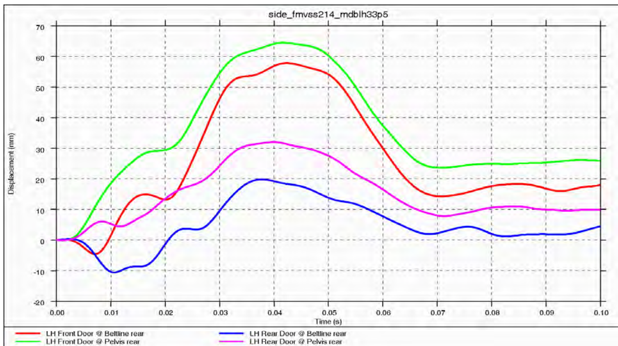
Figure 4.5.4.1.g: Relative Intrusion Displacements (Front/Rear Door)
