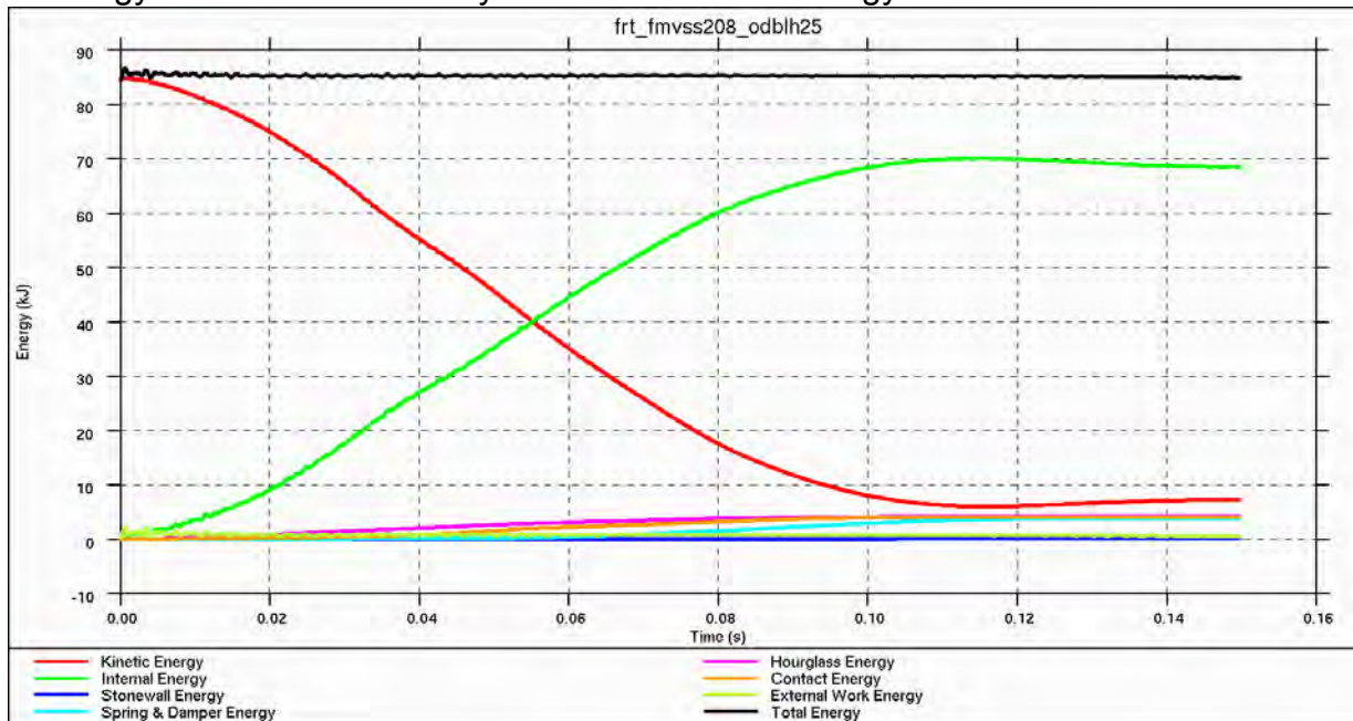
Figure 4.3.2.j: Energy balance for 40-percent overlap frontal impact
