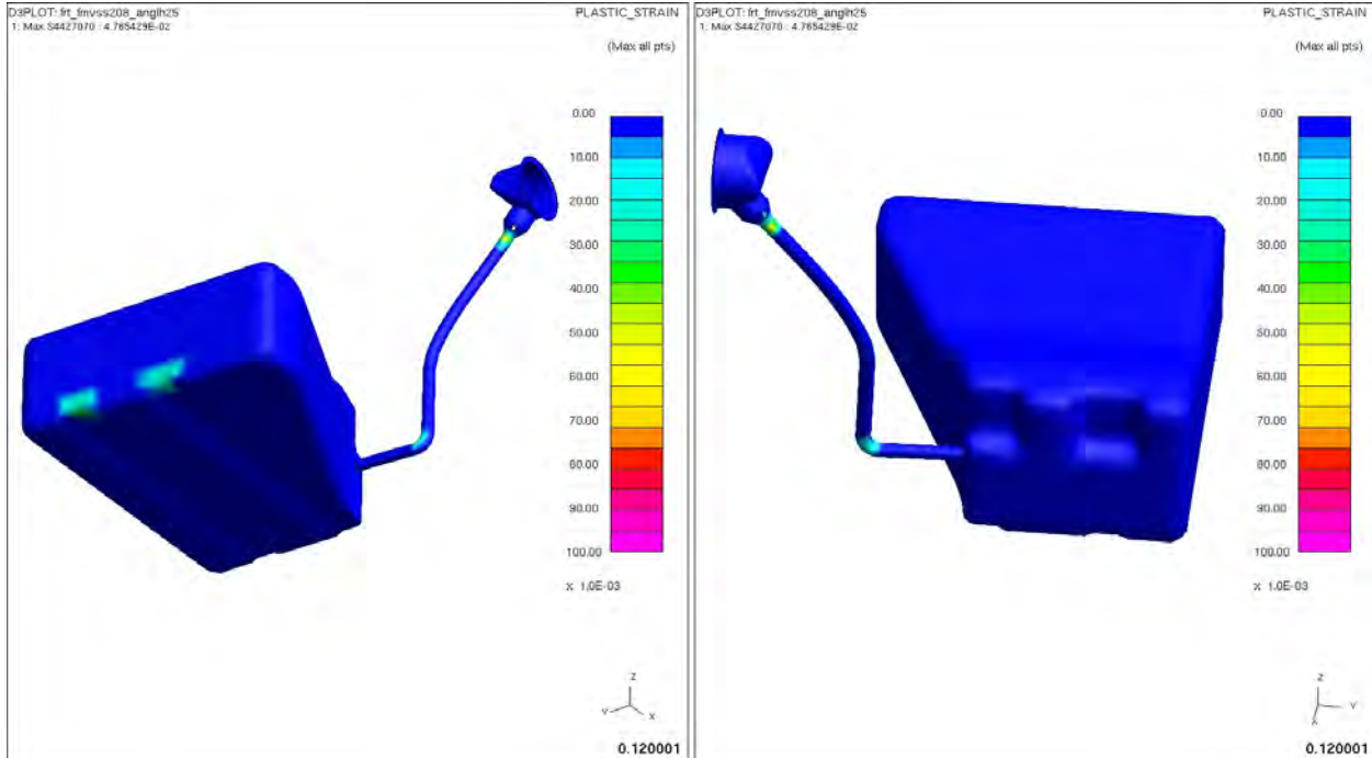
Figure 4.3.3.g: Fuel tank plastic strain after 30°, left-side frontal impact
