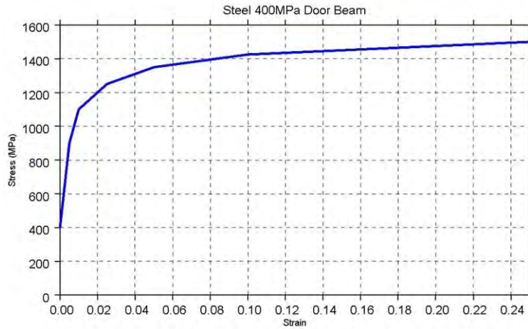
Figure 4.2.2.1.b: Steel stress-strain curve at 400 MPa
