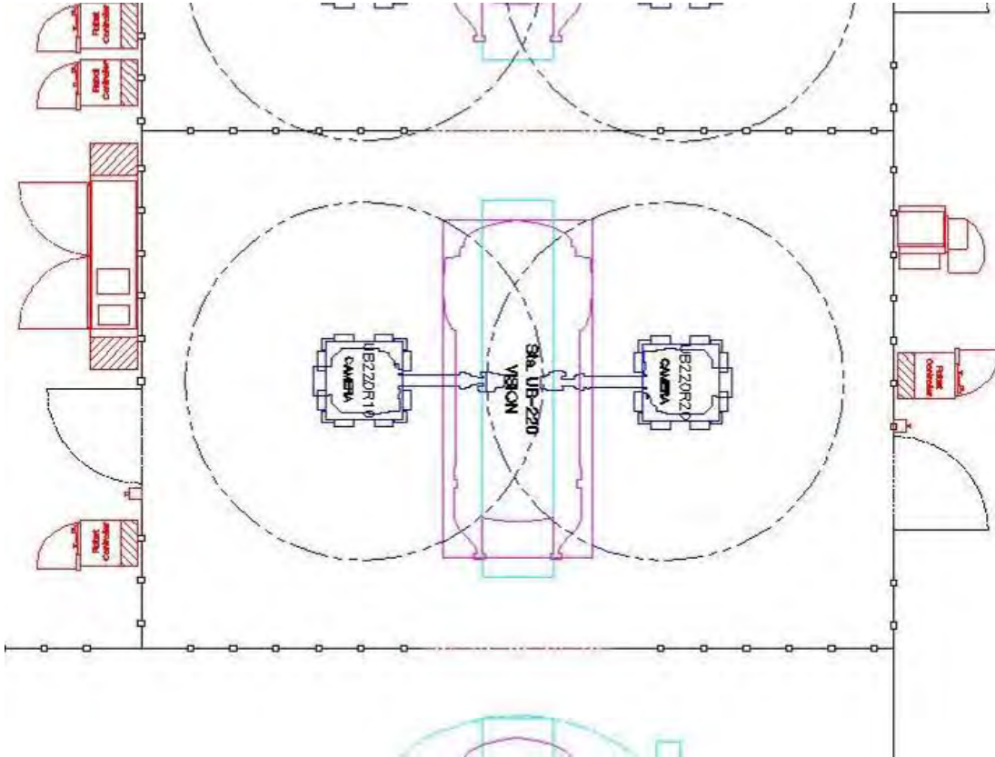
Figure 2.7.af: Station UB220 assembly layout
