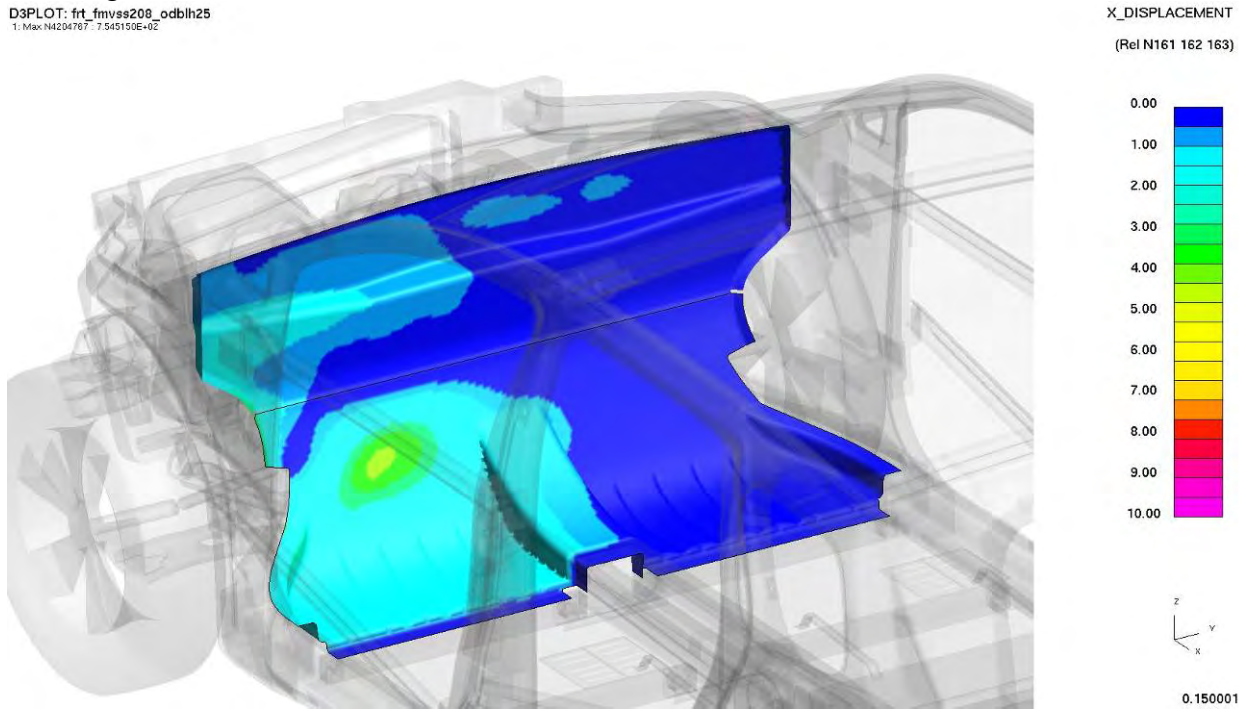
Figure 4.3.2.g: CAE dash intrusion analysis after 40-percent overlap frontal impact
