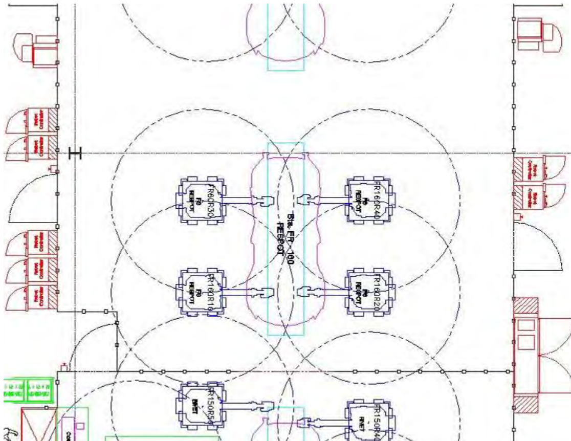
Figure 2.7.ao: Station FR160 assembly layout
