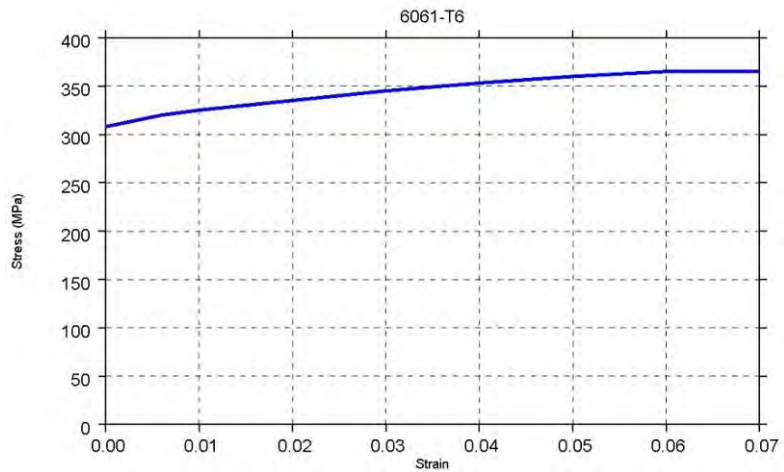
Figure 4.2.2.2.c: 6061 aluminum stress-strain curve
