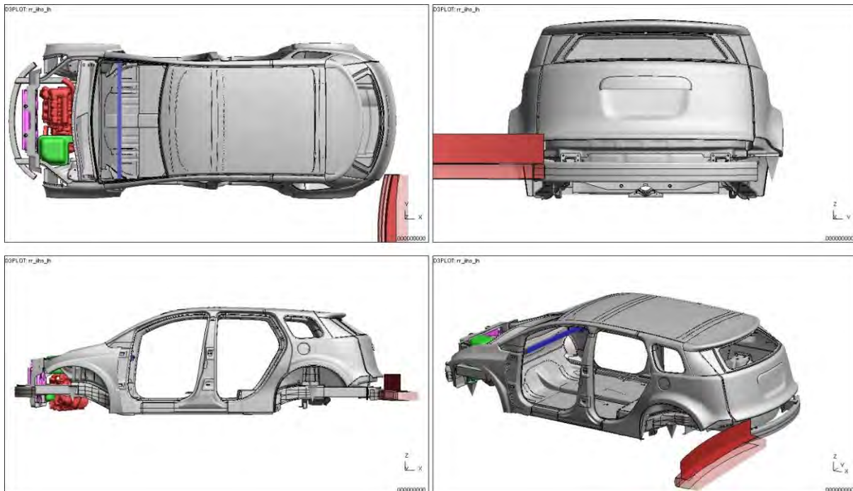
Figure 4.5.4.6.c: IIHS low-speed impact model setup ('offset')
