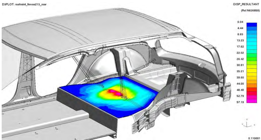
Figure 4.3.6.b: Child-restraint seat pan displacements
