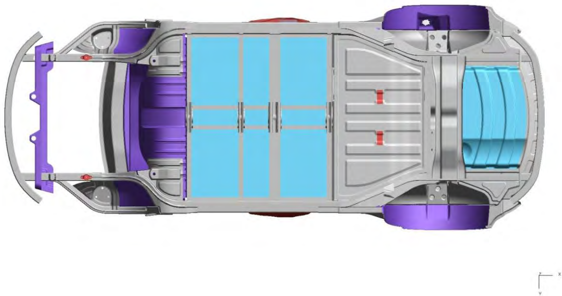
Figure 4.2.3.c: Body-in-white material usage underbody view
