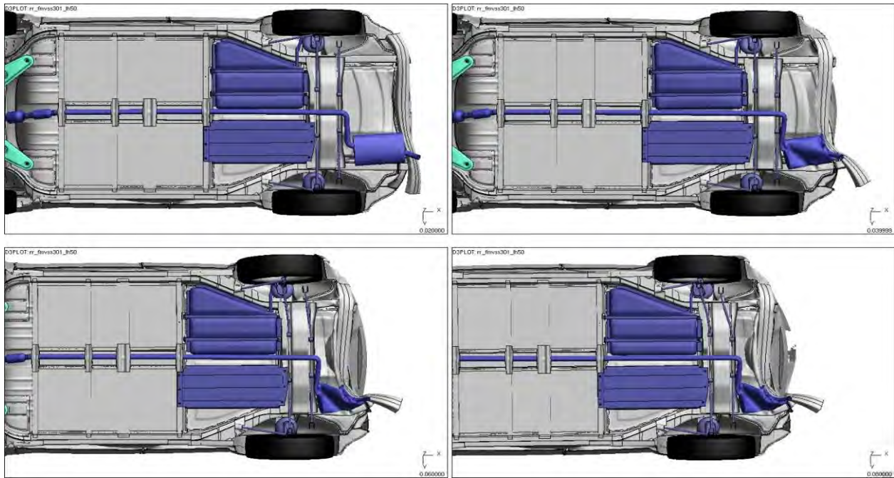
Figure 4.5.4.5.d: Vehicle Deformation (@ 0ms/40ms/80ms/120ms) after rear impact
