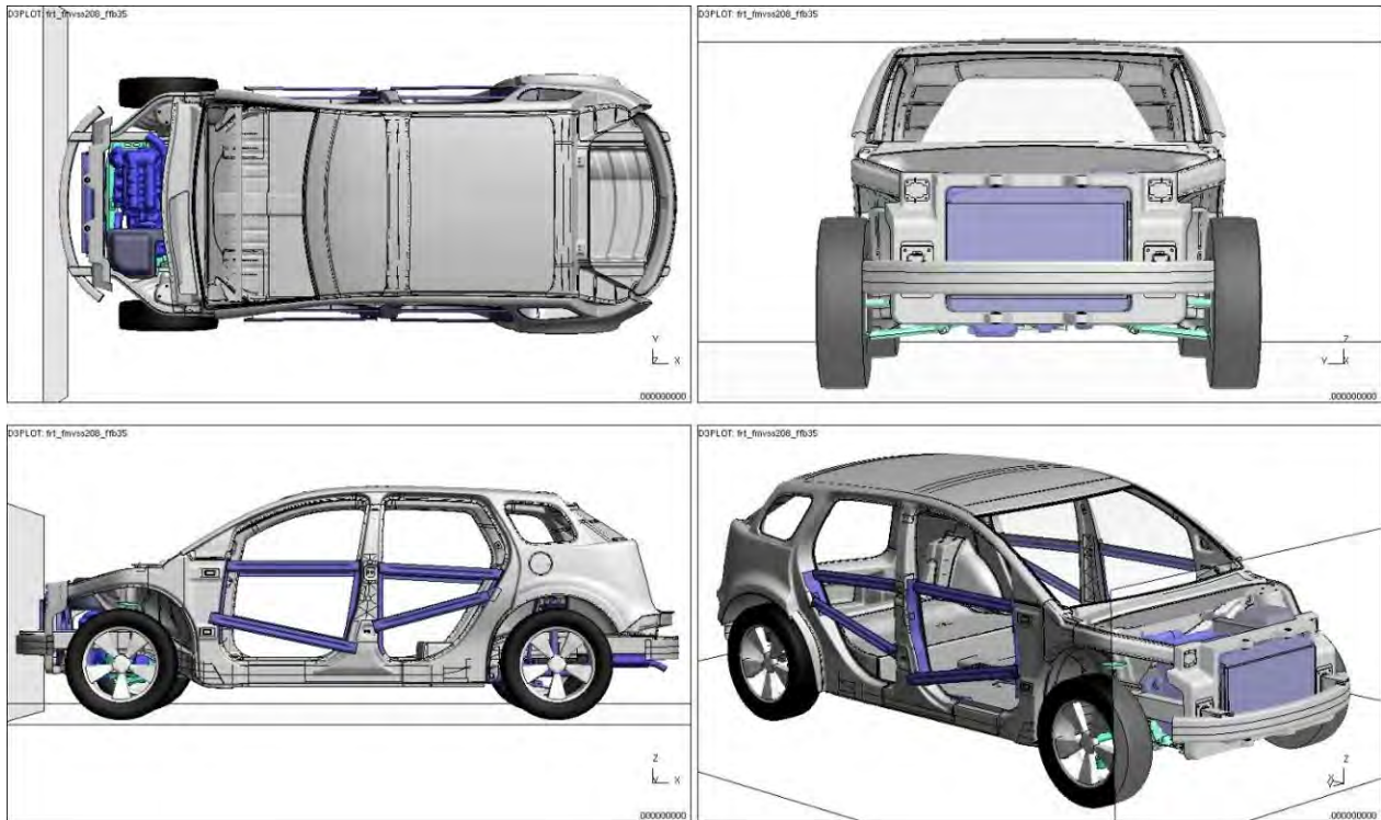
Figure 4.2.5.1.a: Rigid, deformable wall crash-test model setup
