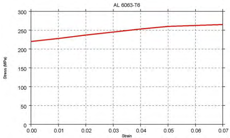
Figure 4.2.2.2.d: 6063 aluminum stress-strain curve
