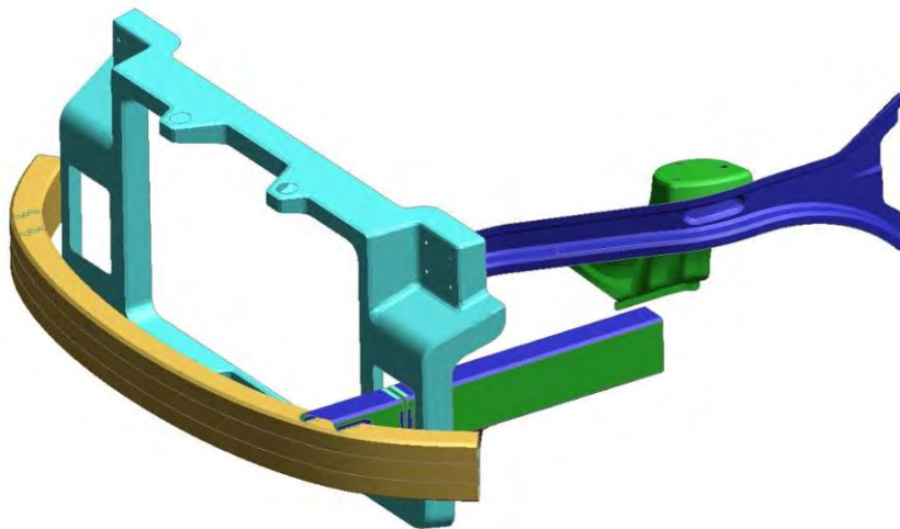
Figure 4.3.3.h: Main energy absorbing body structure for fuel tank plastic strain after 30°, left-side frontal impact
