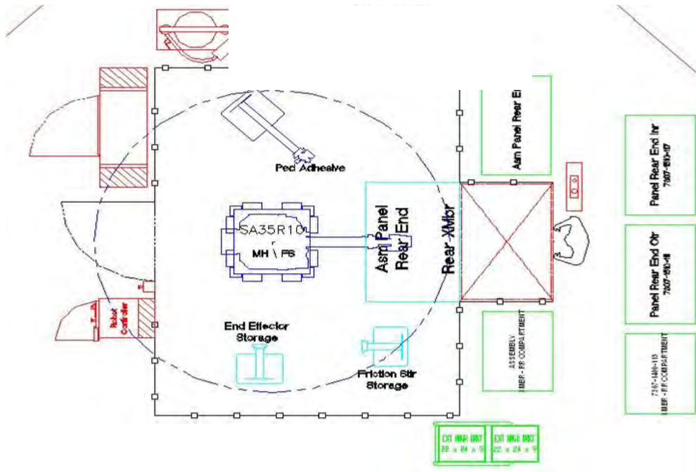
Figure 2.7.f: Station SA35 layout
