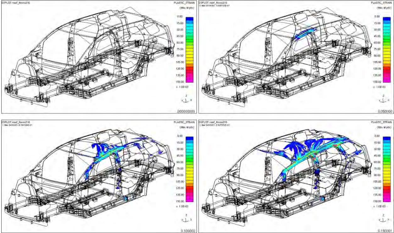
Figure 4.3.10.e: Roof plastic strains at 0/40/80/150 mm of roof crush platen displacement
