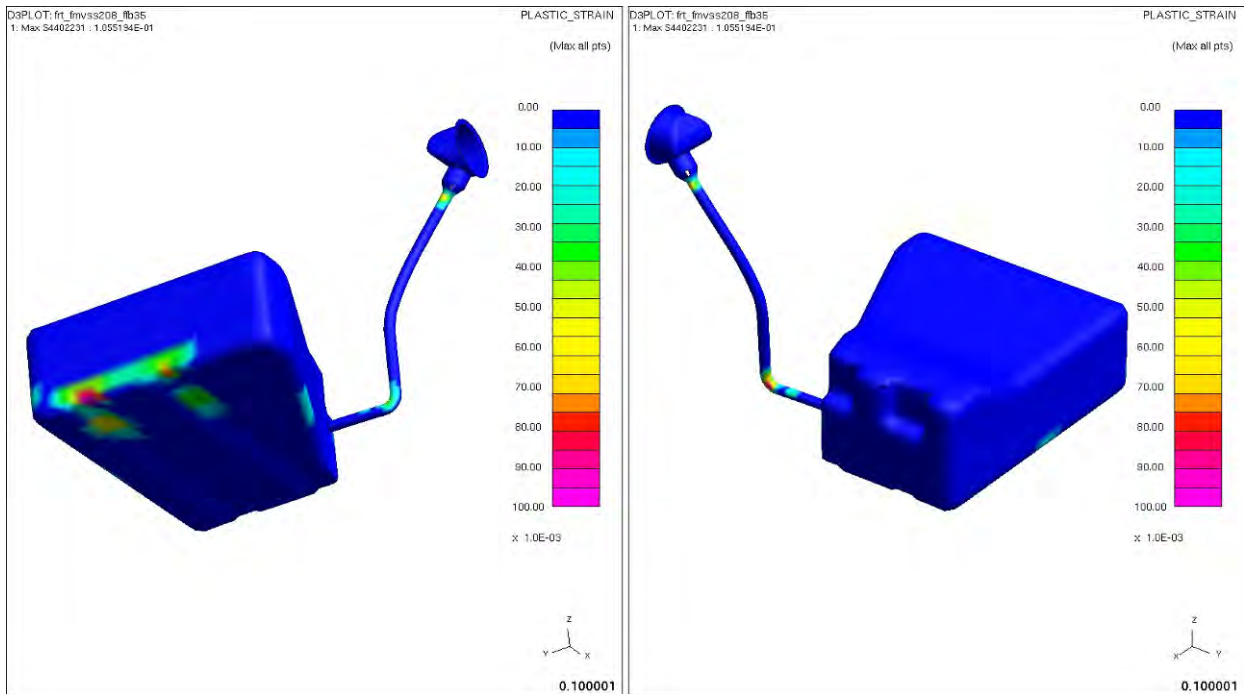
Figure 4.3.1.h: Fuel tank plastic strain after impact
