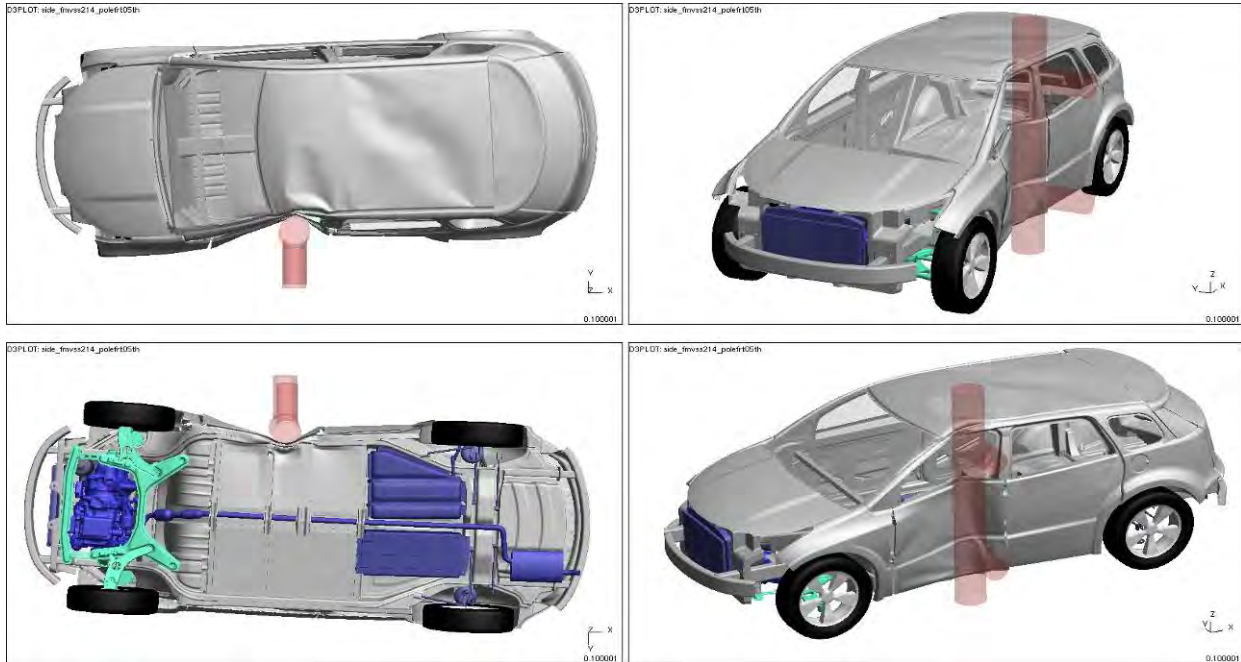
Figure 4.5.4.2.b: Vehicle Deformation (0.1s)
