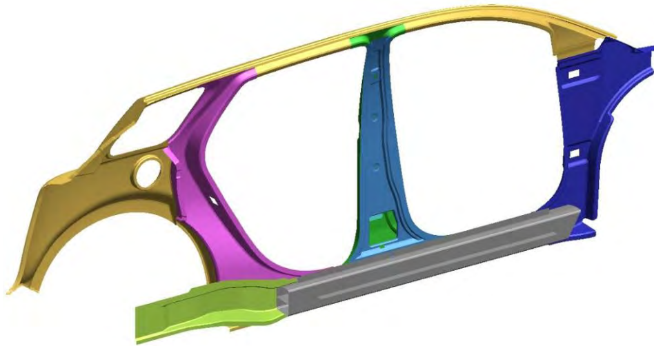
Figure 4.3.7.h: Main energy absorbing body structure parts for crabbed barrier impact
