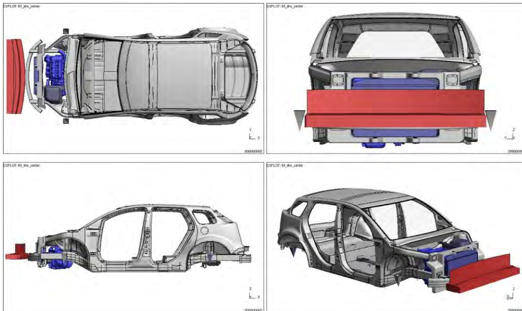
Figure 4.2.5.12.a: IIHS, low-speed, front test model setup ('full impact')
