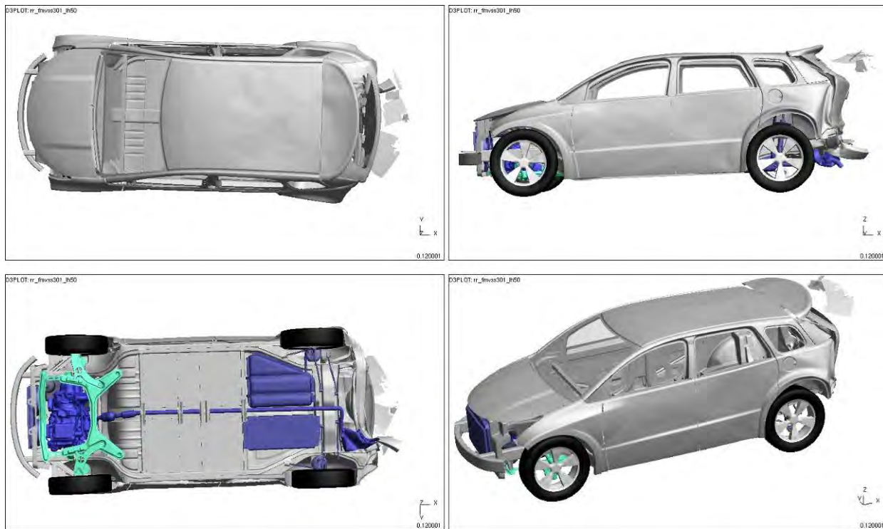
Figure 4.5.4.5.c: Vehicle Deformation (Barrier Blanked)
