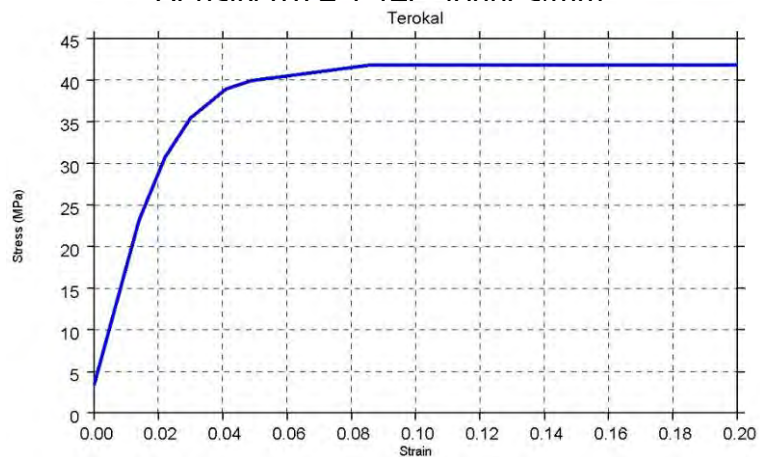
Figure 4.2.2.5.b: Terokal stress-strain curve
