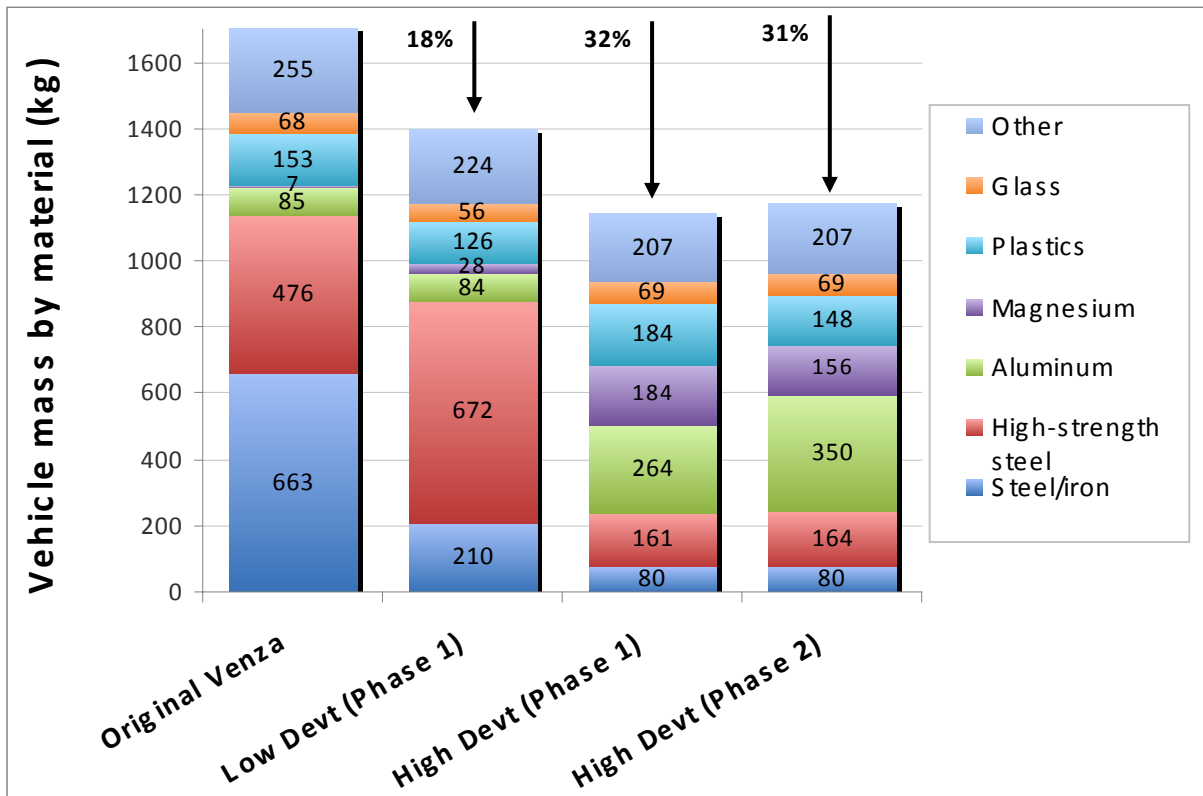
Figure 4.5.5.b: Venza, Phase 1, and Phase 2 full vehicle material composition
