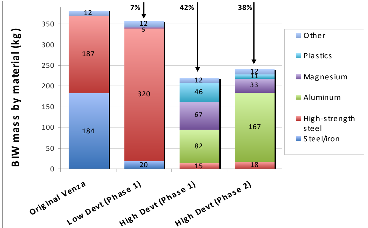
Figure 4.5.5.a: Venza, Phase 1, and Phase 2 vehicle body structure by material
