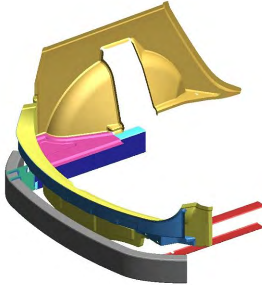
Figure 4.3.11.g: Main energy absorbing body structure for rear deformable barrier impact
