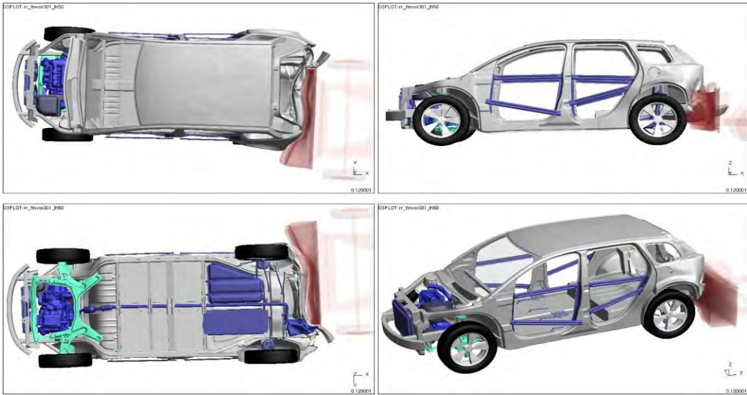
Figure 4.3.11.a: Vehicle deformation ( t=0.12 s) after rear deformable barrier impact
