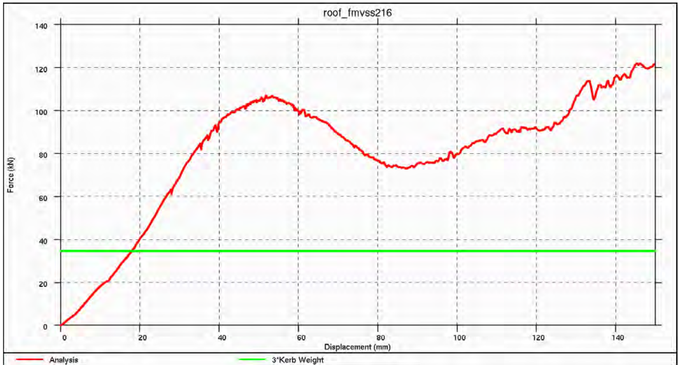
Figure 4.5.4.4.d: Roof Displacement vs. Applied Force – 3 times Curb Weight
