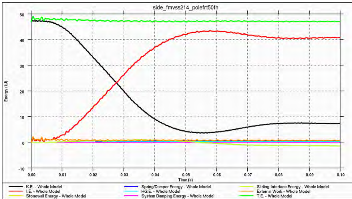
Figure 4.5.4.3.i: Energy Balance for 20-mph, 75-degree side-pole impact -- front (50 th percentile male)
