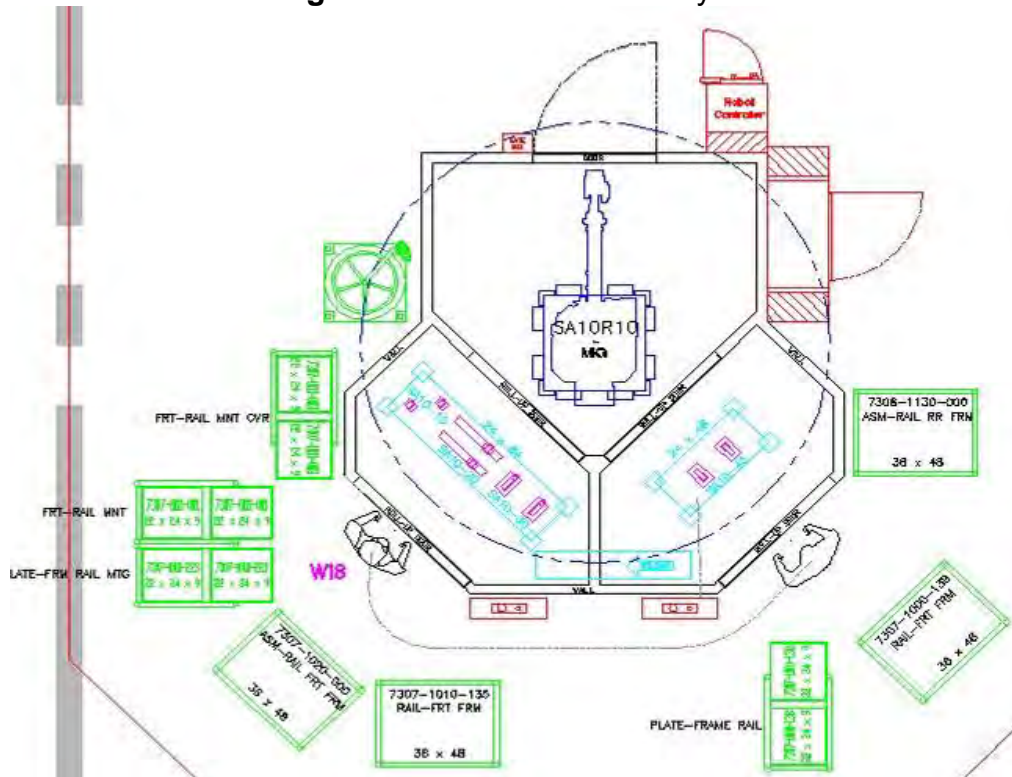
Figure 2.7.b: Station SA 10 layout
