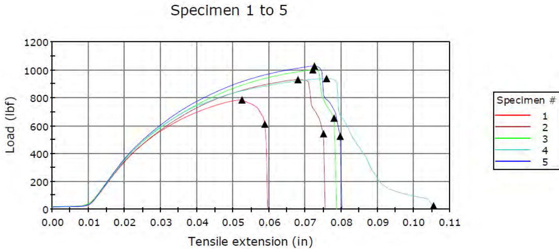
Figure 4.2.4.b: Henkel & Kawasaki lap-shear tests
