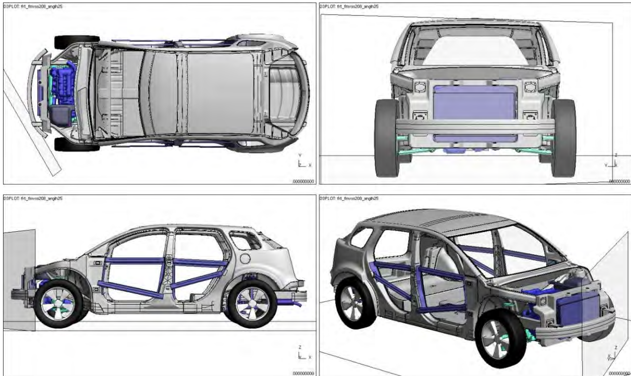
Figure 4.2.5.3.a: 30°, left-side barrier crash-test model setup
