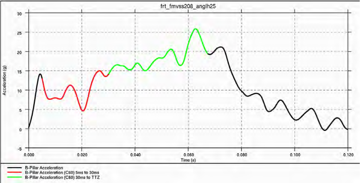
Figure 4.3.3.c: Average vehicle acceleration pulse during 30°, left-side frontal barrier impact
