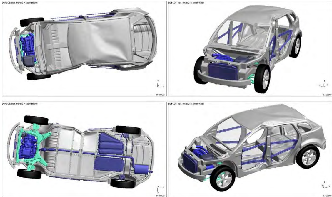
Figure 4.3.9.b: Vehicle deformation after 75°, side, pole impact (pole blanked) – 50 th percentile male
