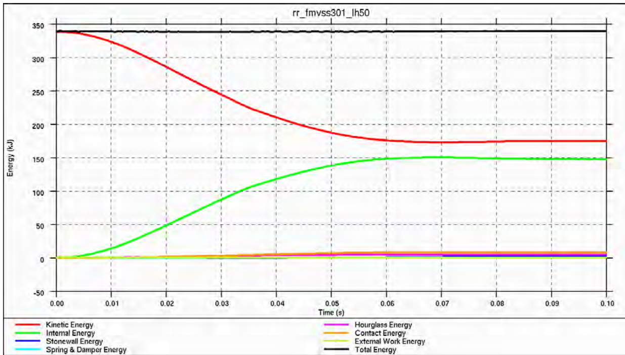
Figure 4.3.11.h: Energy balance for rear deformable barrier impact
