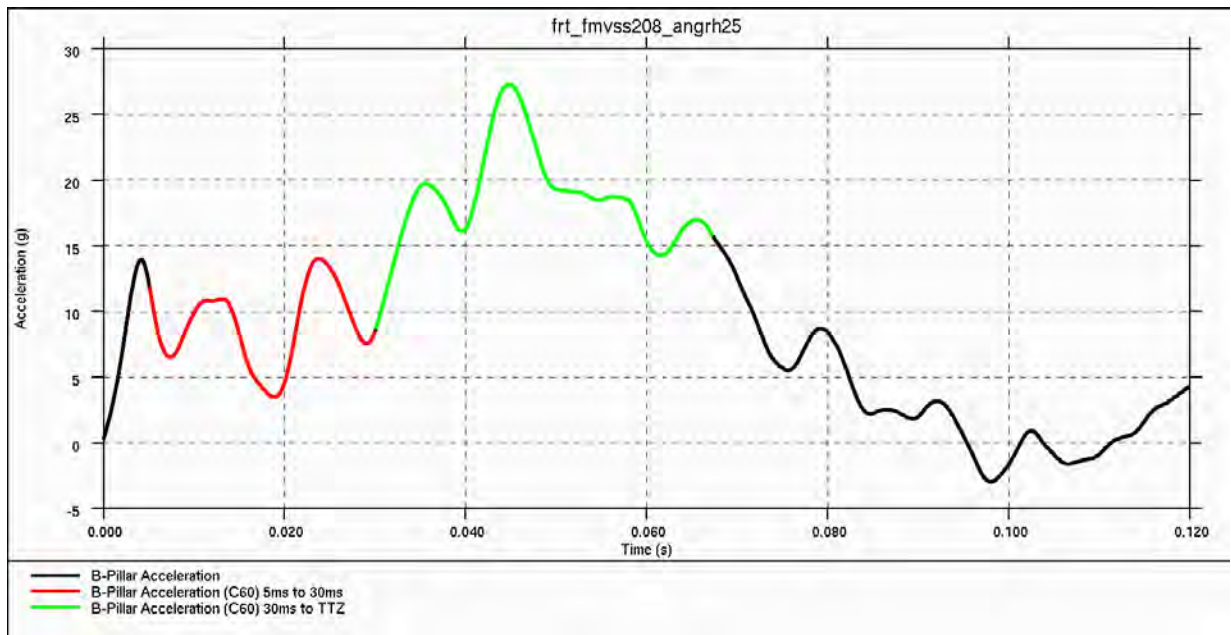
Figure 4.3.4.c: Vehicle average acceleration pulse during 30°, right-side frontal impact
