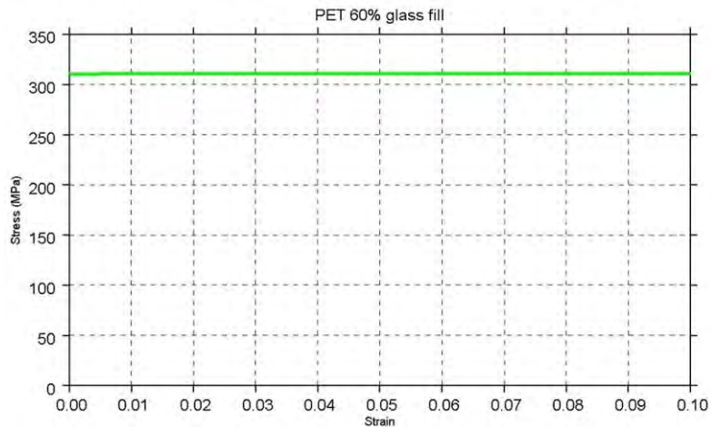
Figure 4.2.2.4.b: 60-percent glass-fiber PET stress-strain curve
