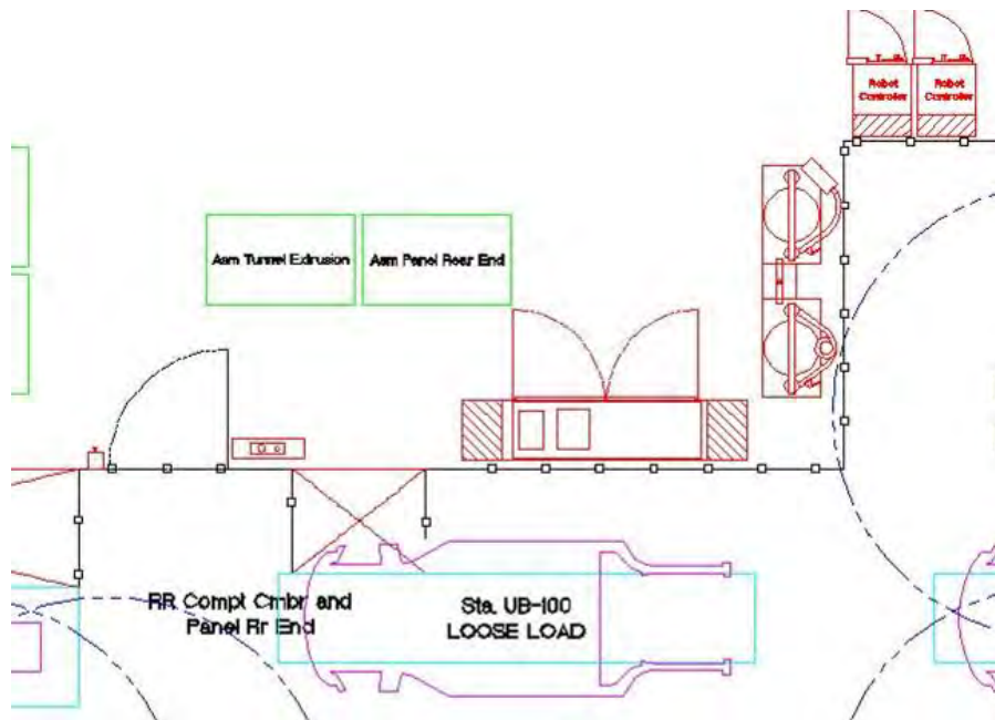
Figure 2.7.t: Station UB100 assembly layout
