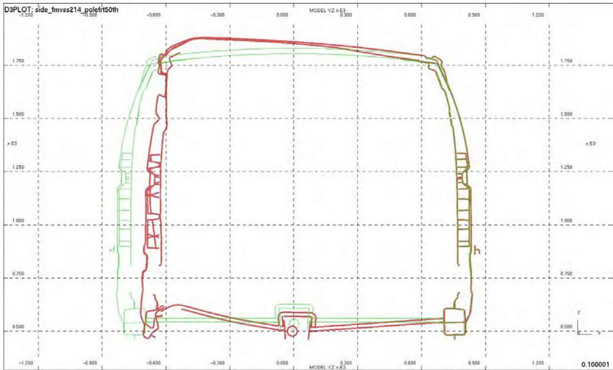
Figure 4.3.9.f: Section through B-pillar after 75°, side, pole impact, x=2842 - 50^{th} percentile male
