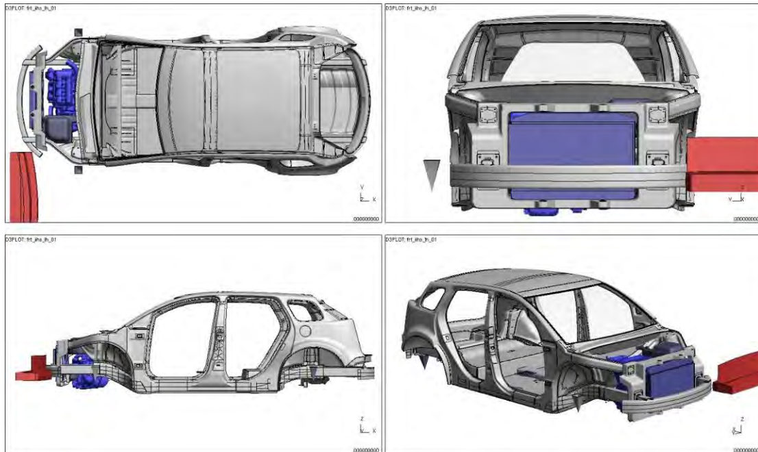
Figure 4.2.5.12.b: IIHS, low-speed front test model setup ('offset impact')
