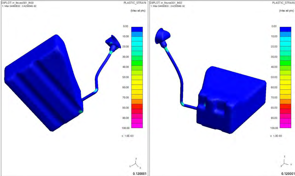
Figure 4.3.11.f: Fuel tank plastic strains after rear deformable barrier impact
