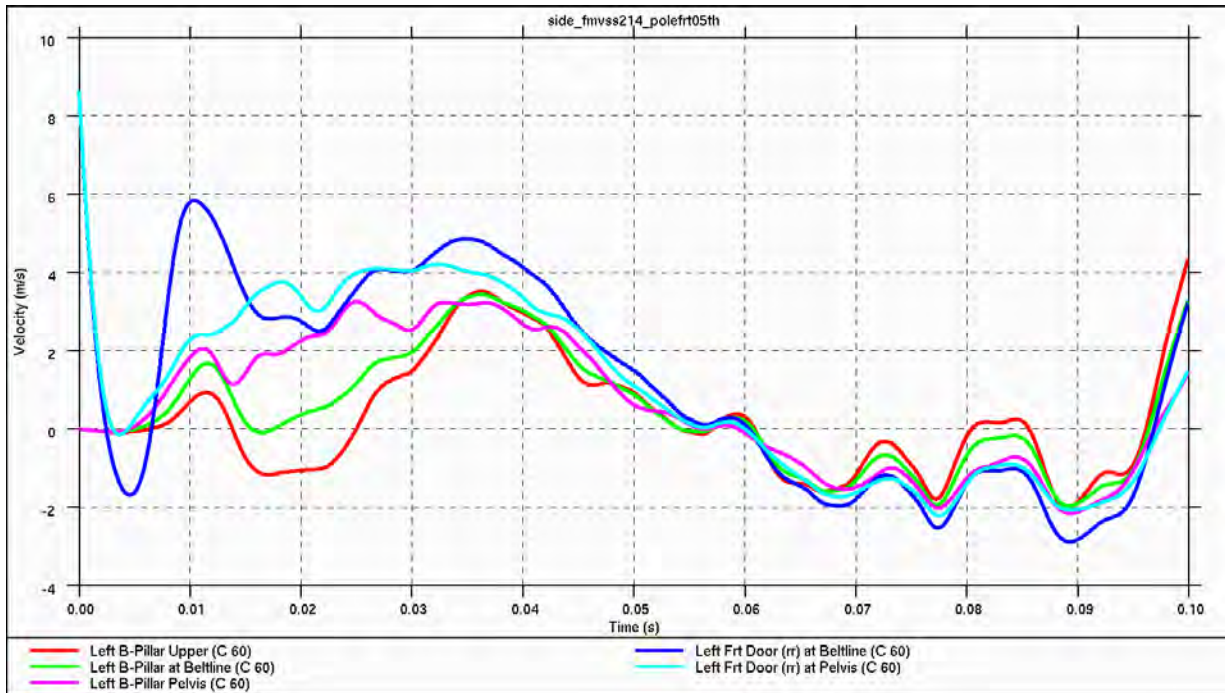
Figure 4.5.4.2.d: Intrusion Velocities (B-Pillar & Front Door)
