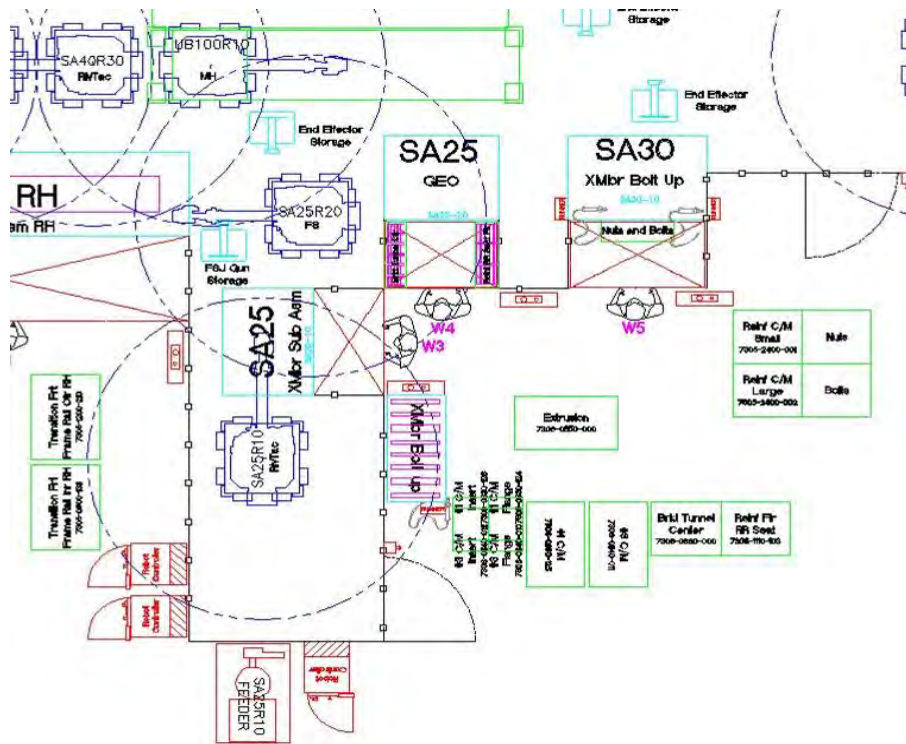
Figure 2.7.e: Stations SA25, SA30 layout
