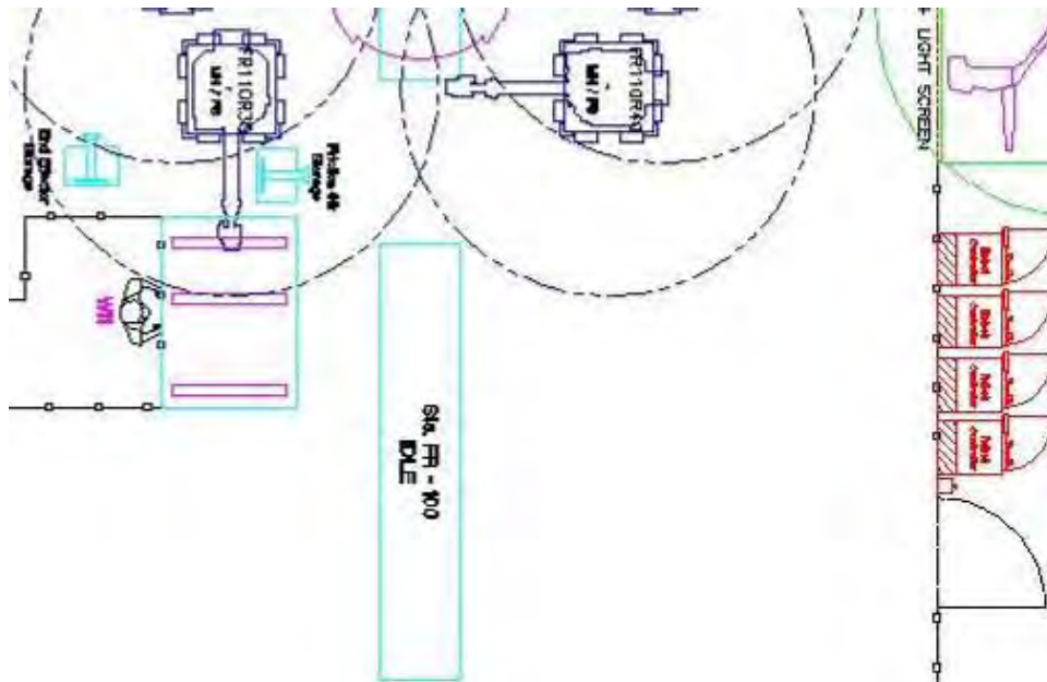
Figure 2.7.ai: Station FR100 assembly layout
