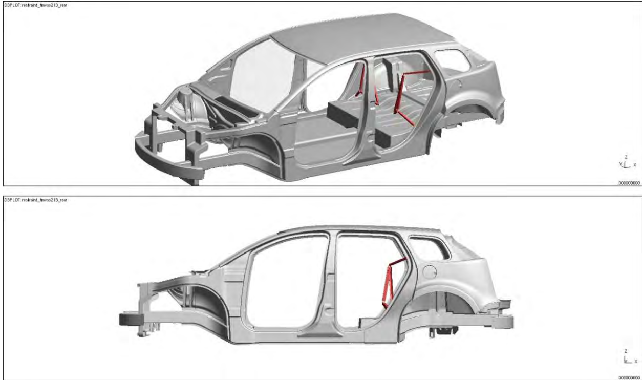
Figure 4.2.5.6.b: Child-restraint test model setup
