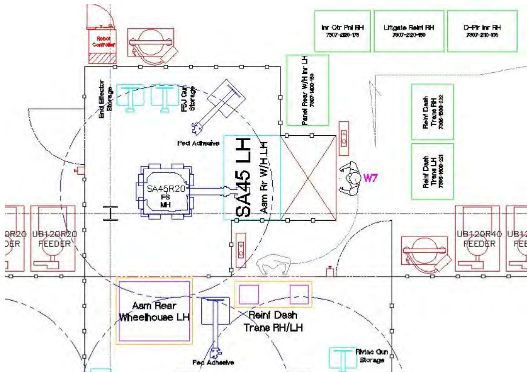
Figure 2.7.i: Station SA45, left-side assembly layout
