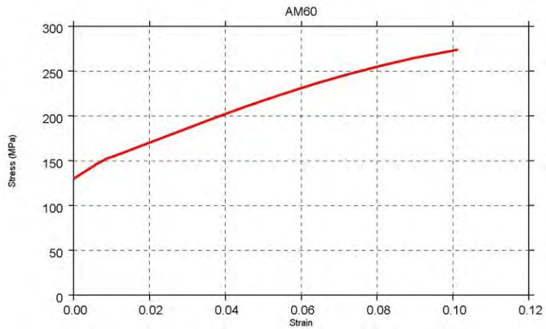
Figure 4.2.2.3.a: AM60 magnesium stress-strain curve
