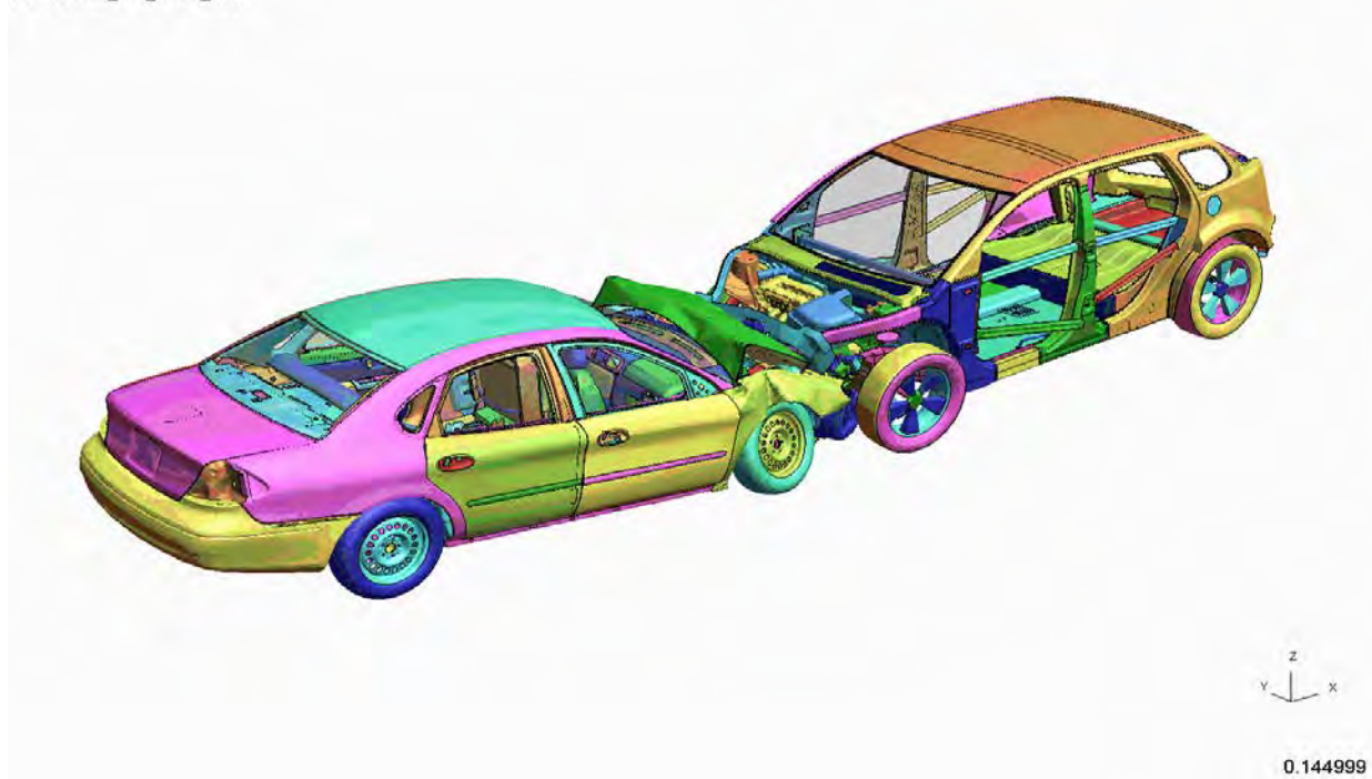
Figure 4.4.9.c: Phase 2 HD vehicle to Ford Taurus crash simulation result – three-quarter view
