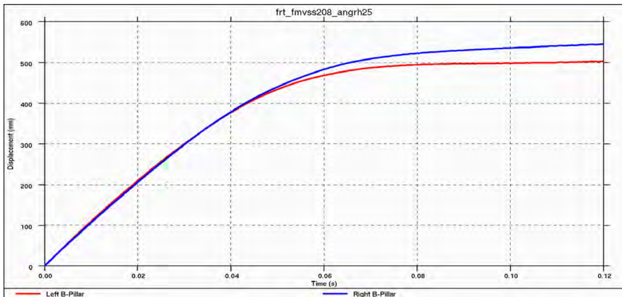
Figure 4.3.4.e: Vehicle displacement during 30°, right-side frontal impact - maximum dynamic crush 524 mm
