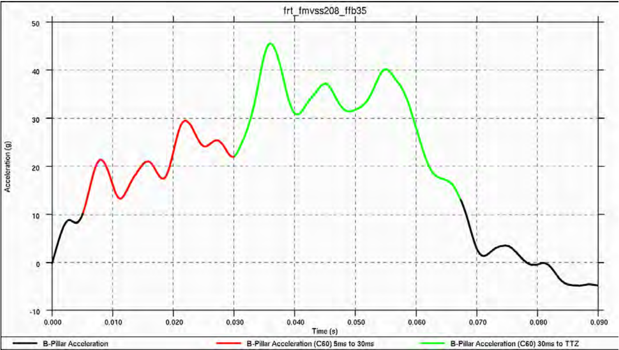
Figure 4.3.1.c: Average vehicle acceleration pulse during frontal impact
