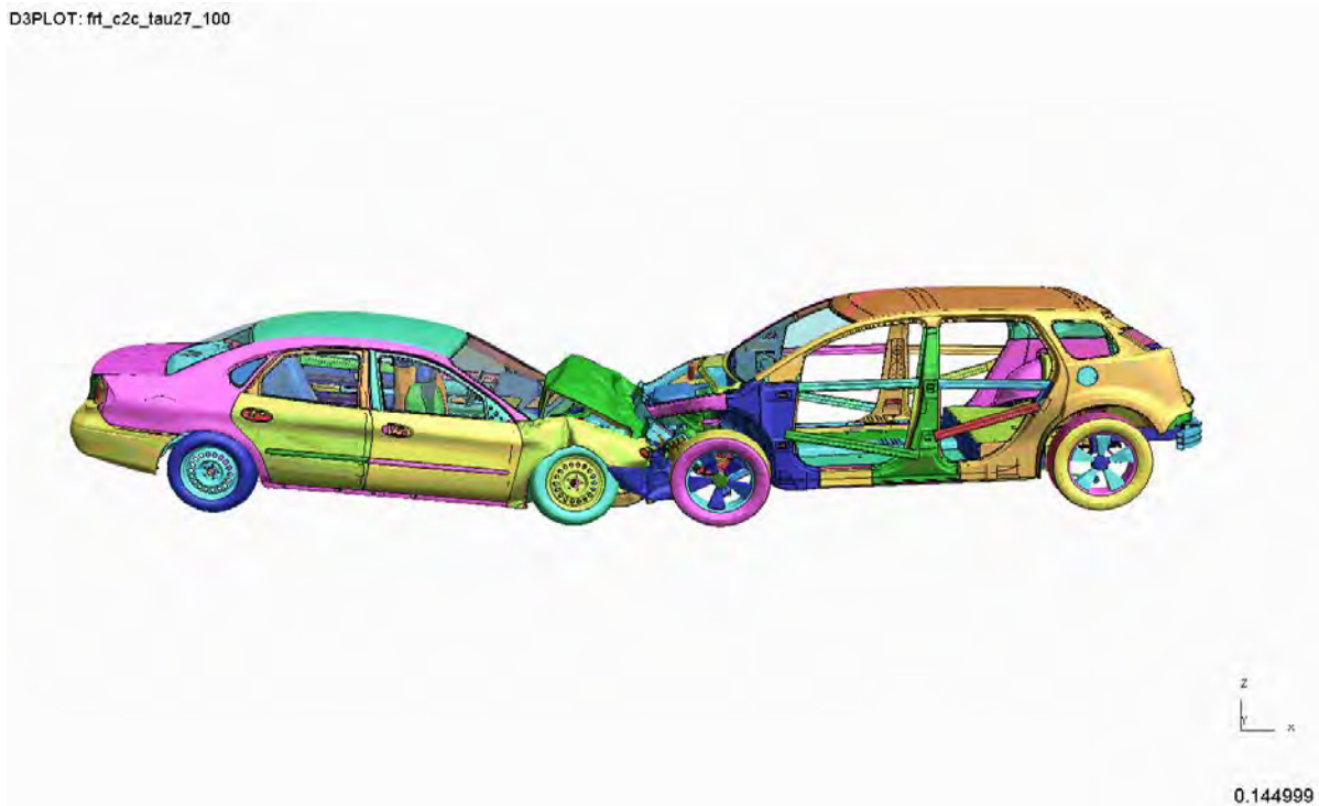
Figure 4.4.9.d: Phase 2 HD vehicle to Ford Taurus crash simulation result – side view
