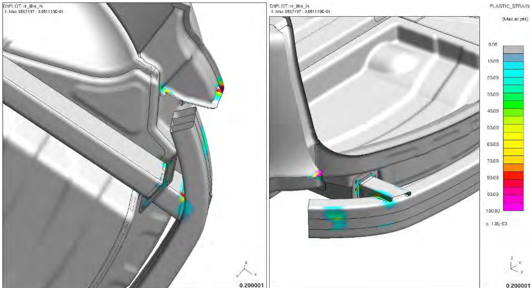
Figure 4.3.13.b: Rear plastic strains after low-speed rear impact ('offset impact')
