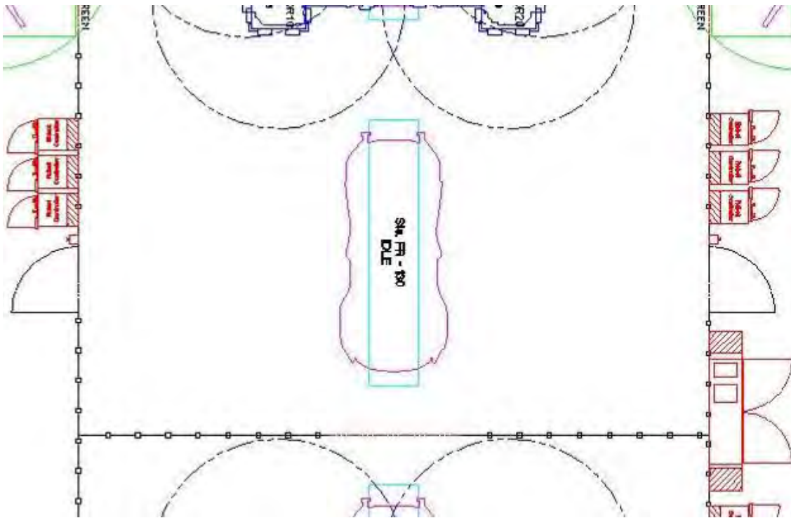
Figure 2.7.aI: Station FR130 assembly layout
