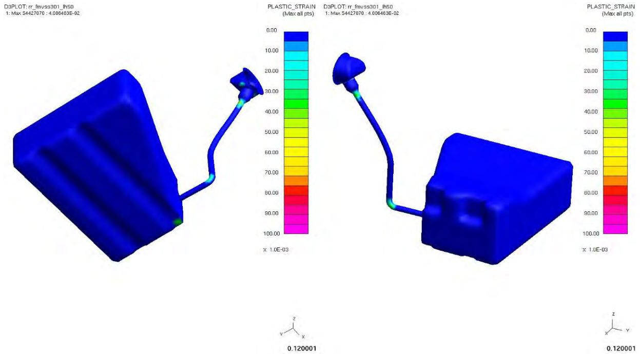
Figure 4.5.4.5.g: Fuel Tank Plastic Strains after rear impact
