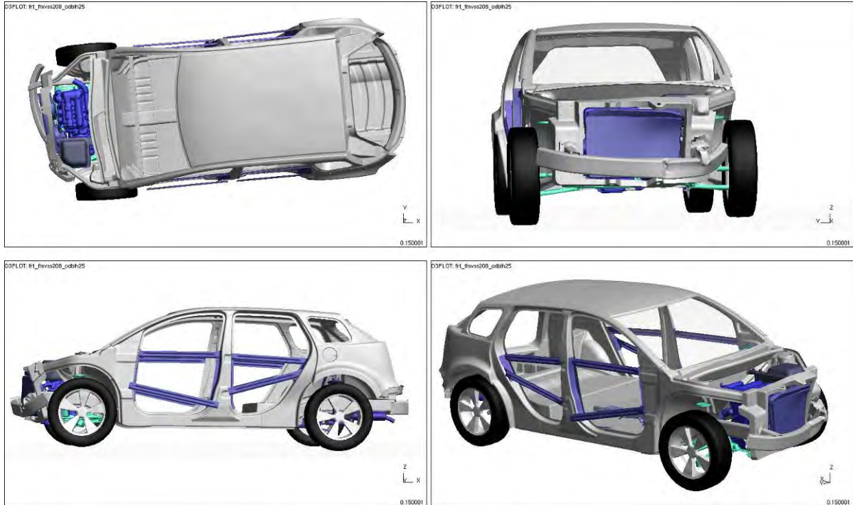
Figure 4.3.2.b: Vehicle deformation ( t=0.15 s, barrier not shown) after 40-percent overlap frontal impact
