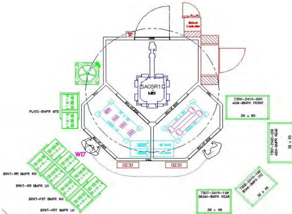
Figure 2.7.a: Station SA05 layout
