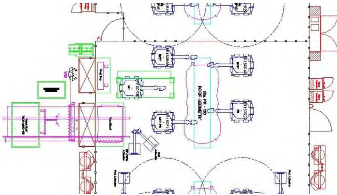
Figure 2.7.an: Station FR150 assembly layout
