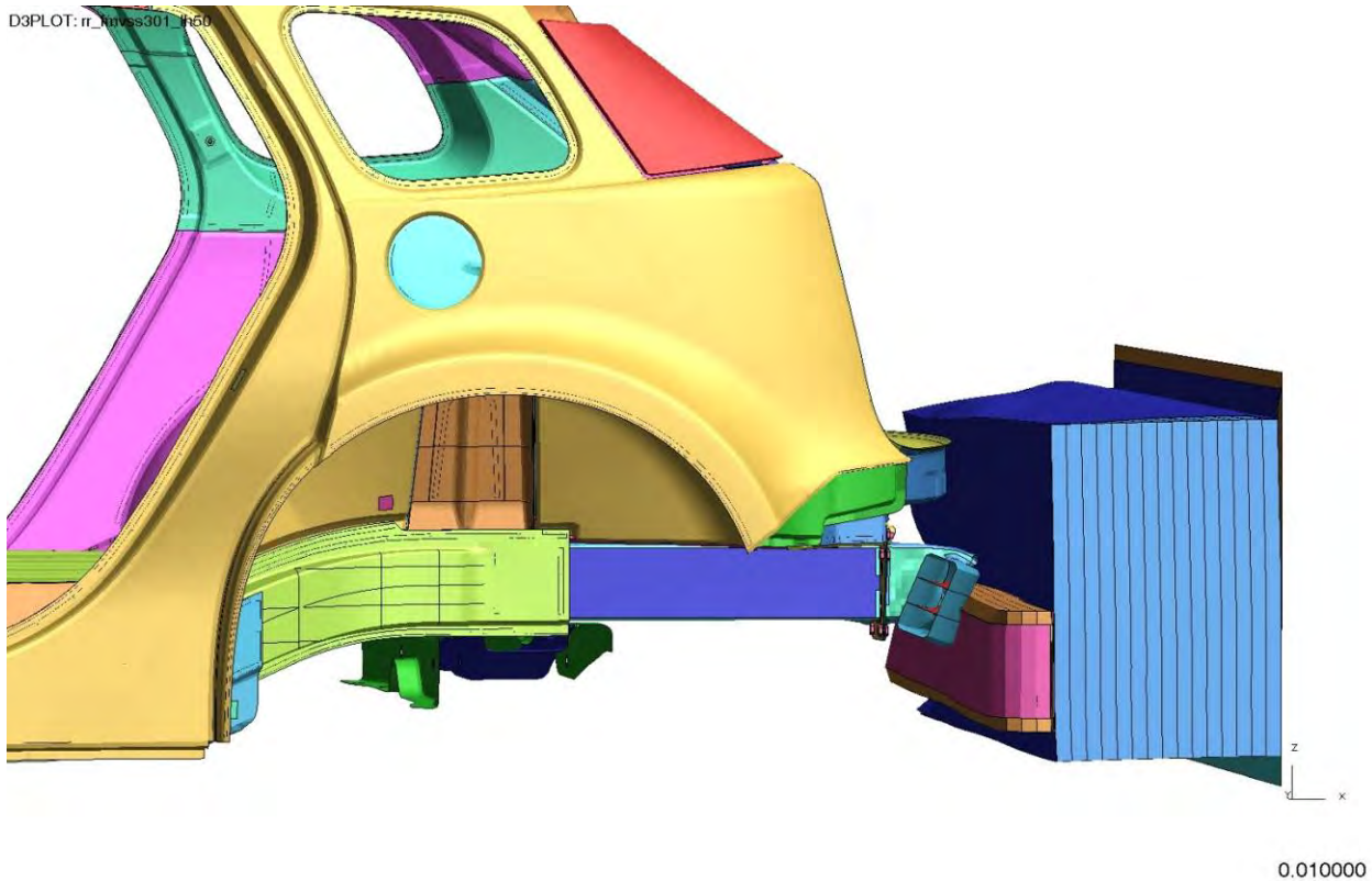
Figure 4.5.4.5.1.b: Initial vehicle armature rotation during rear impact
