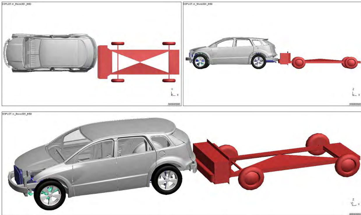
Figure 4.5.4.5.a: Rear Impact Model Set up
