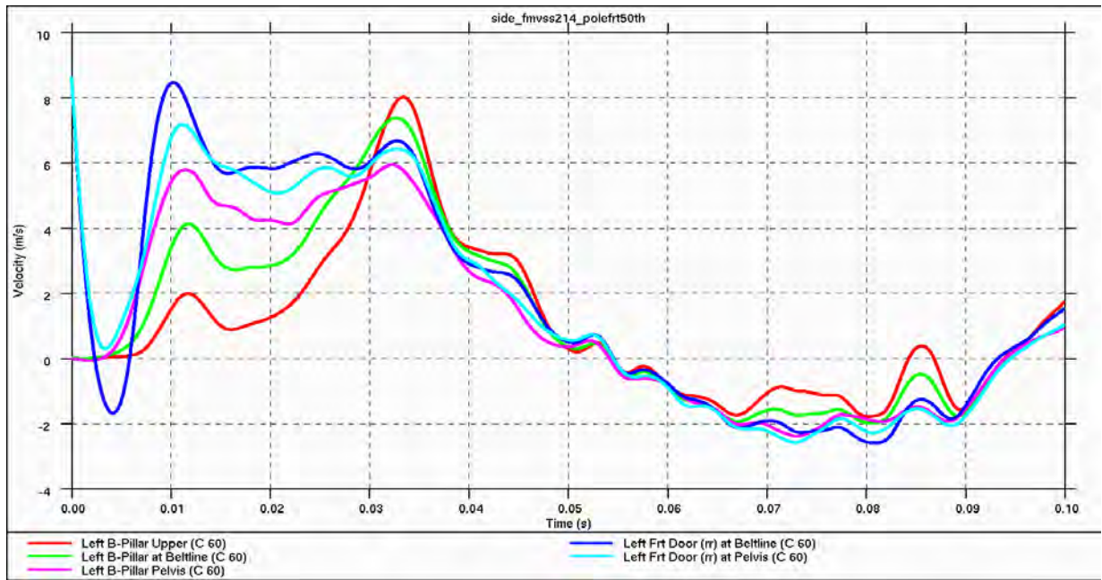
Figure 4.5.4.3.d: Intrusion Velocities (B-Pillar & Front Door) after 20-mph, 75-degree side-pole impact -- front (50 th percentile male)
