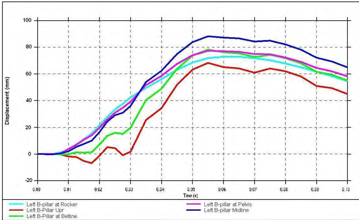
Figure 4.3.9.d: Relative intrusion displacements during 75°, side, pole impact (B-pillar) – 50 th percentile male
