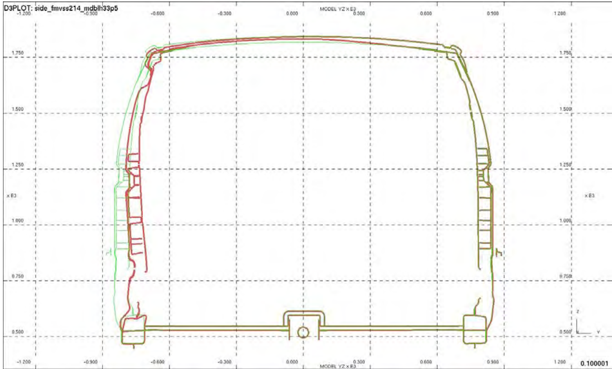
Figure 4.3.7.f: B-pillar intrusion profile after crabbed barrier impact, x=2842
