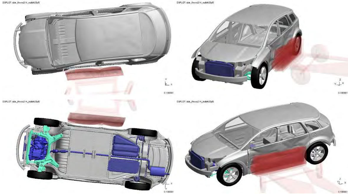
Figure 4.5.4.1.b: Vehicle Deformation (0.1s)
