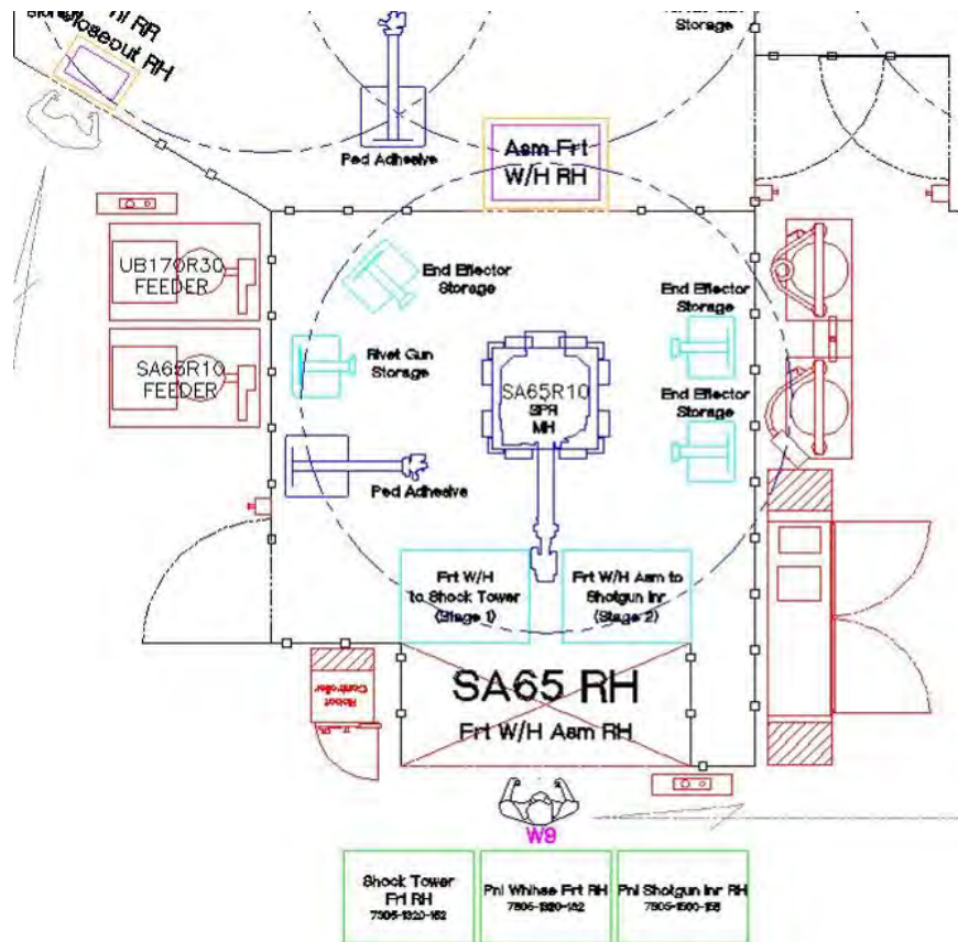
Figure 2.7.I: Station SA65, right-side assembly layout
