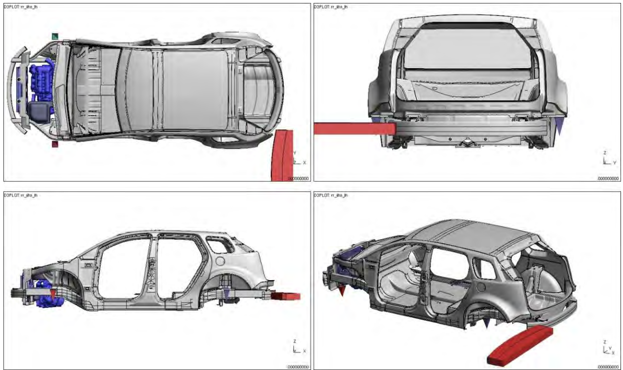
Figure 4.2.5.13.b: IIHS, low-speed rear test model setup ('offset impact')
