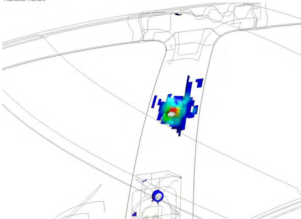
Figure 4.3.5.1.b: Upper seatbelt anchorage plastic strain (@ 0.2 s)
