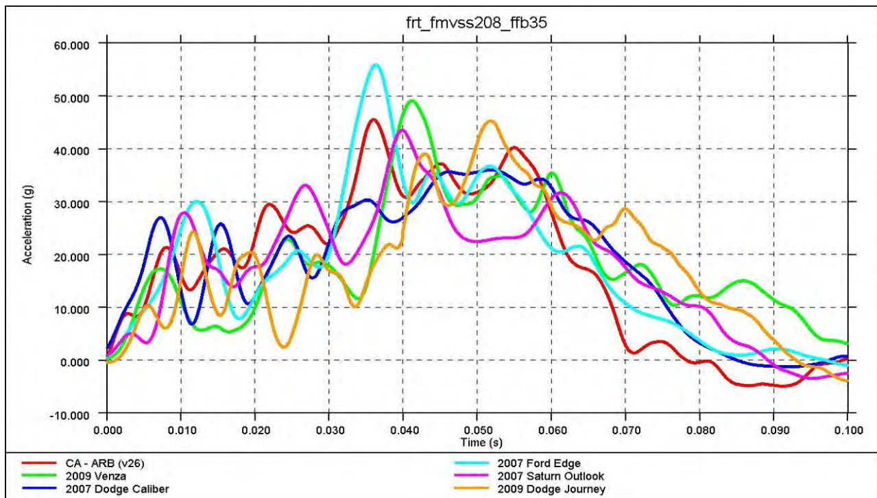
Figure 4.3.2.k: Comparison of production vehicle and Phase 2 HD crash accelerations
