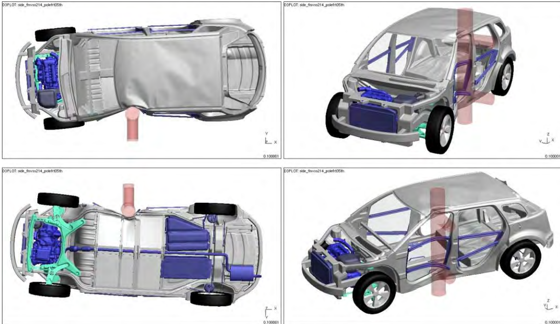
Figure 4.3.8.a: Vehicle deformation (0.1 s) after 75°, side, pole impact – 5 th percentile female
