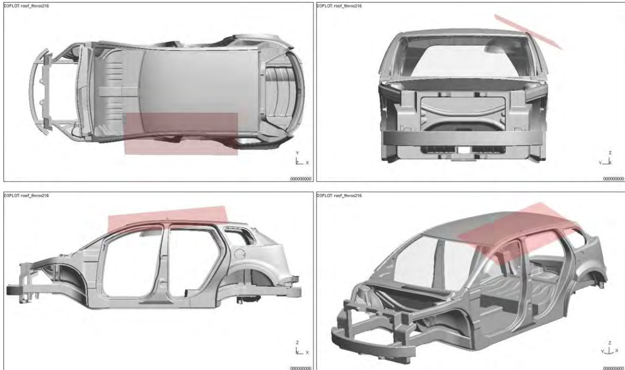
Figure 4.2.5.10.a: Roof crush test model setup
