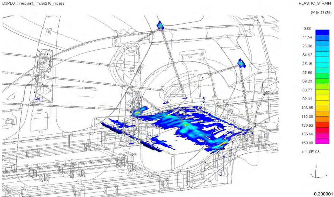
Figure 4.3.5.2.a: Rear seatbelt anchorage plastic strain (@ 0.2 s)
