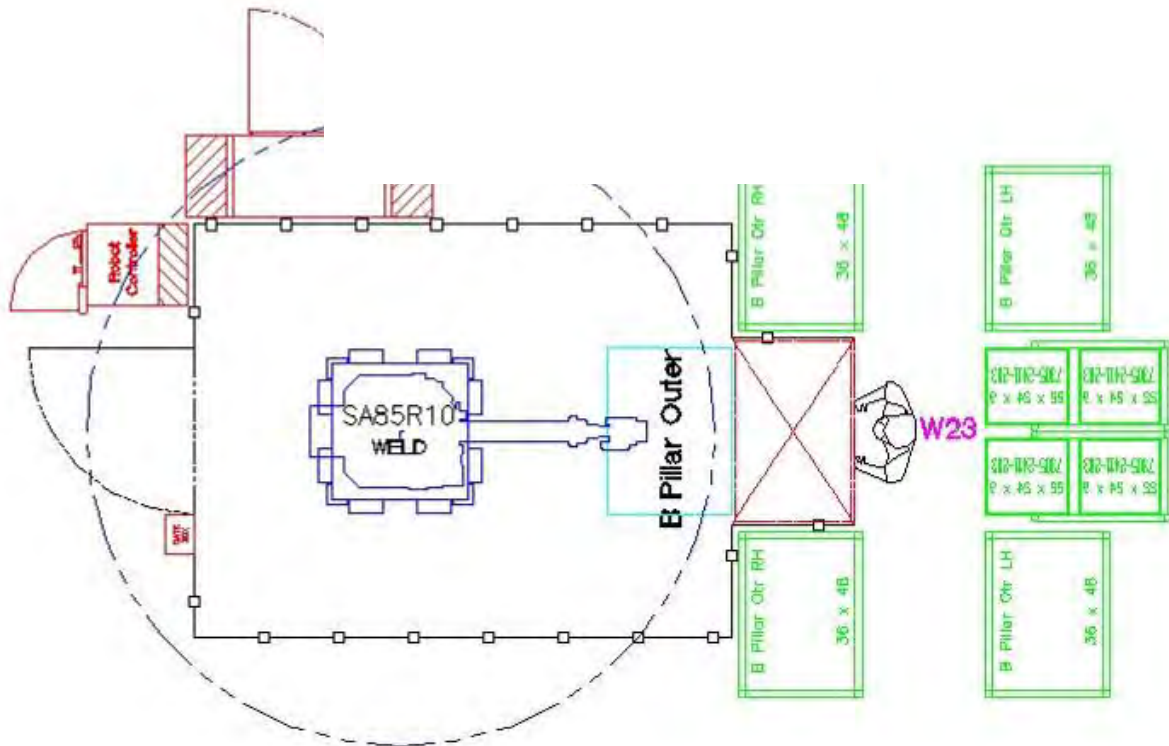
Figure 2.7.s: Station SA85 assembly layout
