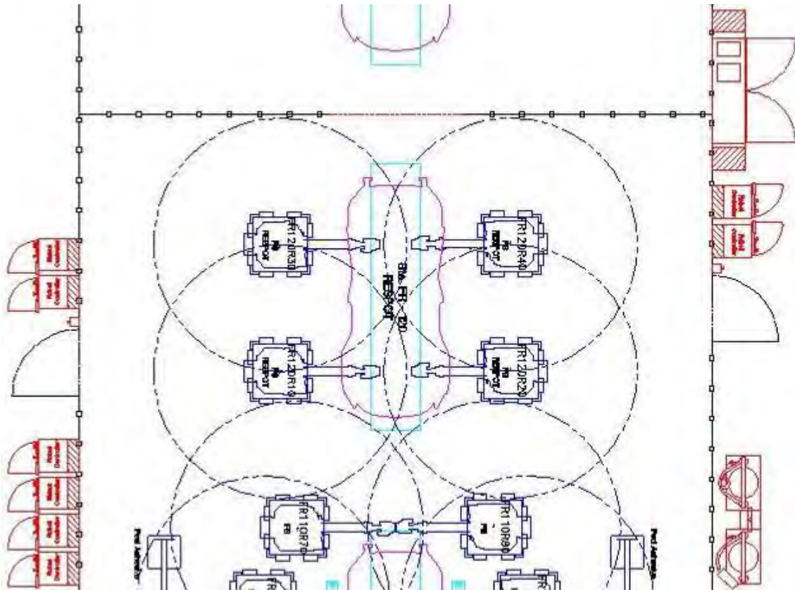
Figure 2.7.ak: Station FR120 assembly layout
