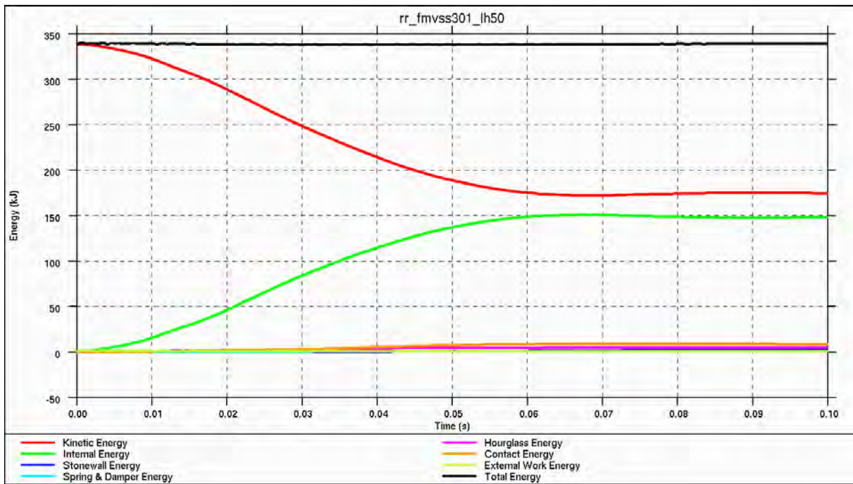
Figure 4.5.4.5.h: Rear impact energy balance
