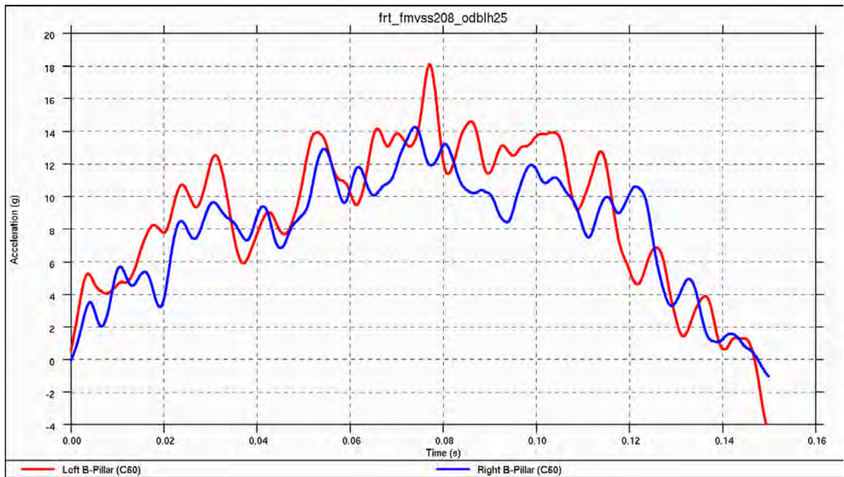
Figure 4.3.2.c: Vehicle acceleration pulse during 40-percent overlap frontal impact
