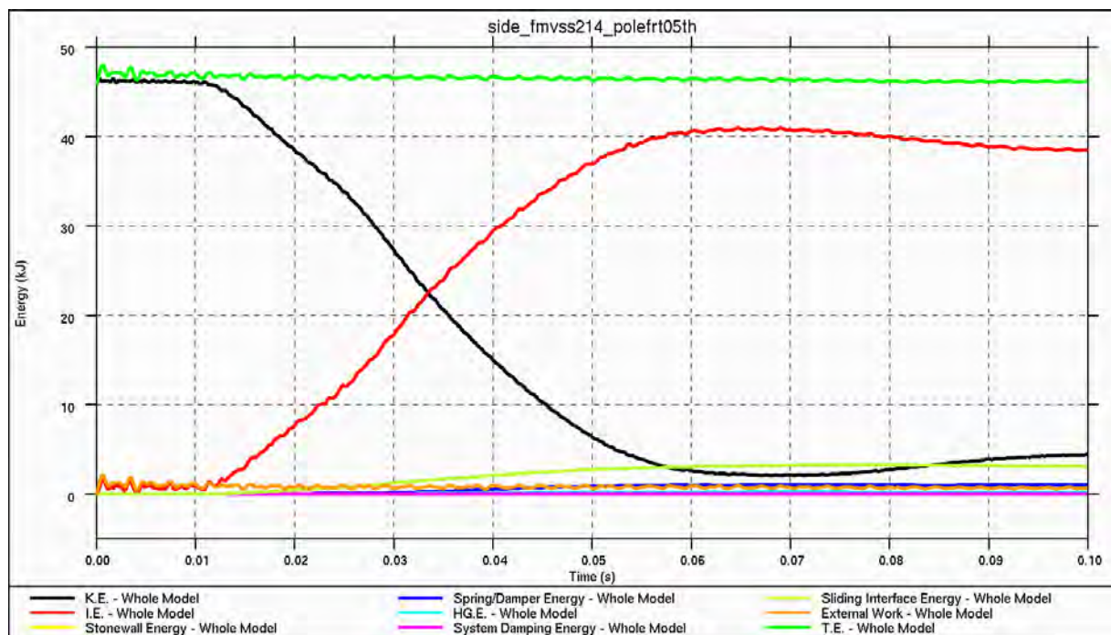
Figure 4.3.8.h: Energy balance for 75°, side, pole impact – 5 th percentile female
