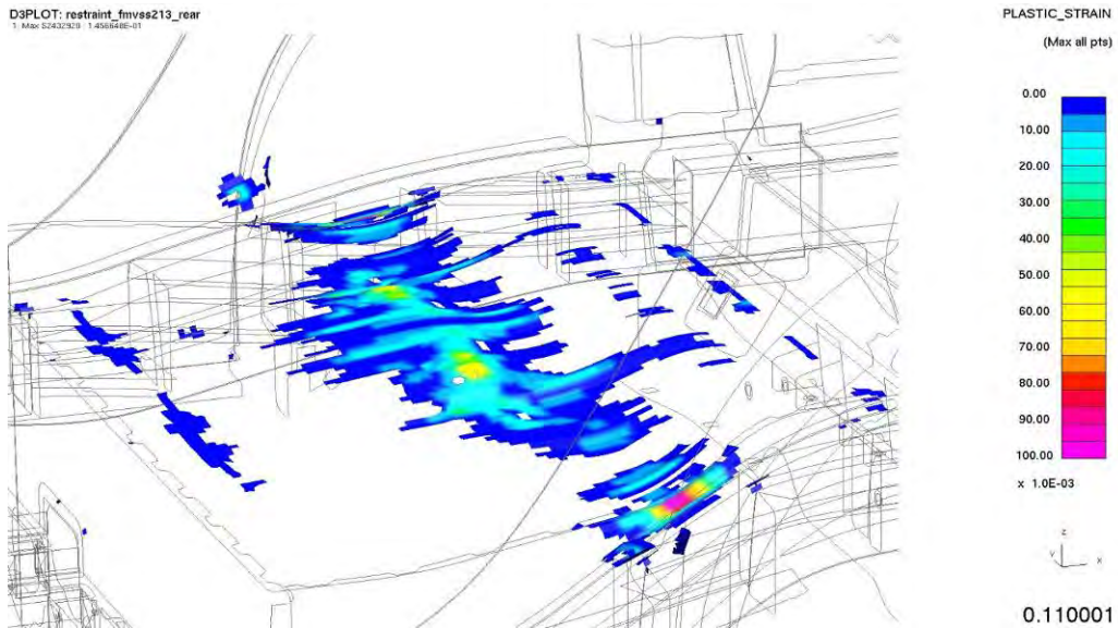
Figure 4.3.6.a: Child-restraint, lower anchorage plastic strain
