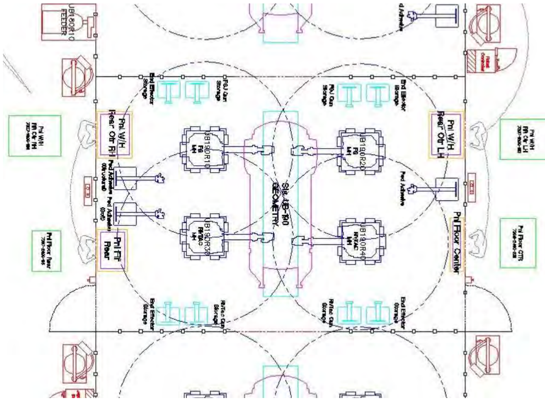
Figure 2.7.ac: Station UB190 assembly layout
