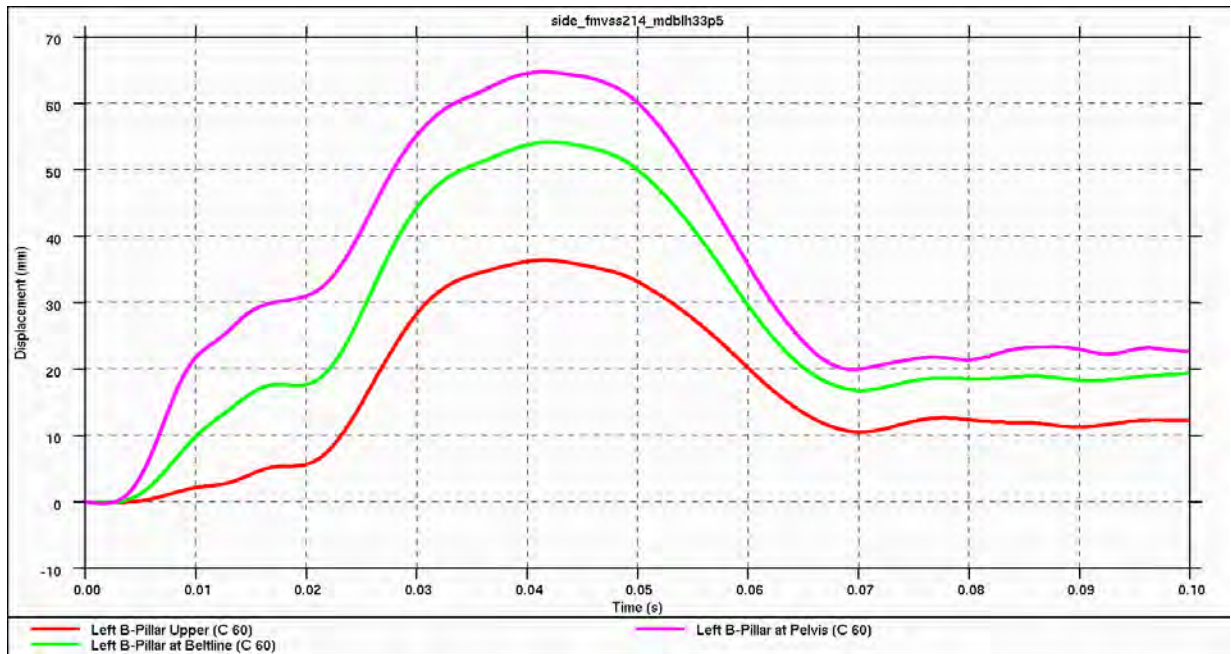
Figure 4.5.4.1.f: Relative Intrusion Displacements (B-pillar)
