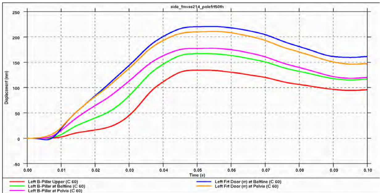
Figure 4.5.4.3.e: Intrusion Displacements (B-Pillar & Front Door) after 20-mph, 75-degree side-pole impact -- front (50 th percentile male)
