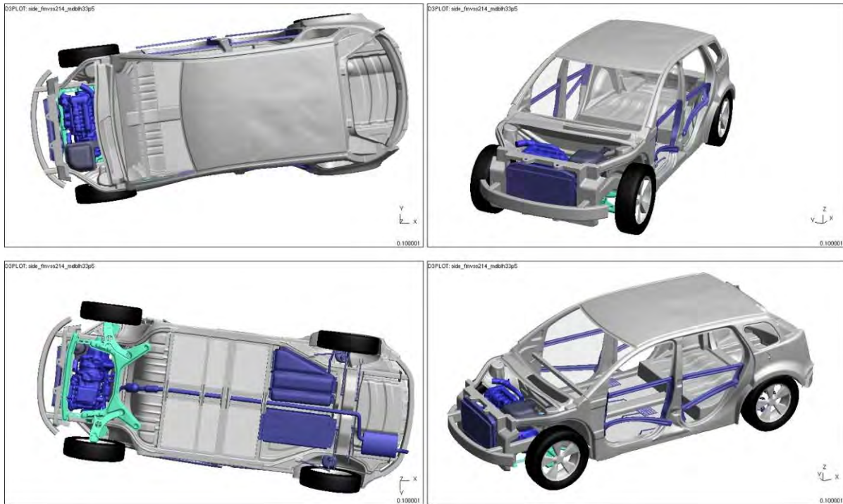
Figure 4.3.7.b: Vehicle deformation (barrier not shown) after crabbed barrier impact
