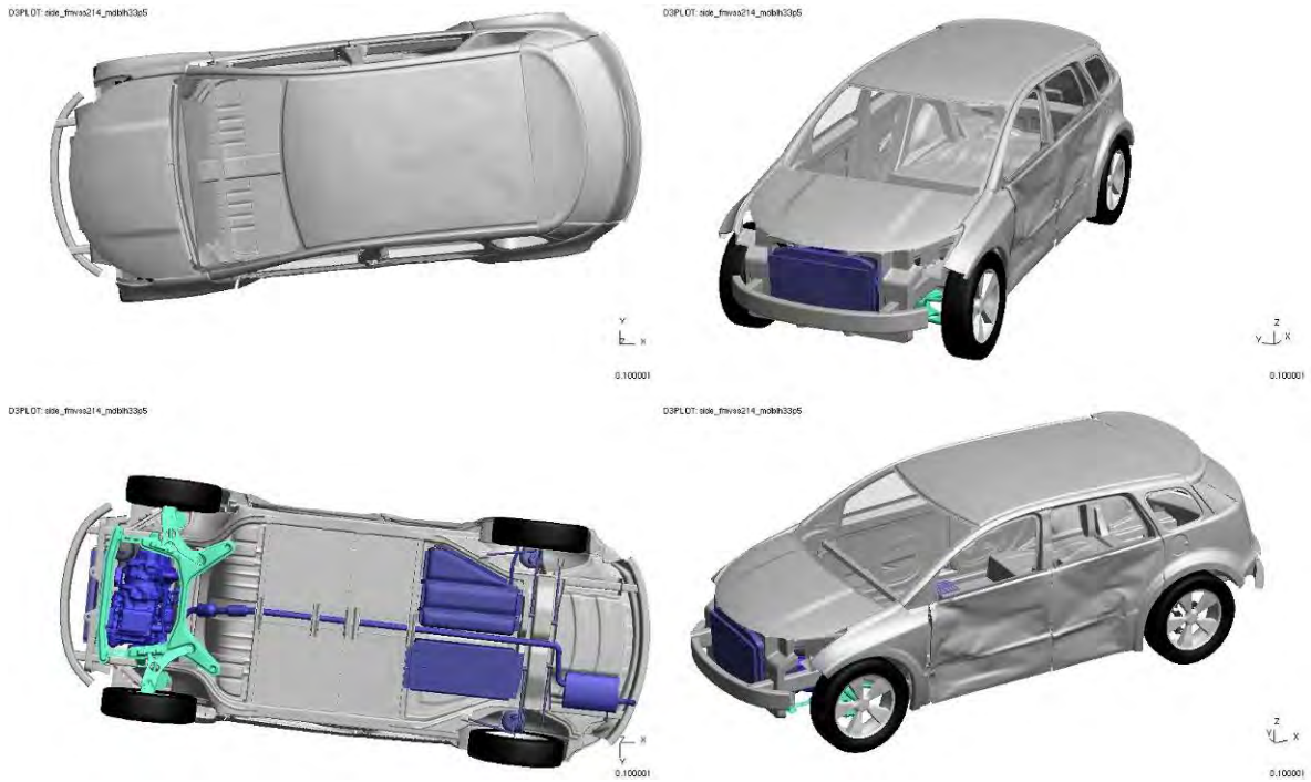
Figure 4.5.4.1.c: Vehicle Deformation (barrier not shown)
