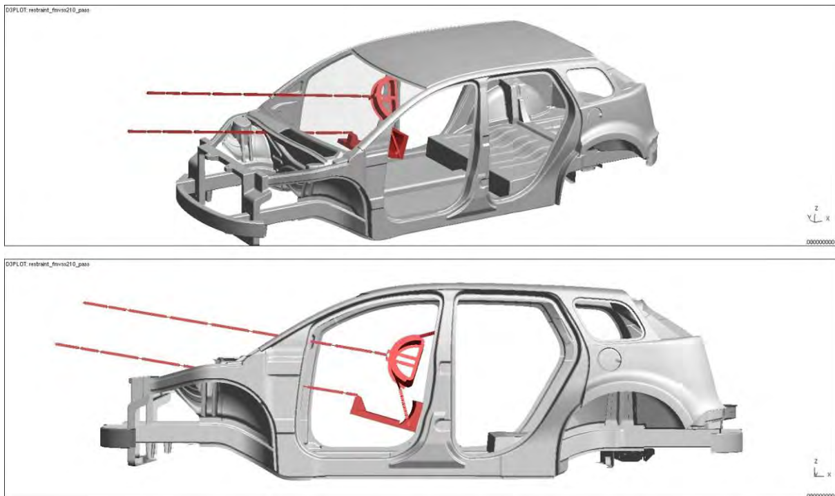
Figure 4.2.5.5.a: Front seatbelt anchorage test model setup
