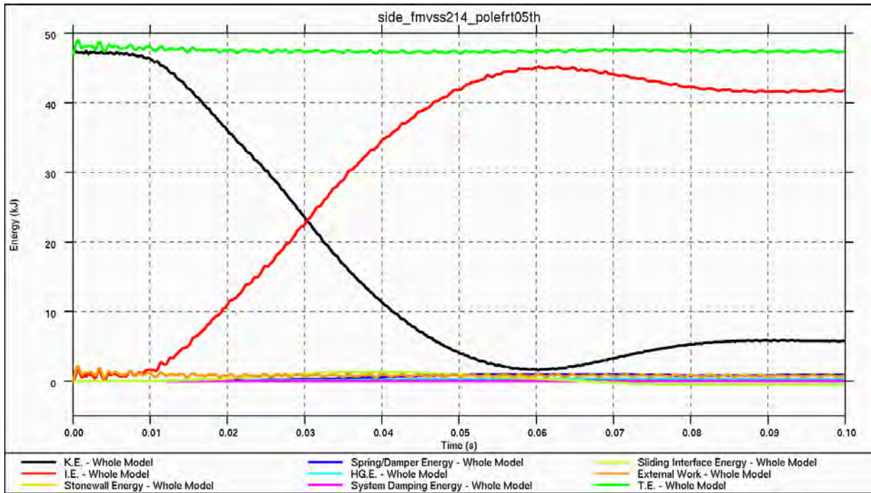
Figure 4.5.4.2.h: Energy Balance
