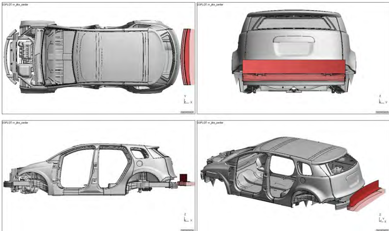
Figure 4.5.4.6.a: Low-speed IIHS impact model setup ('full')
