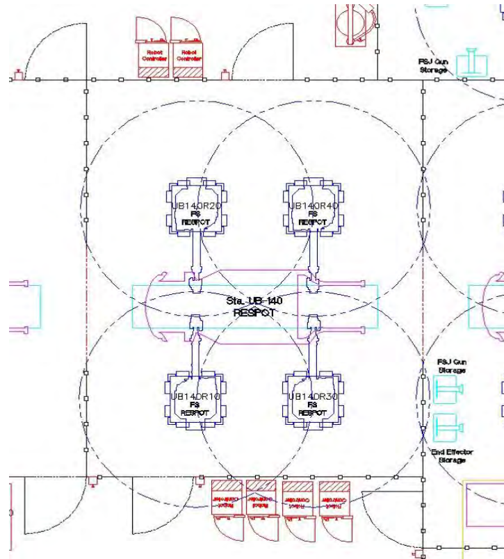
Figure 2.7.x: Station UB140 assembly layout
