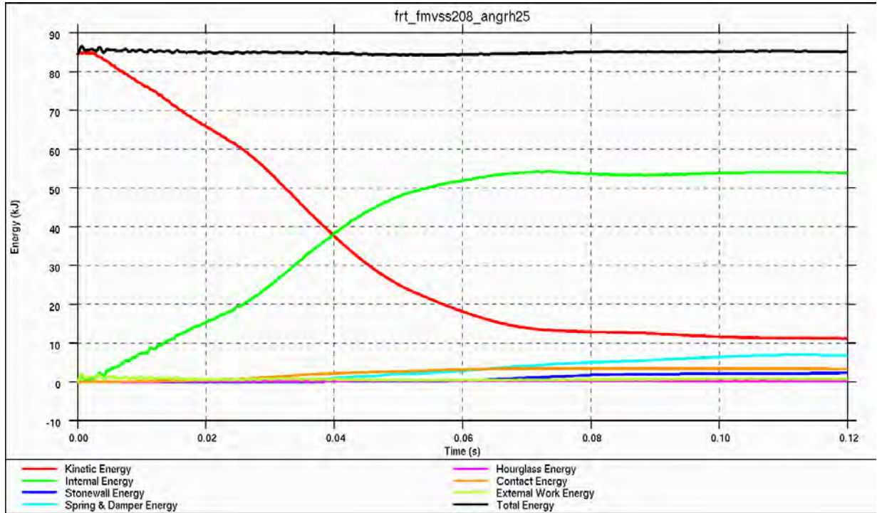
Figure 4.3.4.i: Energy balance for 30°, right-side frontal impact
