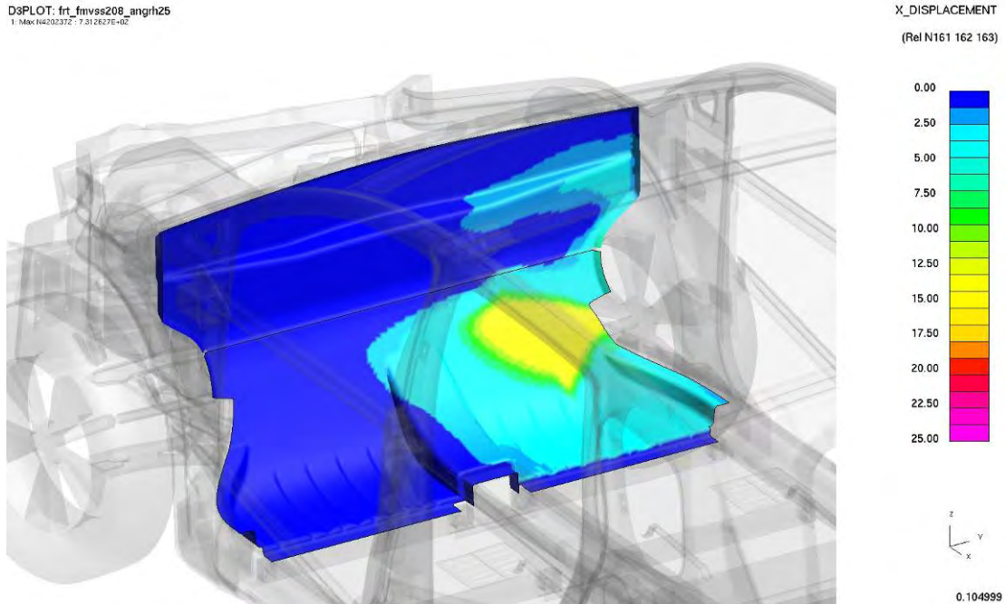
Figure 4.3.4.f: CAE dash intrusion analysis after 30°, right-side frontal impact
