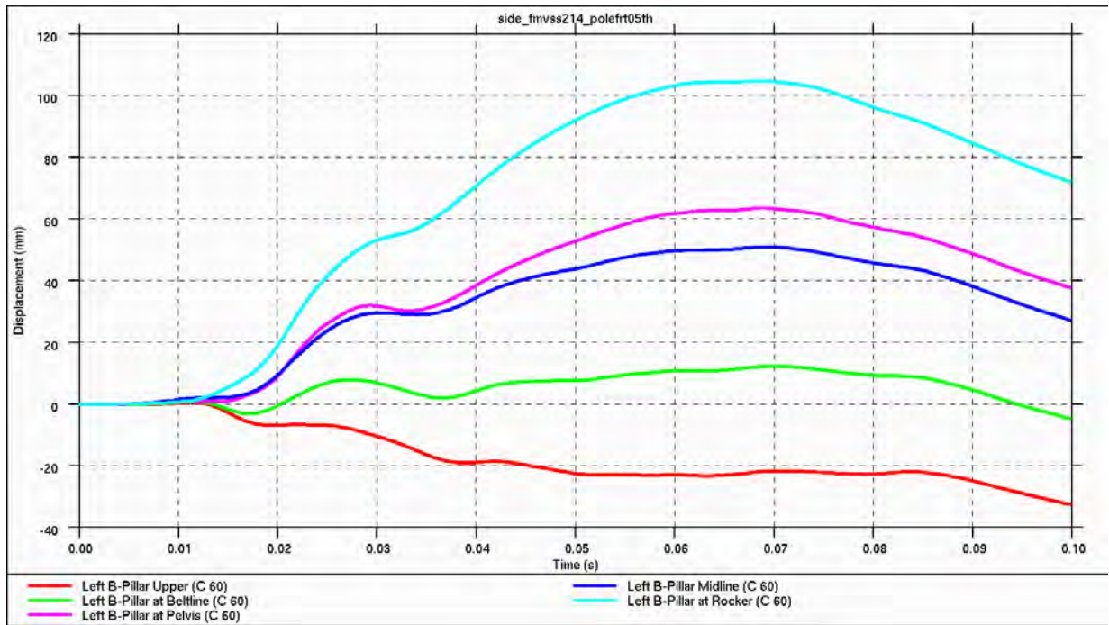
Figure 4.3.8.d: Relative intrusion displacements during 75°, side, pole impact (B-pillar) – 5 th percentile female
