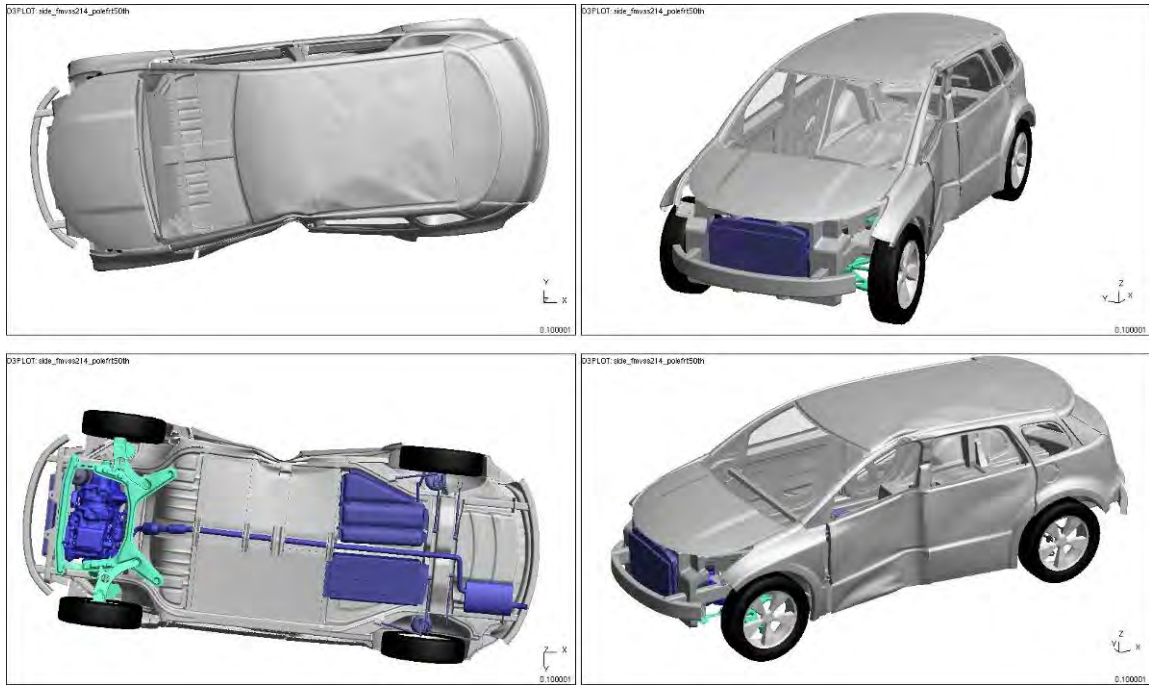
Figure 4.5.4.3.c: Vehicle Deformation (Pole Blanked)
