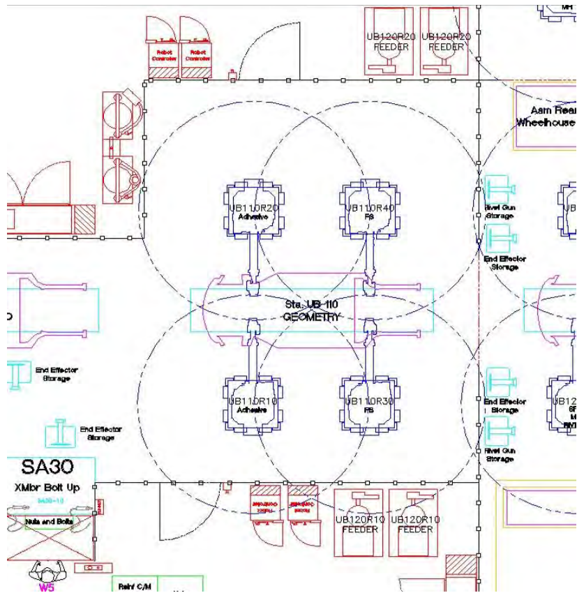
Figure 2.7.u: Station UB110 assembly layout
