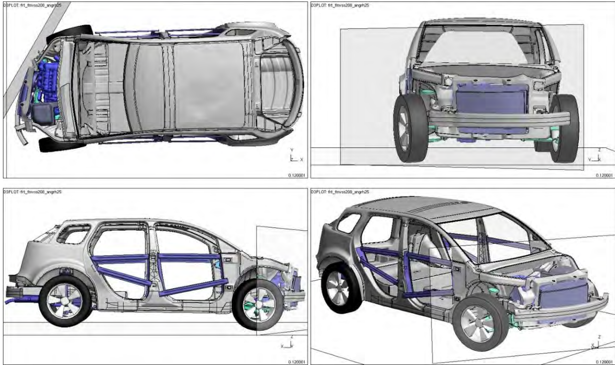
Figure 4.3.4.a: Vehicle deformation (t=0.12 s) after 30°, right-side frontal impact
