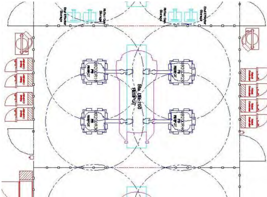
Figure 2.7.ad: Station UB200 assembly layout
