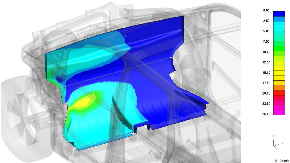
Figure 4.3.3.f: CAE dash intrusion analysis after 30°, left-side frontal impact
