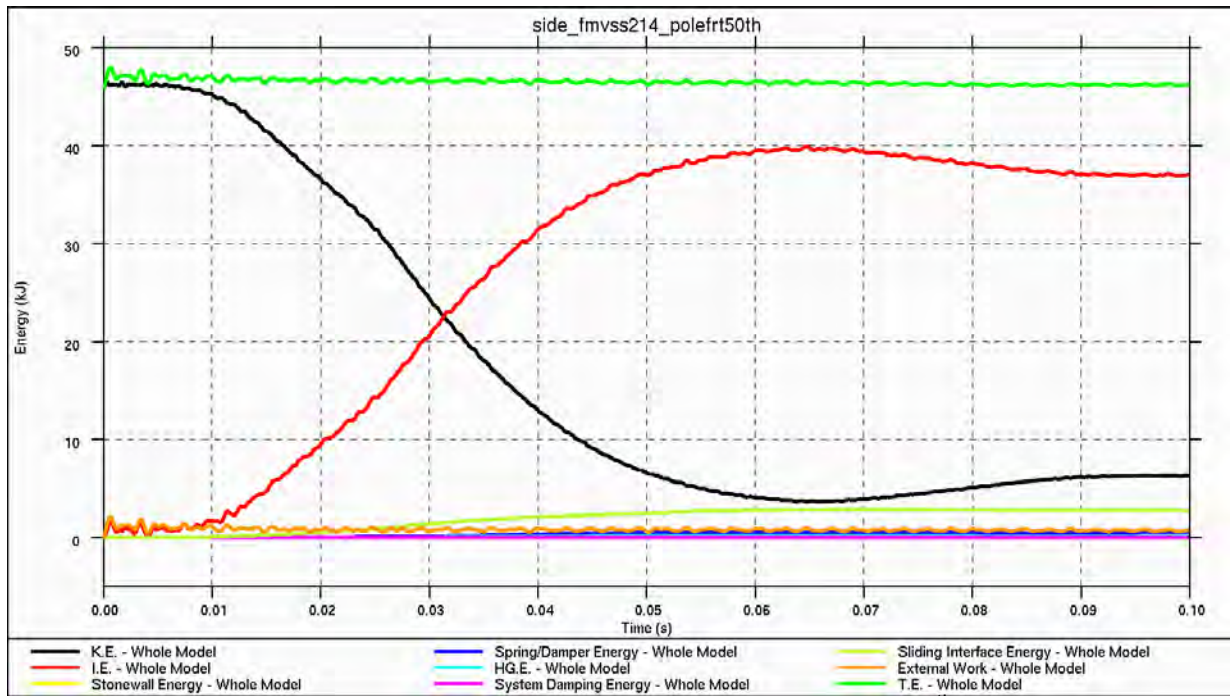
Figure 4.3.9.h: Energy balance for 75°, side, pole impact – 50 th percentile male
