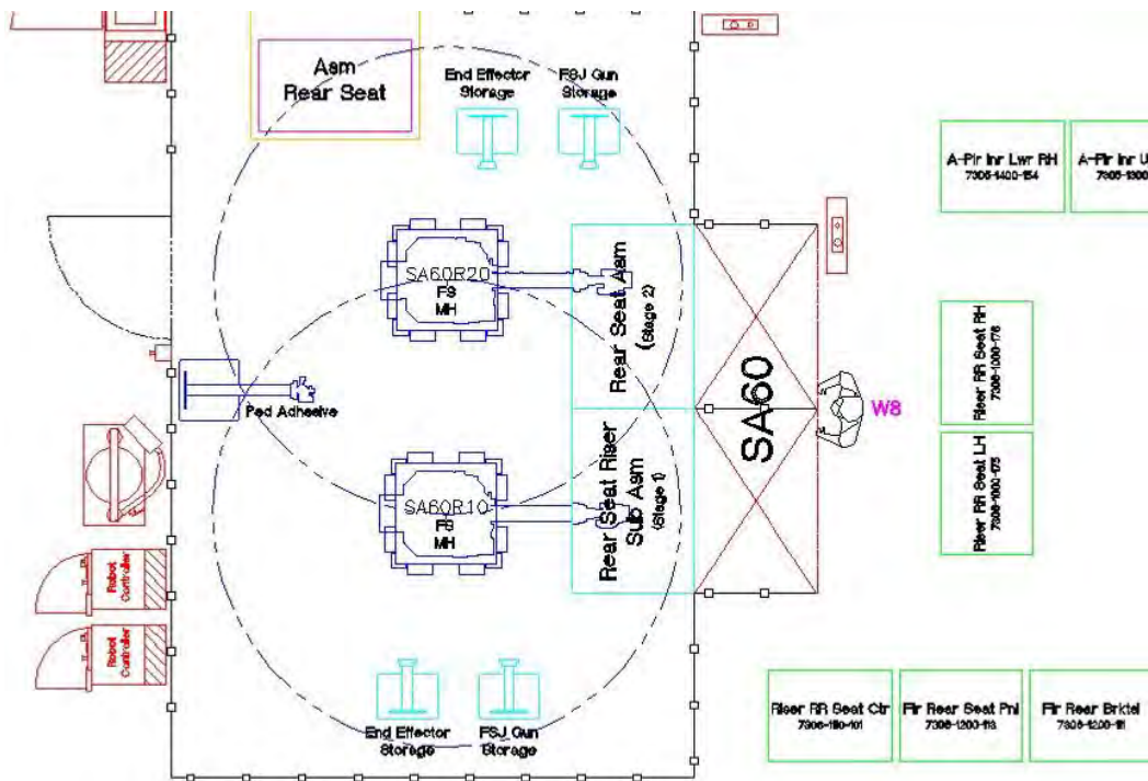
Figure 2.7.k: Station SA60 layout
