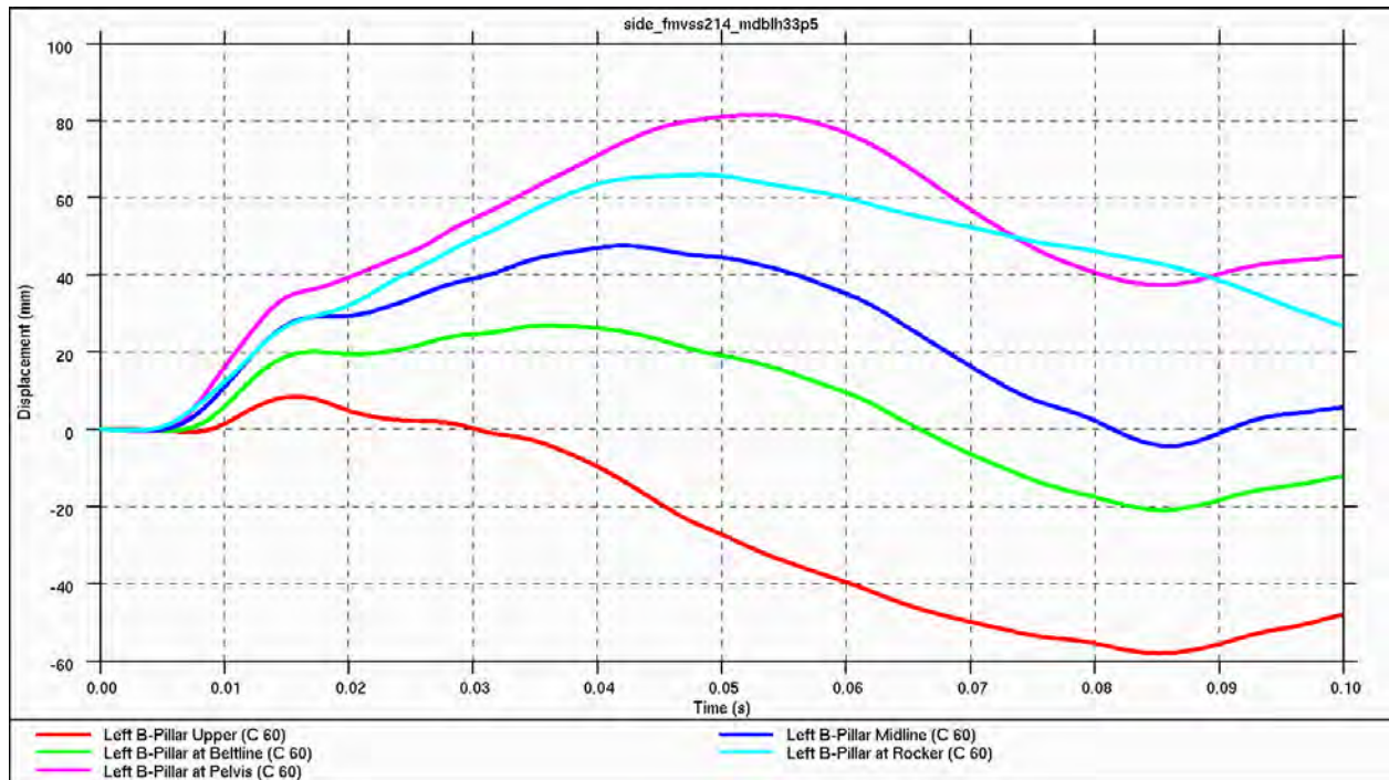
Figure 4.3.7.e: Relative intrusion displacements (B-pillar) during crabbed barrier impact
