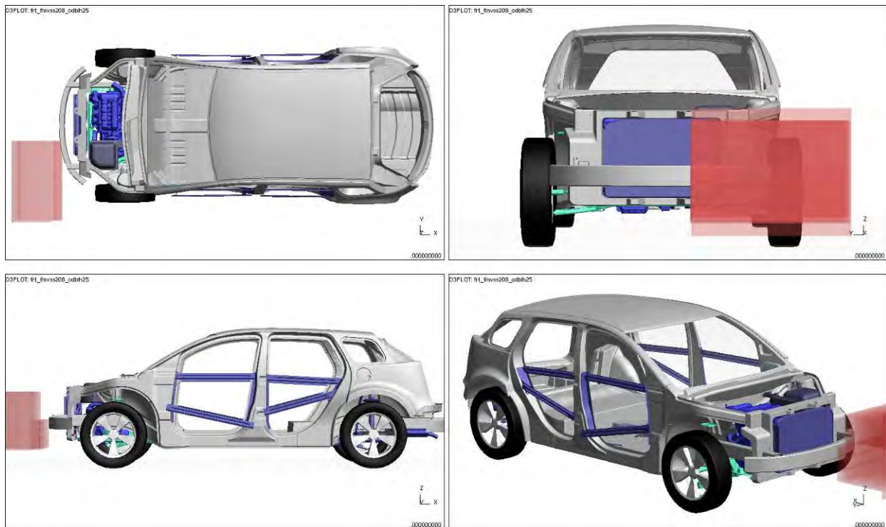
Figure 4.2.5.2a: 40-percent barrier overlap crash-test model setup
