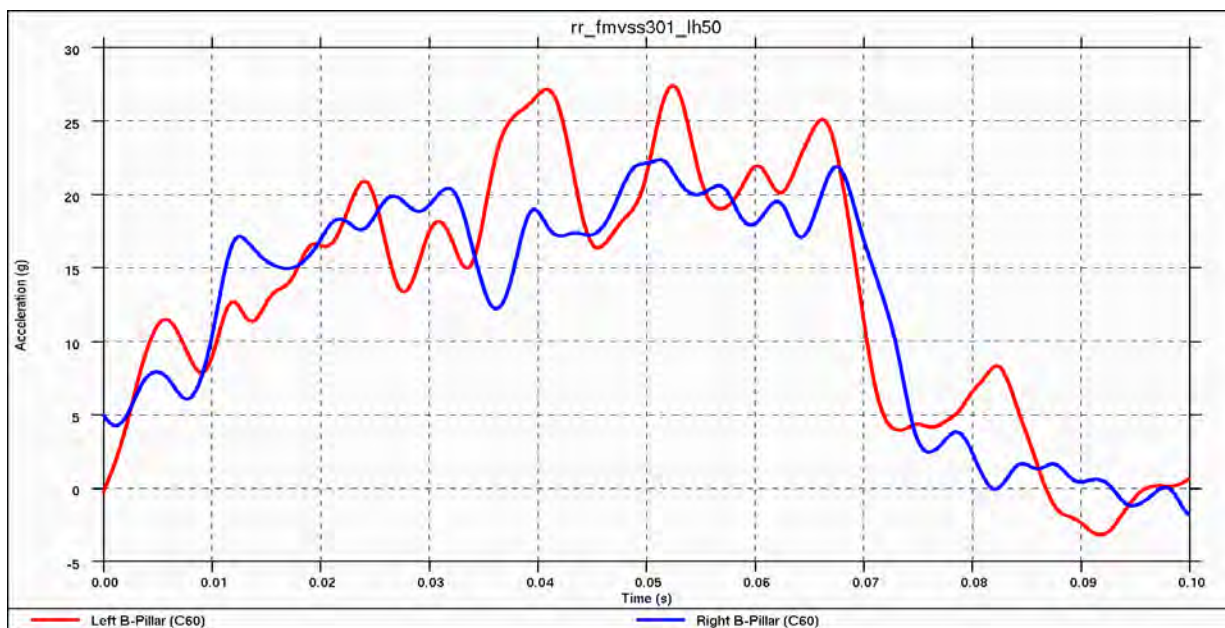
Figure 4.5.4.5.e: Vehicle Acceleration Pulse during rear impact
