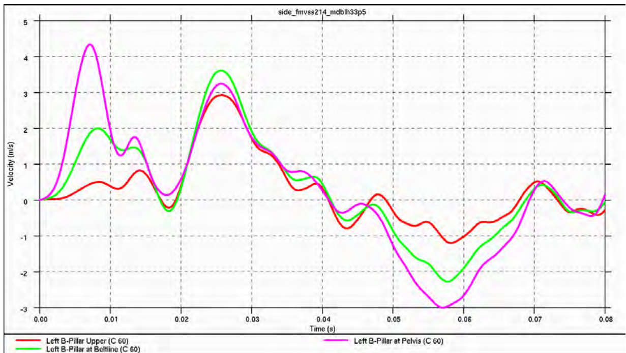
Figure 4.5.4.1.e: Relative Intrusion Velocities (B-pillar)
