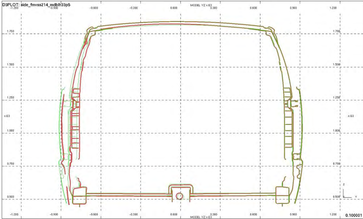
Figure 4.5.4.1.h: B-Pillar Intrusion profile x=2842
