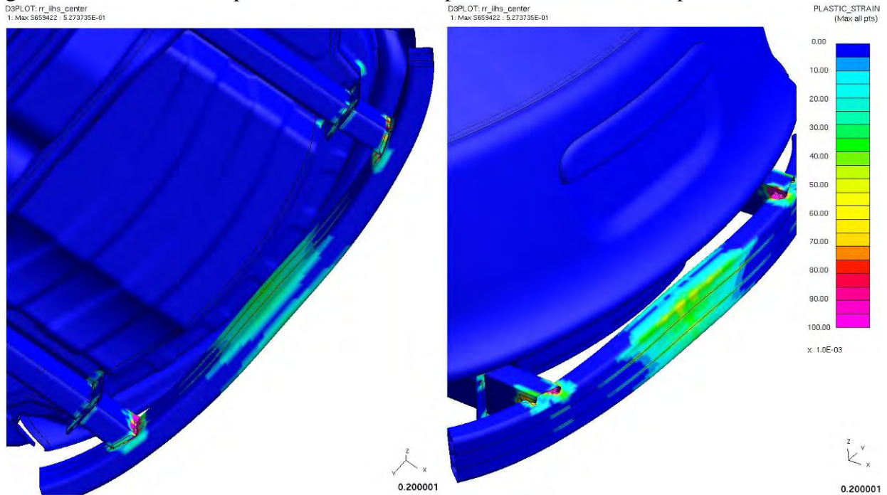
Figure 4.5.4.6.b: IIHS low-speed impact element plastic strains ('full')
