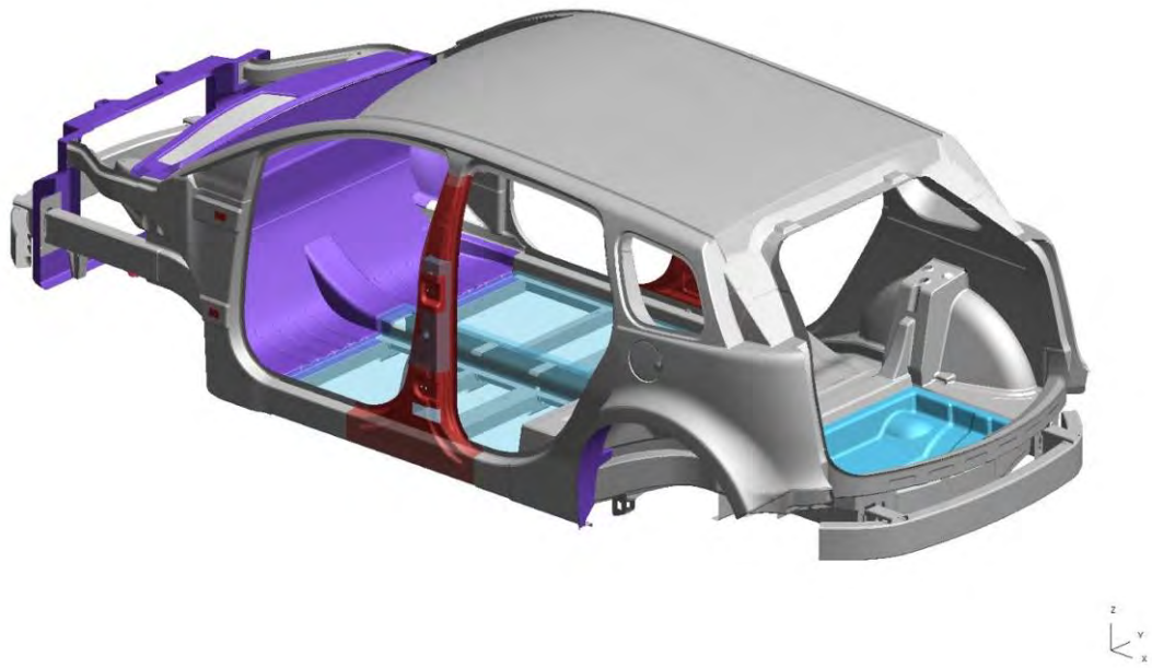
Figure 4.2.3.b: Body-in-white material usage rear three-quarter view
