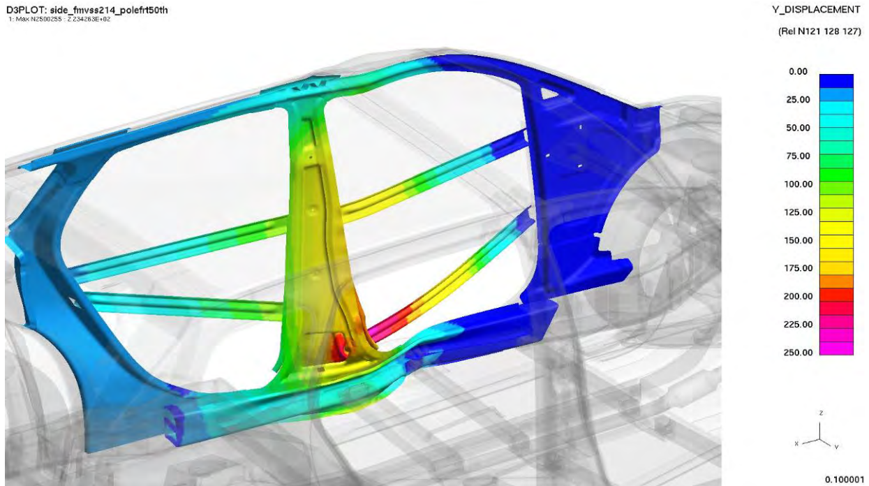
Figure 4.3.9.e: Intrusion levels after 75°, side, pole impact on struck side – 50 th percentile male
