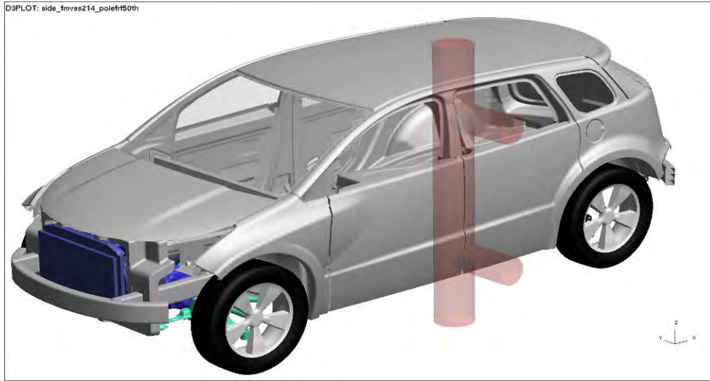
Figure 4.5.4.3.a: 20-mph, 75-degree side-pole impact -- front (50th percentile male) model setup
