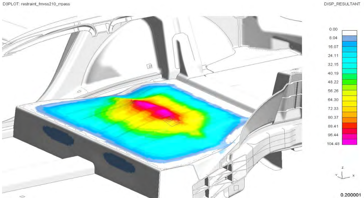
Figure 4.3.5.2.b: Displacement at lower seatbelt anchorages (@0.2 s)
