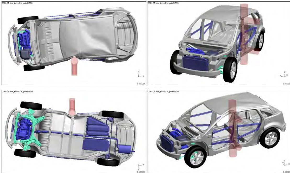
Figure 4.3.9.a: Vehicle deformation (0.1 s) after 75°, side, pole impact – 50 th percentile male
