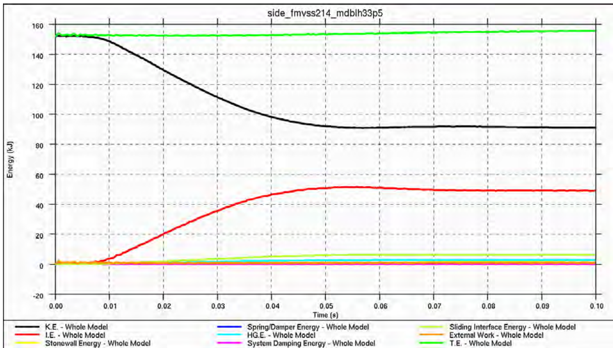
Figure 4.3.7.i: Energy balance for crabbed barrier impact
