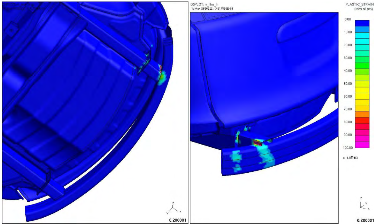
Figure 4.5.4.6.d: IHS low-speed impact element plastic strain ('offset')
