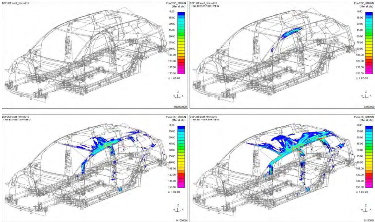
Figure 4.5.4.4.f: Plastic Strains @ 0/40/80/150mm of Roof Platen Displacement
