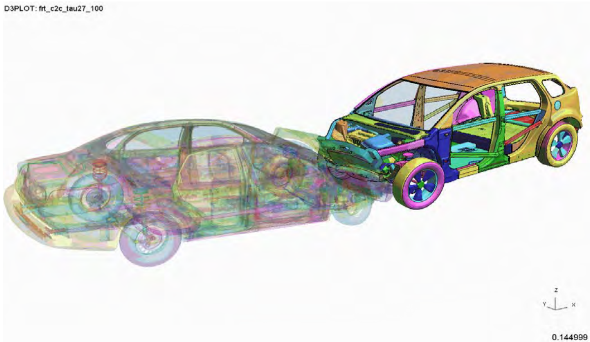
Figure 4.4.9.e: Phase 2 HD vehicle to Ford Taurus crash simulation result – three-quarter view, opaque Taurus
