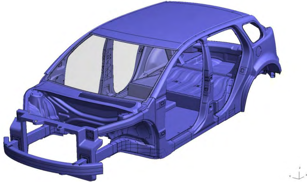
Figure 4.2.1.1.a: Body-in-white – Front
