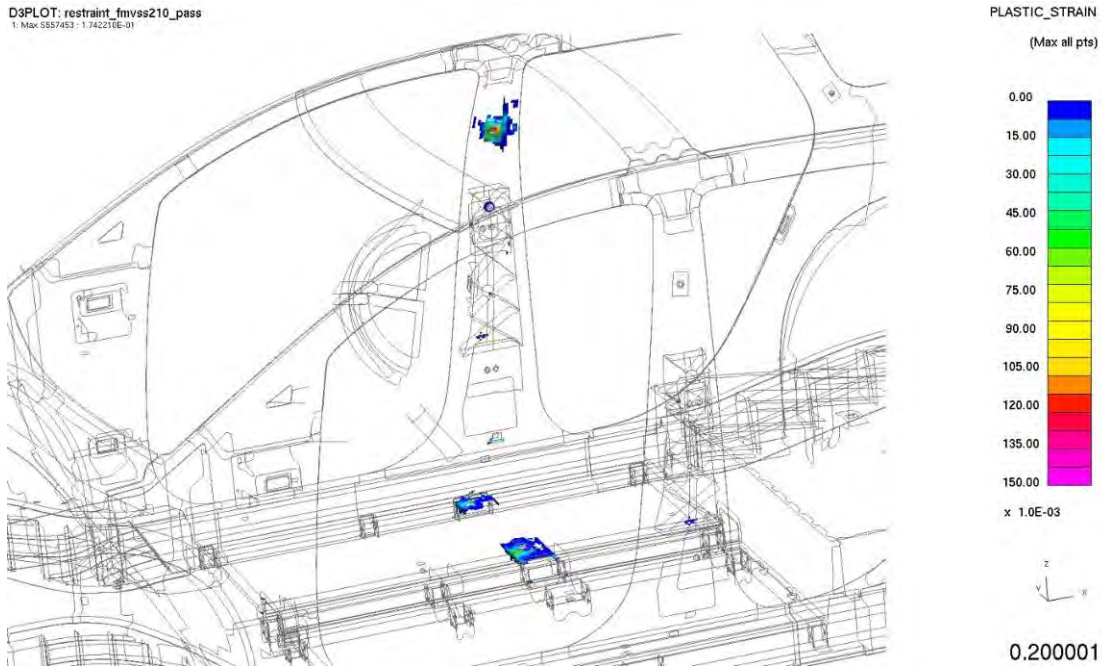
Figure 4.3.5.1.a: Seatbelt anchorage plastic strains (@ 0.2 s)
