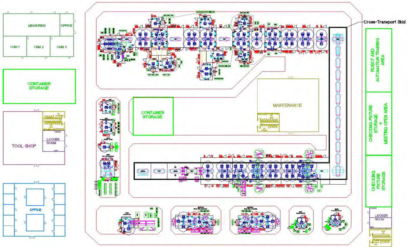
Figure 2.7.at: Overall body shop assembly layout
