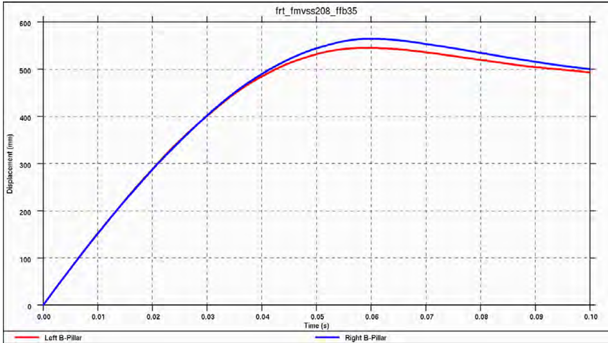
Figure 4.3.1.f: Vehicle displacement from frontal impact - max dynamic crush = 555 mm
