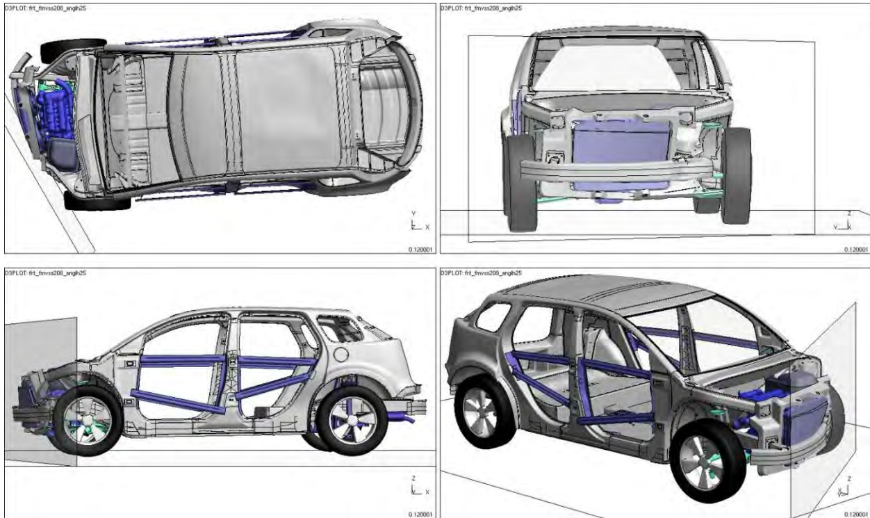
Figure 4.3.3.a: Vehicle deformation (t=0.12 s) after 30°, left-side frontal barrier impact
