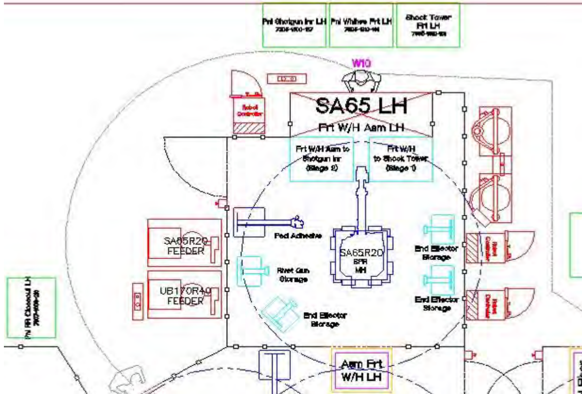
Figure 2.7.m: Station SA65, left-side assembly layout
