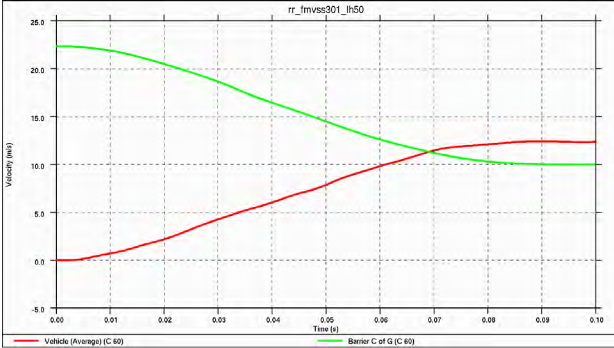
Figure 4.3.11.e: Vehicle and barrier velocities during rear deformable barrier impact
