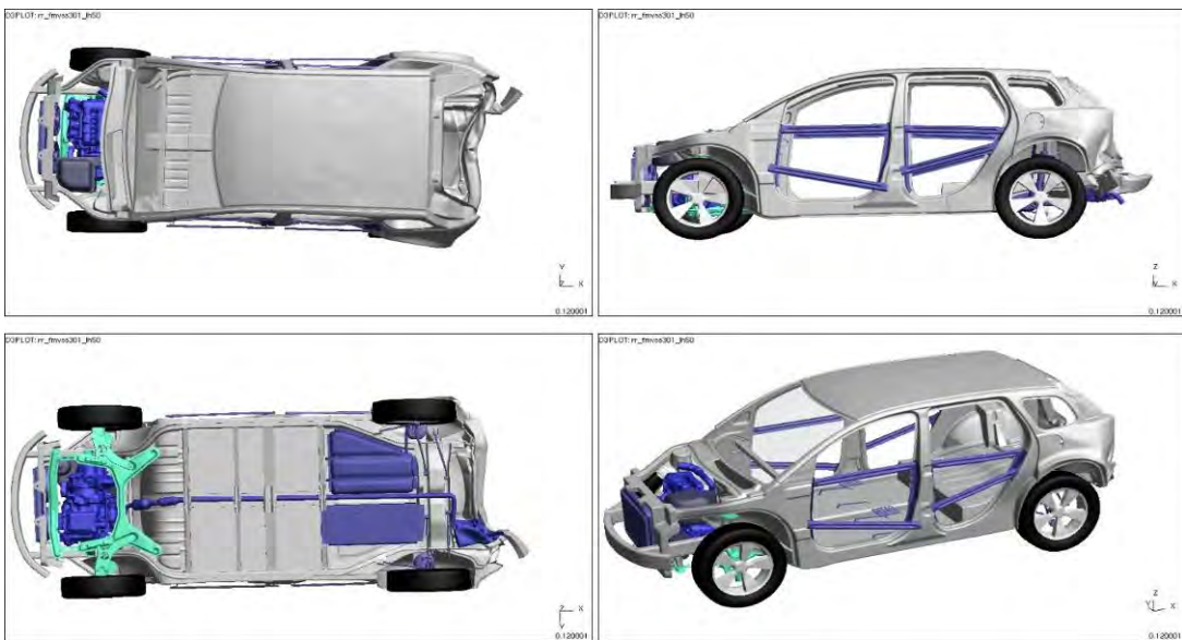
Figure 4.3.11.b: Vehicle deformation (barrier blanked) after rear deformable barrier impact
