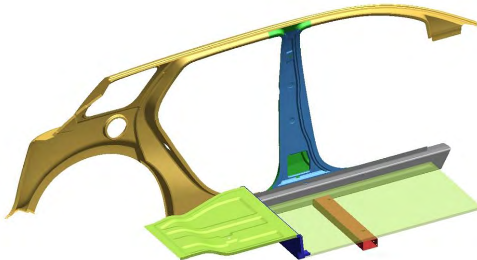
Figure 4.3.9.g: Main energy absorbing body structure for 75°, side, pole impact – 50 th percentile male
