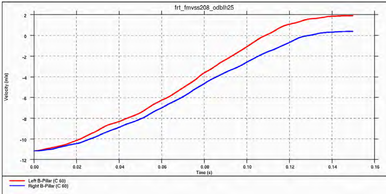
Figure 4.3.2.e: Vehicle velocity after 40-percent overlap frontal impact - time to zero (TTZ) = 0.117 s
