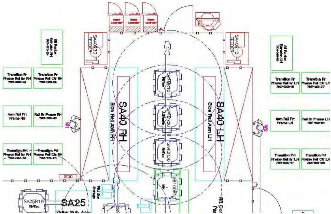
Figure 2.7.g: Station SA40 layout
