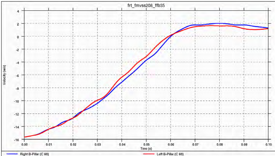
Figure 4.3.1.d: Vehicle velocity during frontal impact - time to 0 velocity (TTZ) = 59.5 ms
