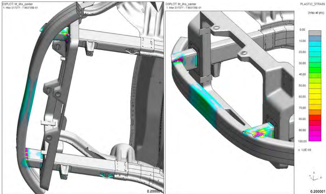
Figure 4.3.12.a: Front plastic strain after low-speed frontal impact ('full impact')
