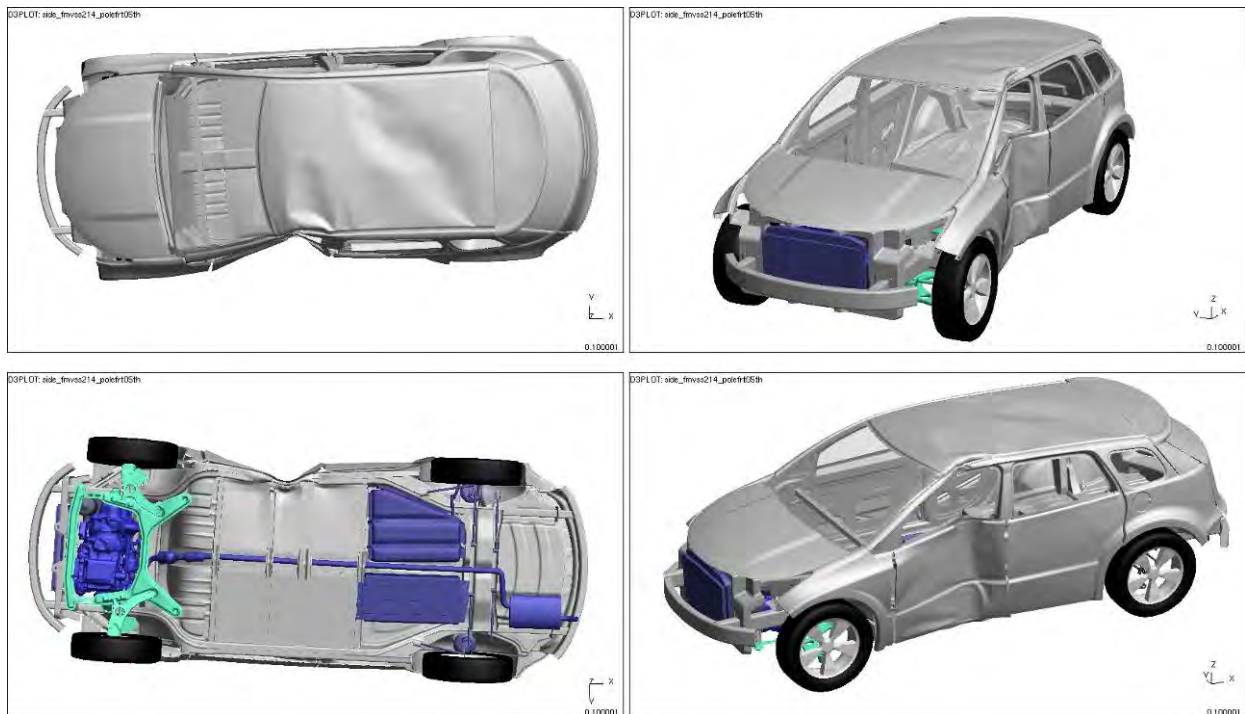
Figure 4.5.4.2.c: Vehicle deformation from 20-mph, 75-degree side-pole impact -- front (5th percentile female, pole blanked)
