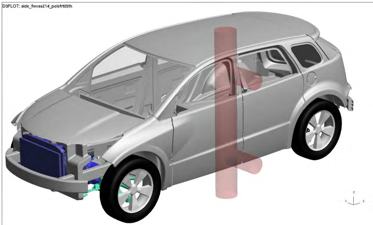
Figure 4.5.4.2.a: 20-mph, 75-degree side-pole impact -- front (5th percentile female) model setup
