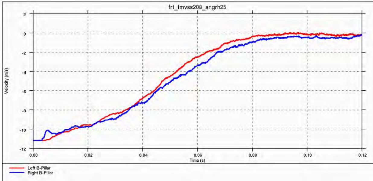
Figure 4.3.4.d: Vehicle velocity during 30°, right-side frontal impact - time to zero velocity (TTZ) = 92 ms
