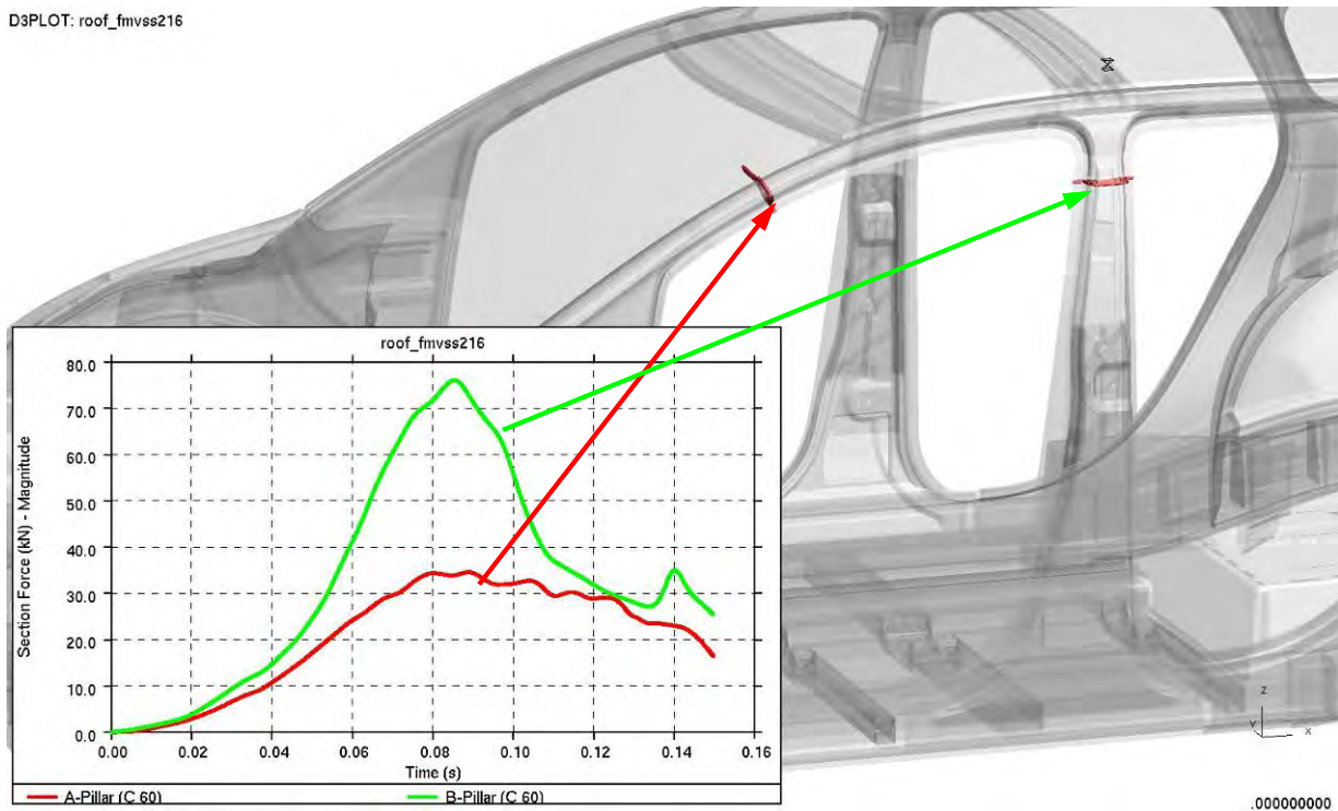
Figure 4.5.4.4.1.a: Resultant force magnitude in A & B-Pillars from roof crush test
