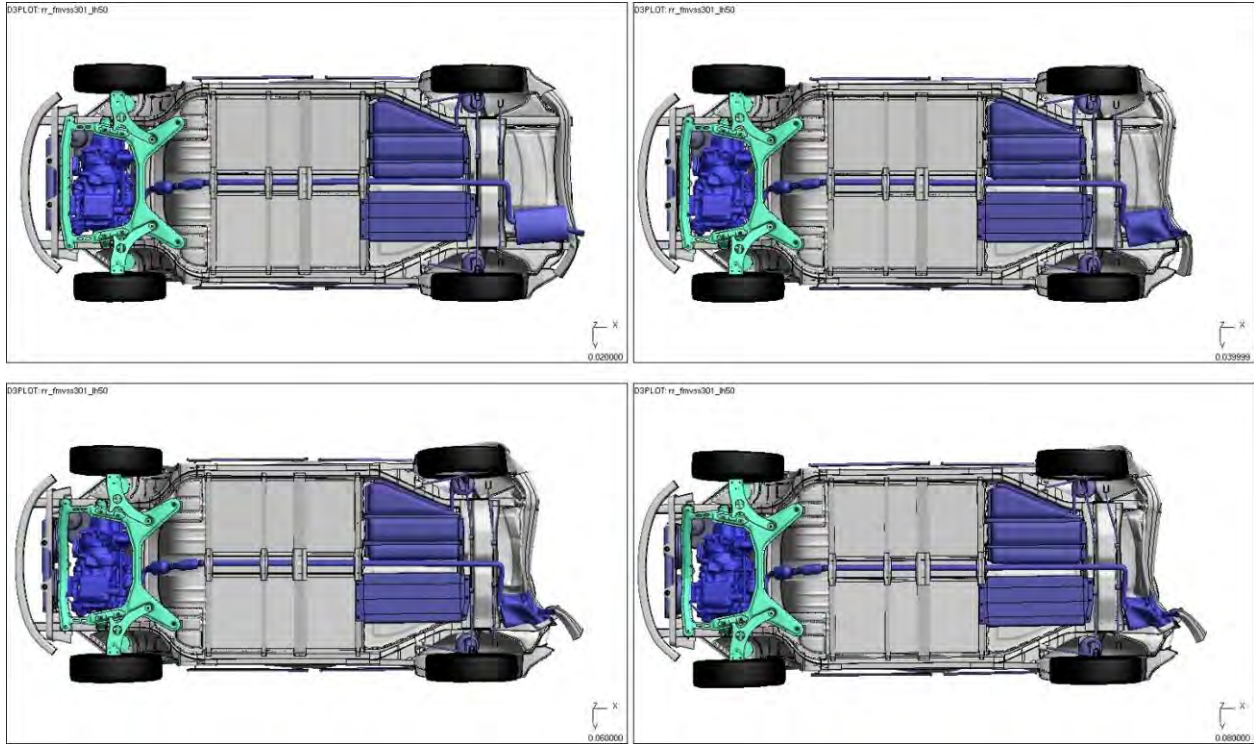
Figure 4.3.11.c: Vehicle deformation (at 0/40/80/120 ms) after rear deformable barrier impact
