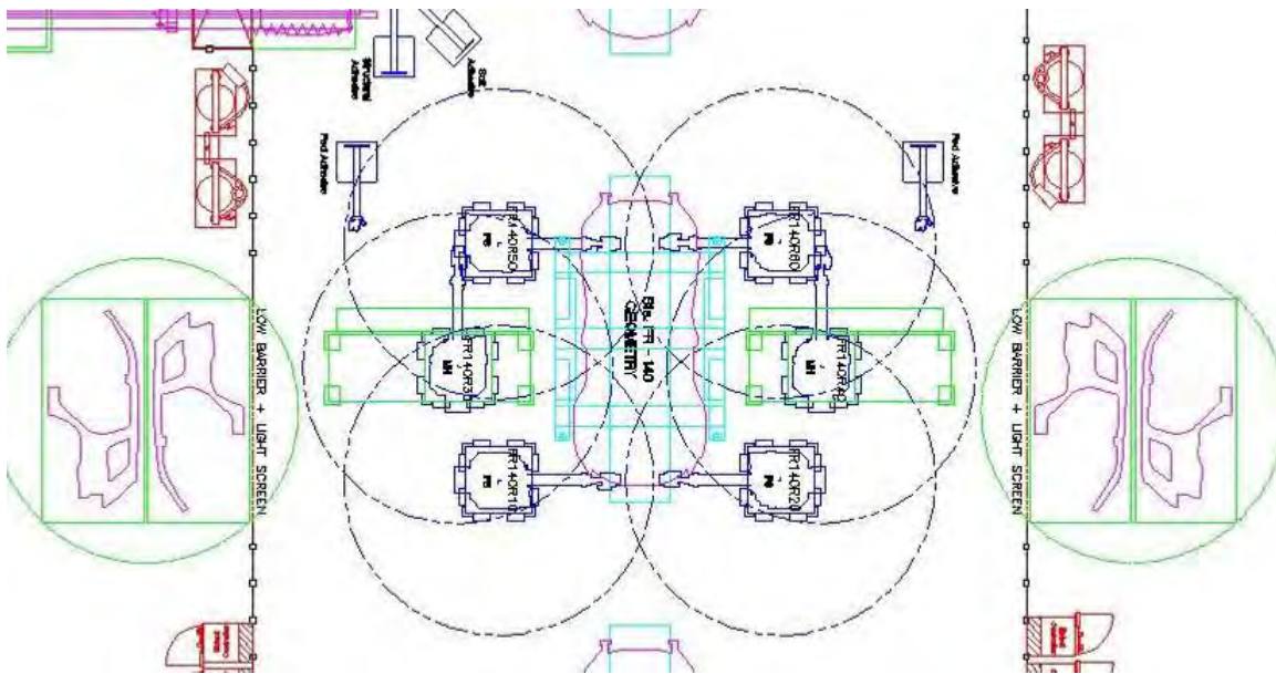
Figure 2.7.am: Station FR140 assembly layout
