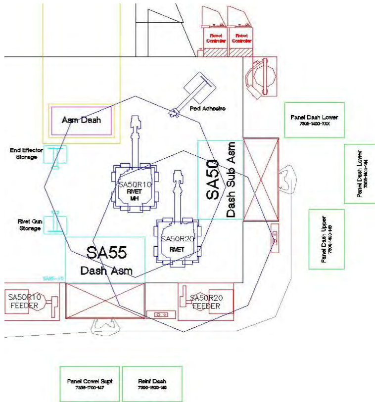
Figure 2.7.j: Stations SA50, SA55 layout
