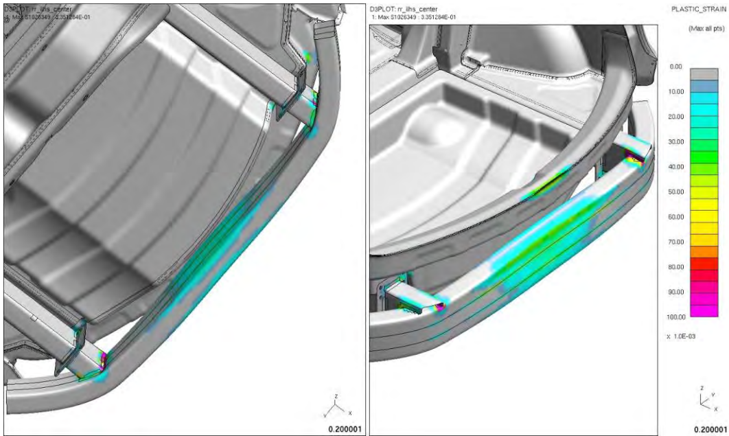
Figure 4.3.13.a: Rear plastic strains after low-speed rear impact ('full impact')
