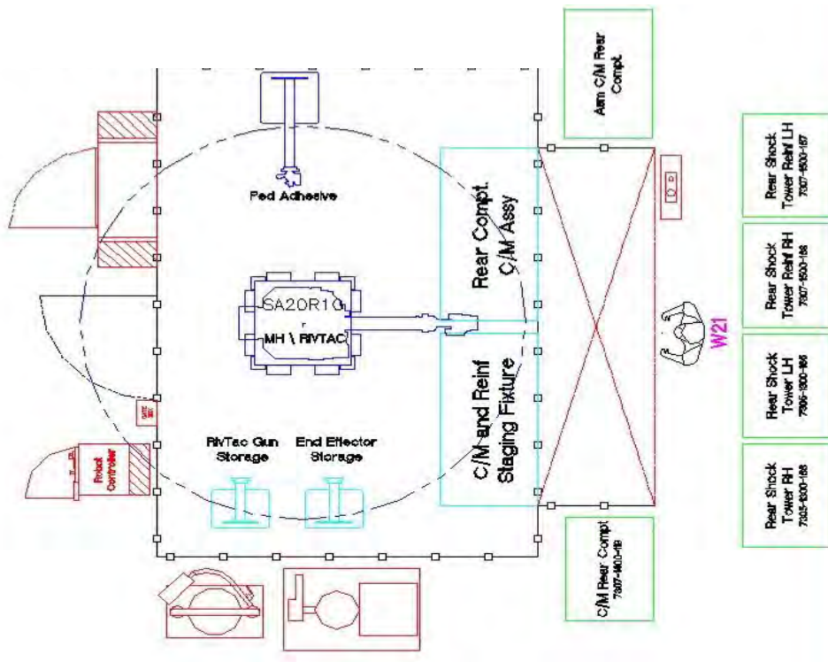
Figure 2.7.d: Station SA20 layout
