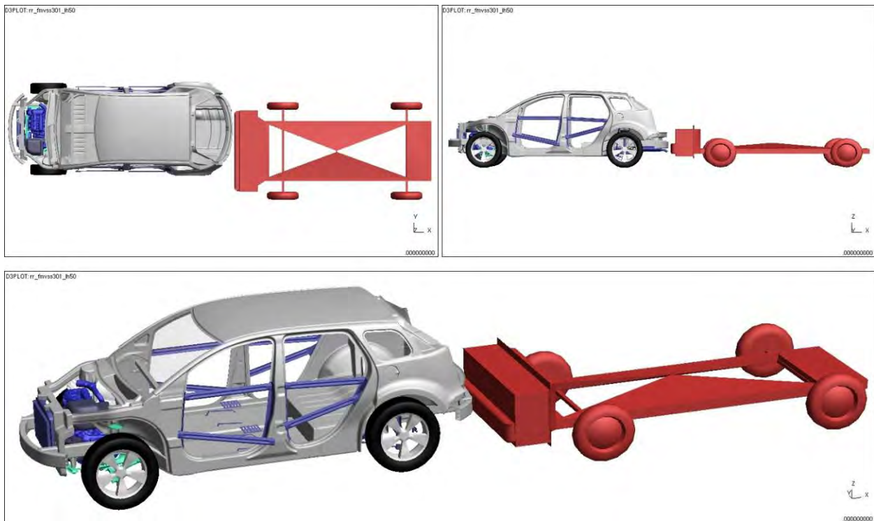
Figure 4.2.5.11.a: Deformable, moving barrier rear impact test model setup
