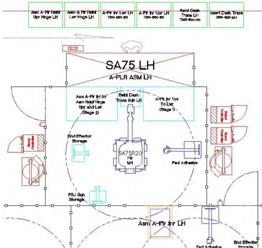
Figure 2.7.q: Station SA75, left-side assembly
