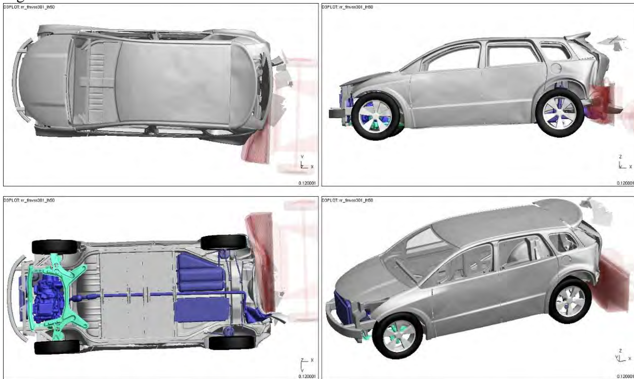
Figure 4.5.4.5.b: Vehicle Deformation ( t=0.12s )
