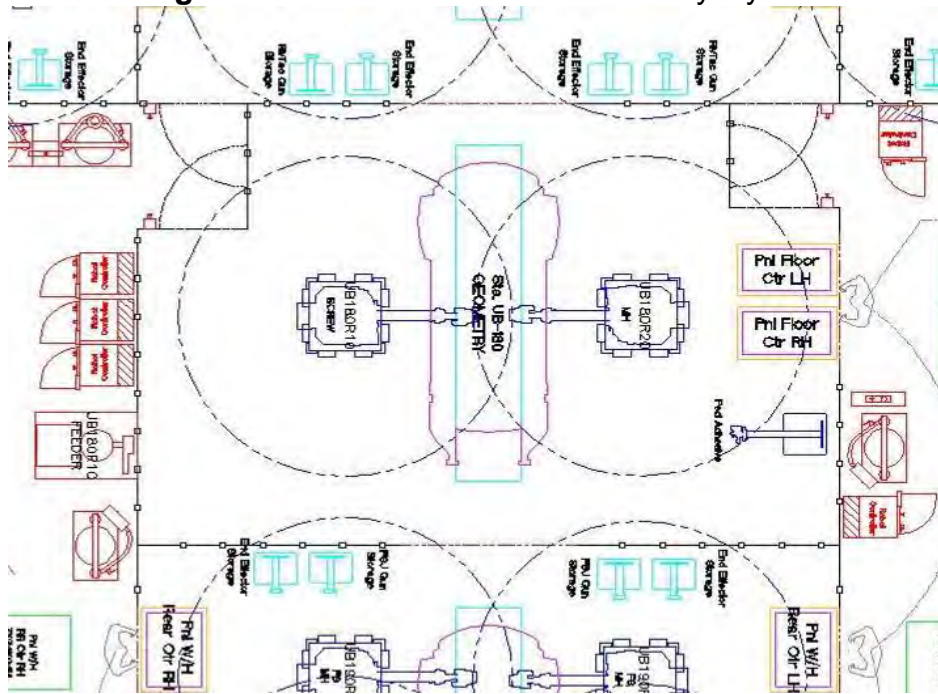
Figure 2.7.ab: Station UB180 assembly layout
