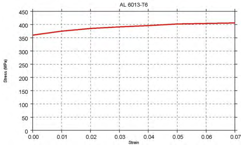
Figure 4.2.2.2.a: 6013 aluminum stress-strain curve
