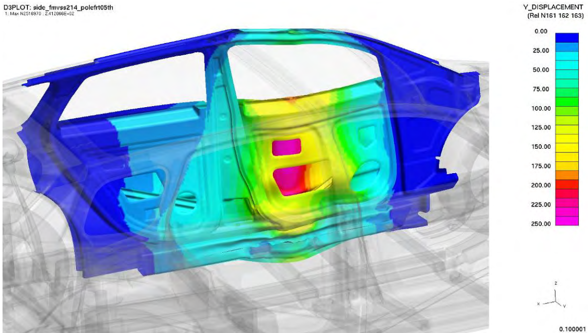
Figure 4.5.4.2.g: Intrusion levels on struck side
