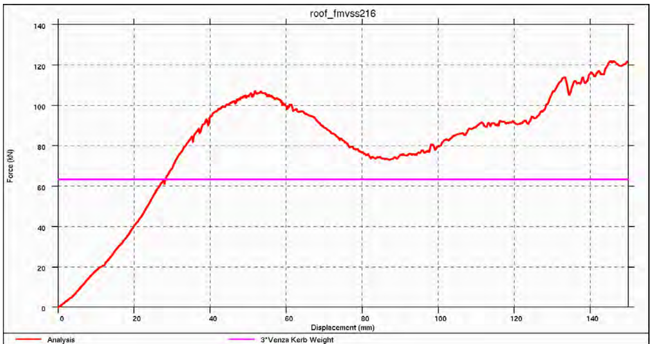
Figure 4.5.4.4.e: Roof Displacement vs. Applied Force – 3 times Venza Weight
