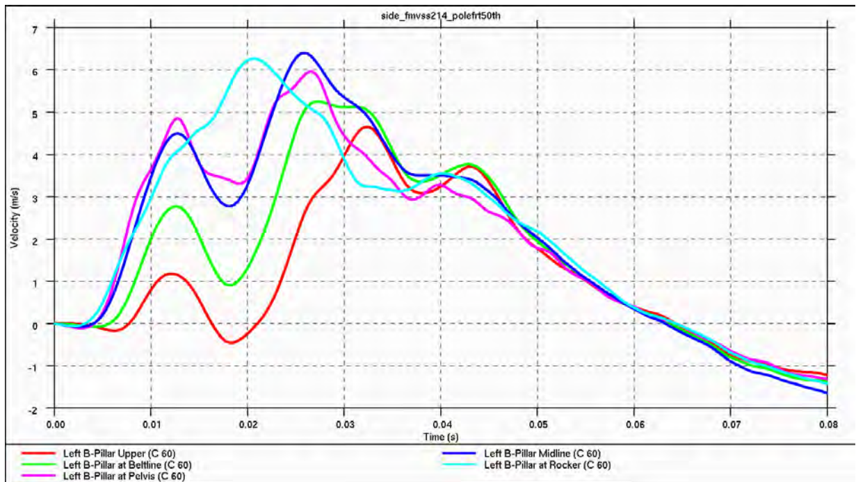
Figure 4.3.9.c: Relative intrusion velocities during 75°, side, pole impact (B-pillar) – 50 th percentile male
