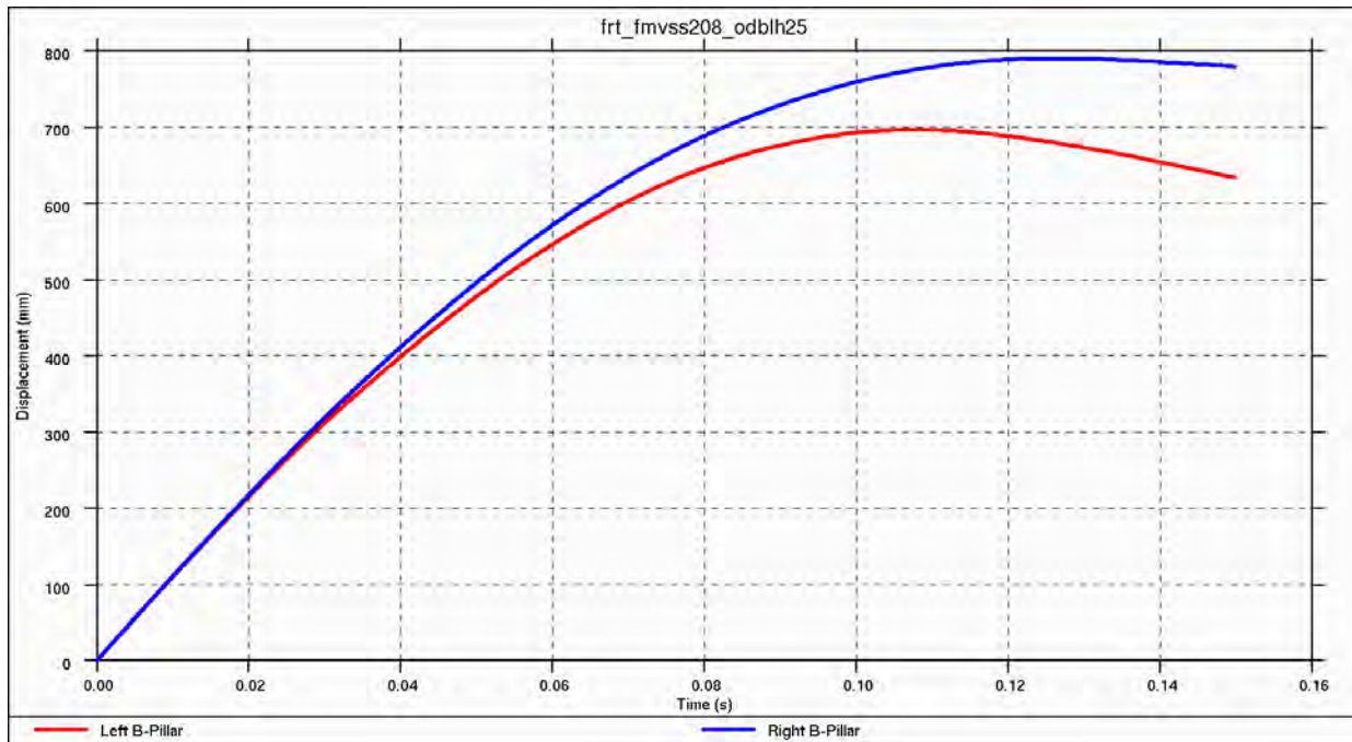
Figure 4.3.2.f: Vehicle displacement after 40-percent overlap frontal impact
