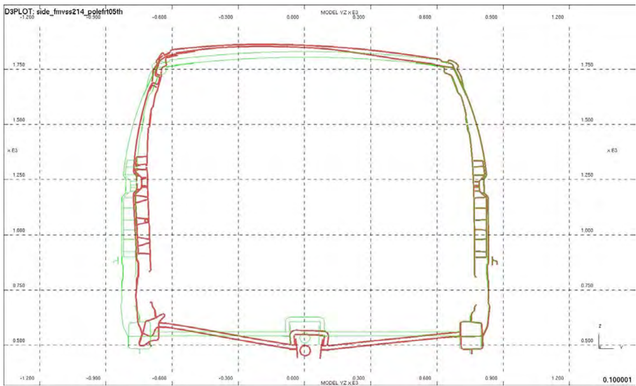
Figure 4.3.8.e: Section through B-pillar after 75°, side, pole impact, x= 2842 – 5 th percentile female
