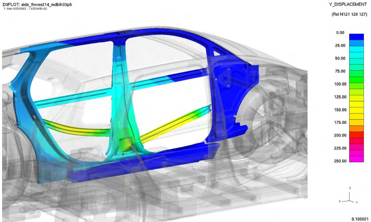
Figure 4.3.7.g: Intrusion levels after crabbed barrier impact on struck side
