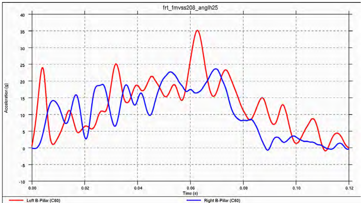
Figure 4.3.3.b: Vehicle acceleration pulse during 30°, left-side frontal barrier impact
