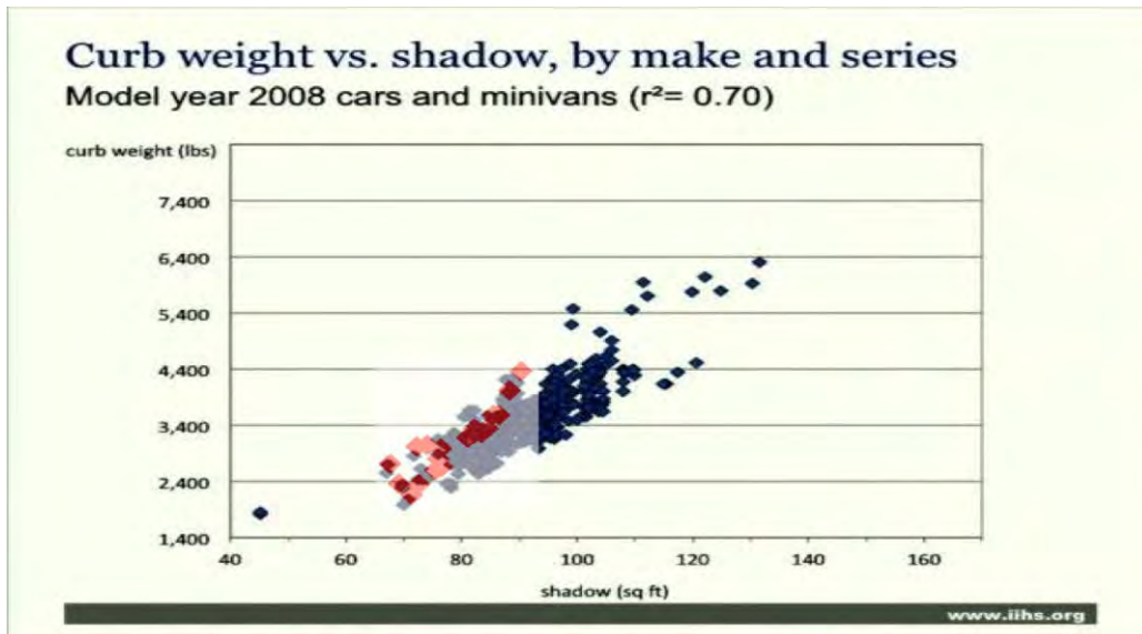
Figure B.a: IIHS and Lotus vehicle data, curb weight as a function of shadow
