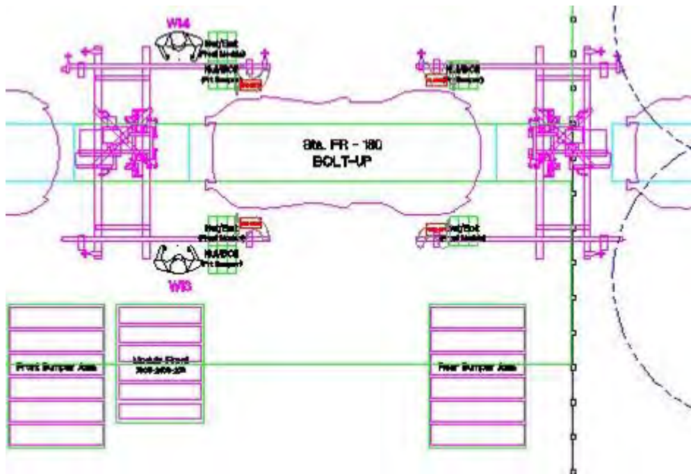
Figure 2.7.aq: Station FR180 assembly layout
