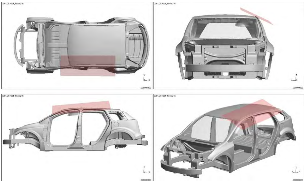
Figure 4.5.4.4.a: Roof crush model setup
