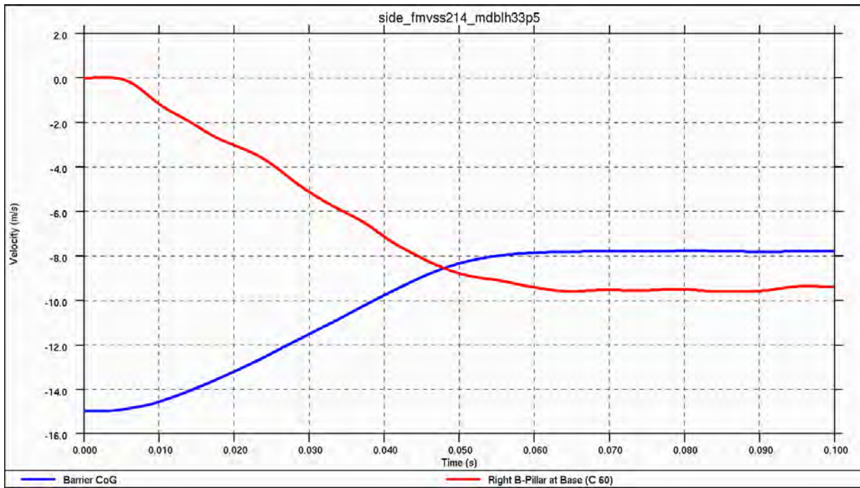
Figure 4.5.4.1.d: Global Vehicle and Barrier Velocities
