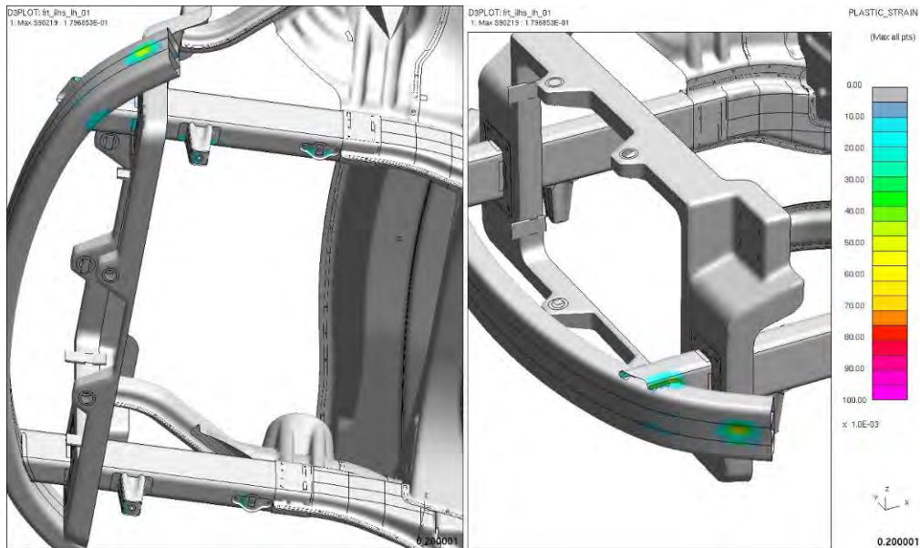
Figure 4.3.12.b: Front plastic strain after low-speed frontal impact ('offset impact')
