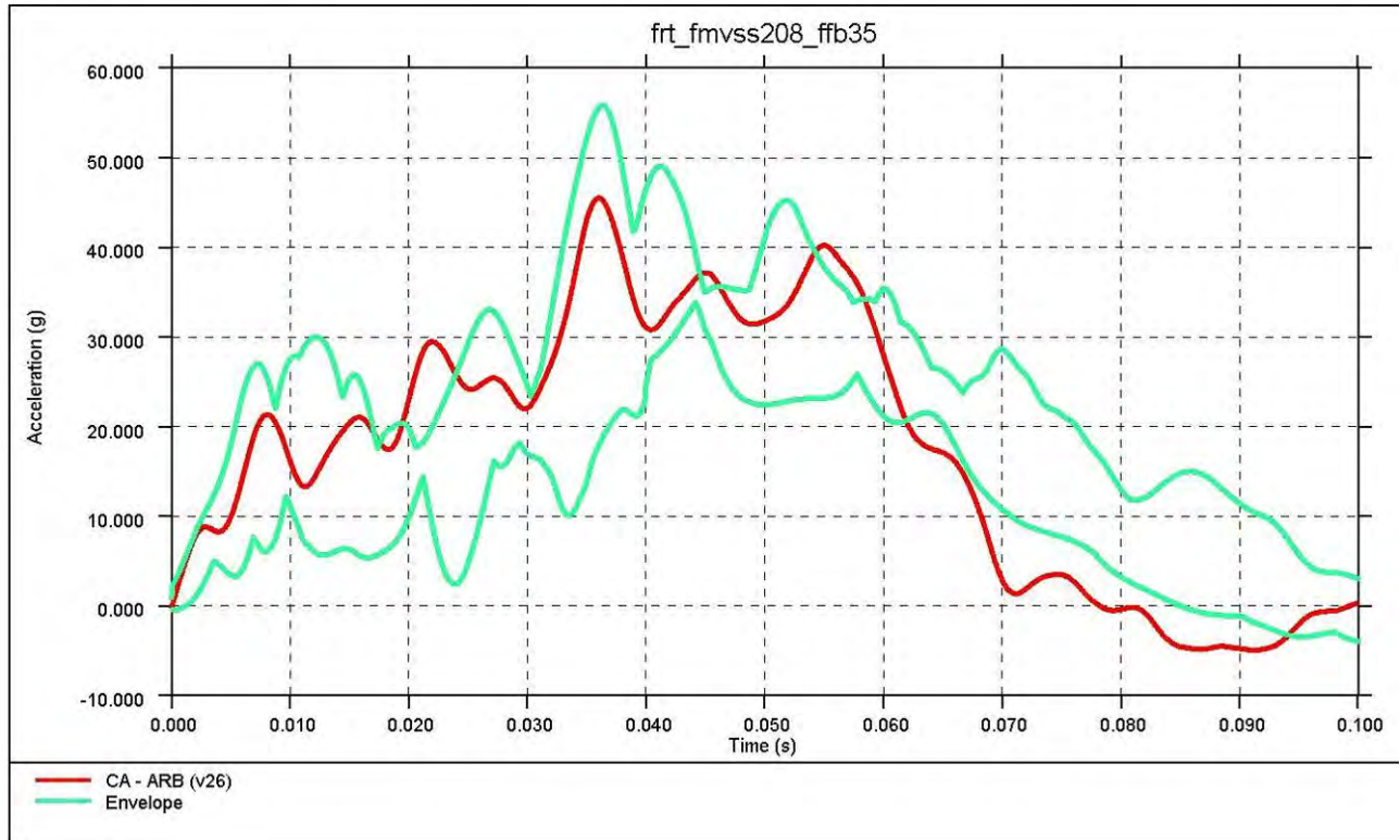
Figure 4.3.2.I: Comparison of production vehicle envelope and Phase 2 HD crash accelerations
