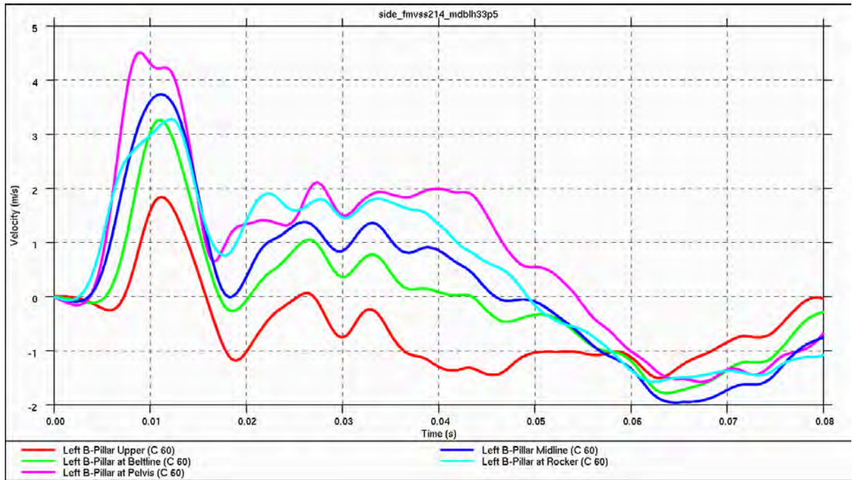
Figure 4.3.7.d: Relative intrusion velocities (B-pillar) during crabbed barrier impact
