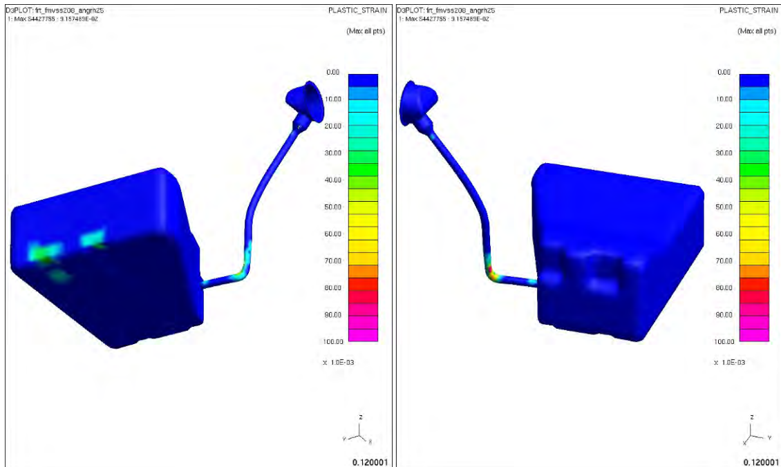
Figure 4.3.4.g: Fuel tank plastic strains after 30°, right-side frontal impact
