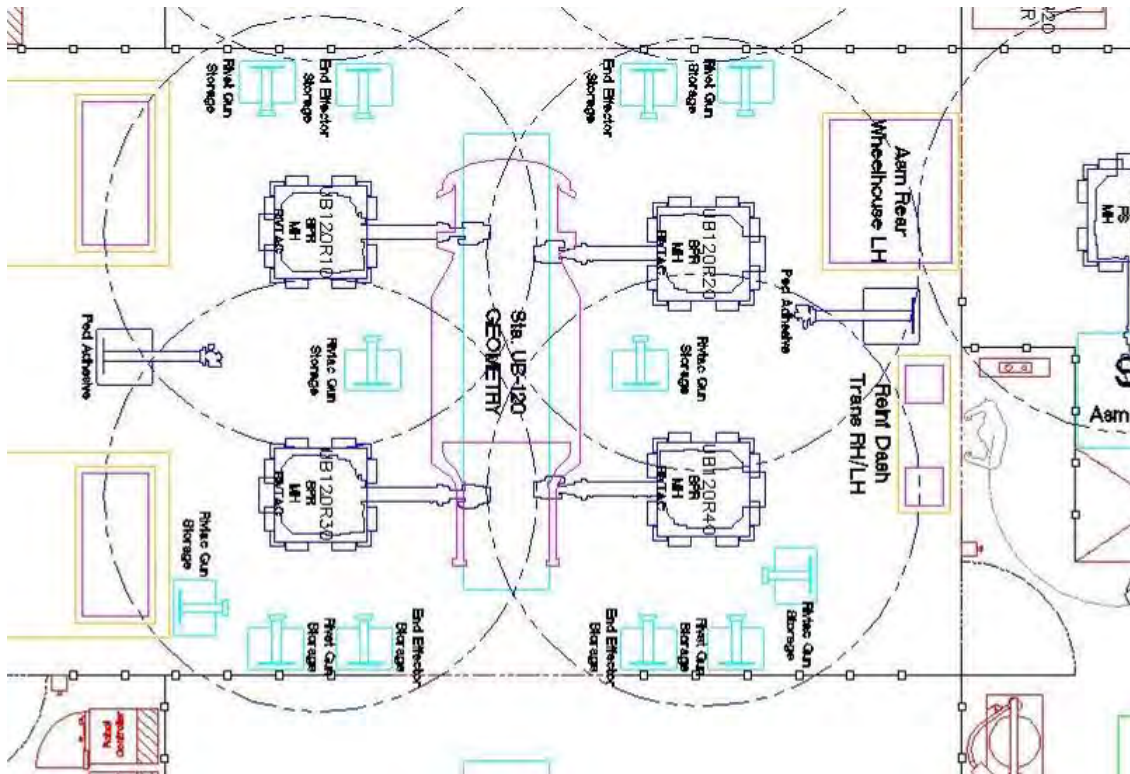
Figure 2.7.v: Station UB120 assembly layout
