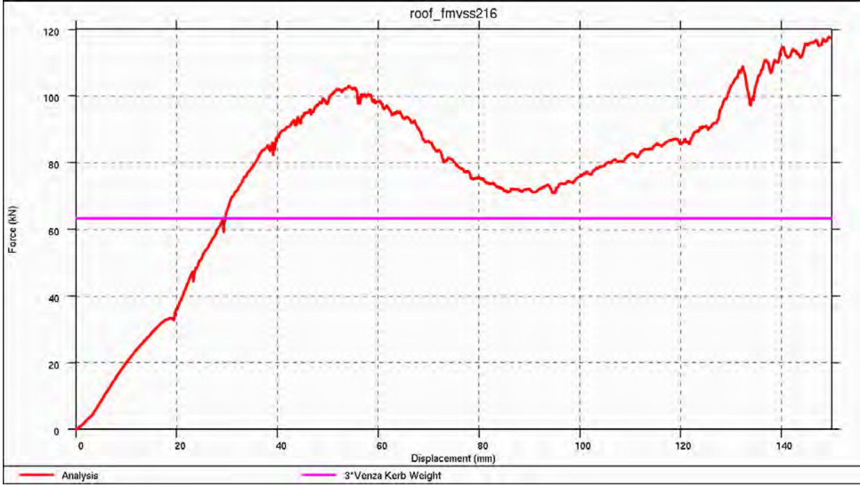
Figure 4.3.10.d: Roof displacement vs. applied force – 3 times Venza weight
