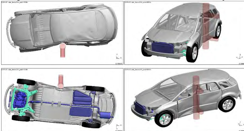
Figure 4.5.4.3.b: Vehicle Deformation (0.1s) after impact
