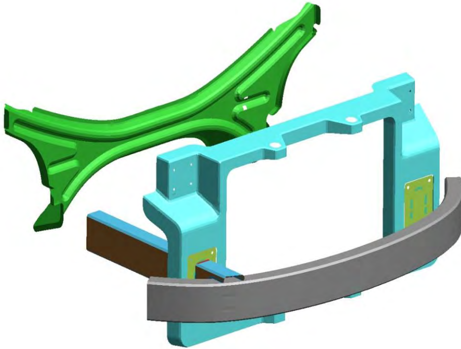
Figure 4.3.4.h: Main energy absorbing body structure for 30°, right-side frontal impact
