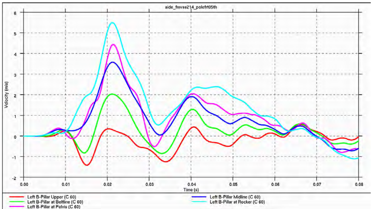
Figure 4.3.8.c: Relative intrusion velocities during 75°, side, pole impact (B-pillar) – 5 th percentile female
