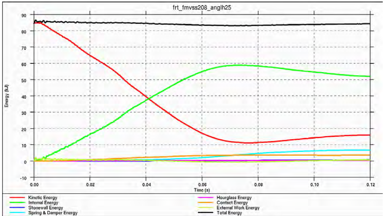
Figure 4.3.3.i: Energy balance for 30°, left-side frontal impact
