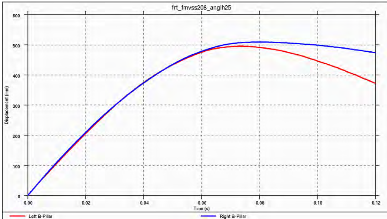
Figure 4.3.3.e: Vehicle displacement during 30°, left-side frontal impact – max dynamic crush = 500 mm
