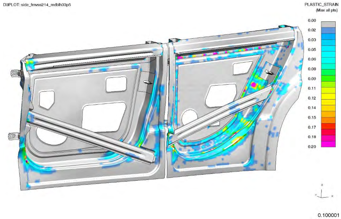
Figure 4.5.4.1.j: Plastic Strain in Struck-side Doors
