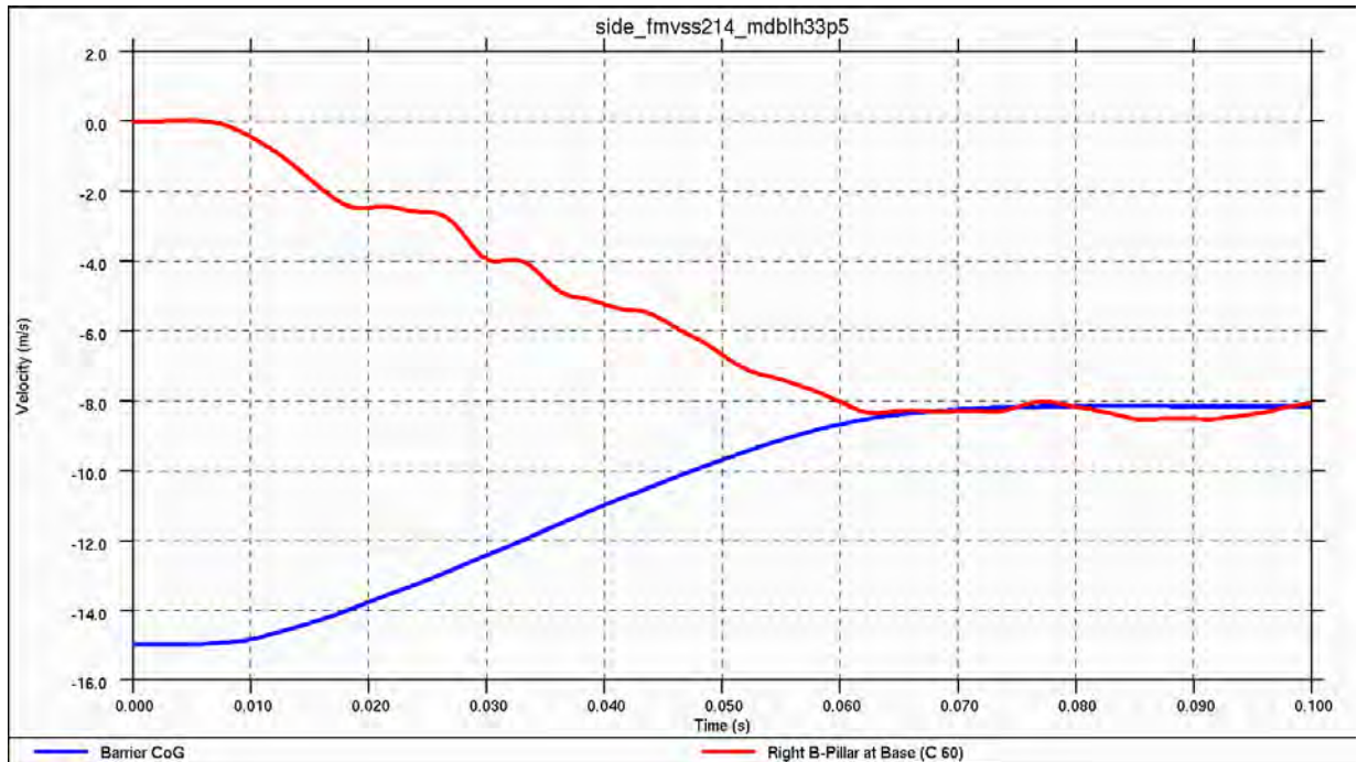
Figure 4.3.7.c: Global vehicle and barrier velocities for crabbed barrier impact
