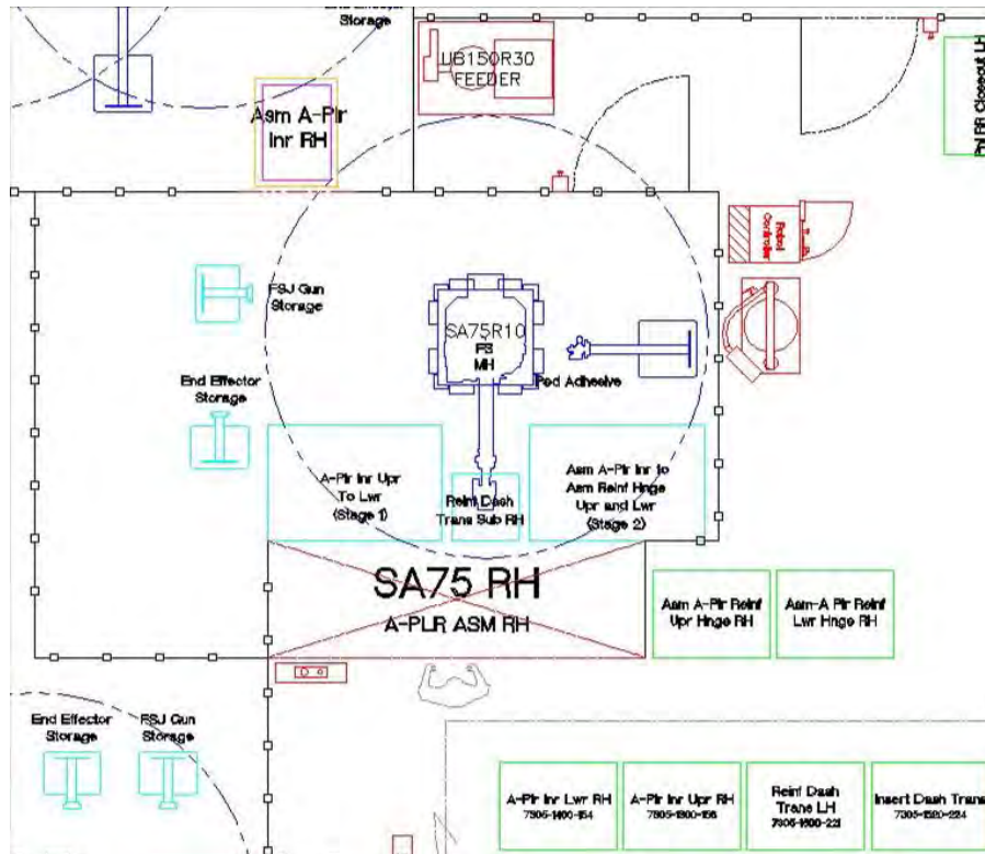
Figure 2.7.p: Station SA75, right-side assembly layout
