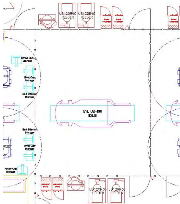
Figure 2.7.w: Station UB130 assembly layout
