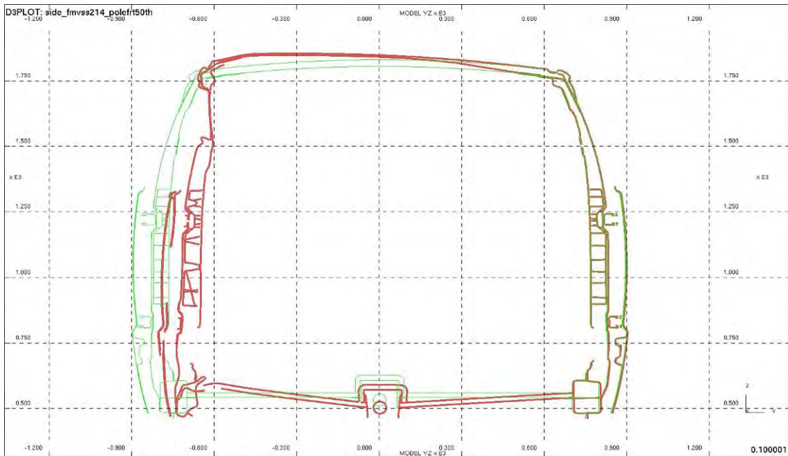
Figure 4.5.4.3.g: Section through B-Pillar, x = 2842 after 20-mph, 75-degree side-pole impact -- front (50 th percentile male)
