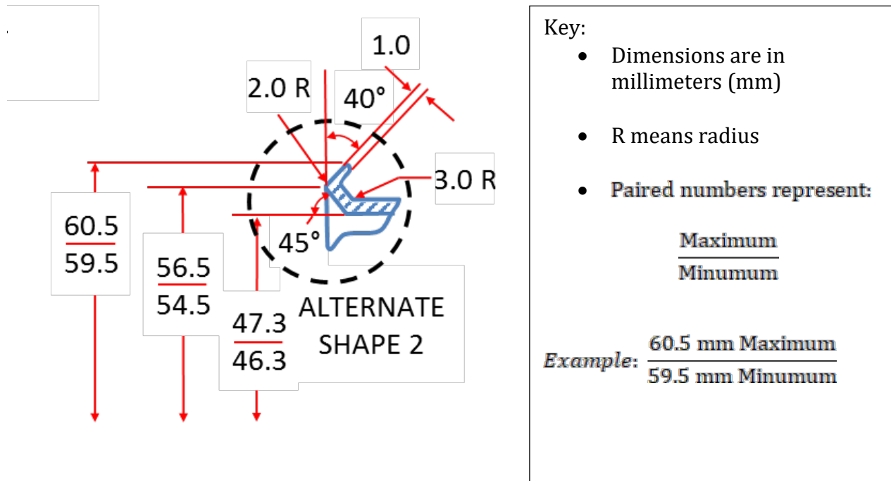
Figure A: Alternate Shape 2, cross-section of a vehicle fill pipe head.
