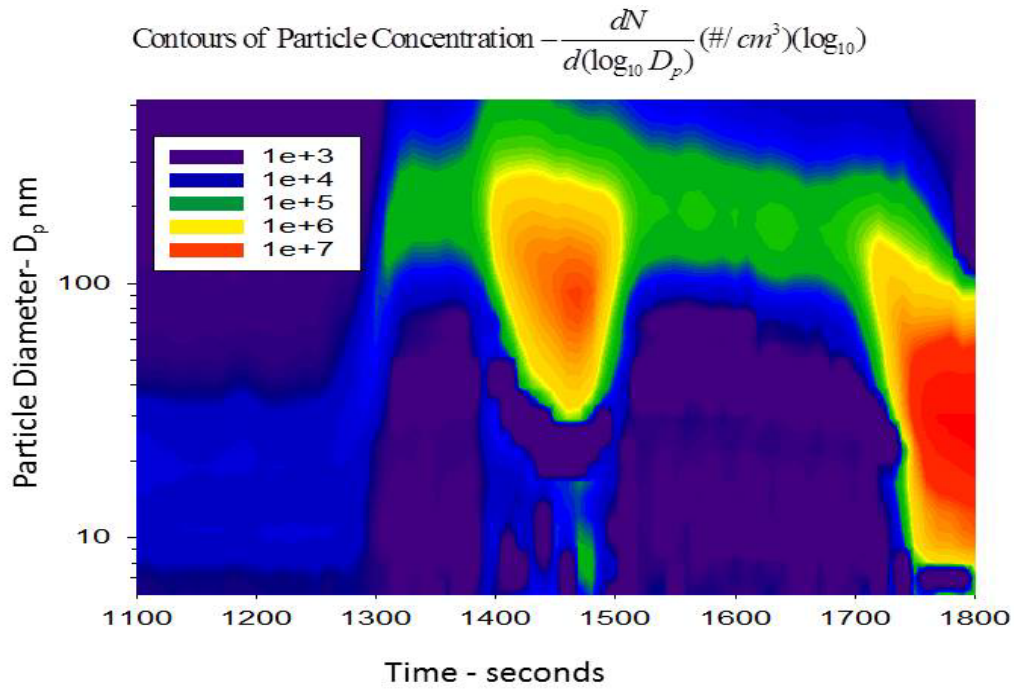
Figure III-23 Expanded view of EEPs particle number concentration emissions during the initial part of the regeneration event. Test3
