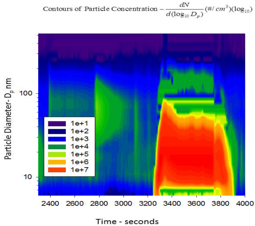
Figure III-7 EEPS particle number concentration emissions during the high emission part of the continued regeneration event. Test1(b)
