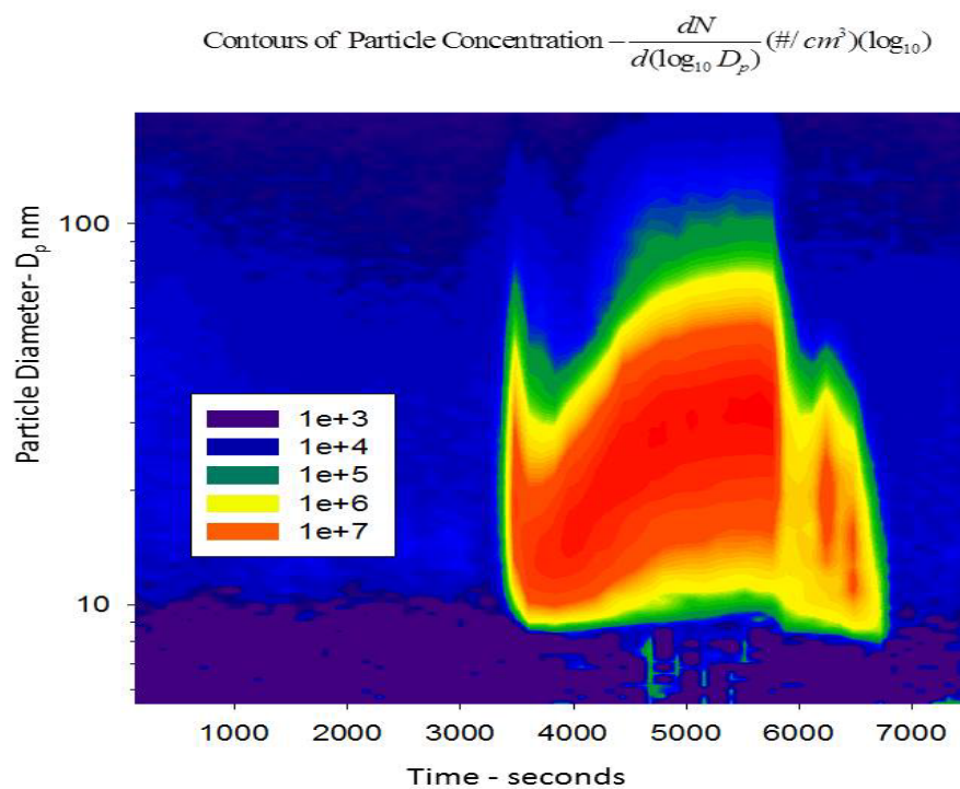
Figure III-33 SMPS particle number concentration emissions during the regeneration event. Test4(a)
