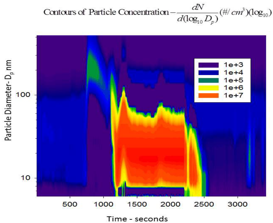
Figure III-18 EEPS particle number concentration emissions during the forced regeneration event. Test2
