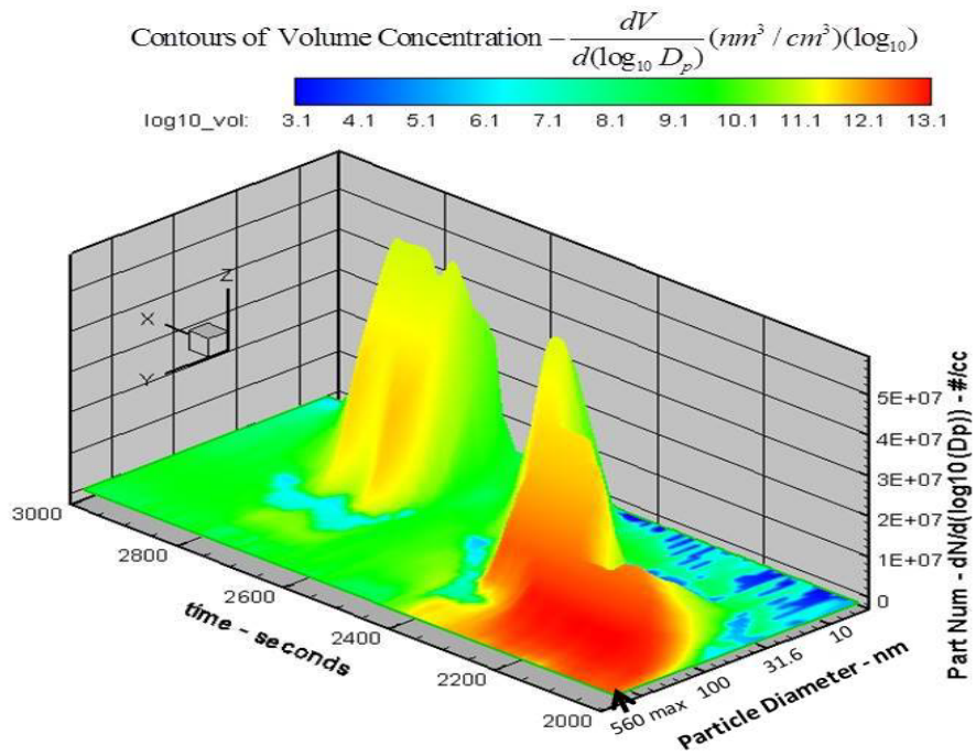
Figure III-6 Expanded view of EEPS particle number and volume concentrations emissions during the initial part of the regeneration event. Test1(a).
