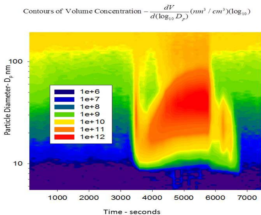
Figure III-34 SMPS Volume concentration emissions during the regeneration event. Test4(a)
