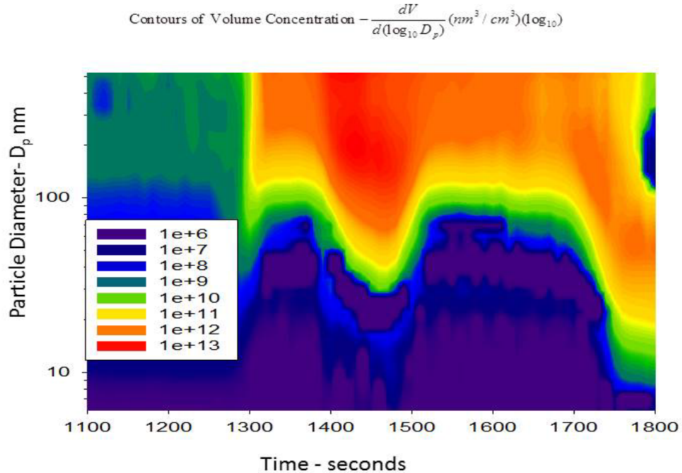
Figure III-24 Expanded view of EEPs particle volume concentration emissions during the initial part of the regeneration event. Test3
