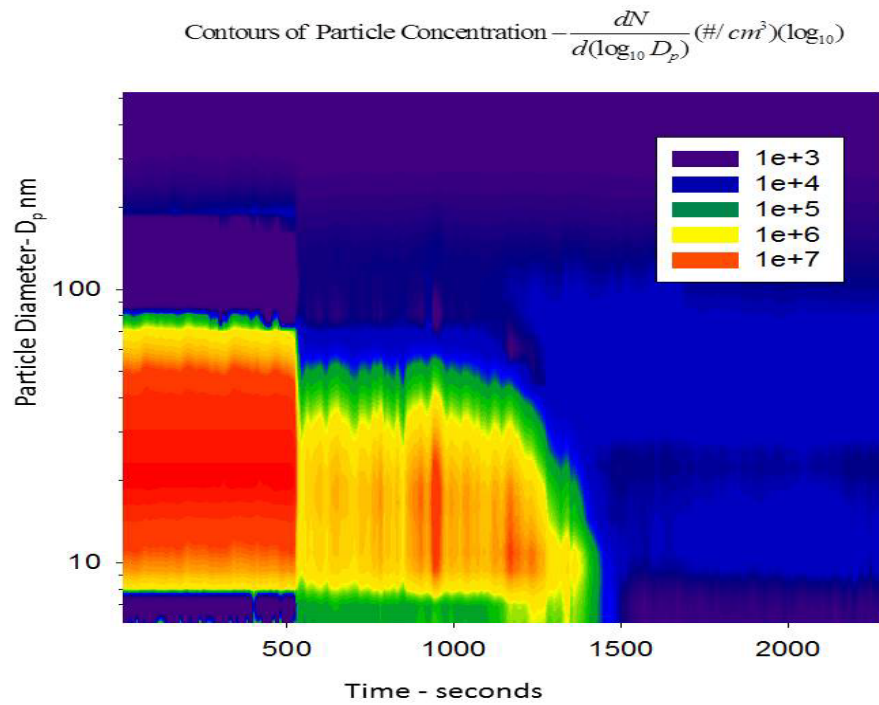
Figure III-35 EEPS particle number concentration emissions during the regeneration event. Test4(a)
