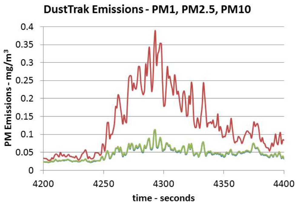
Figure III-38 PM1 and PMTotal Emissions from the DustTrak during large particle emissions. Test4(a)
