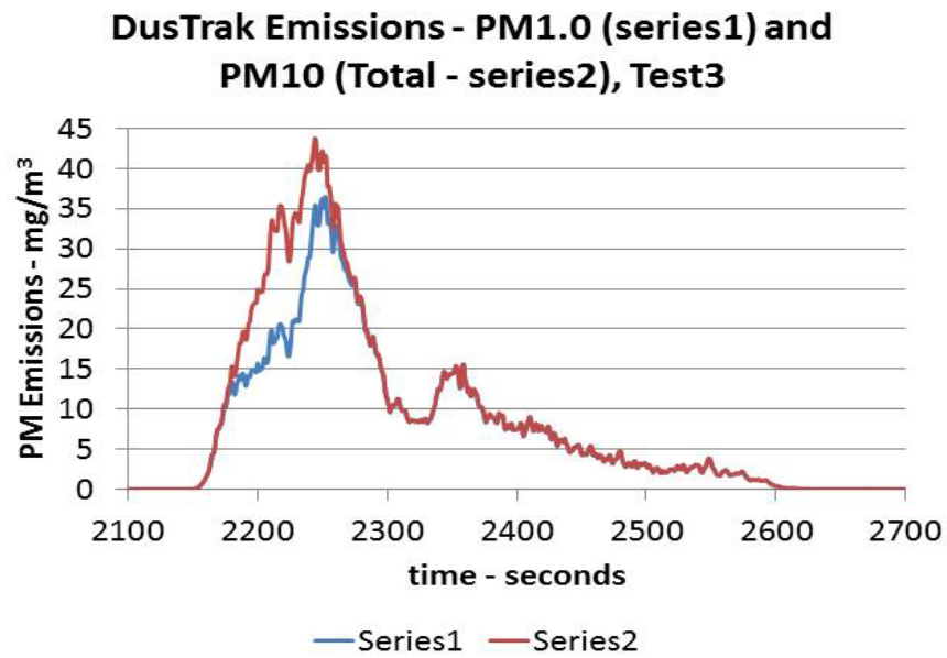
Figure III-21 PM1.0 and Total Emissions from the DusTrak during the high emission part of the regeneration event. Test3
