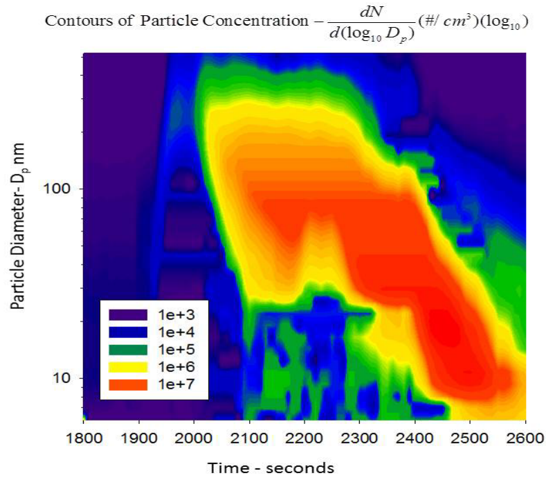
Figure III-5 Expanded view of EEPS particle number concentration emissions during the initial part of the regeneration event. Test1(a)
