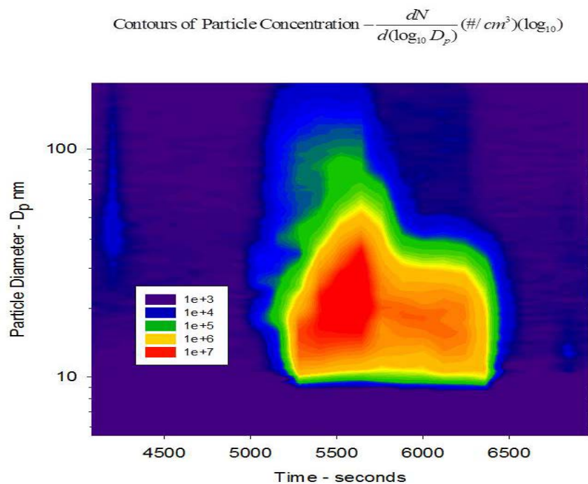
Figure III-40 SMPS particle number concentration emissions during three regeneration events. Test5(a)
