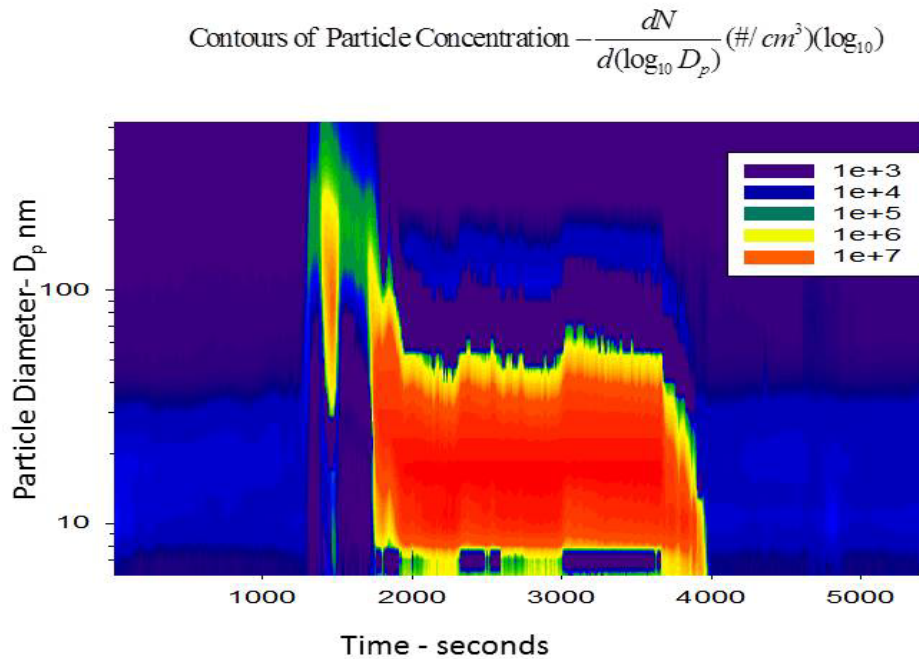
Figure III-22 EEPS particle number concentration emissions during the regeneration event. Test3
