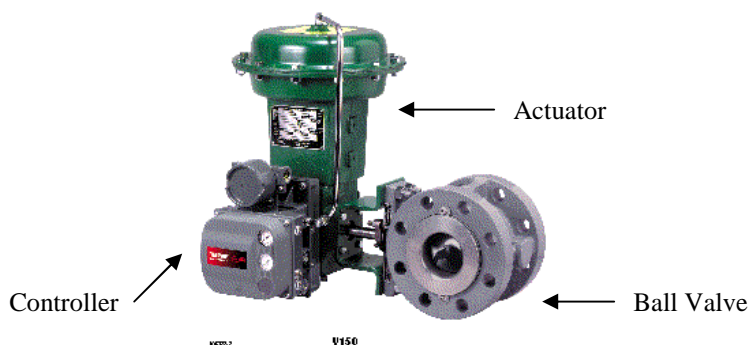
Figure 1. Typical Vee-Ball® Valves with Type 1052 Actuators and DVC6020 Digital Valve Controllers.
