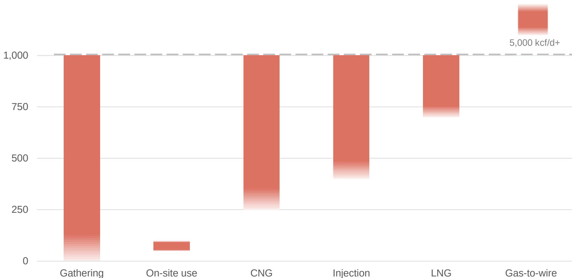
Range of optimal flare capture by abatement method* kcf/d
