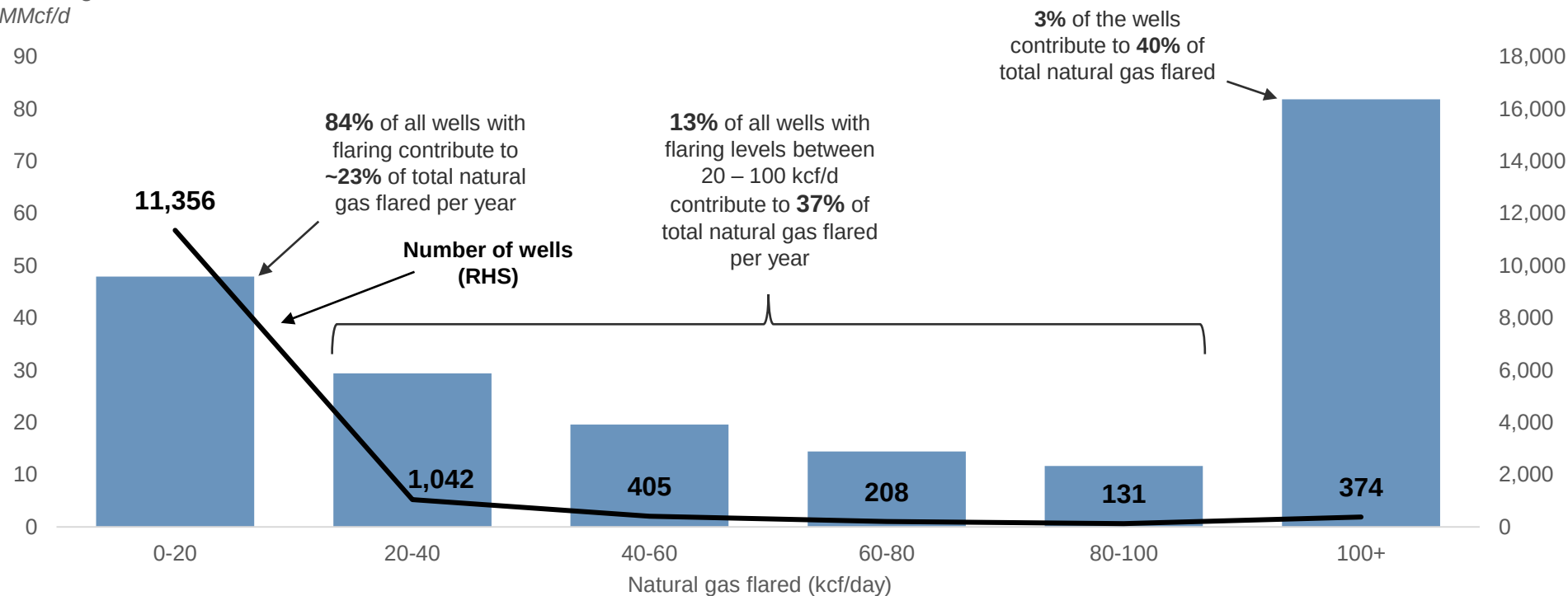
Total natural gas burned in H1 2021, split by amount burned per day on a well level
