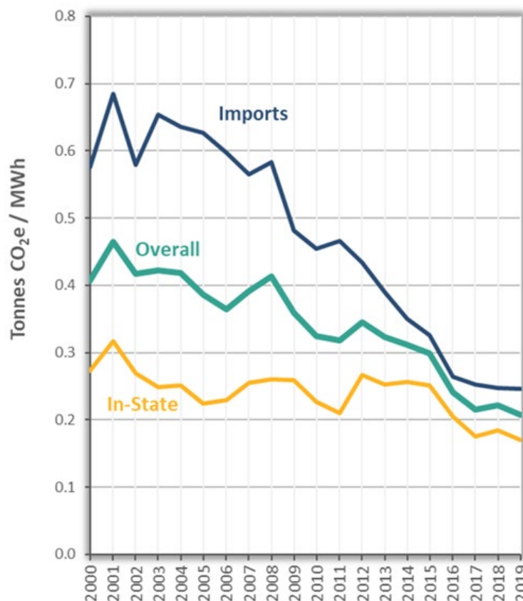
Figure 9. GHG Intensity of Electricity.
