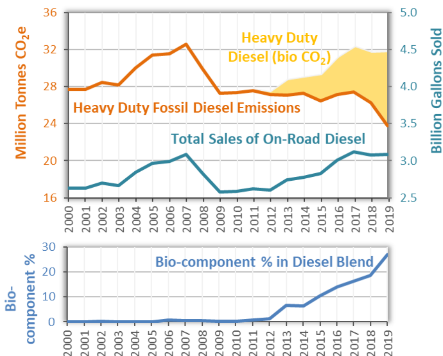
Figure 7. Trends in On-Road Diesel Vehicle Emissions.
