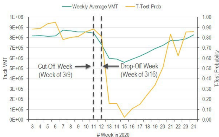
Figure C.17 Truck VMT and aggregated t-test probability. Large drop-off VMT and t-test probability values suggest that traffic volume decreased significantly away from typical conditions.
