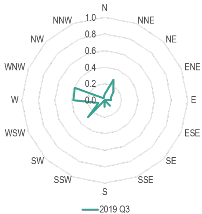
Figure C.28 Quarterly CPF for Biogenic Factor 1. The wind directions were associated with Factor contributions > 75th percentile.
