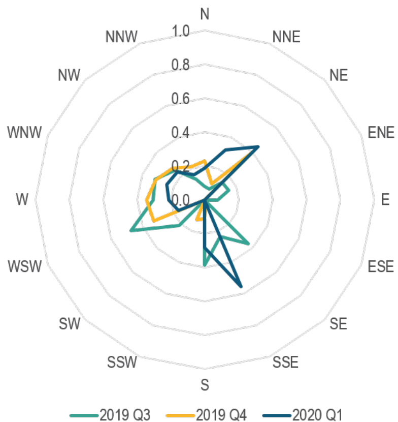
Figure C.19 Quarterly CPF for Mobile Source Factor 2. The wind directions were associated with Factor contributions > 75th percentile.
