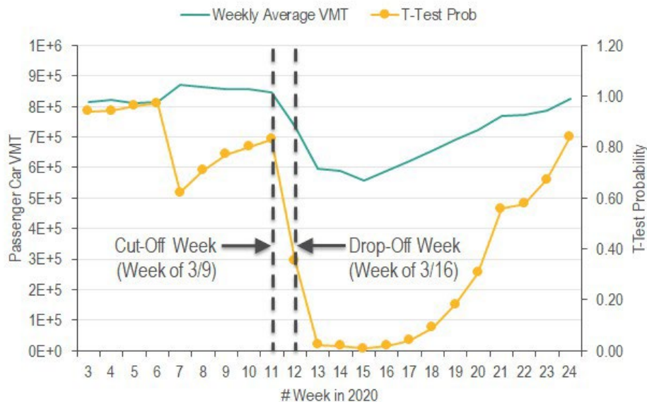
Figure C.16 Passenger car VMT and aggregated t-test probability. Large drop-off VMT and t-test probability values suggest that traffic volume decreased significantly away from typical conditions.
