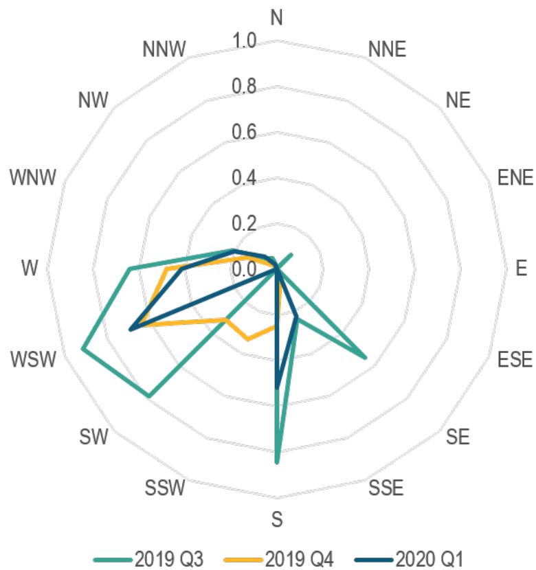
Figure C.22 Quarterly CPF for O&G Operation Factor 1. The wind directions were associated with Factor contributions > 75th percentile.
