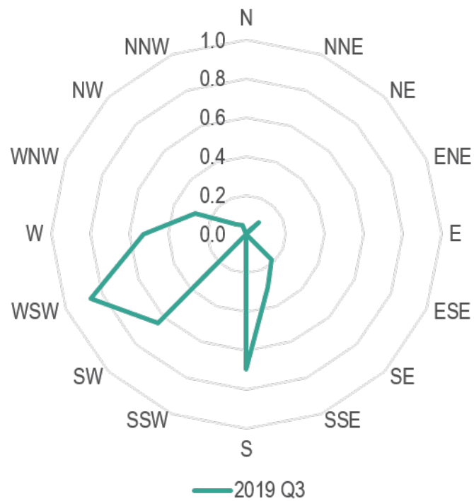
Figure C.26 Quarterly CPF for O&G Operation Factor 5. The wind directions were associated with Factor contributions > 75th percentile.
