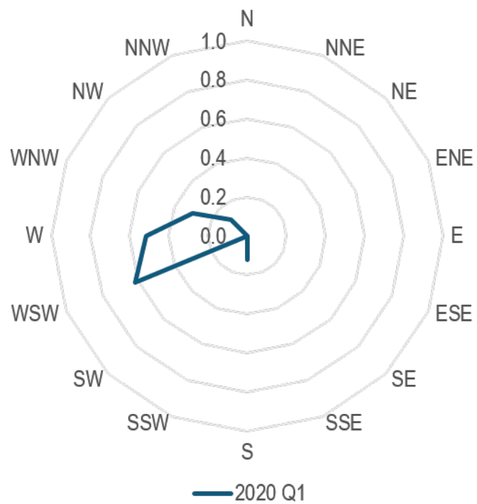
Figure C.27 Quarterly CPF for O&G Operation Factor 6. The wind directions were associated with Factor contributions > 75th percentile.
