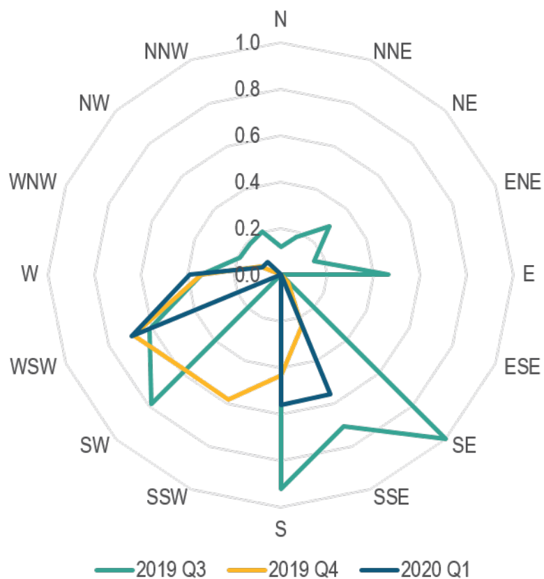
Figure C.24 Quarterly CPF for O&G Operation Factor 3. The wind directions were associated with Factor contributions > 75th percentile.
