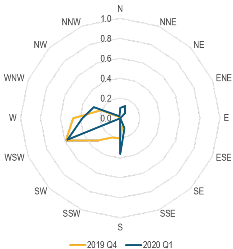
Figure C.25 Quarterly CPF for O&G Operation Factor 4. The wind directions were associated with Factor contributions > 75th percentile.
