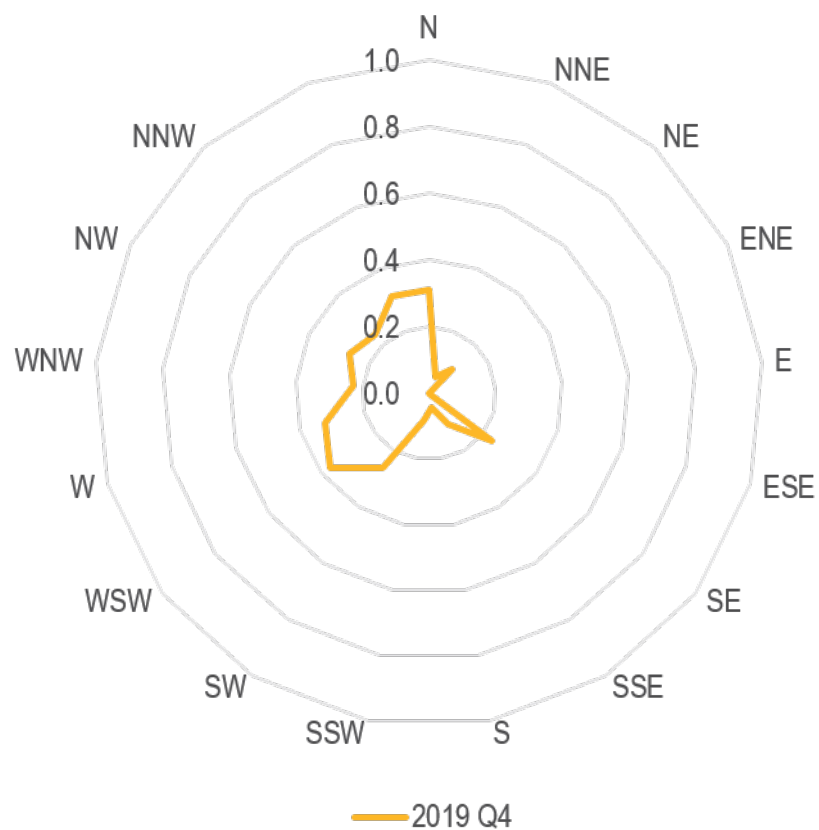
Figure C.21 Quarterly CPF for Mobile Source Factor 4. The wind directions were associated with Factor contributions > 75th percentile.
