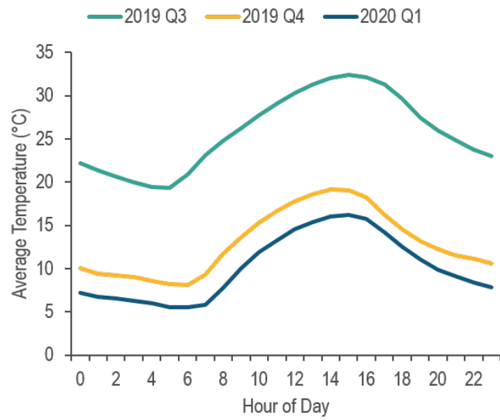
Figure C.15 Diurnal average temperature change in each quarter of SNAPS ambient air monitoring at Lost Hills, CA.
