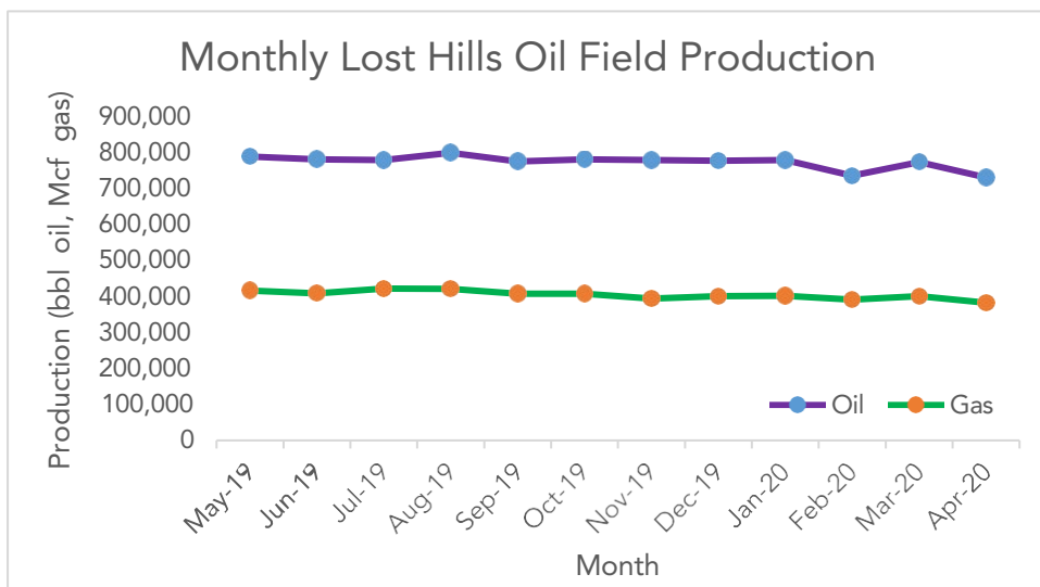
Figure C.4 O&G production between May 2019 and April 2020 on the Lost Hills Oil Field.
