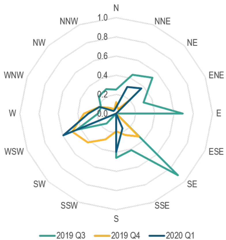
Figure C.18 Quarterly CPF for Mobile Source Factor 1. The wind directions were associated with Factor contributions > 75th percentile.
