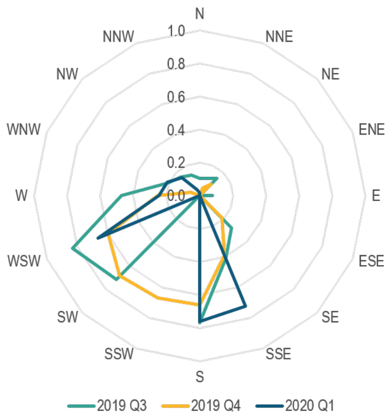
Figure C.23 Quarterly CPF for O&G Operation Factor 2. The wind directions were associated with Factor contributions > 75th percentile.
