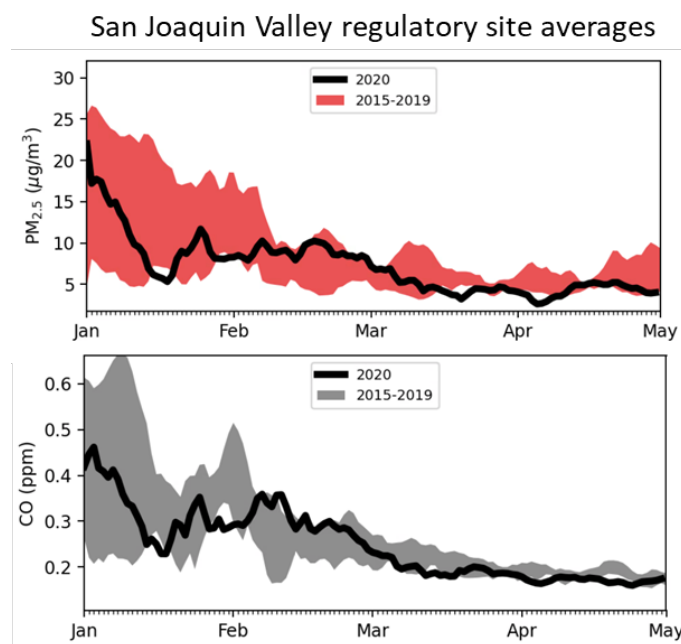
Figure 3.13 Average PM 2.5 and carbon monoxide (CO) concentrations at San Joaquin Valley regulatory sites in 2020 (black lines) compared to 2015-2019 (shaded areas).
