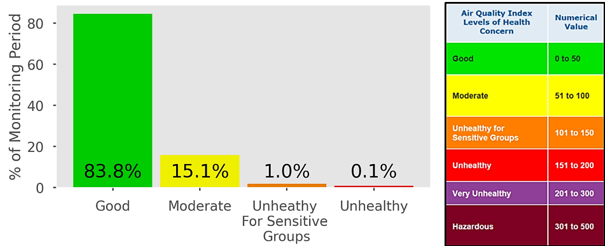
Figure 3.5 The Air Quality Index (AQI) in Lost Hills during the SNAPS monitoring period (May 2019 – April 2020), based on a rolling 24-hr average for PM 2.5 and rolling 8-hr average for O 3 .
