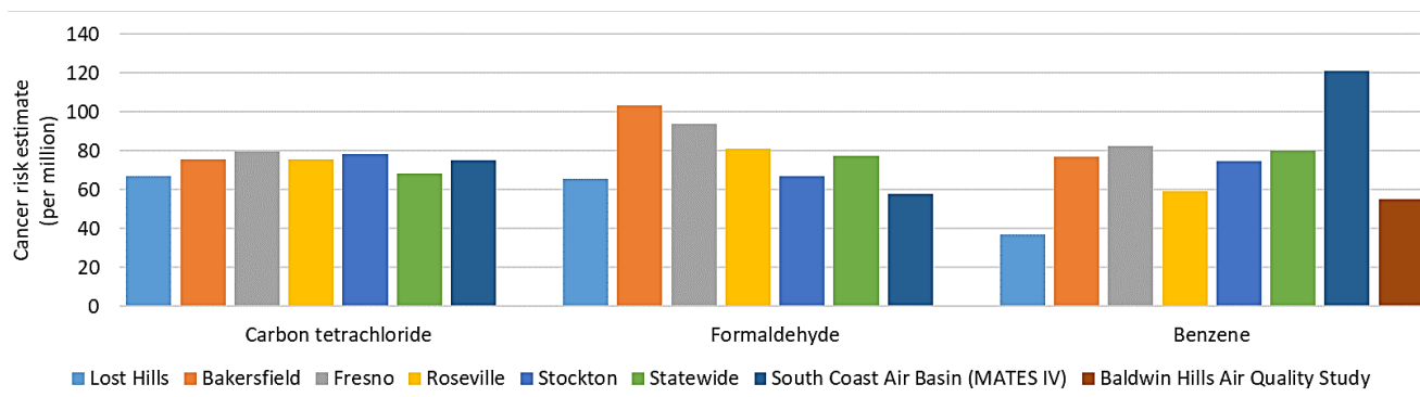
Figure 4.5 Cancer risk estimate comparisons for carbon tetrachloride, formaldehyde, and benzene based on average concentrations from: (1) SNAPS discrete data for Lost Hills (monitoring 2019-2020), (2) various Central Valley sites (CARB; monitoring 2016-2019 73 ), (3) Statewide (CARB; 2017 for formaldehyde and 2018 for carbon tetrachloride and benzene 73 ), (4) MATES IV air monitoring study of the South Coast Air Basin (monitoring 2012-2013) 118 , and (5) the Baldwin Hills Air Quality Study 33 (monitoring 2013; carbon tetrachloride not measured; formaldehyde data not reported). Cancer risks were estimated using the methods described in Appendix G.
