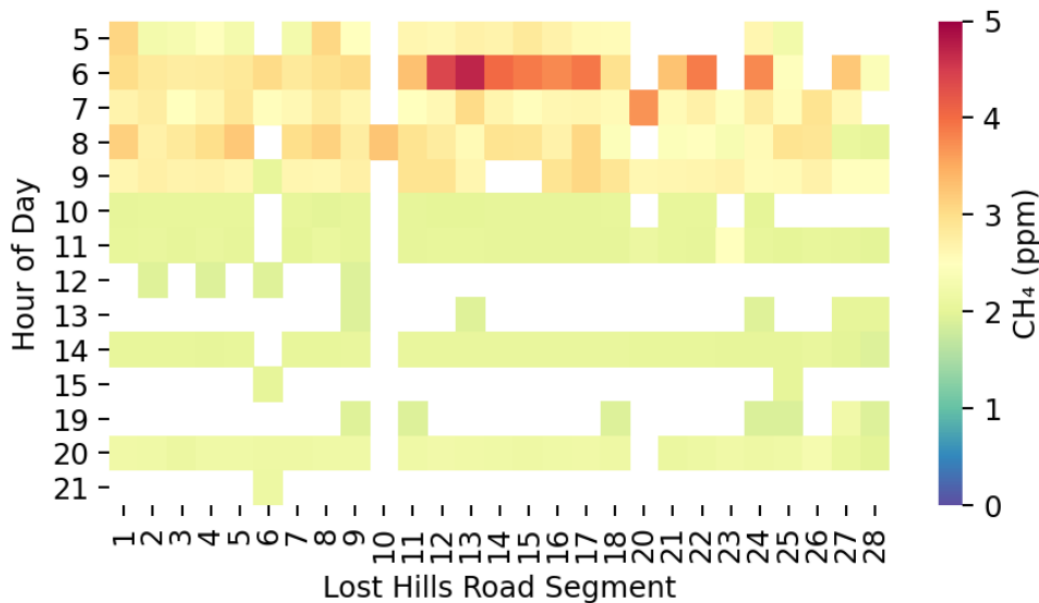
Figure 3.29 Heat map of methane concentrations as a function of segment (Table 3.4) and hour of day averaged over all mobile monitoring runs.
