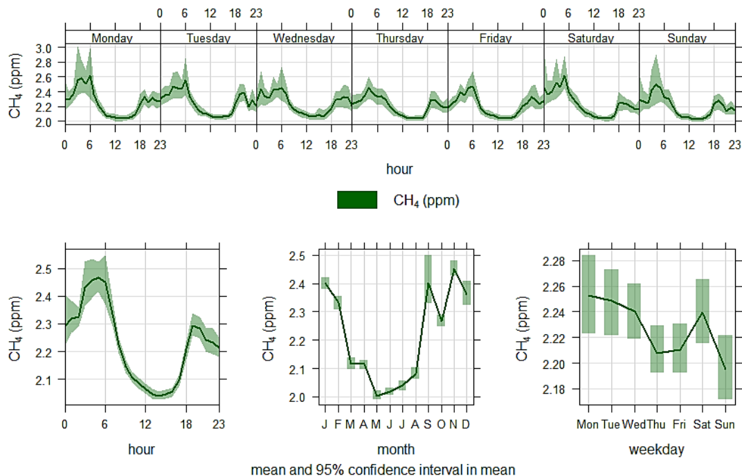
Figure 3.8 Time variation plot 58 for methane, including hourly, daily, and monthly pollutant trends. The solid line denotes the average pollutant concentration, while the shading indicates the potential range in the average.
