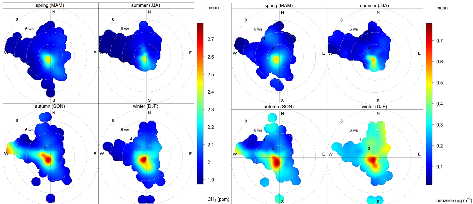
Figure 3.25 Seasonal polar plots for methane (left) and benzene (right). Successively increasing wind speeds are shown further out from the center of each plot, with the average concentration of each pollutant at that specific wind speed and wind direction shaded according to the keys on the right. Each box represents average concentrations during the corresponding Season (Spring – top left, Summer – top right, Fall – bottom left, Winter – bottom right).
