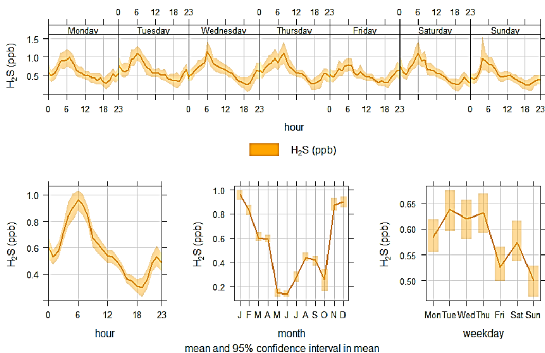
Figure 3.9 Time variation plot 58 for hydrogen sulfide, including hourly, daily, and monthly pollutant trends. The solid line denotes the average pollutant concentration, while the shading indicates the potential range in the average.
