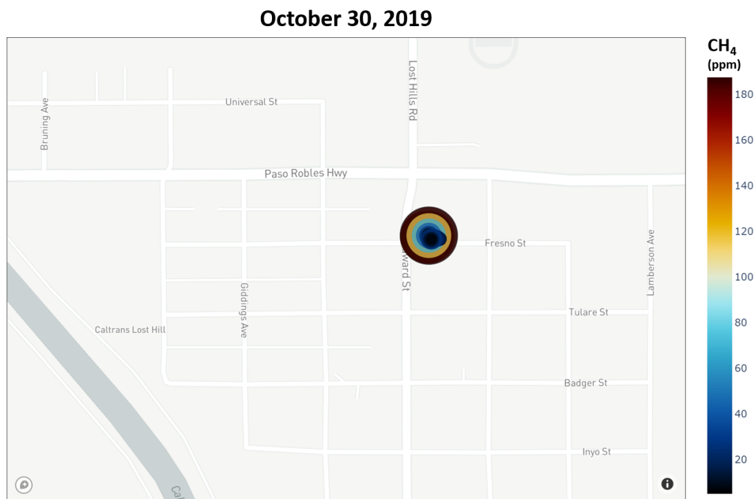
Figure 3.30 Natural gas leaks detected during the October 30, 2019 mobile monitoring campaign. Top: Time series, with methane leaks denoted by the pink dots. Bottom: Map with corresponding leak locations (dot size increases as concentration increases). In this instance, the instrument was removed from the platform to sample while walking the sidewalk.
