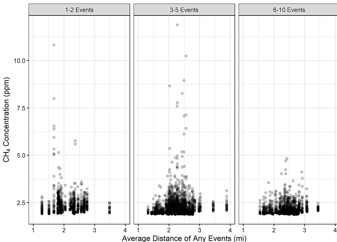
Figure 3.20 Distance of operator events from the SNAPS trailer vs measured methane concentration. Each individual box represents a specific range in number of operator events on a given day.
