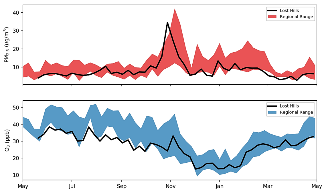
Figure 3.4 Seven-day average of PM 2.5 (top) and O 3 (bottom) at the Lost Hills monitoring site (black line) and the range for other sites in the region (shaded area). PM 2.5 and O 3 regional data include 10 sites from the Central Valley (Manteca, Tracy, Modesto, Turlock, Visalia, Hanford, Corcoran, Porterville, Oildale, and Bakersfield).
