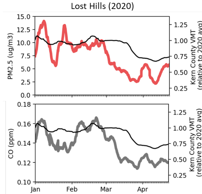
Figure 3.14 PM 2.5 and carbon monoxide (CO) concentrations in Lost Hills from January to April 2020. The thinner black lines denote the Kern County VMT (vehicle miles traveled).
