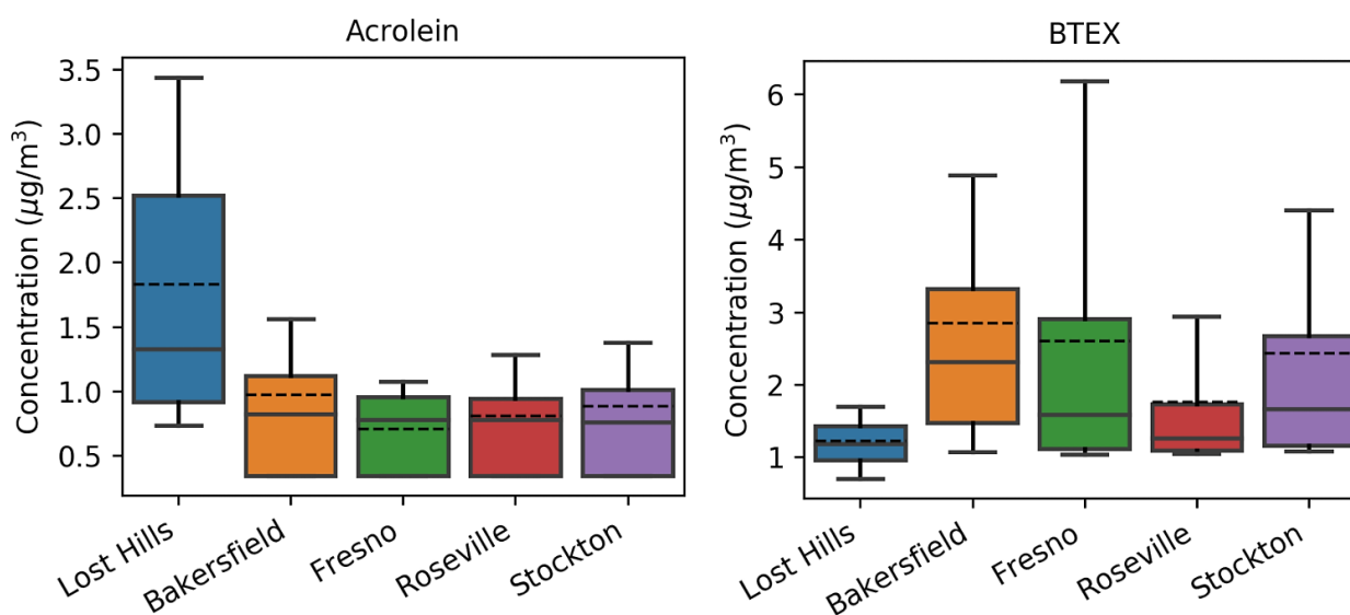
Figure 3.16 Concentrations of acrolein (left) and BTEX (right) measured in Lost Hills vs. at four regional sites in the Central Valley. Lost Hills data are from SNAPS monitoring equipment from 2019-20. Data for regional sites are from the iADAM dataset 73 for the years 2016-19. The median concentration at each site is denoted by individual solid lines within each box while the mean (average) concentration is denoted by individual dashed lines within each box.
