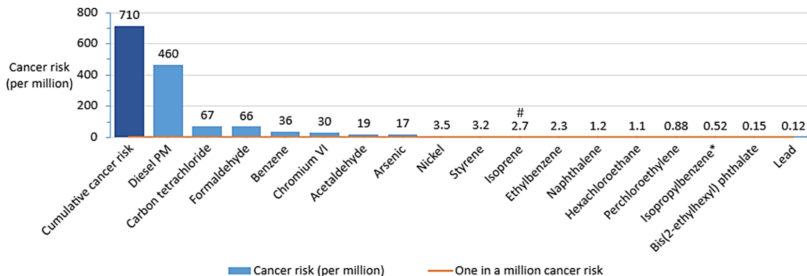
Figure 4.4 Cancer risk estimates for carcinogens measured in Lost Hills air. Cumulative cancer risk (dark blue, leftmost bar) and cancer risk estimates for each compound (lighter blue bars) are arranged by cancer risk in decreasing order. The orange horizontal line represents one in a million cancer risk, which is a threshold of concern for cancer among the general population. *Indicates that the health guidance value used to calculate risk for isopropylbenzene is provisional (not derived by OEHHA). #Indicates that isoprene is likely from biogenic sources.
