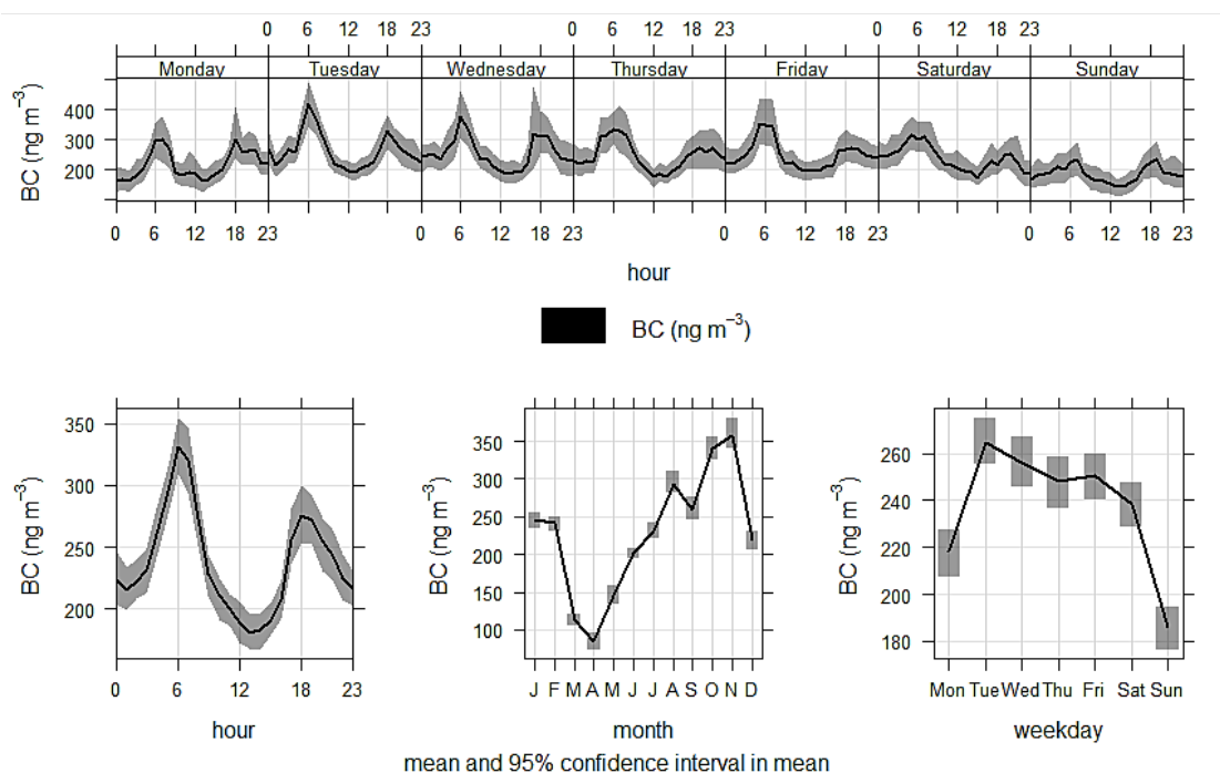
Figure 3.10 Time variation plot 58 for black carbon, including hourly, daily, and monthly pollutant trends. The solid line denotes the average pollutant concentration, while the shading indicates the potential range in the average.
