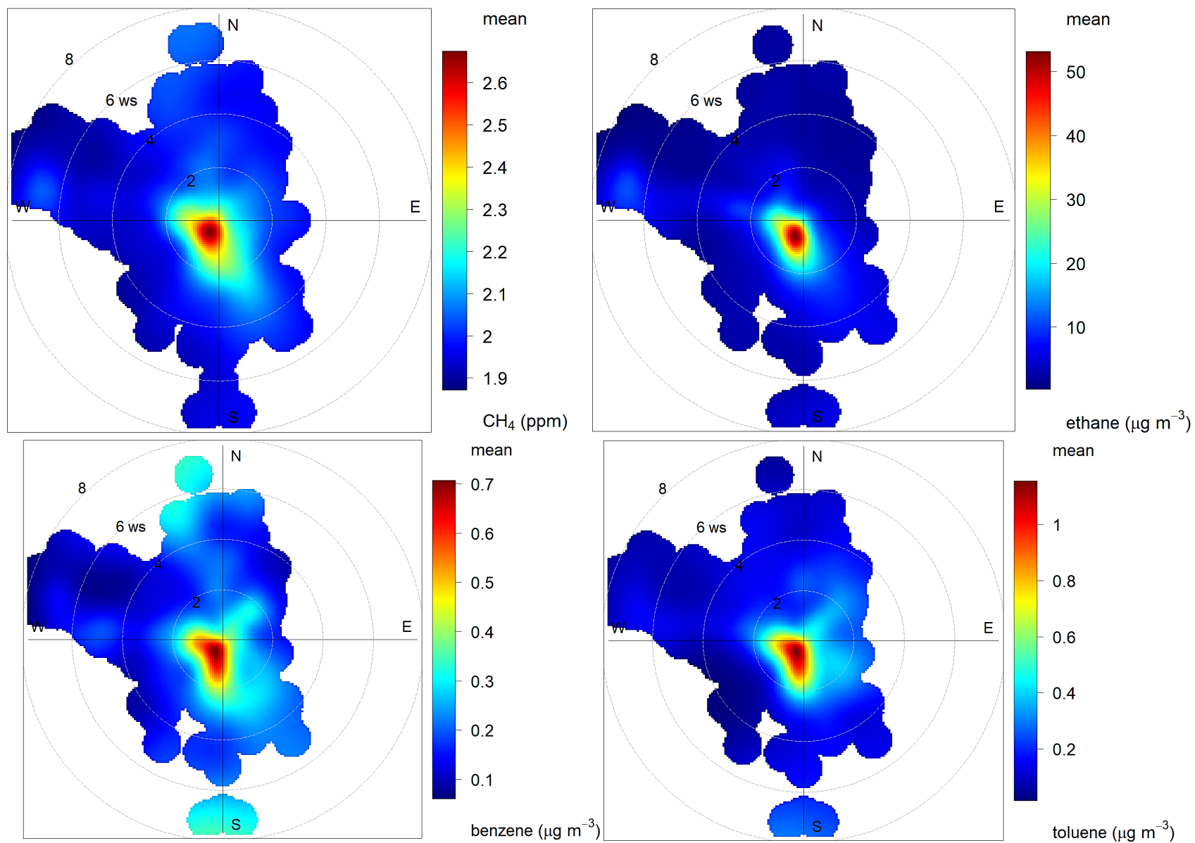
Figure 3.23 Polar plots 58 for methane, ethane, benzene, and toluene. Successively increasing wind speeds are shown further out from the center of each plot, with the average concentration of each pollutant at that specific wind speed and wind direction shaded according to the keys on the right.
