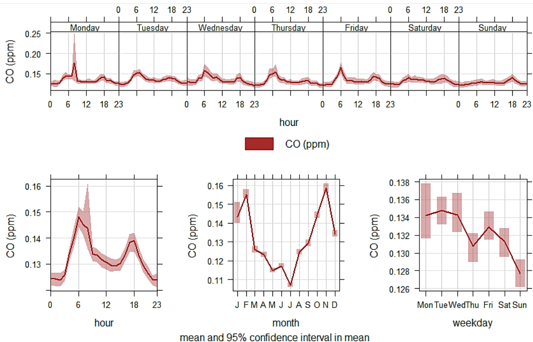
Figure 3.11 Time variation plot 58 for carbon monoxide, including hourly, daily, and monthly pollutant trends. The solid line denotes the average pollutant concentration, while the shading indicates the potential range in the average.
