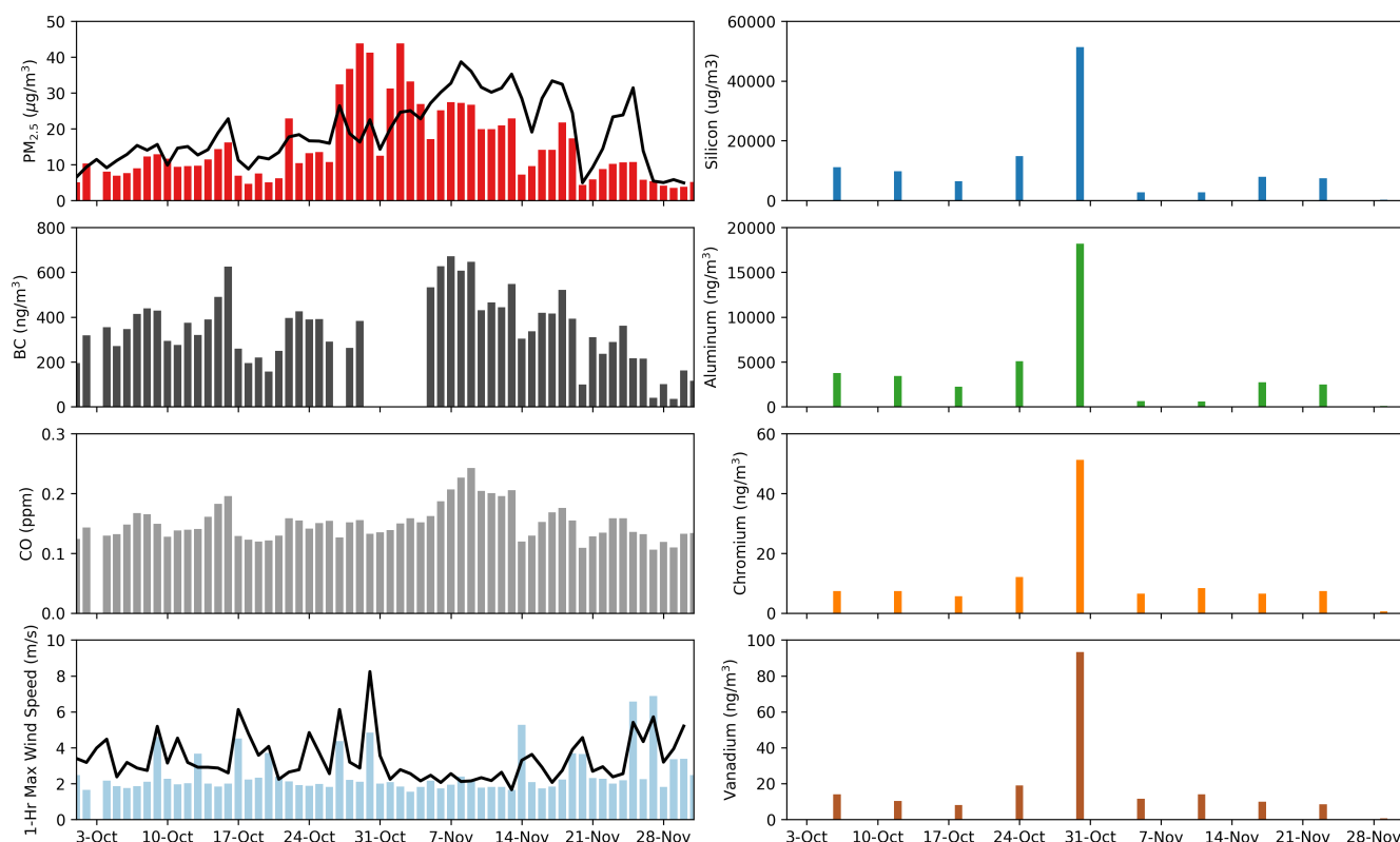
Figure 3.17 Selected Lost Hills 24-hr averages of 1-hr maximum wind speed (bottom left), pollutant (left), and metals (right) concentrations from October through November 2019, denoted by bars. Regional 24-hr average PM 2.5 concentrations and max 1-hr wind speeds (across all sites in Kern and Tulare counties) are denoted by black lines. Days with missing bars indicate that no measurement was made on that day.
