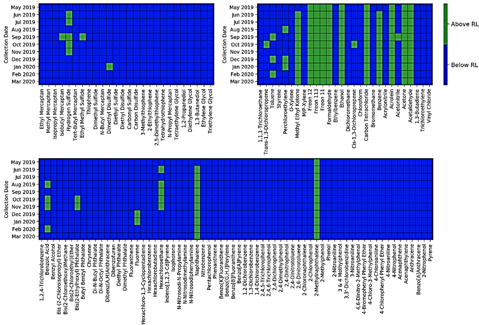
Figure 3.15 Graphic depicting compounds detected by laboratory methods above the reporting limit (RL) in green and those not detected in blue. Each cell represents the maximum of the 24-hourly canister samples taken in that month. Compounds are organized by retrieval methods, split into Glycols and Sulfur (top left), Monitoring and Lab Division (MLD) lab analyzed compounds (top right), and PAHs and other compounds (bottom).
