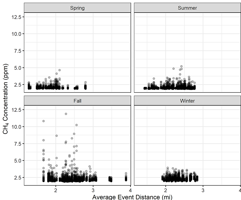
Figure 3.21 Distance of operator events from the SNAPS trailer vs methane concentration observed, separated by season (spring, summer, fall, and winter).
