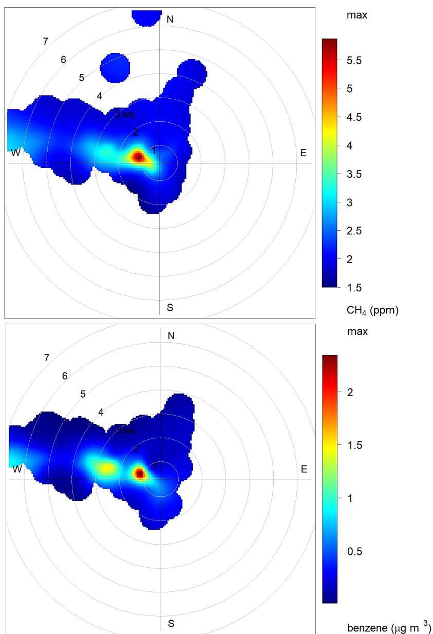
Figure 3.27 Polar plots 58 for methane and benzene, including dates from 9-16-2020 through
