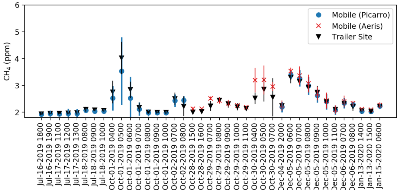
Figure 3.28 Time series of all available hours when the mobile platform made measurements within 1 square mile of Lost Hills. Vertical bars represent 1 standard deviation of the CH 4 concentrations measured within each hour for each instrument.
