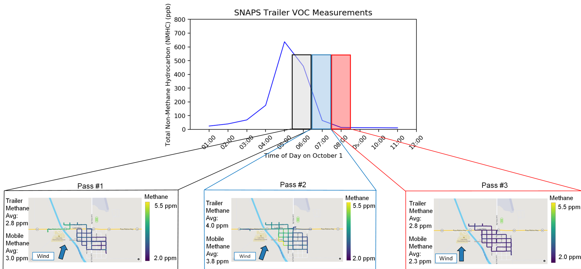
Figure 3.32 Summary of three routes during the morning of October 1, 2019 mobile monitoring run relative to the total non-methane hydrocarbon species measured at the SNAPS trailer.
