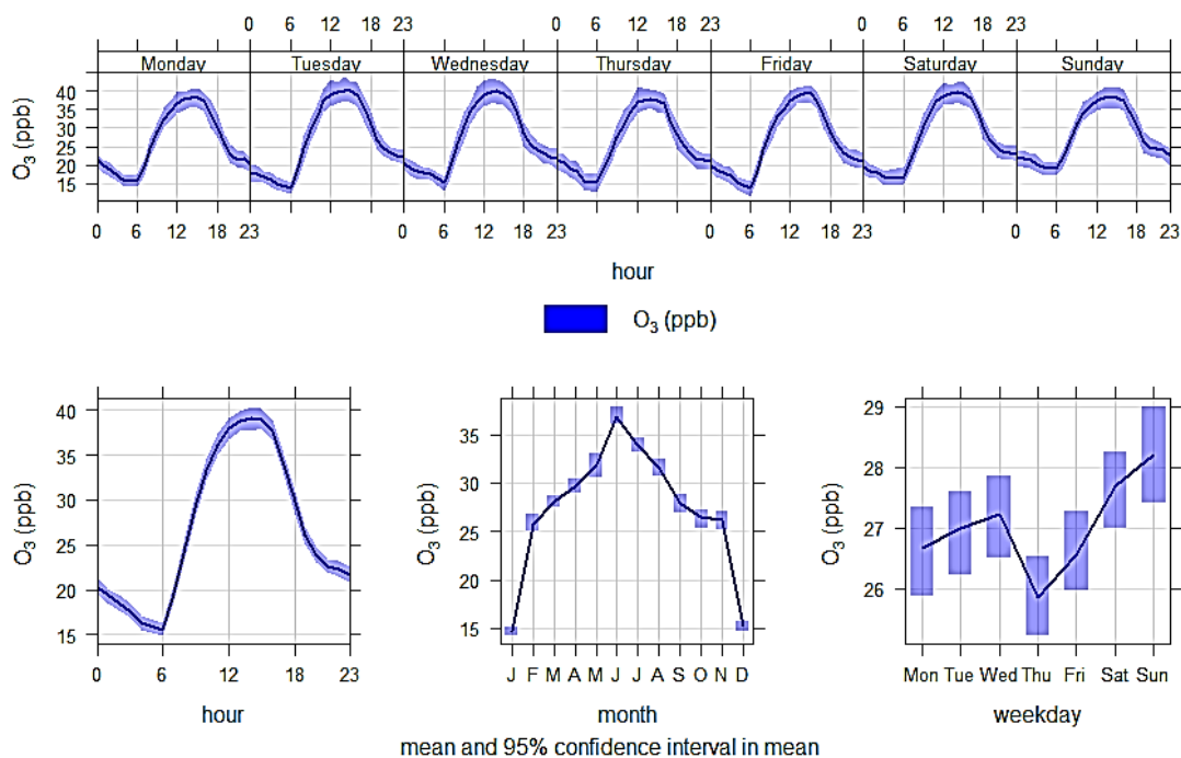
Figure 3.7 Time variation plot 58 for ozone, including hourly, daily, and monthly pollutant trends. The solid line denotes the average pollutant concentration, while the shading indicates the potential range in the average.
