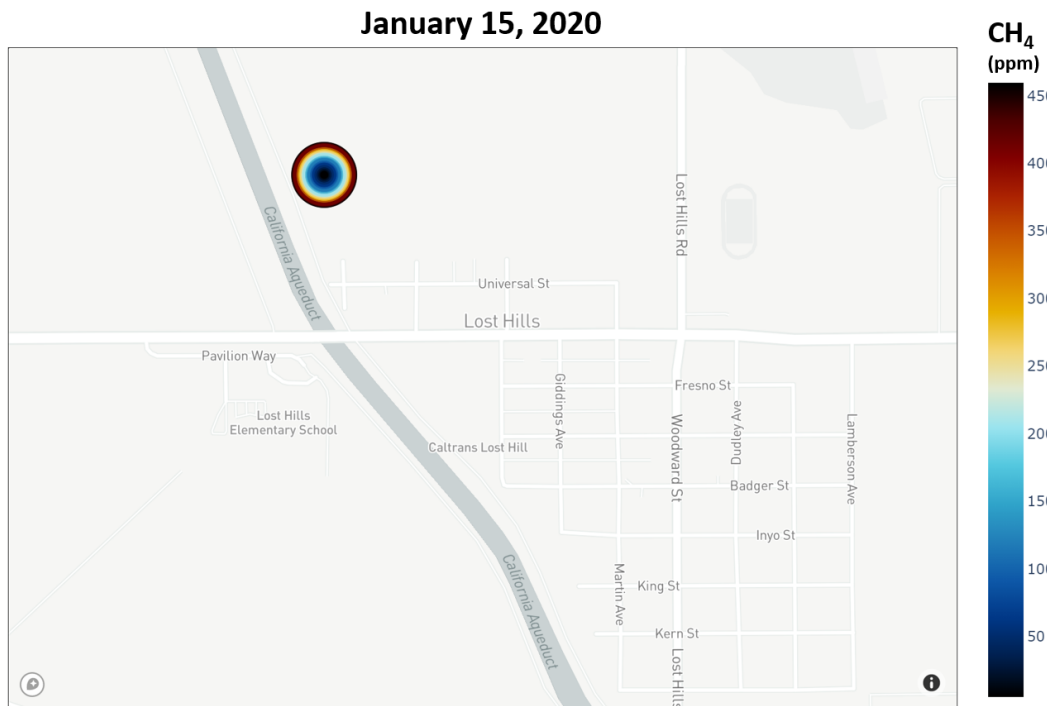
Figure 3.31 Natural gas leaks detected during mobile monitoring on January 15, 2020. Top: Time series, with methane leaks denoted by the pink dots. Bottom: Map with corresponding leak locations (dot size increases as concentration increases).
