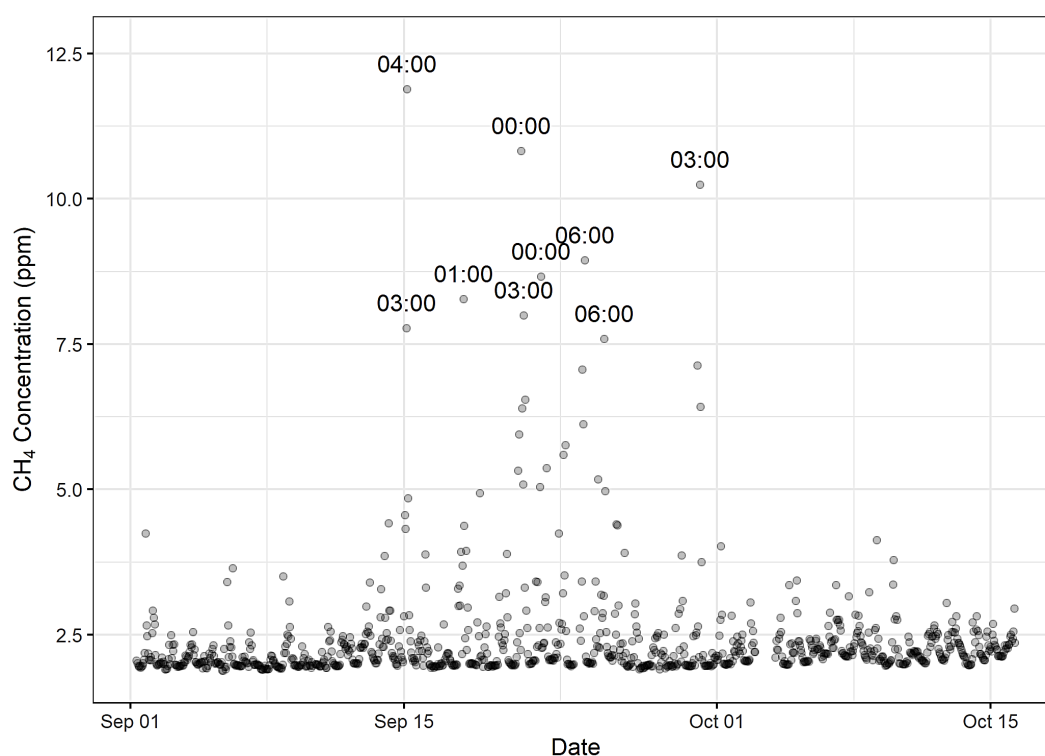
Figure 3.22 Hourly methane concentrations from September 2019 to mid-October 2019 at the SNAPS trailer. The labels on the higher concentration circles are the time of the measurements.
