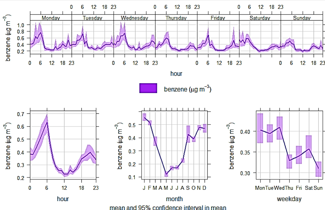
Figure 3.12 Time variation plot 58 for benzene, including hourly, daily, and monthly pollutant trends. The solid line denotes the average pollutant concentration, while the shading indicates the potential range in the average.
