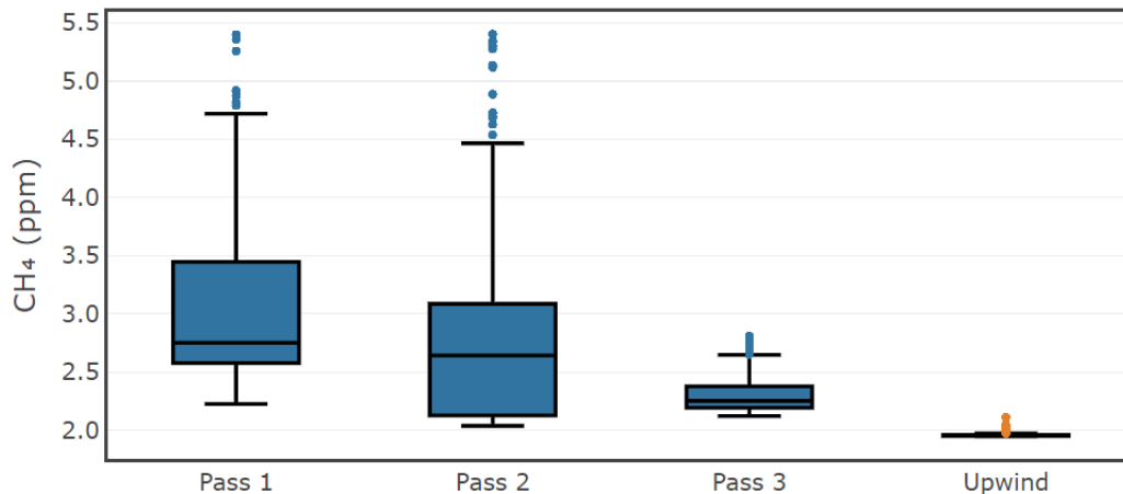
Figure 3.33 Box and whisker plot showing the distribution of methane concentrations on October 1, 2019 during three passes beginning at 5:25, 6:25, and 7:39 AM. Upwind/background measurements were taken west of Lost Hills at 11:00 AM on October 1.
