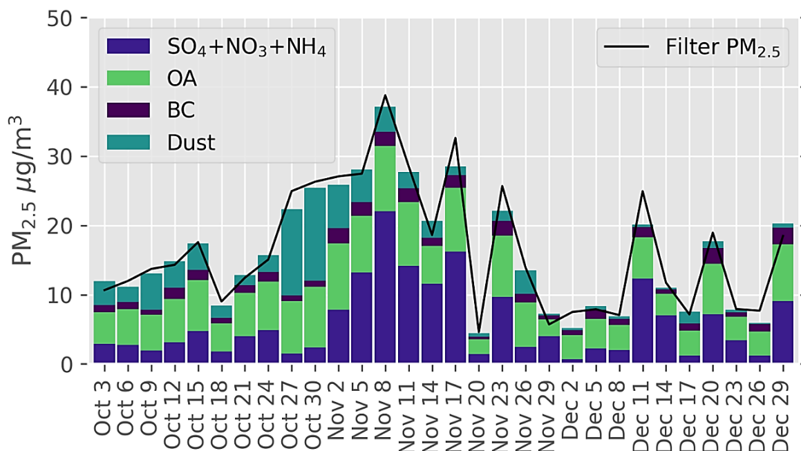
Figure 3.18 PM 2.5 components derived from the Chemical Speciation Network sites at Bakersfield and Fresno. Inorganic (sulfate+nitrate+ammonium [ \text{SO}_4+\text{NO}_3+\text{NH}_4 ]), organic (OA), black carbon (BC) and dust components are shown with the filter PM 2.5 from independent filter measurements. Staff calculated OA from organic carbon and dust from metals measurements following Malm and Hand, 2007 85 .
