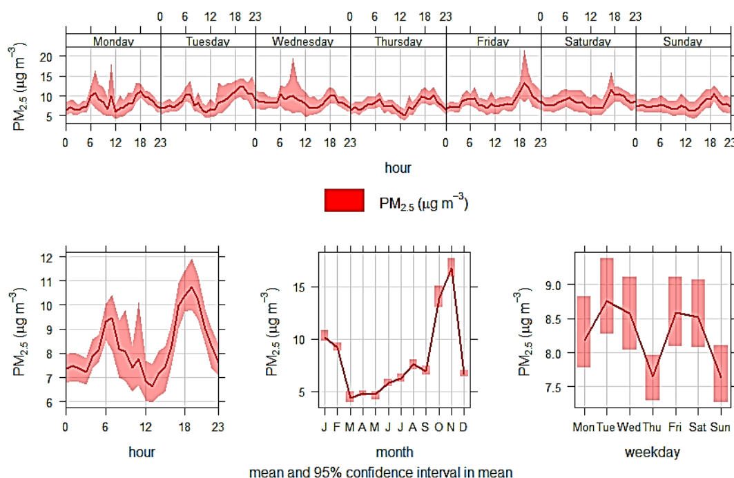
Figure 3.6 Time variation plot 58 for PM 2.5 , including hourly, daily, and monthly pollutant trends. The solid line denotes the average pollutant concentration, while the shading indicates the potential range in the average.
