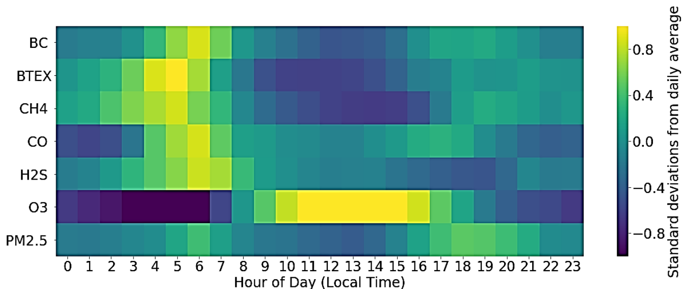
Figure 3.3 Heat map denoting the relative hourly concentrations of black carbon (BC); benzene, toluene, ethylbenzene, xylenes (BTEX); methane (CH 4 ); carbon monoxide (CO); hydrogen sulfide (H 2 S); ozone (O 3 ), and PM 2.5 .
