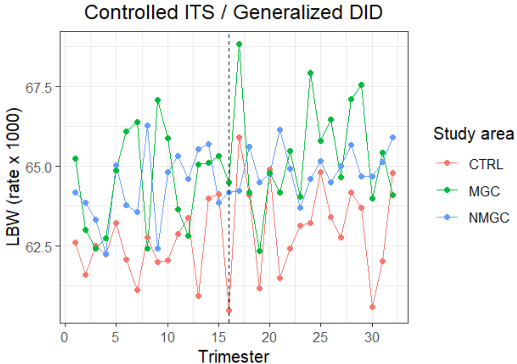
Figure 6. Temporal Trends in Low Birth Weight (LBW) Rates Across Study Areas Using Controlled Interrupted Time Series (Generalized DiD Analysis) Models
