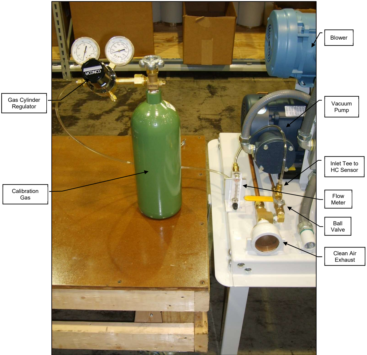
FIGURE 8-1 Equipment Configuration for Verifying Hydrocarbon Sensor Performance
