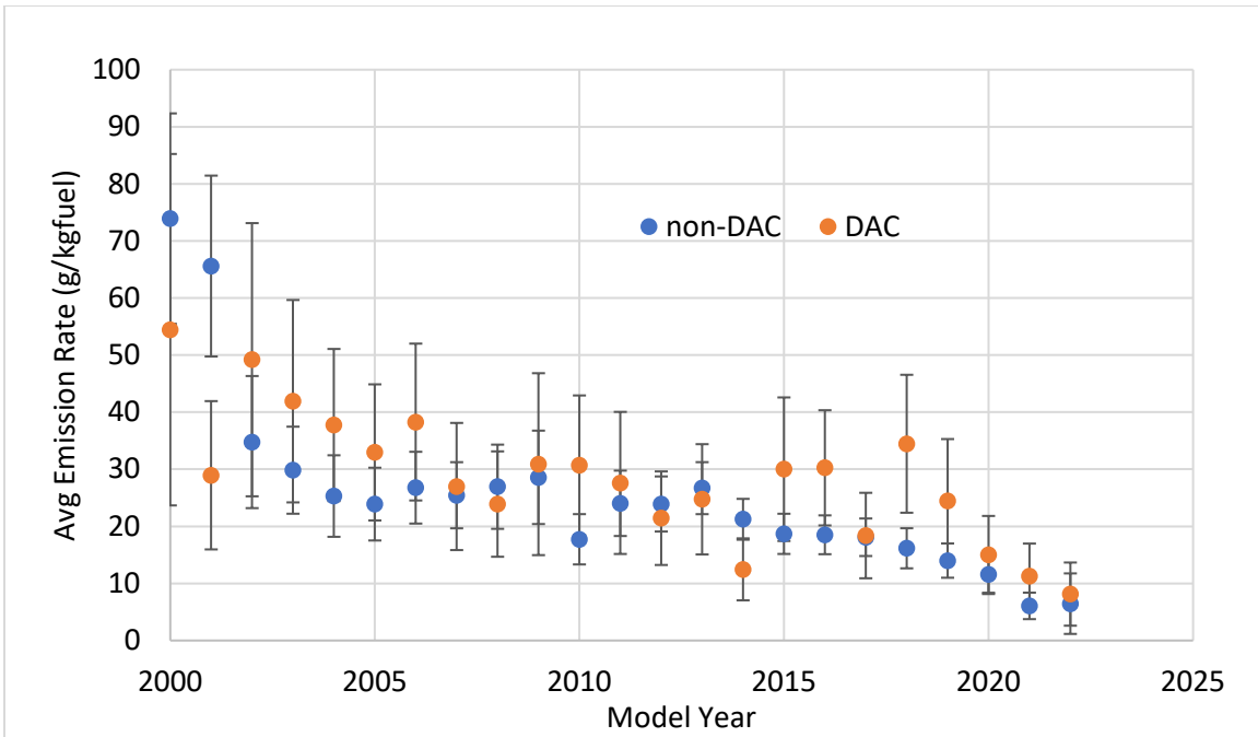
Figure 23. CO emission rates for non-DAC and DAC LDVs averaged by model year for the Oakland campaign. Error bars indicate 95% confidence intervals.
