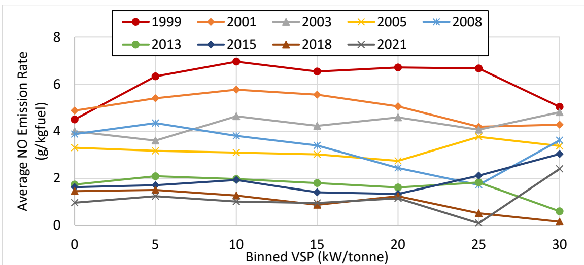
Figure 38. Average VSP-binned NO emission rates by measurement year
