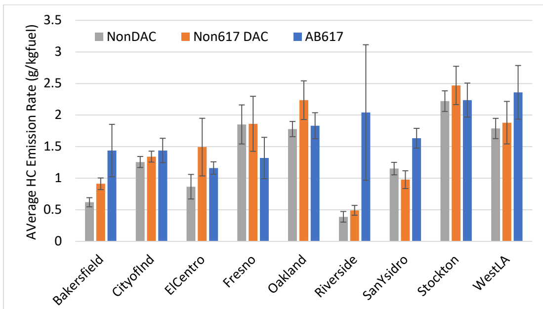
Figure 19. The average HC emission rates for non-DAC, AB617, and non-617 DAC by RSD campaign. Error bars indicate 95% confidence intervals.
