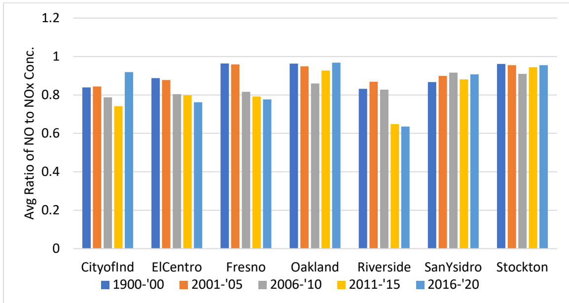
Figure 17. Average ratio of NO to NOx concentration for diesel-powered LDVs by model year bin and campaign.
