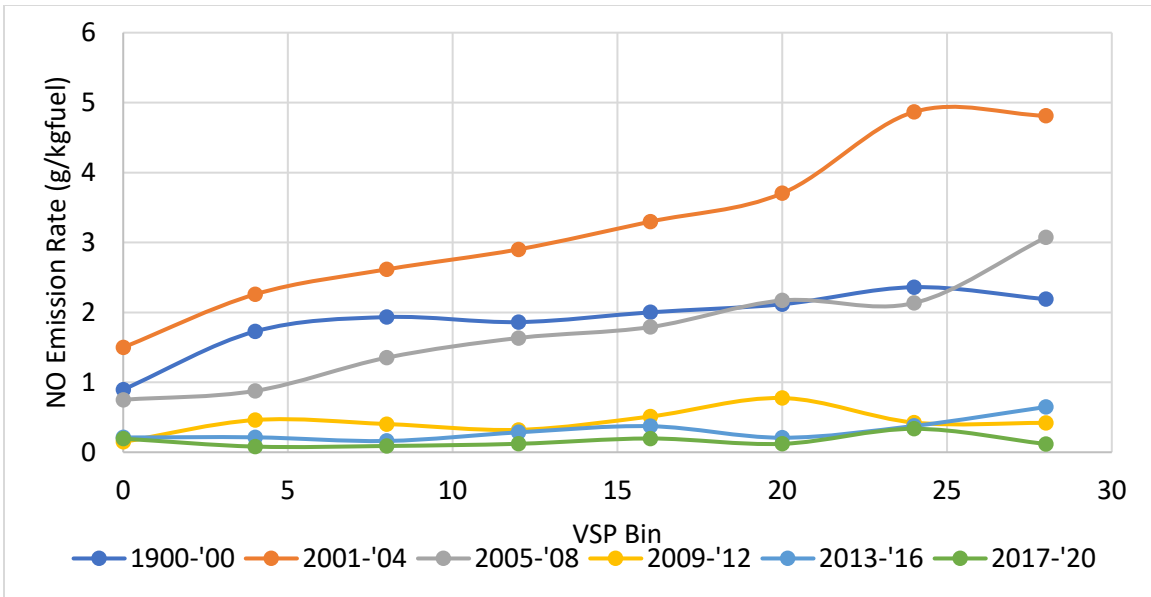
Figure 67. The trend in NO emission rate against VSP bin by model year bin for the City of Industry campaign.
