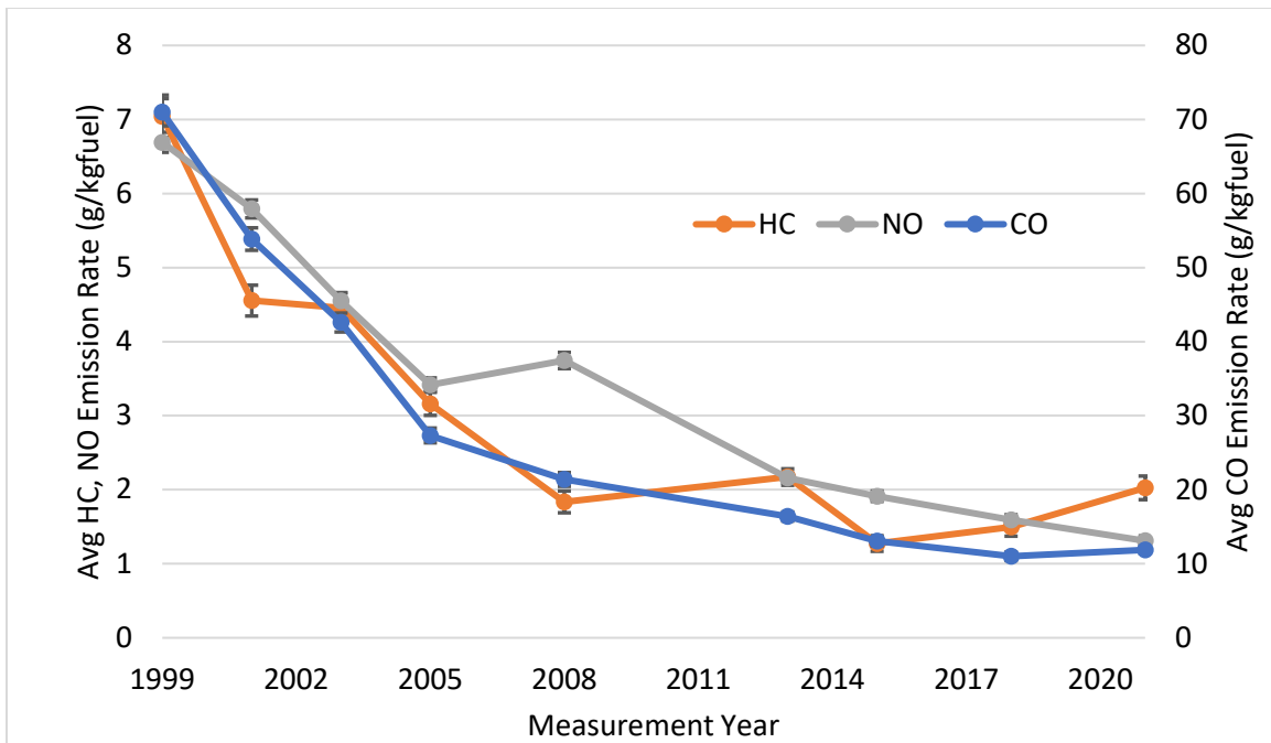
Figure 29. Overall average emissions measured at the La Brea Site by measurement year. Error bars indicate 95% confidence intervals.
