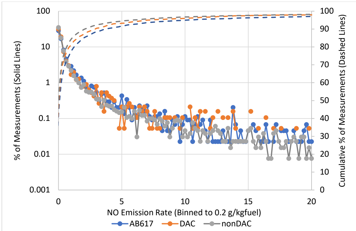
Figure 27. The distributions of NO emission rates for non-DAC, non-617 DAC, and AB617 community vehicles. Emission rates are binned to the nearest 0.2 g/gkfuel.
