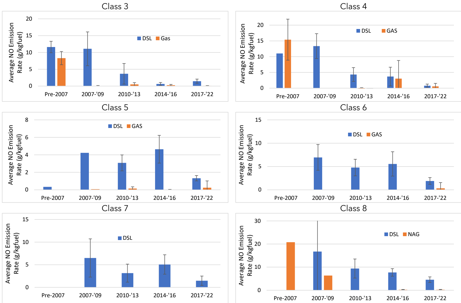
Figure 53. HDV average NO emission rates by model year, truck class and fuel type, for the City of Industry campaign
