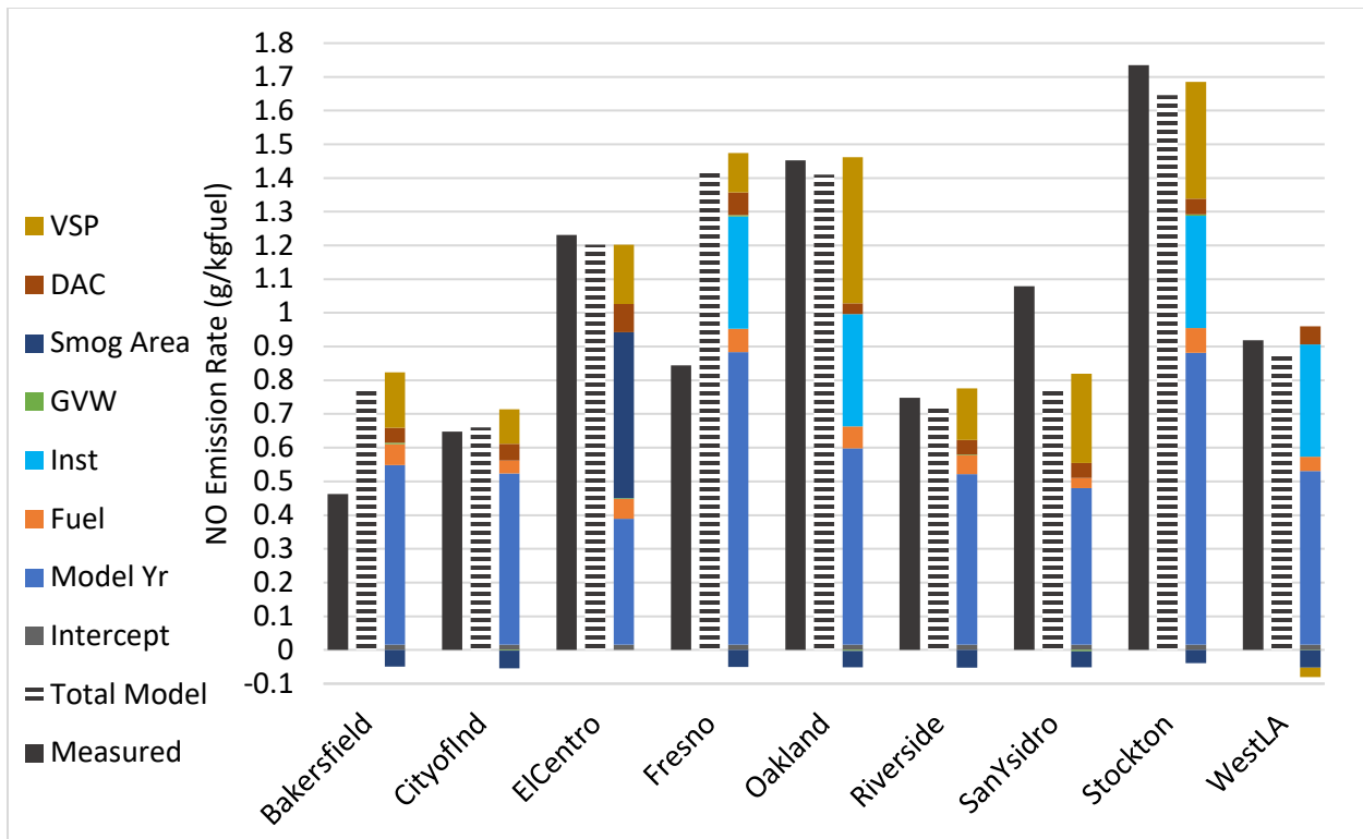
Figure 69. The campaign-average LDV NO emission rates as measured, as modeled, and separated into components for each quantifiable/categorical variable
