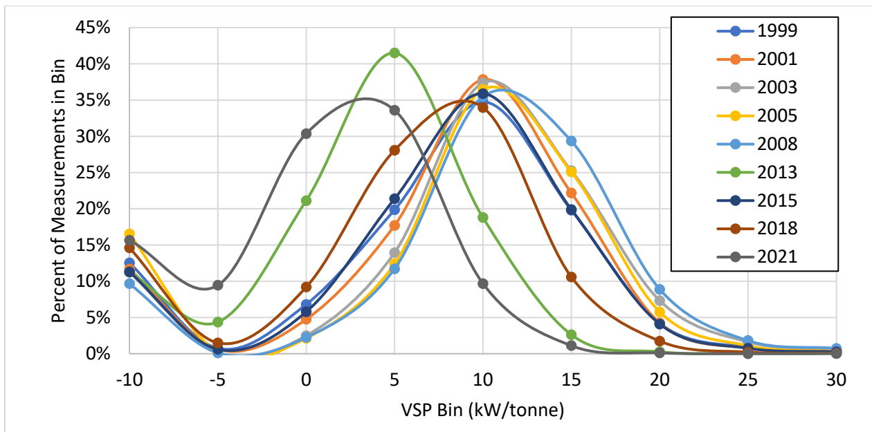
Figure 35. Distribution of estimated VSP in each measurement year.
