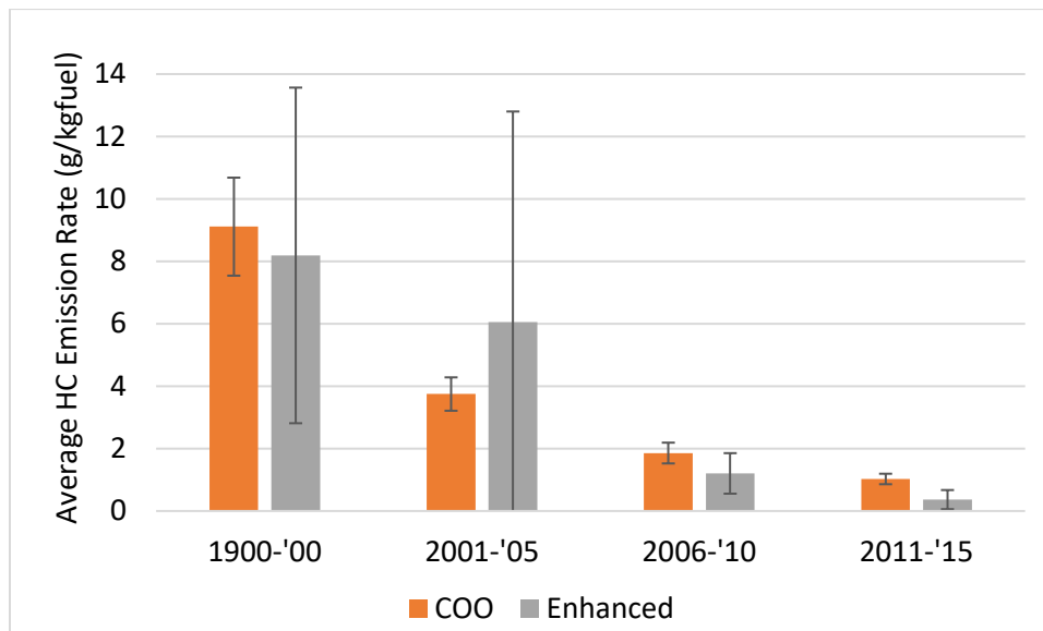
Figure 56. HC emission rate by model year bin for COO and Enhanced areas, averaged for gasoline vehicles observed at El Centro
