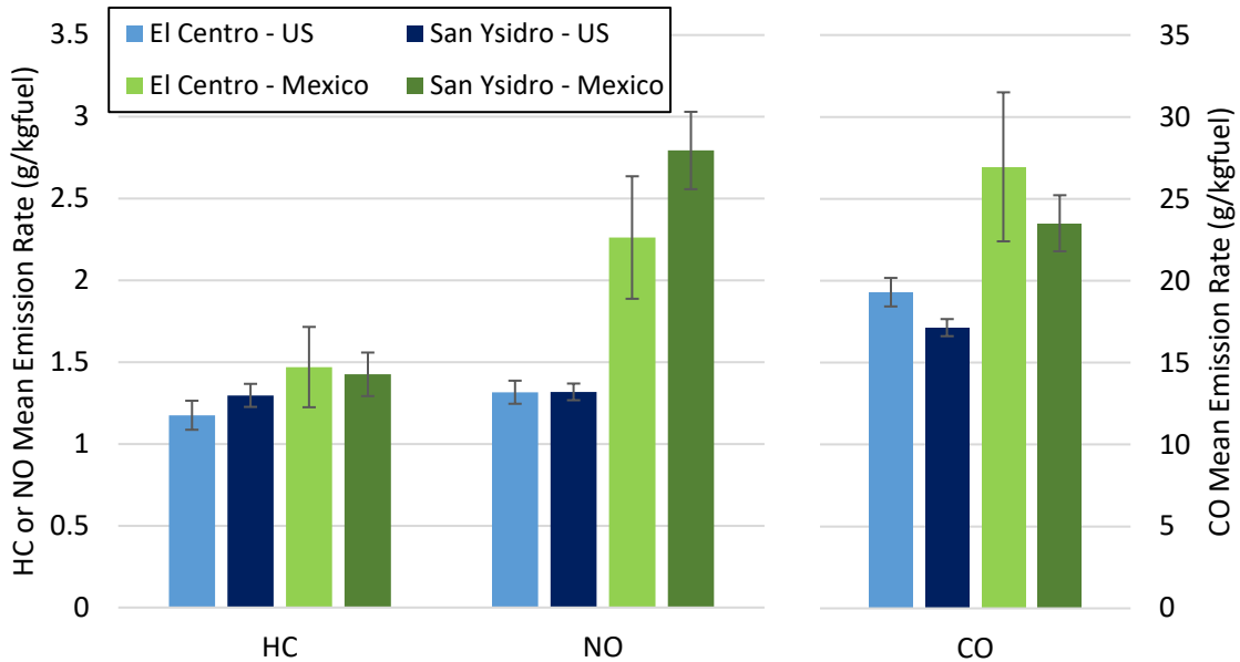
Figure 40. The average emission rates for the CA and Mexican fleets of vehicles at each border site. Error bars represent 95% confidence intervals.
