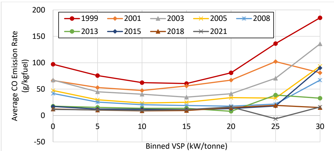
Figure 37. Average VSP-binned CO emission rates by measurement year
