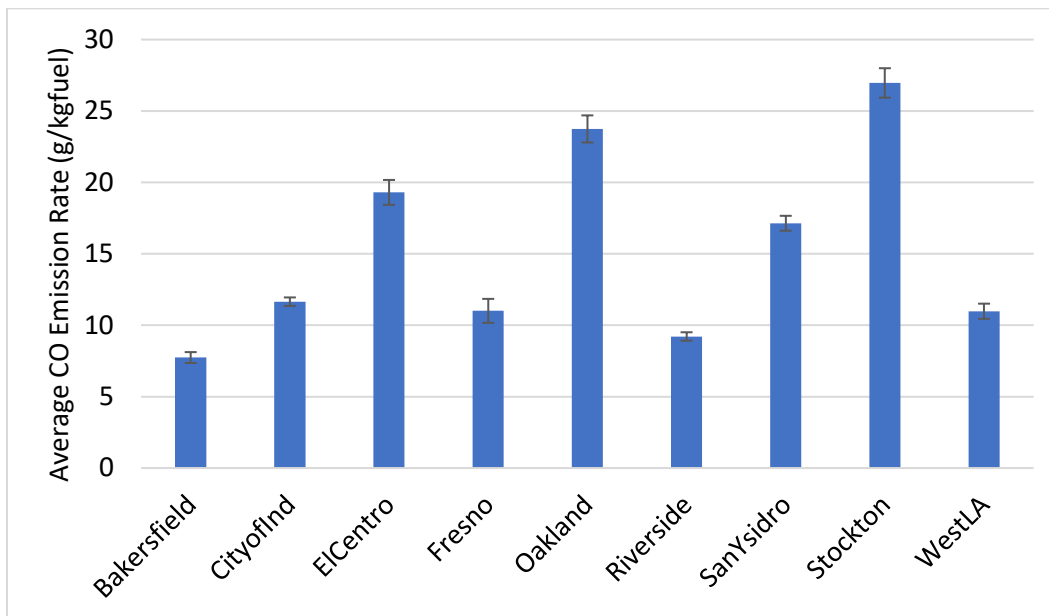
Figure 15. The average CO emission rate observed for all LDVs at each campaign. Error bars indicate 95% confidence interval.
