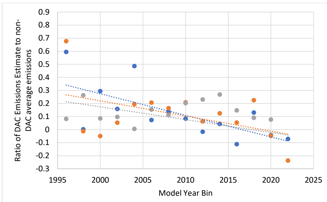
Figure 68. The ratio of the regression-modeled DAC status additive emission rate to the modeled non-DAC average emission rate by model year for each pollutant.
