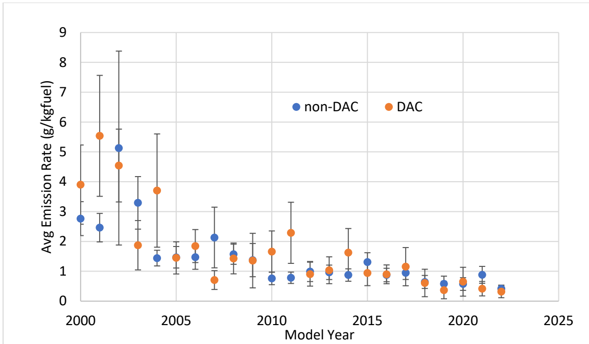
Figure 22. HC emission rates for non-DAC and DAC LDVs averaged by model year for the San Ysidro campaign. Error bars indicate 95% confidence intervals.
