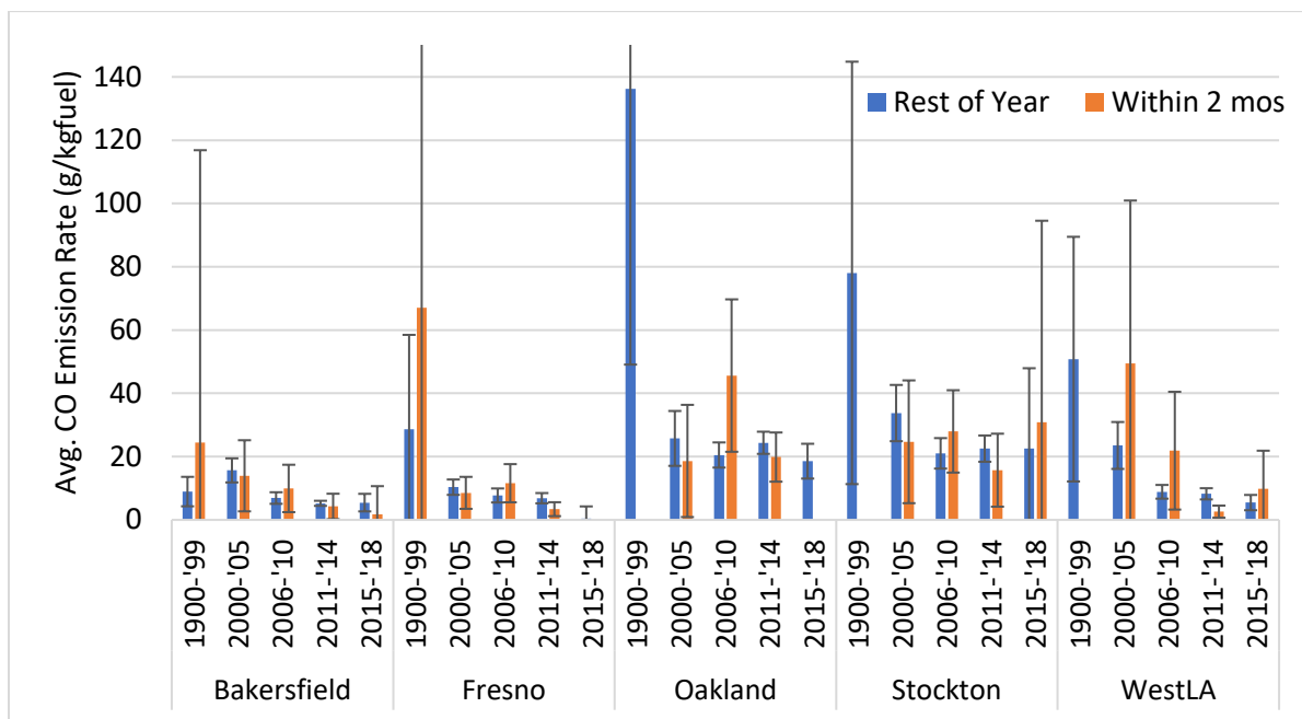
Figure 59. The average CO emissions of vehicles immediately following their Smog Check test as compared to all others by model year.
