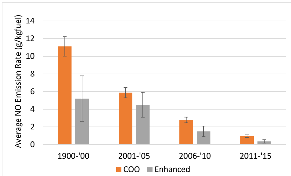
Figure 58. NO emission rate by model year bin for COO and Enhanced areas, averaged for gasoline vehicles observed at El Centro
