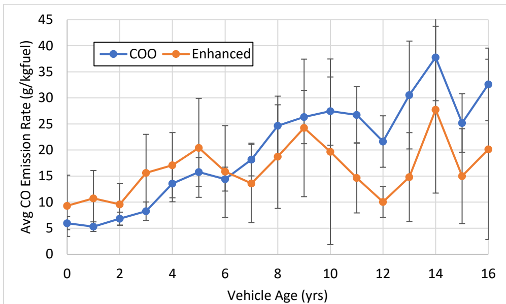
Figure 62. Average gasoline-powered LDV CO emissions by vehicle age, El Centro campaign. Error bars represent 95% confidence intervals.
