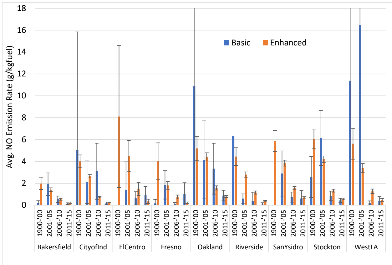
Figure 55. Average NO emissions by model year bin of Enhanced-area gasoline-powered LDVs vs Basic-area gasoline powered vehicles across all campaigns.
