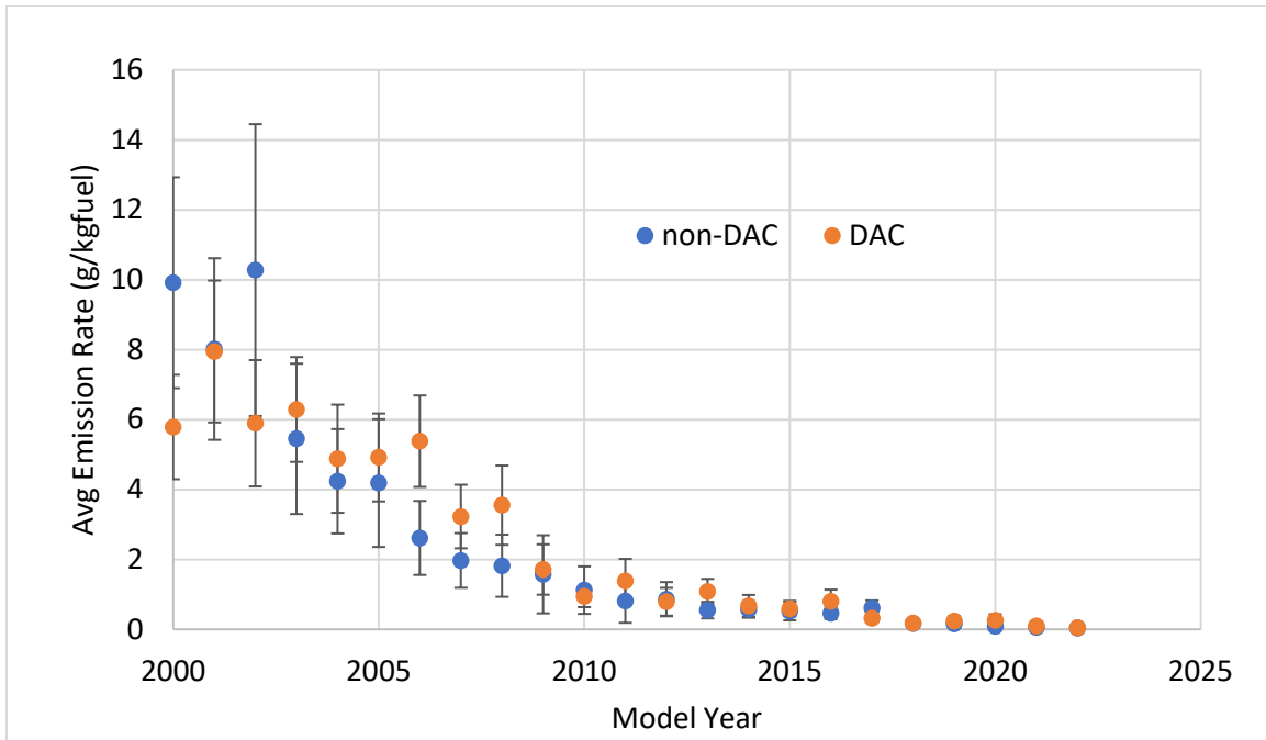
Figure 24. NO emission rates for non-DAC and DAC LDVs, averaged by model year for the El Centro campaign. Error bars indicate 95% confidence intervals.
