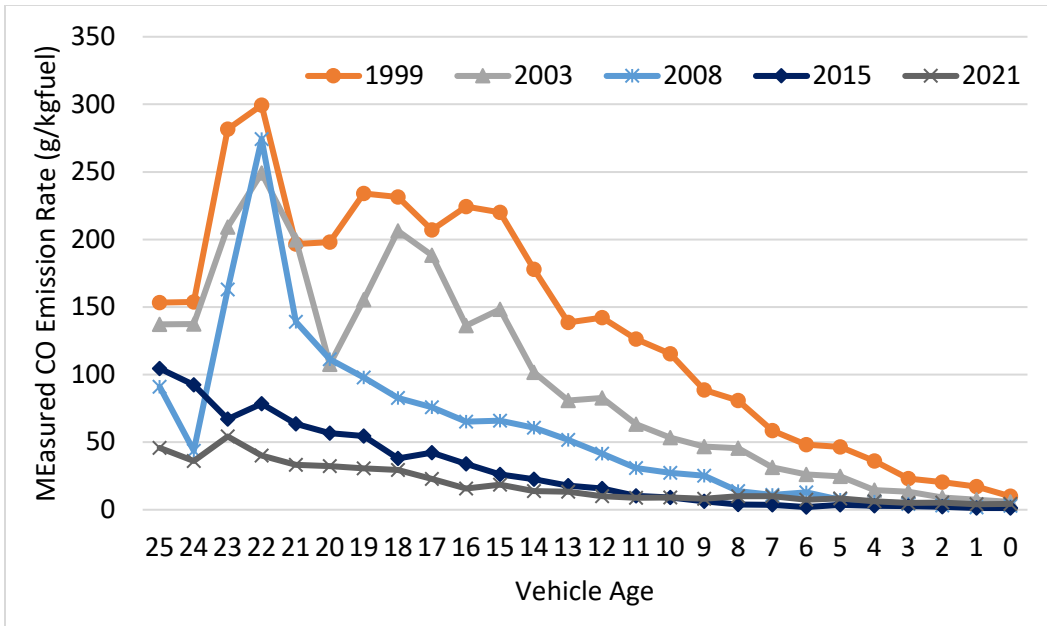
Figure 33. Average CO emission rates by vehicle age for the different measurement years
