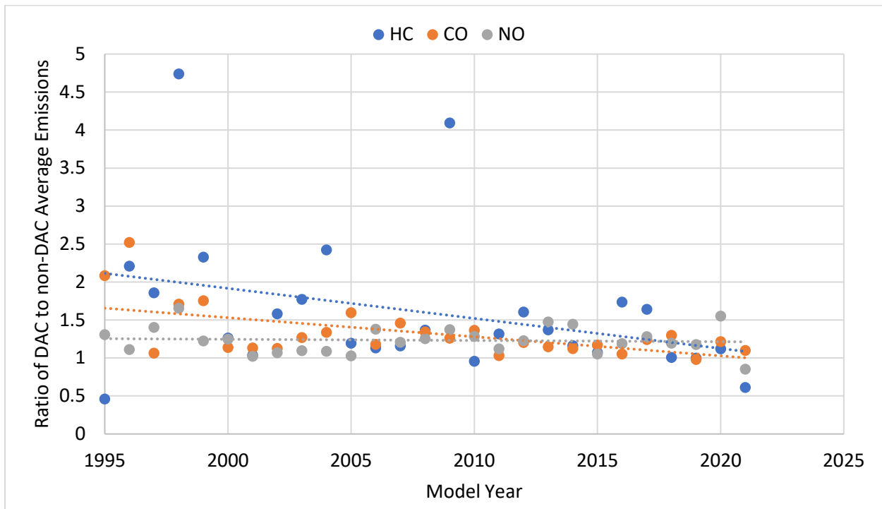
Figure 28. The campaign-averaged ratio of DAC to non-DAC emission rates by model year for HC, CO, and NO.
