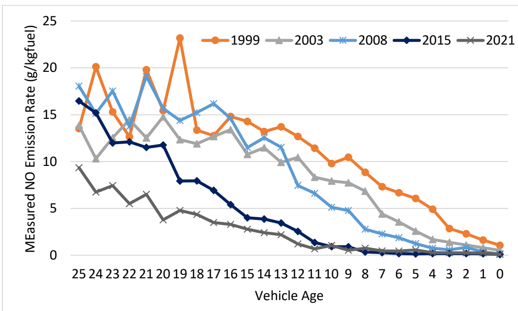
Figure 34. Average NO emission rates by vehicle age for the different measurement years
