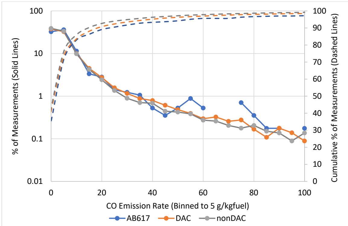
Figure 26. The distributions of CO emission rates for non-DAC, non-617 DAC, and AB617 community vehicles. Emission rates are binned to the nearest 5 g/gkfuel.
