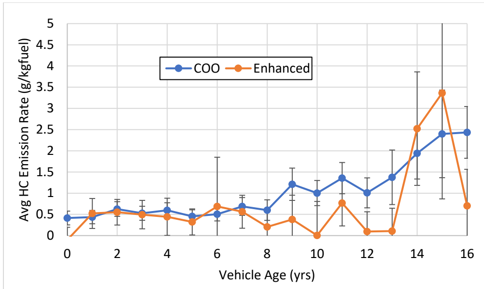
Figure 61. Average gasoline-powered LDV HC emissions by vehicle age, El Centro campaign. Error bars represent 95% confidence intervals.
