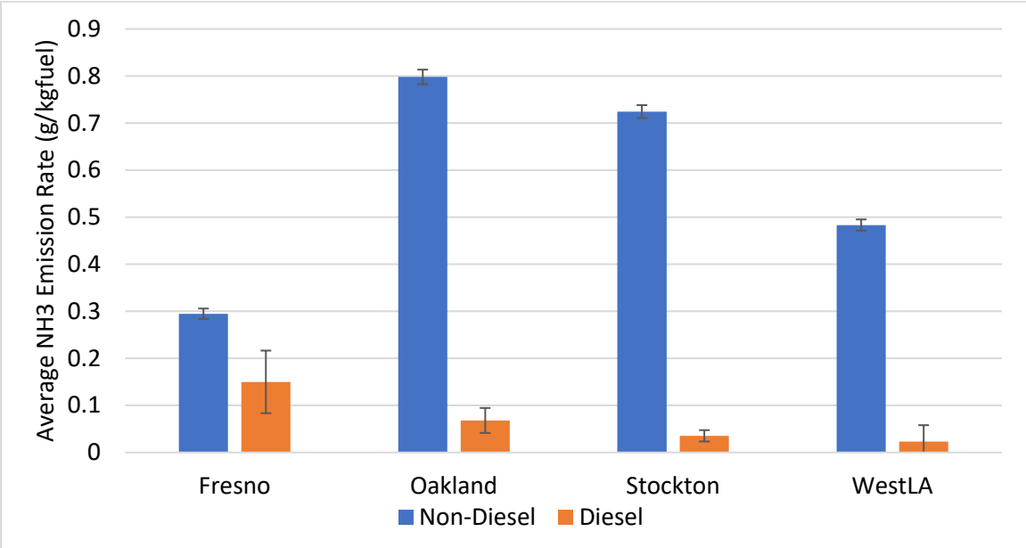
Figure D-1. Average NH 3 emission rates of LDVs by campaign and fuel type. Error bars represent 95% confidence intervals (CI).
