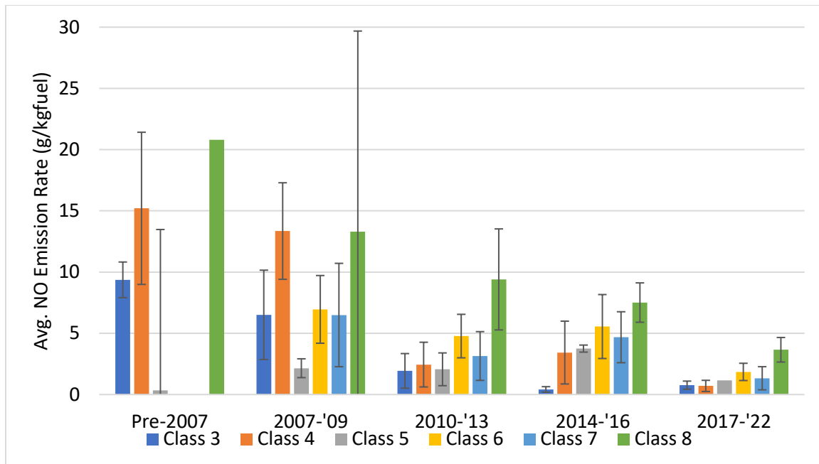
Figure 51. The average emission rate for all HDVs by each truck class and model year bin for all fuels, observed at the City of Industry campaign. Error bars indicate 95% confidence intervals.
