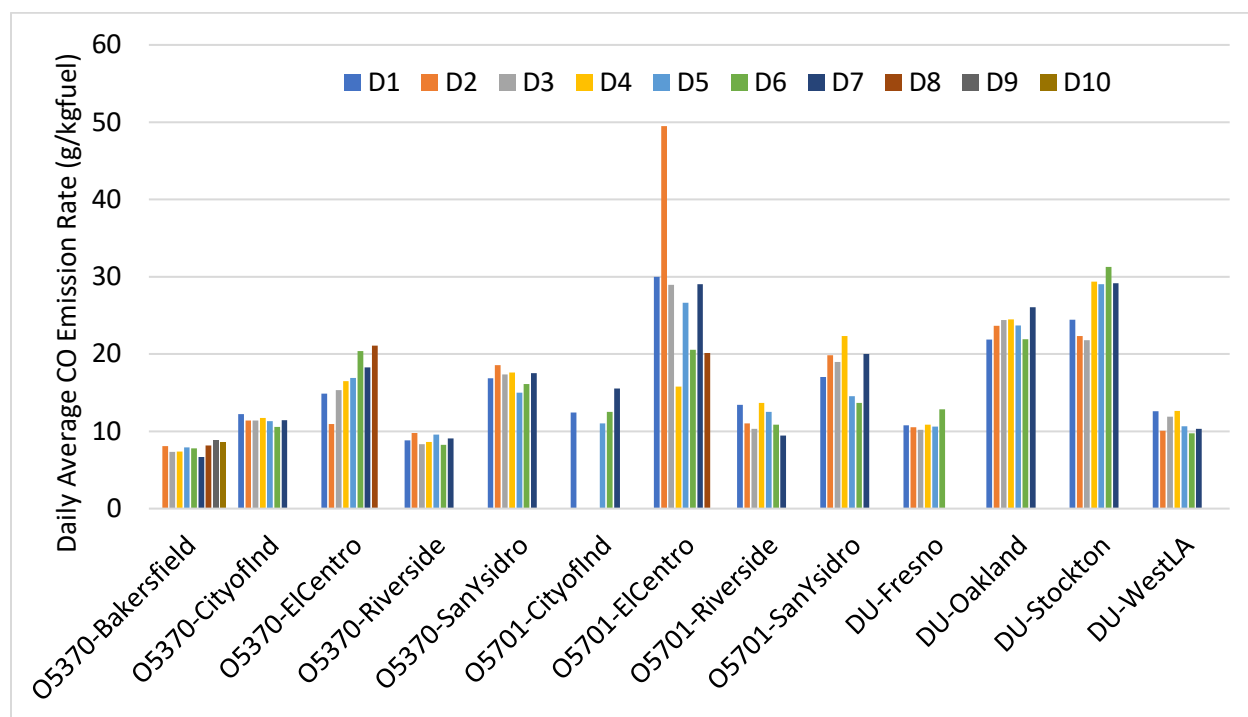
Figure 65. The average LDV CO emission rate by Subcontractor/Instrument and campaign, by campaign test day number (D#).
