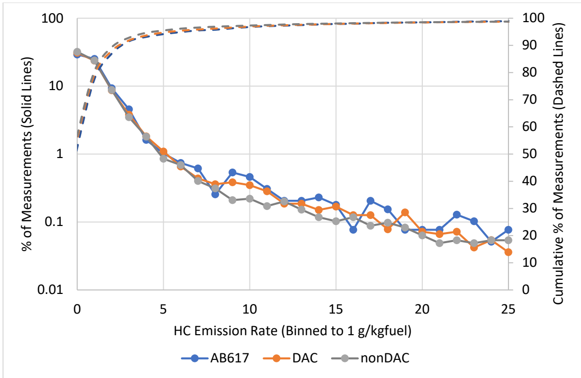
Figure 25. The distributions of HC emission rates for non-DAC, non-617 DAC, and AB617 community vehicles at the City of Industry campaign. Emission rates are binned to the nearest 1 g/gkfuel.
