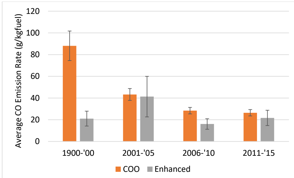
Figure 57. CO emission rate by model year bin for COO and Enhanced areas, averaged for gasoline vehicles observed at El Centro
