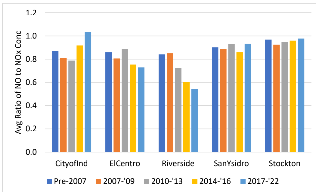
Figure 18. Average ratio of NO to NOx concentration for diesel-powered HDVs by model year bin and campaign.
