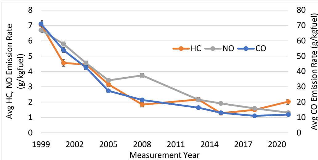
Figure ES-3. The overall-average emission rates of HC, NO, and CO at each La Brea Ave. campaign conducted by DU.
