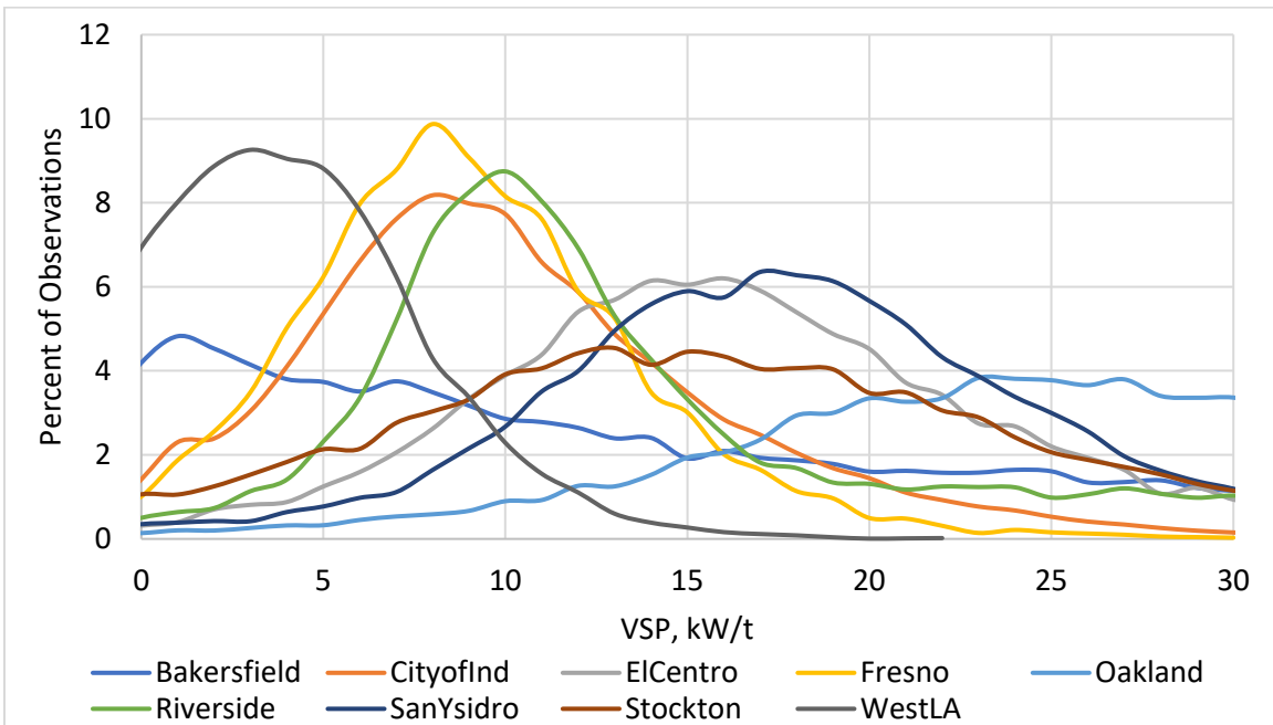
Figure 66. The distributions of LDV VSP observed during each campaign.
