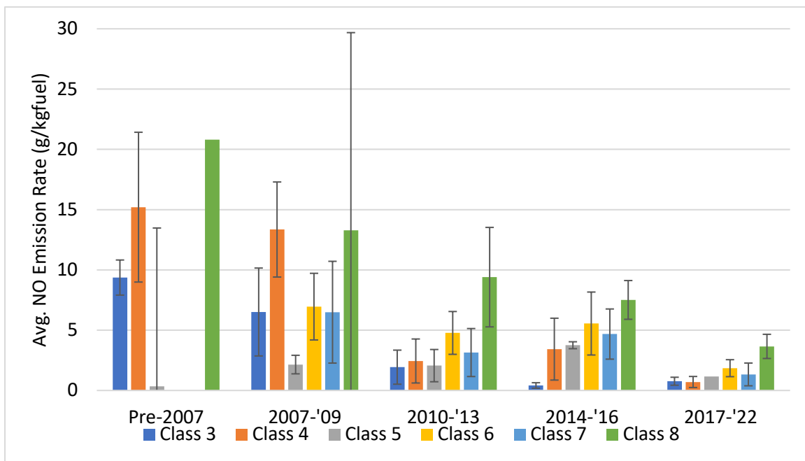
Figure 72. The average emission rate for all HDVs of each truck class and model year bin for all fuels at the City of Industry campaign. Error bars indicate 95% confidence intervals.
