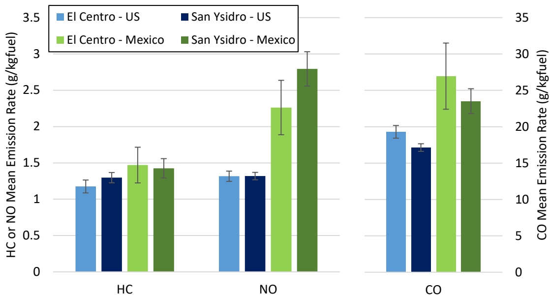
Figure 71. The average emission rates for the CA and Mexican fleets of vehicles at each border site. Error bars represent 95% confidence intervals.
