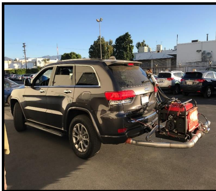
PEMS testing for excess on road emissions
